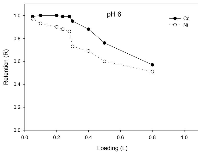
Figure 5.19: Retention Profiles of \text{Cd}^{2+} and \text{Ni}^{2+} in Binary Metal Mixtures at pH 6.5 and pH 6
