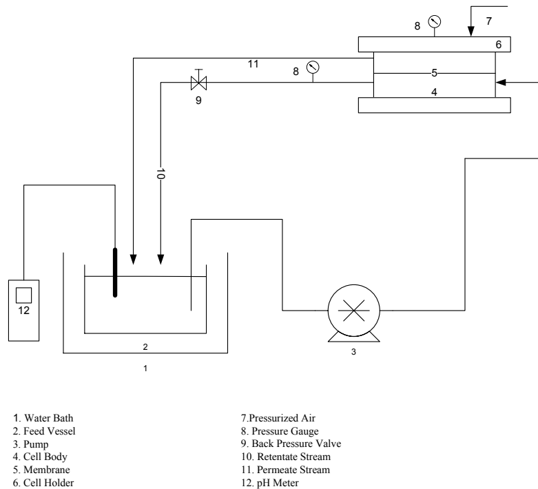
Figure 4.3: Schematic Diagram of Osmonics Sepa CF Membrane Cell
