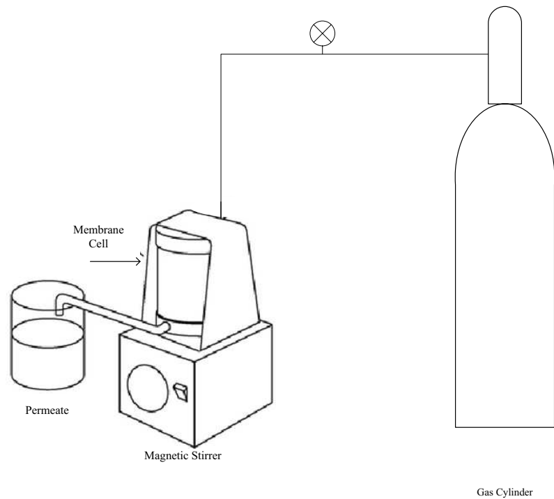
Figure 4.4: Schematic of Model 8050 Stirred Cell
