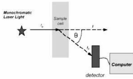
Figure 2.3: Schematic of Static Light Scattering
