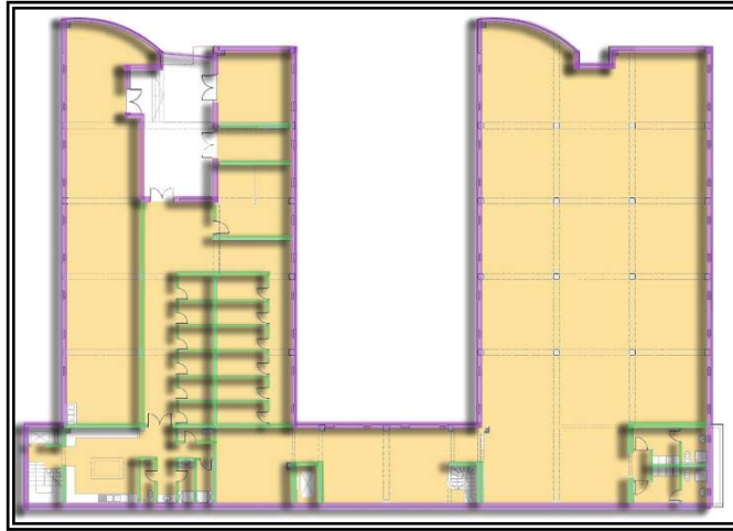
Figure 4.11 : Adopted basement floor plan of METU Twins. Source: METU Technopolis Coordination Office.
