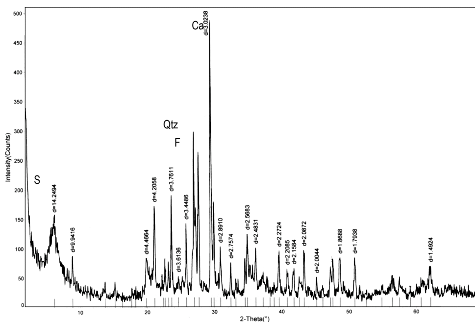
Figure 4.15 X-Ray diffraction pattern of the <170 mesh (bulk) fraction of the sample CRD 356. Qtz: Quartz, F: Feldspar, Ca: Calcite, S: Smectite; I: Illite, See Appendix-D for full size graphics.
