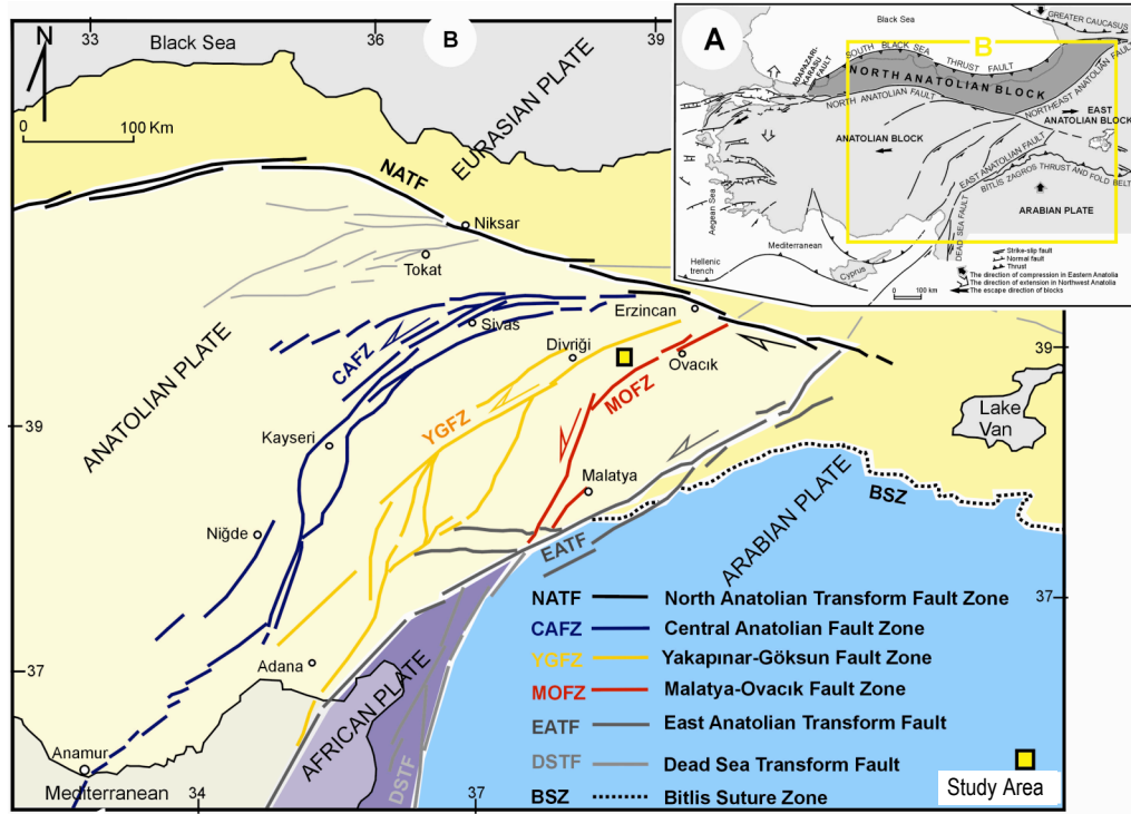
Figure 2.10 A: Major neotectonic elements of Anatolia (from Elmas, 1996) B: Simplified neotectonic map showing major tectonic escape induced structures in Eastern half of Turkey and the adjacent areas (from Sial, 2004).
