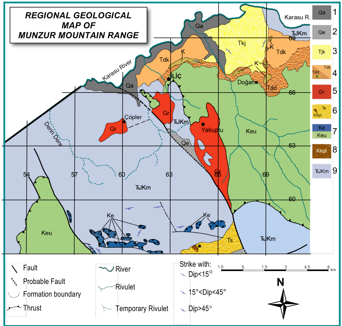
Figure 2.4 Map illustrating the regional geology in the vicinity of the study area (1:Quaternary alluvium, 2:Quaternary talus, 3:Kemah Formation, 4: Dedek Formation-Tdk: Koçkar volcanics member, Tdd: Dolugün Member, 5:Granite-Granodiorite intrusion, 6: Subaşı Formation, 7: Eriç ophiolitic mélangé-Ke: Undifferentiated, Keu: Uluyamaç member, 8: Pelagic Blocks of Kemaliye Formation, 9: Munzur Limestone) (After Özgül et al. , 1981).
