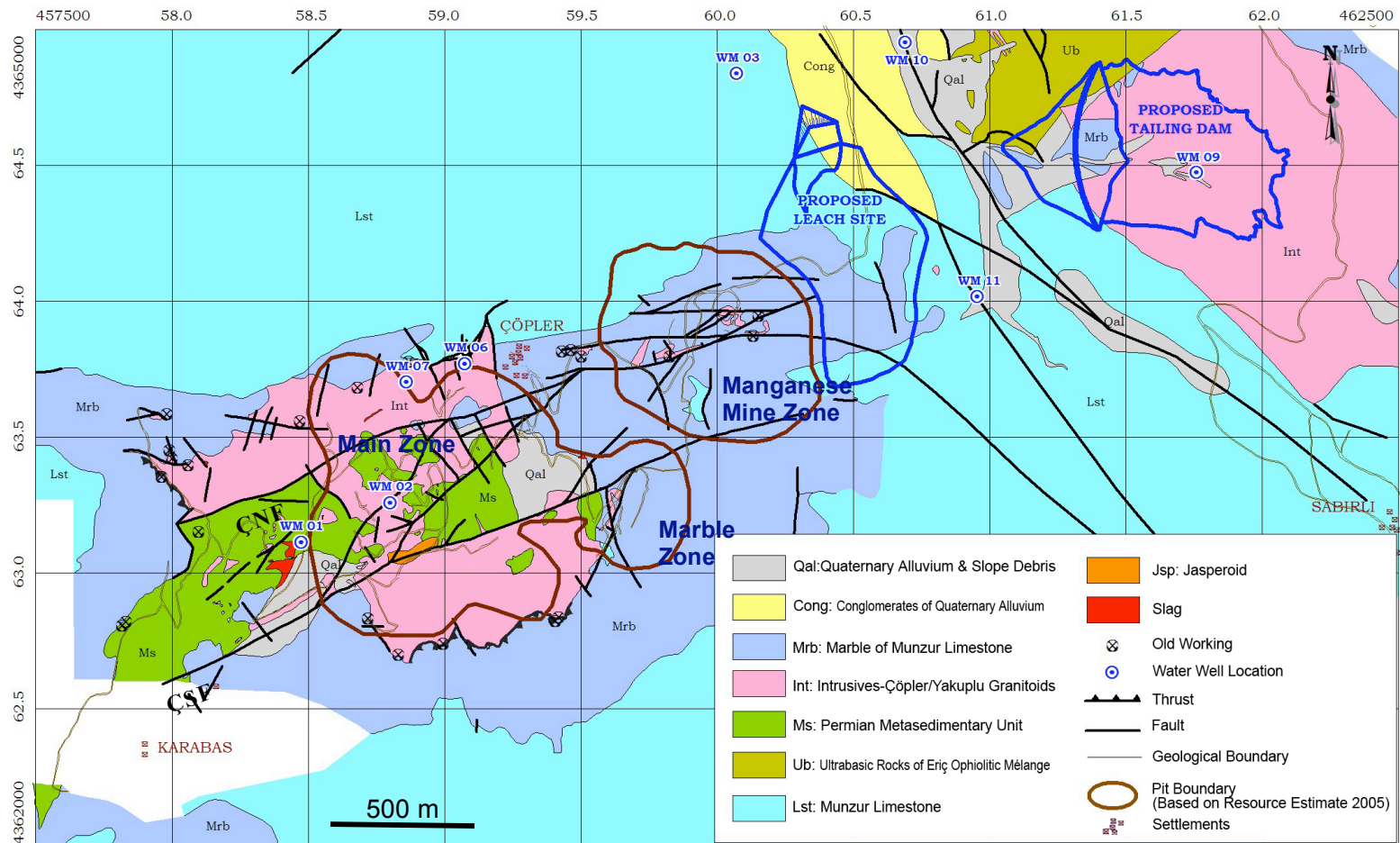
Figure 2.5 Detailed geology of the study area, ÇNF: Çöpler North Fault, ÇSF: Çöpler South Fault (Modified after Poyraz, 2005).
