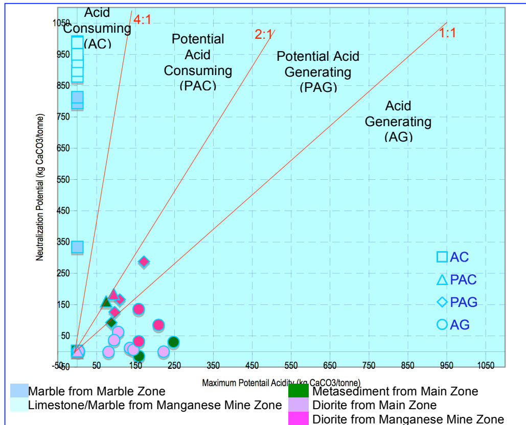
Figure 4.23 Distribution of the samples based on NPR values.
