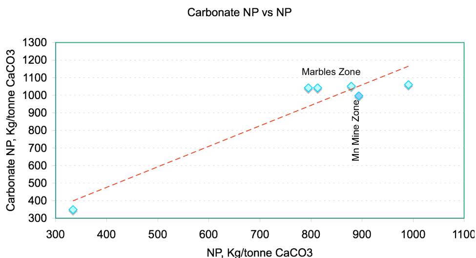
Figure 5.1 Carbonate Carbon Neutralization Potential vs. tested Neutralization Potential of some marbles from the marble zone and one limestone sample from the manganese mine zone.
