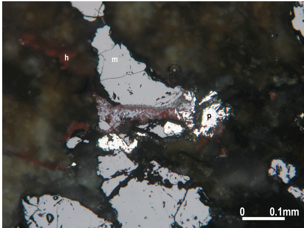
Figure 4.13 Subhedral to euhedral magnetite (m) with unhedral hematite (h) grains
