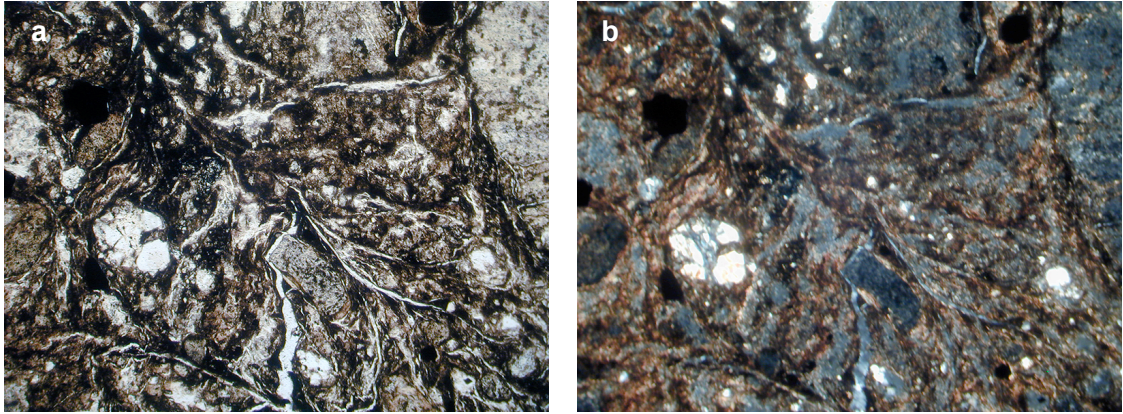
Figure 4.3 The thin section of the metasedimentary lithology that show rock fragments and small veinlets that indicate cataclastic activity; a: single nicole, b: cross nicole (Sample from CDD334) (magnification 100X).
