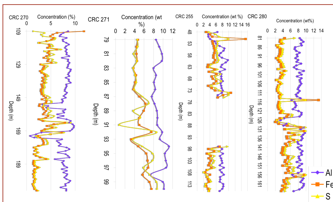
Figure 4.18 Fluctuation of %Al, %Fe and %S with respect to depth.
