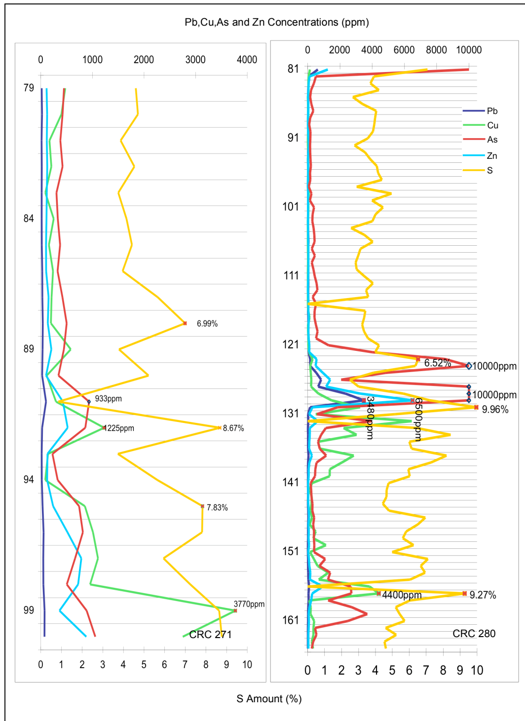
Figure 4.20 Variation of Pb, Cu, Zn and As concentrations in ppm and S content in percentage with respect to depth for drill hole samples CRC 271 and CRC 280 (The 10000 ppm is the upper detection limit of the reported analysis results, and 10% S is the upper detection limit of the reported results).
