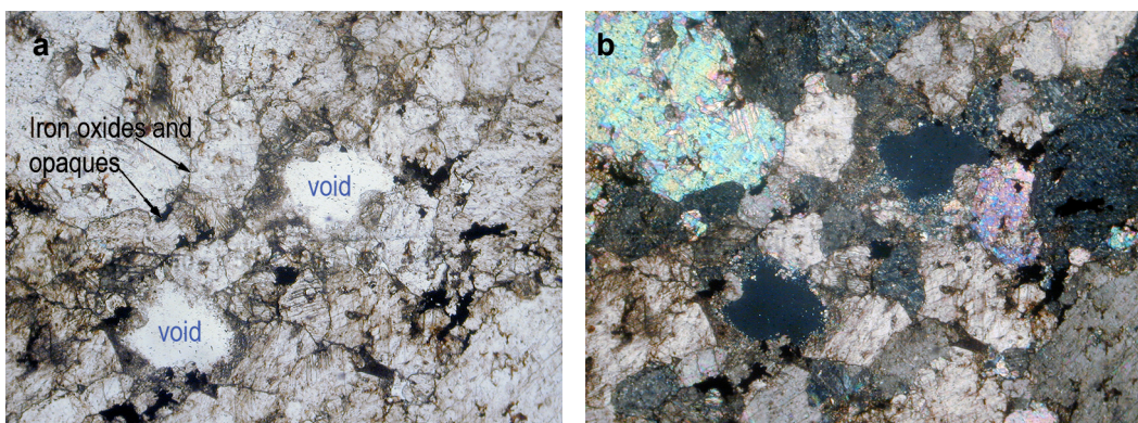
Figure 4.7 Karstic voids and mineral boundaries lined with iron oxides in marbles, , a: single nicole, b: cross nicole. (Sample CDD-98; 13m). (Magnification 45X).
