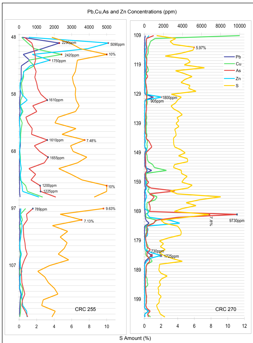
Figure 4.19 Variation of Pb, Cu, Zn and As concentrations in ppm and S content in percentage with respect to depth for samples from drill holes CRC 255 and CRC 270 (The 10000 ppm is the upper detection limit of the reported analysis results, and 10% S is the upper detection limit of the reported results).
