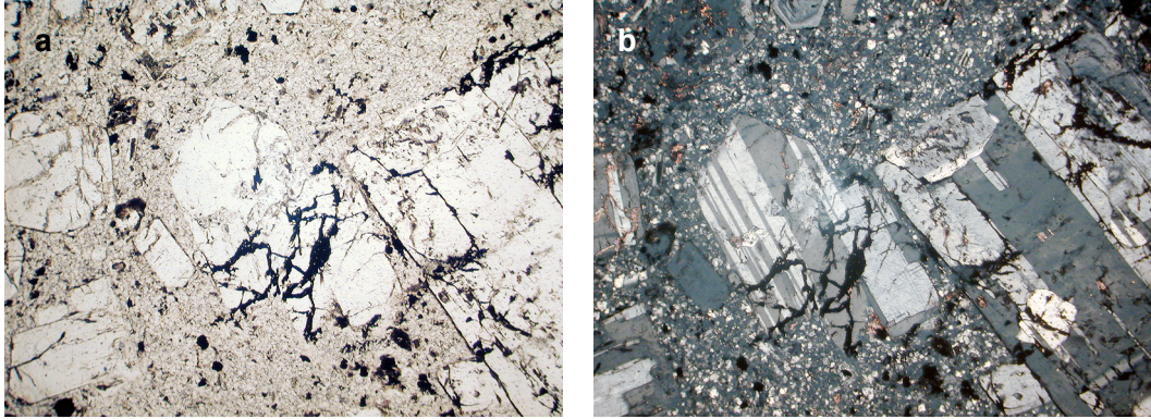
Figure 4.8 A sample (CDD-85) from Çöpler Granitoid exhibiting porphyritic texture with very fine grained silica matrix and highly deformed feldspar crystals, a: single nicole, b: cross nicole (Magnification 45X).
