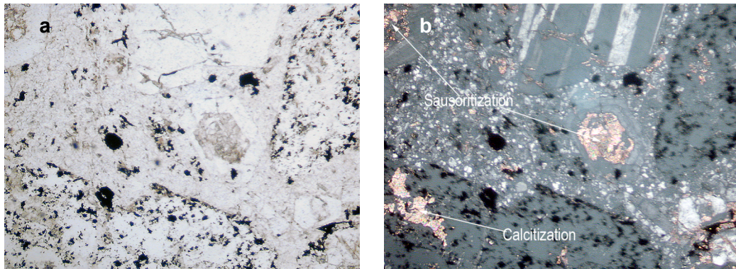
Figure 4.10 Plagioclase phenocrysts with saursoritization and calcitization (from CDD-84); a: single nicole, b: cross nicole. Magnification 45X.
