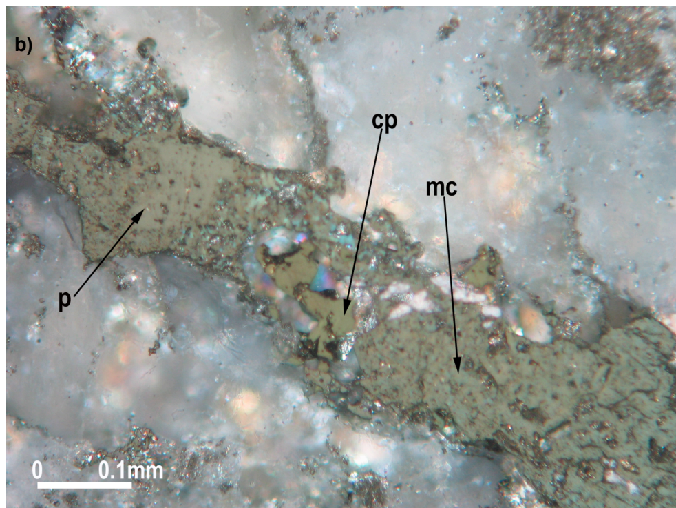
Figure 4.12 Vein filling pyrite (p), subhedral chalcopyrite (cp) and marcasites (mc) engulfed in pyrite fillings (a: picture with single nicole; b: picture with cross nicole).
