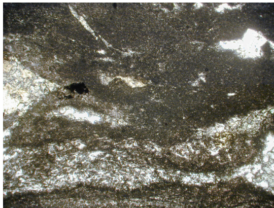
Figure 4.1 Fine clayey textures with boudinage like microstructures of a Metasedimentary rock sample (RMH02; 32.45-32.55) (Magnification 45X)
