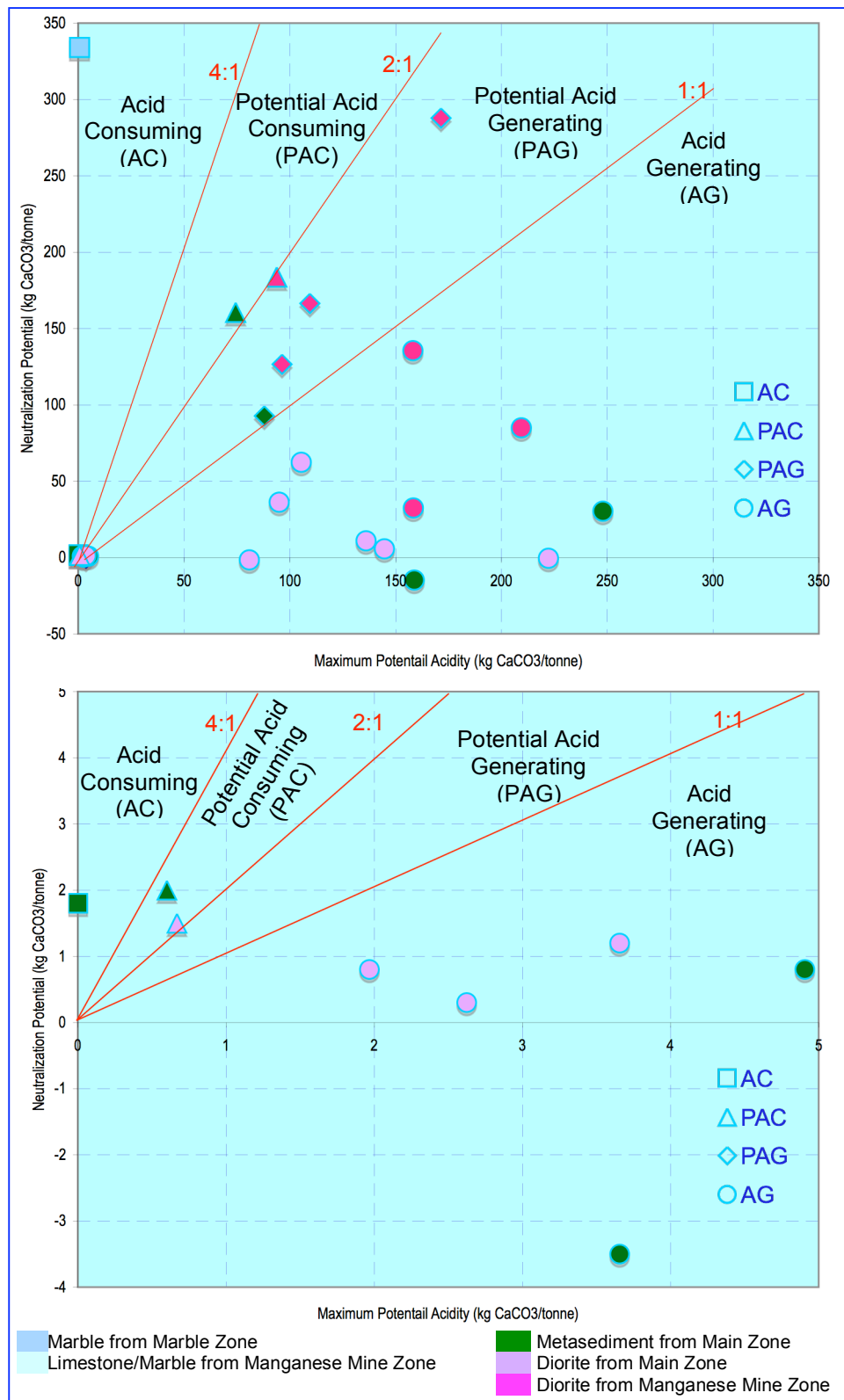
Figure 4.24 Graph that shows the NPR distribution of the tested samples in a detailed scale.
