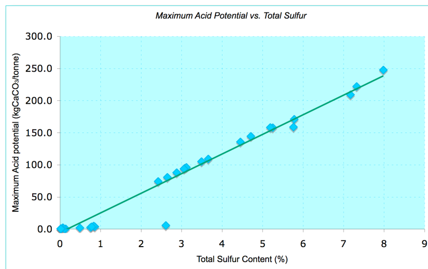
Figure 5.2 Graph indicating positive correlation between maximum potential acidity (MPA) and total sulfur content.
