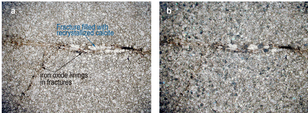
Figure 4.6 A Limestone sample (CDD 91) exhibiting fractures lined with iron oxides and filled with recrystallized calcite, a: single nicole, b: cross nicole. (Magnification 45X).
