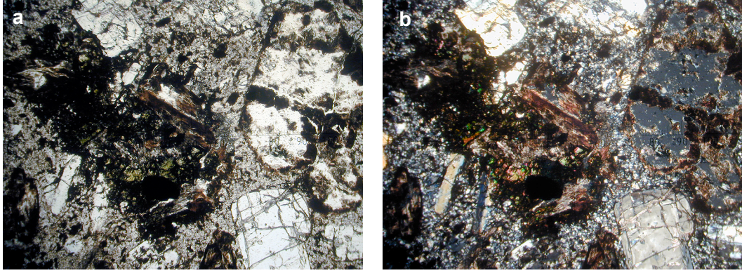
Figure 4.9 A Sample (CDD-99) from Dioritic Çöpler Granitoid exhibiting Phenocrysts with sericitization, opaques, kaolinitization, feldspath and ferromagnesian phenocrysts in a micro-silica matrix; a: single nicole, b: cross nicole. Magnification 45x.
