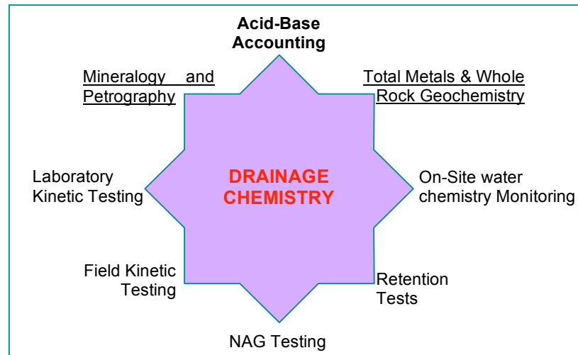
Figure 6.1 Significant issues that effect final drainage chemistry, modified after Morin and Hutt (2005).
