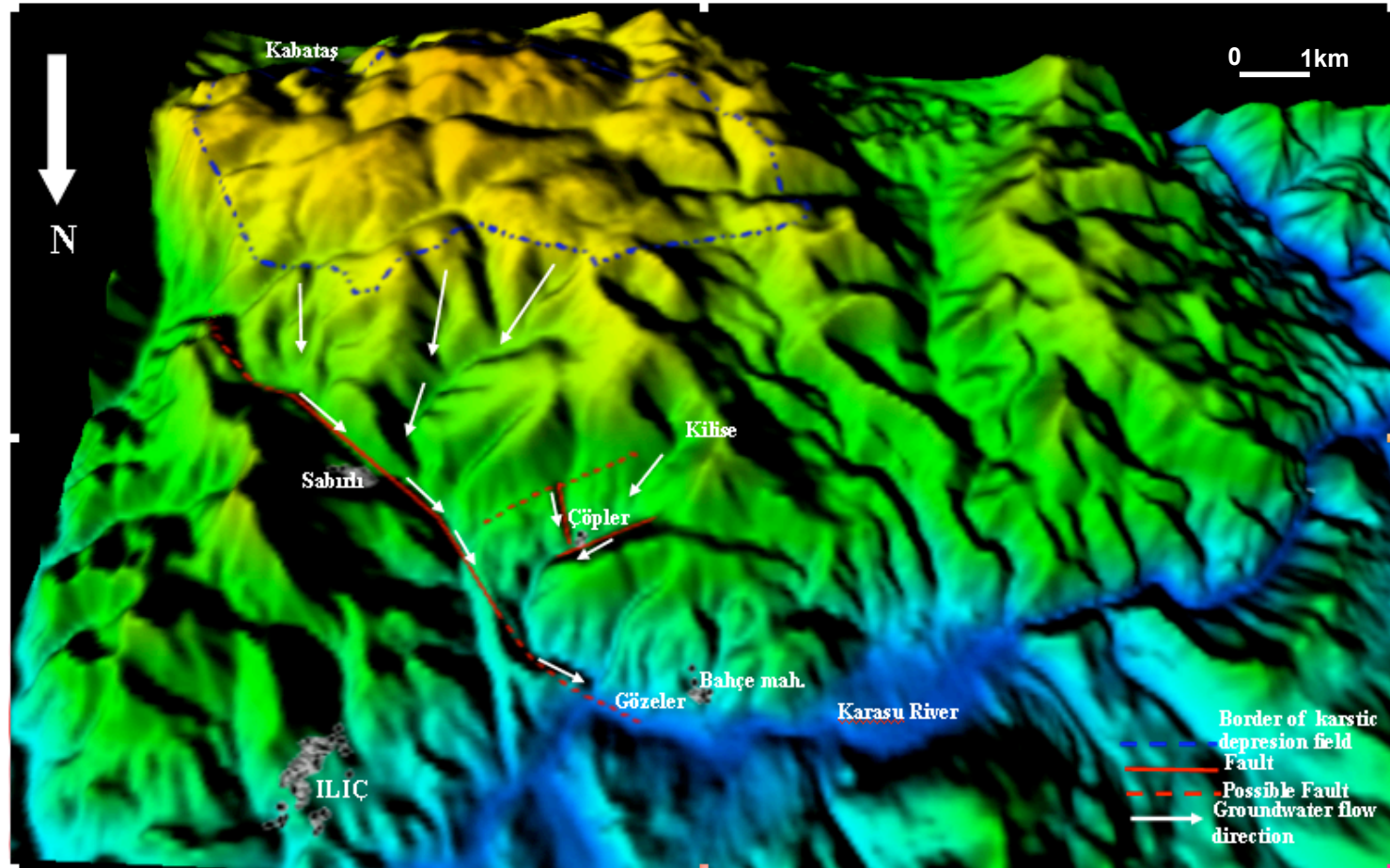
Figure 2.16 Conceptual model for groundwater movement in Çöpler region and surroundings. Model shown on a 3D topographic elevation model). (From Ekobil, 2005).
