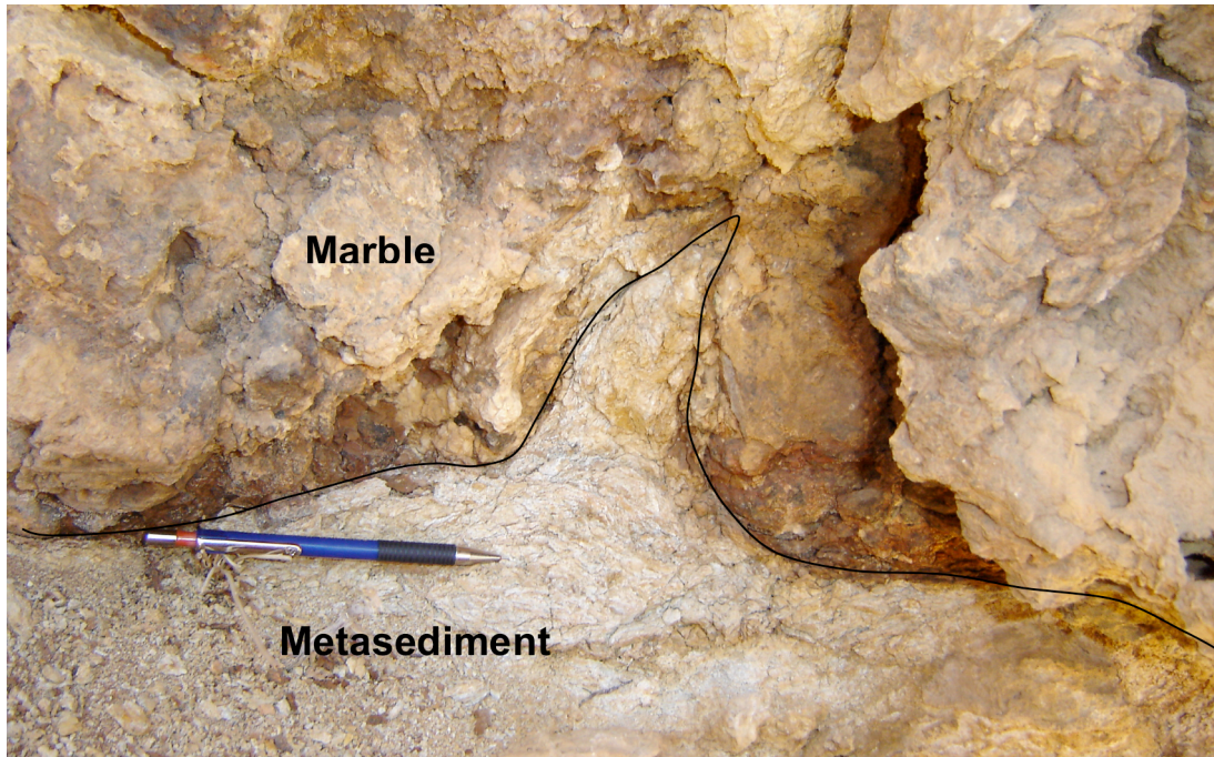
Figure 2.8 Munzur limestone exhibiting massive structures with indistinct bedding. It lies unconformably above the meta-sedimentary unit and its contacts display evidence of tectonic emplacement and soft-sediment flame structures (Easterday, 2004).
