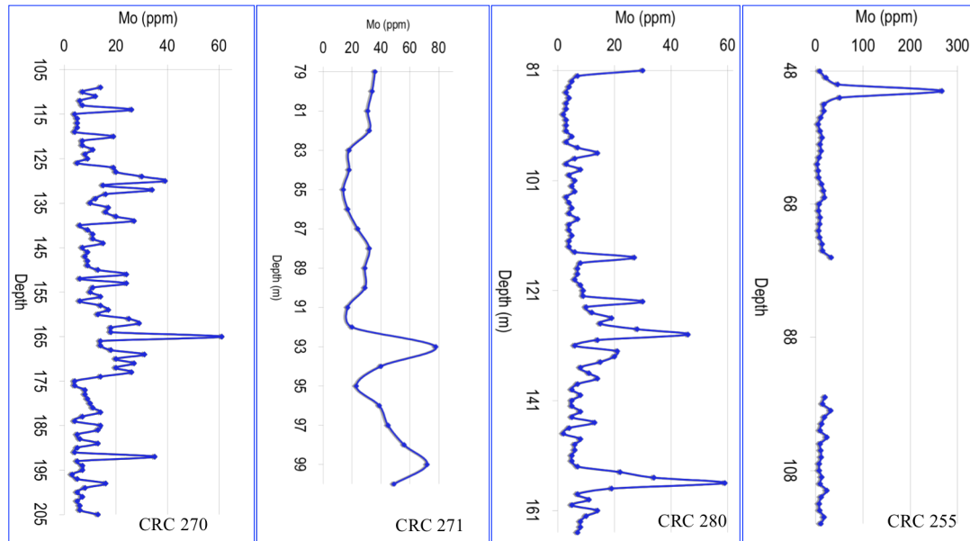
Figure 4.17 The change in Mo concentration with depth, in diorite drill hole samples. Elevated Mo concentrations indicate hydrothermal contribution.
