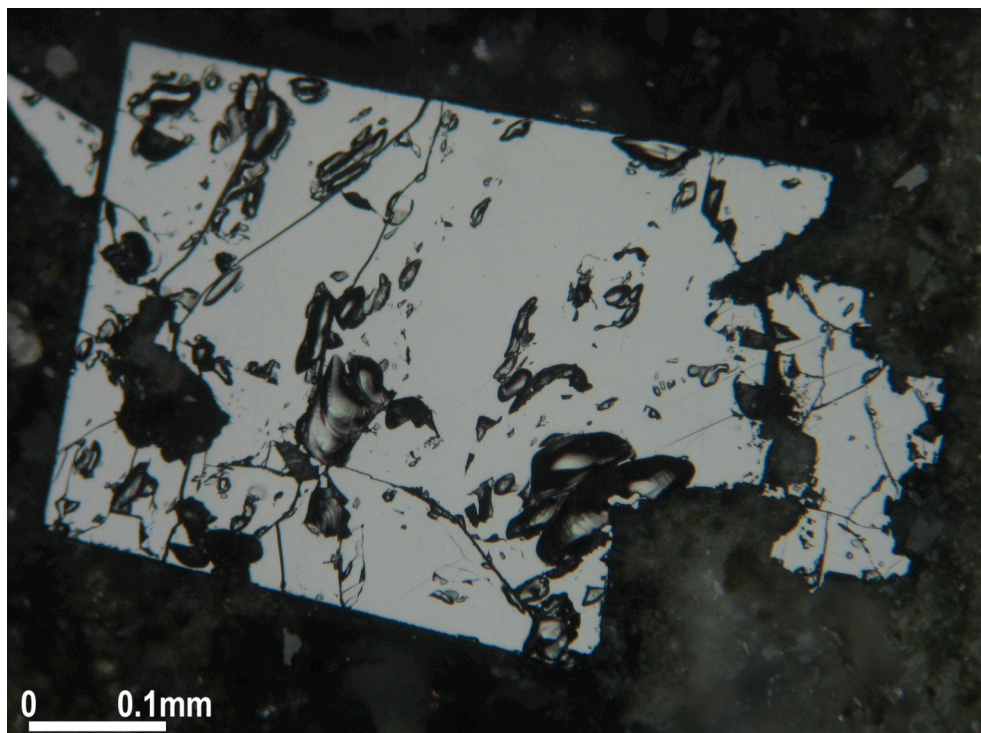
Figure 4.14 A large euhedral magnetite grain
