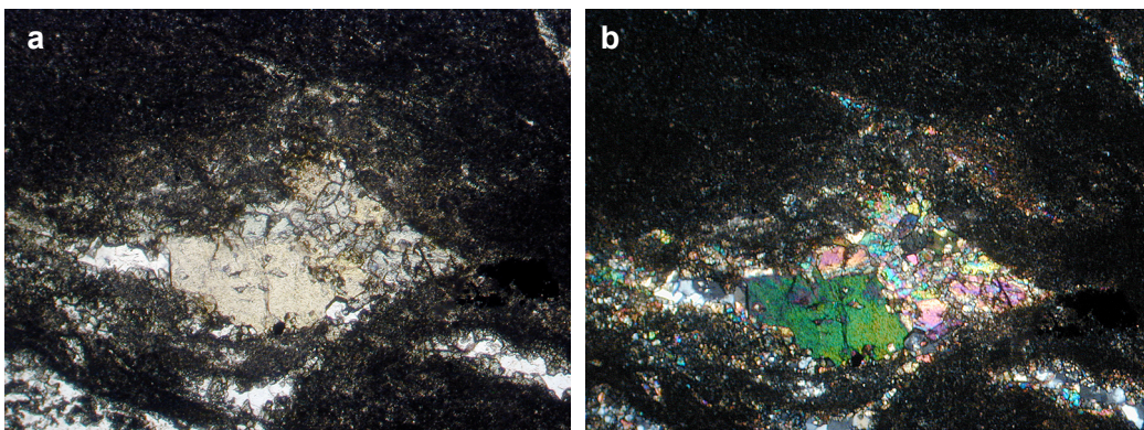
Figure 4.4 Metasedimentary rock sample (RMH02; 32.45-32.55) exhibiting epidotization, a: single nicole, b: cross nicole (magnification 100X).
