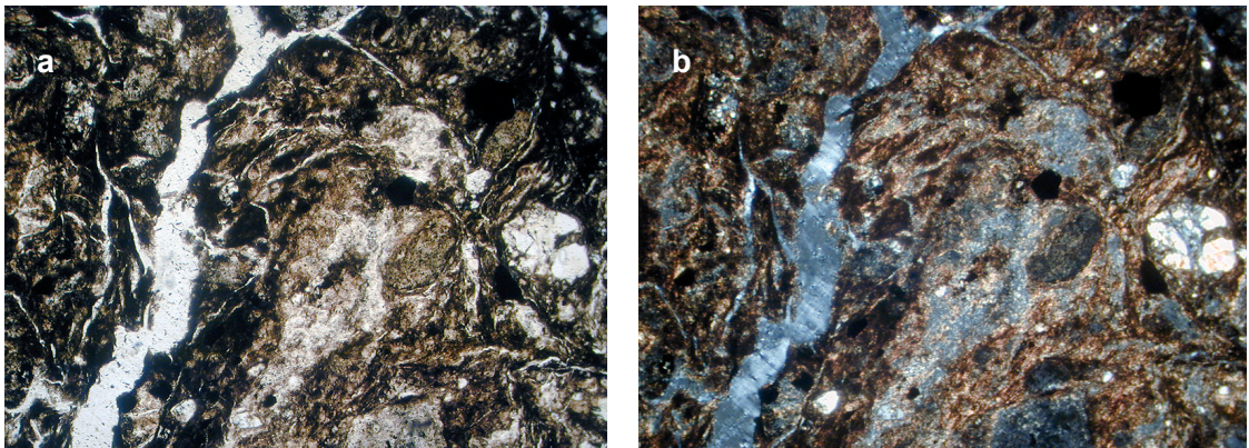
Figure 4.2 Metasedimentary lithology that exhibit major chalcedony veins, rock fragments and fine-grained clayey minerals. a: single nicole, b: cross nicole, magnification 45X (Sample from CDD334).
