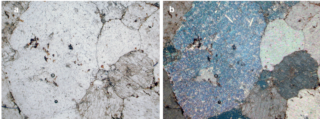
Figure 4.5 Microscopic view of a Marble sample (CDD-98;51.7-51.9) with large euhedral to subhedral calcite crystals, a: single nicole, b: cross nicole (Magnification 45X)
