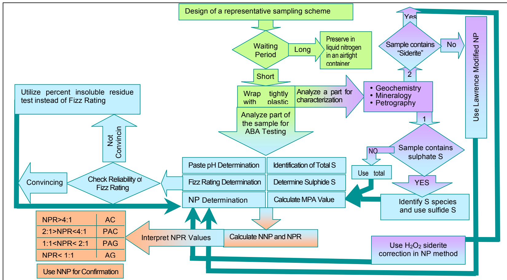
Figure 3.3 Flow Chart Summarizing Acid Base Accounting procedures and critical issues to be considered.
