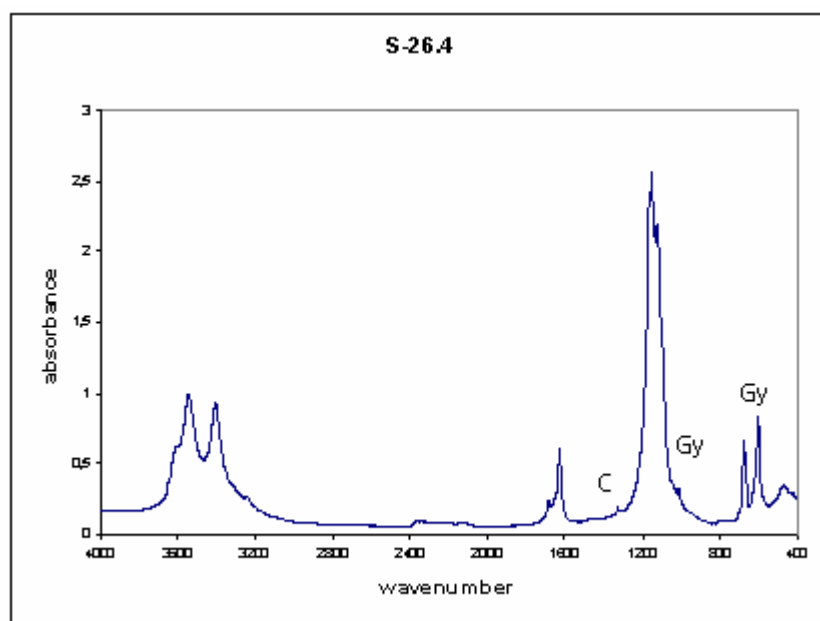
Figure 3.42 FTIR trace of S-26.4 layer at: 2% CH 3 COOH treated.
