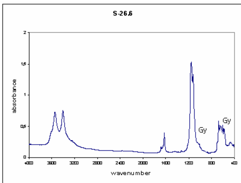
Figure 3.44 FTIR trace of S-26.6 layer at: 2% CH 3 COOH treated.
