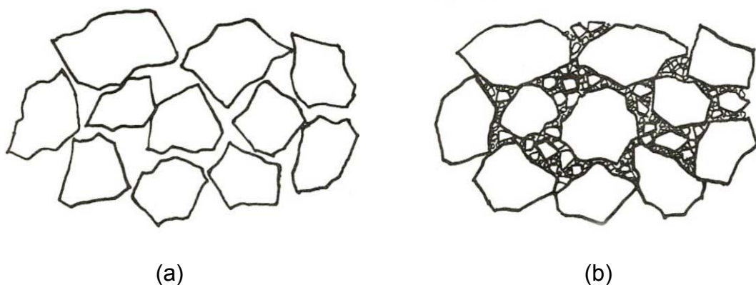
Figure 1.1 Distribution of sand grains (a) Badly graded sand (b) Well graded sand
