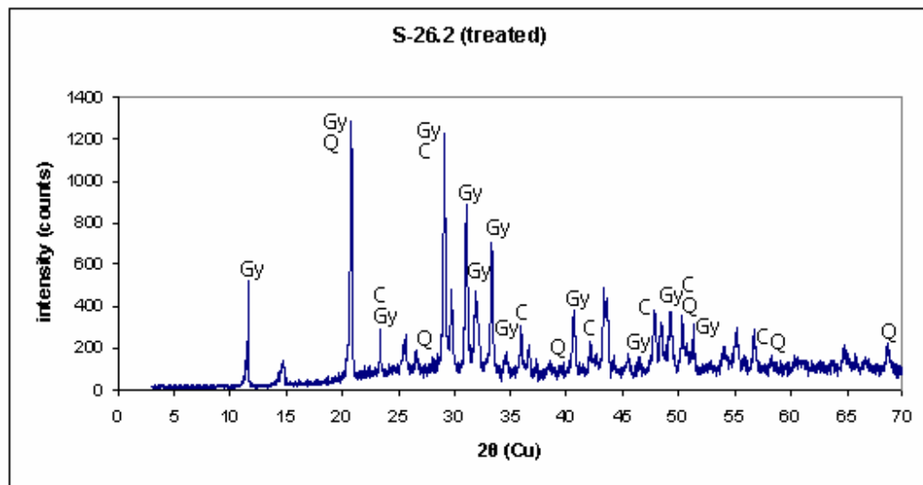
Figure 3.20 (a) XRD trace of S-26.2 rough plaster layers (b) XRD trace of S-26.2 treated plaster layers C: Calcite, Gy: Gypsum, Q: Quartz
