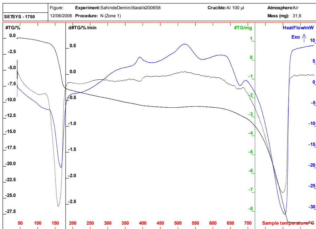
Figure 3.51 TGA trace of a green plaster layer S-26.6
