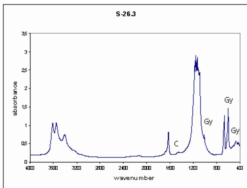
Figure 3.41 FTIR trace of S-26.3 layer at: 2% CH 3 COOH treated.
