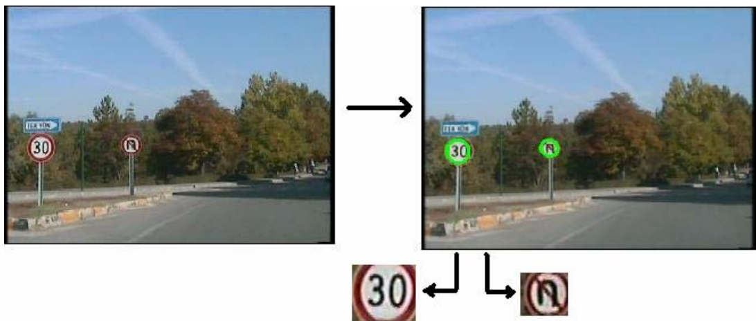
Figure 3.13: Traffic scene with circular signs taken in a sunny day with detected and cropped circular signs
