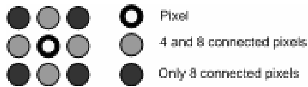
Figure 2.9: Pixel connectivity to neighbor pixels
