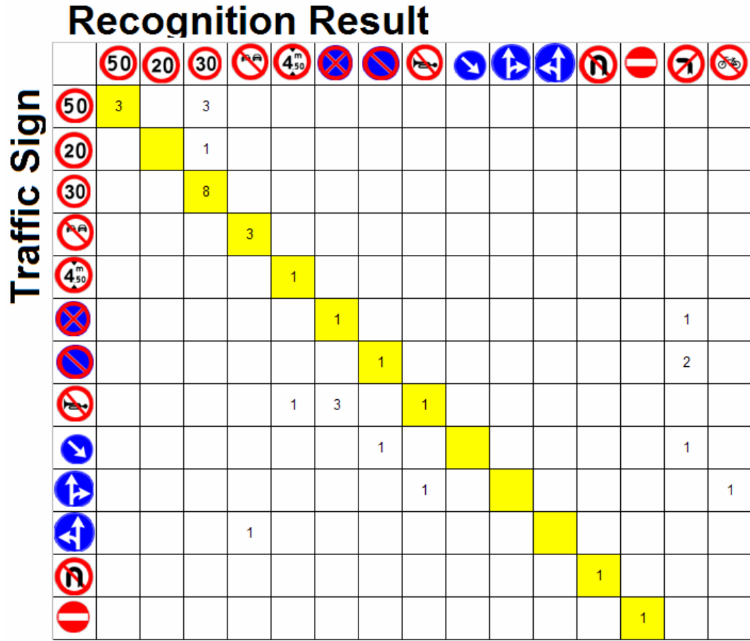
Figure 5.65: Confusion matrix for Table 5.41, for circular signs in Figure 5.64
