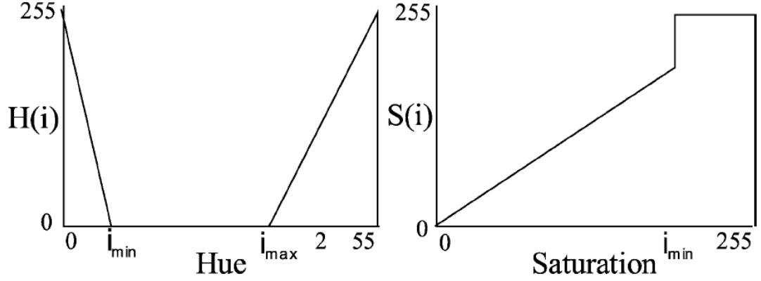
Figure 2.1: Hue for red and saturation transfer functions [35] [43]
