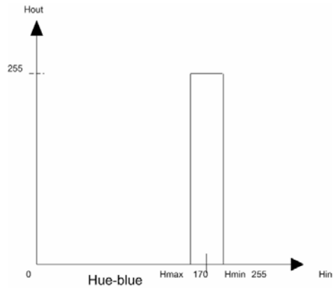
Figure 2.6: Hue transfer function for blue [28]
