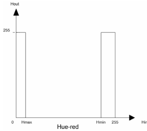
Figure 2.4: Hue transfer function for red [28]
