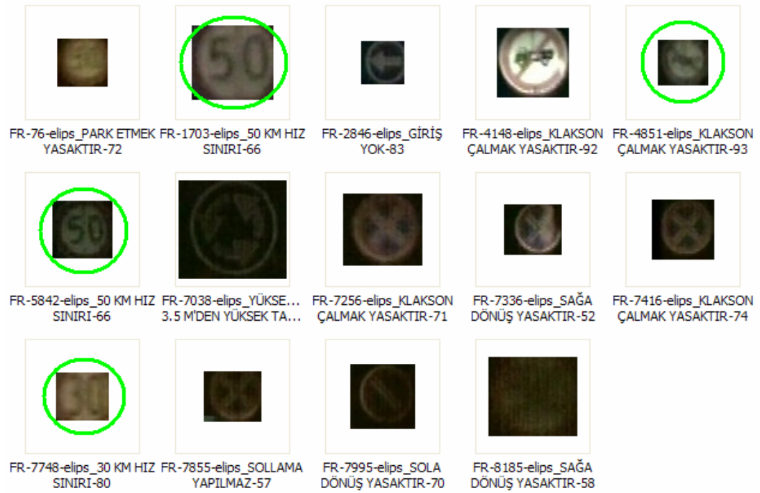
Figure 5.35: Detected and recognized circular signs for parameter Set-2 and Threshold Set-2 (5 levels) for Table 5.23
