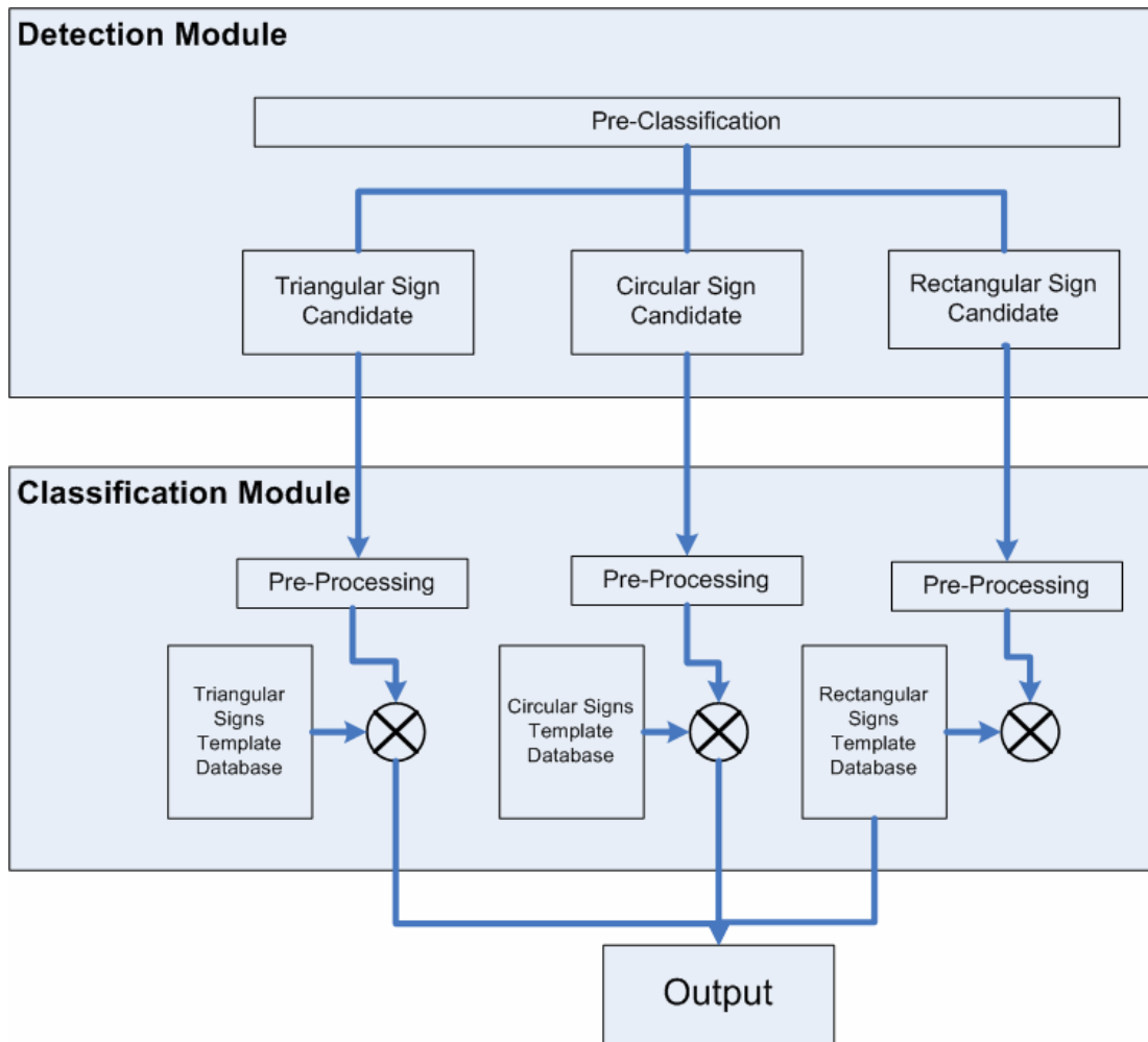
Figure 4.11: Simplified block diagram of recognition scheme
