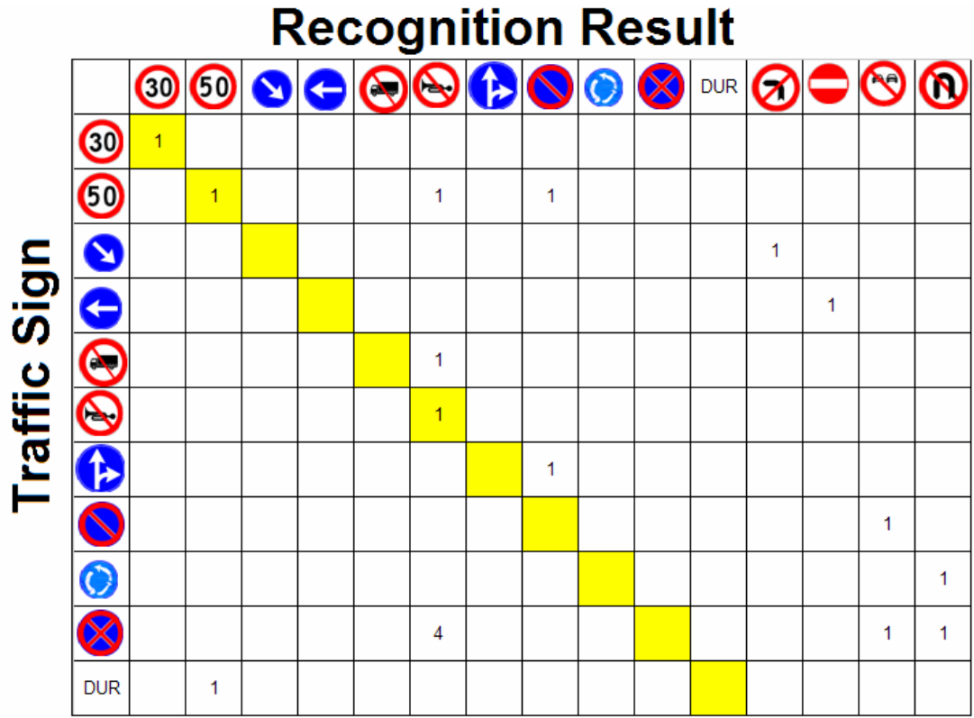
Figure 5.21: Confusion matrix for Table 5.19, for circular signs in Figure 5.20
