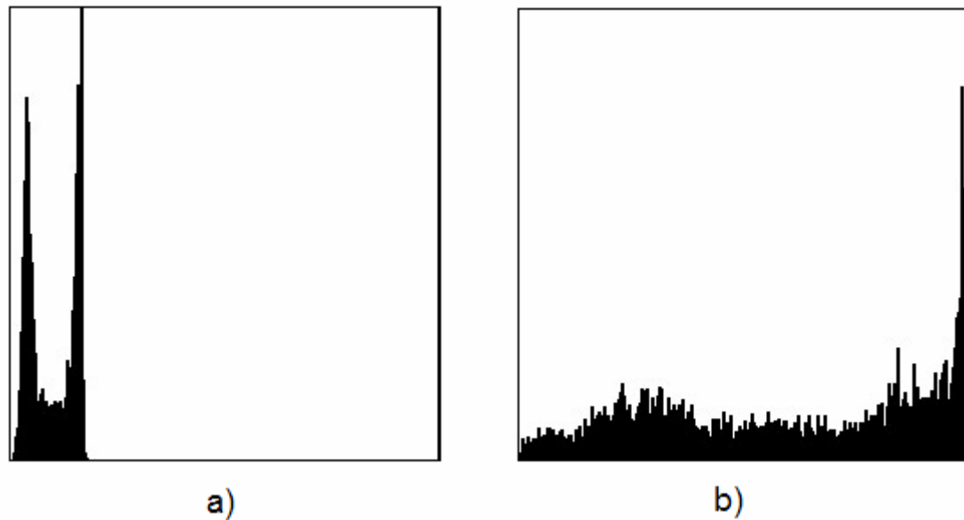
Figure 4.8: (a) Histogram graph of traffic sign candidate image in Figure 4.7-c before applying histogram equalization, (b) histogram graph of traffic sign candidate image in Figure 4.7-d after applying histogram equalization
