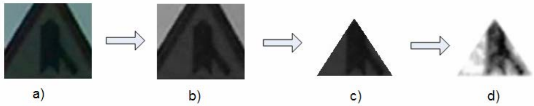
Figure 4.7: (a) Transformed, RGB, traffic sign candidate image, (b) V channel of HSV equivalent transformed image, (c) masked image where the region around traffic sign is cut out, (d) traffic sign candidate after histogram equalization
