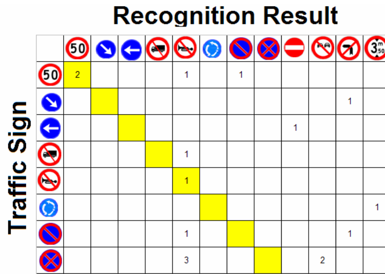
Figure 5.25: Confusion matrix for Table 5.20, for circular signs in Figure 5.24
