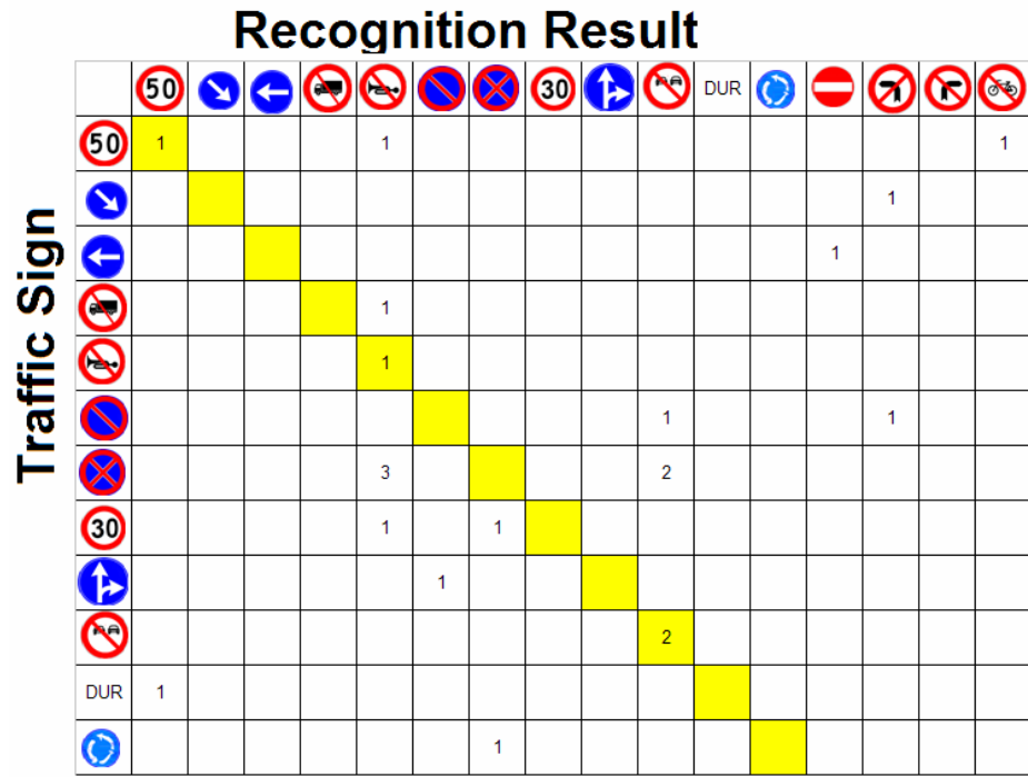
Figure 5.32: Confusion matrix for Table 5.22, for circular signs in Figure 5.31
