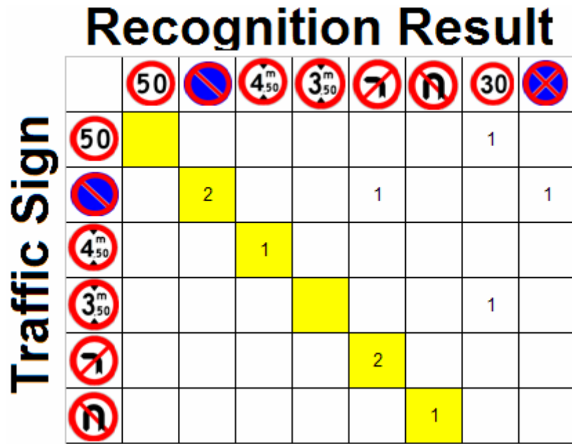
Figure 5.57: Confusion matrix for Table 5.36, for circular signs in Figure 5.56
