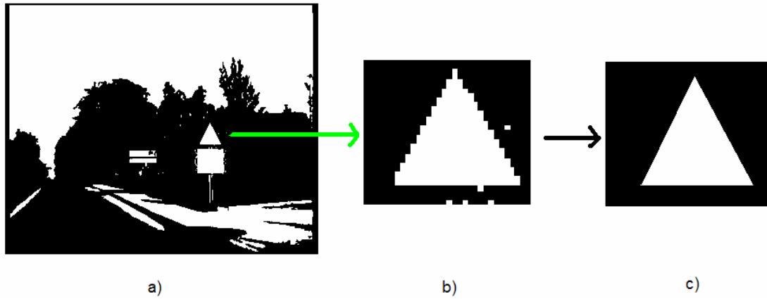
Figure 3.3: a) Level-9 binary threshold contour representation, b) enlarged view of triangular object which is to be checked as a candidate of traffic sign, c) illustration of polyline approximation output by Douglas-Peucker algorithm [52]
