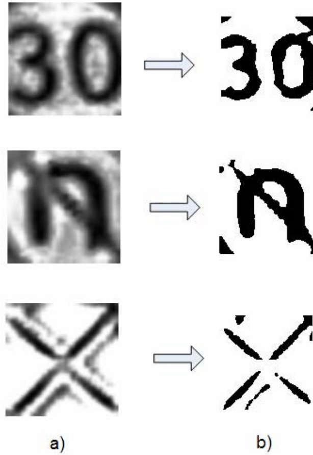
Figure 4.10: (a) Examples of circular traffic sign candidates after histogram equalization, (b) ideograms extracted after shrinking and binary threshold
