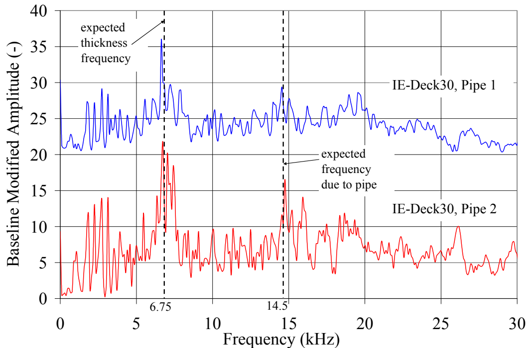
Figure 4.22 Two of the resulting spectra obtained from pipes in IE-Deck30
