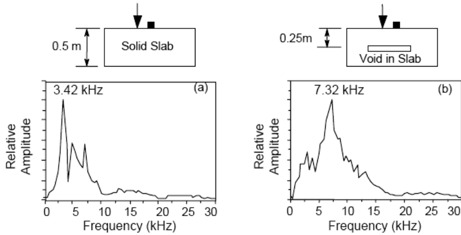
Figure 2.6 The resulting spectra with and without a void in a slab [1]
