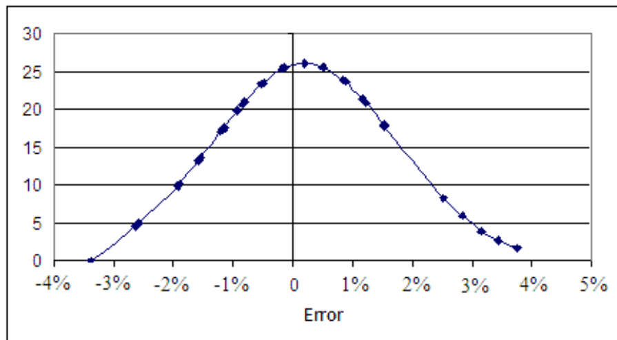
b-) The graph of 56 data points drawn as a probability density function (pdf)
