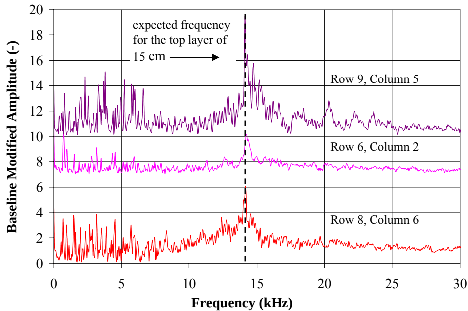
Figure 4.28 Sample resulting graphs while testing the effects of base layer when there is an aggregate layer below the concrete section
