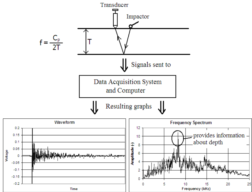
Figure 2.3 Schematic description of the impact-echo test procedure
