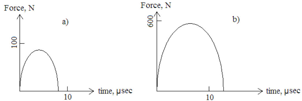
Figure 2.8 Force-time diagrams of impacts caused by two different steel impactors: a) 3 mm diameter b) 6.5 mm diameter
