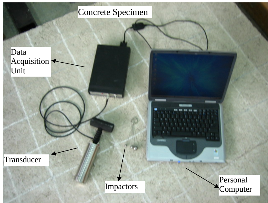
Figure 2.7 The main components of the impact-echo method
