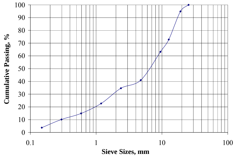
Figure 4.26 The gradation of the aggregates used to create a layer in between the two slabs
