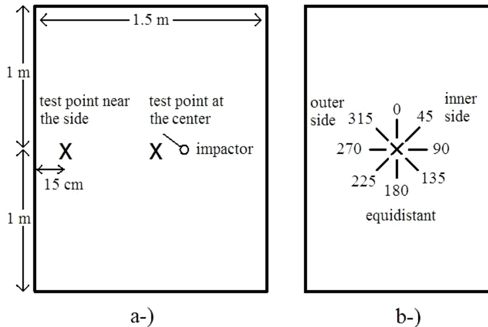
Figure 4.8 Schematic view of the test locations a-) Location of test point at the center and near the side b-) Grouping of recordings obtained at various angles
