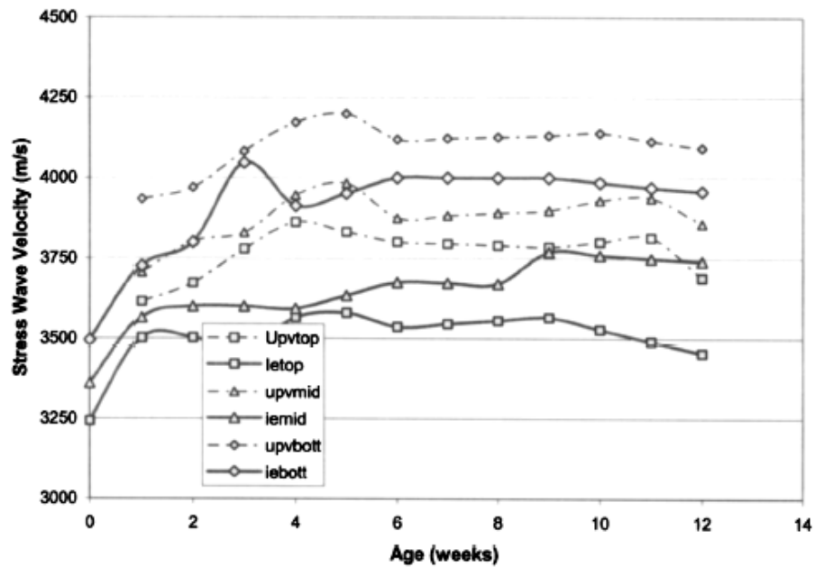
Figure 2.11 Comparative wave velocities in a concrete specimen with 0.65 W/C ratio [11]
