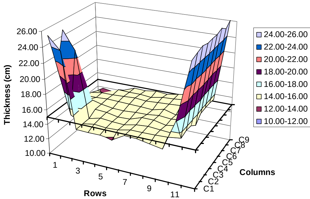
a-) Thickness values found by using impact-echo from IE-Deck15
