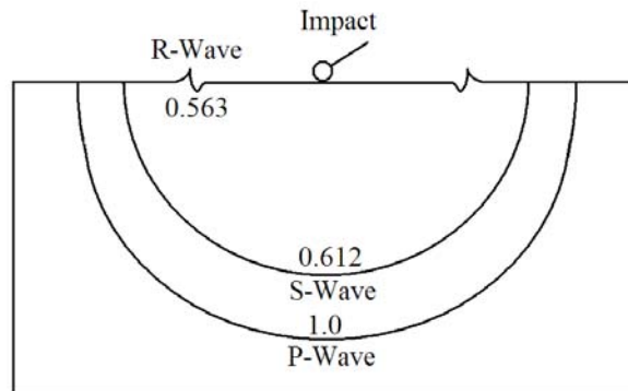
Figure 2.1 The relative position of different types of waves created by an impact. Numbers indicate relative values normalized according to P-wave speed.
