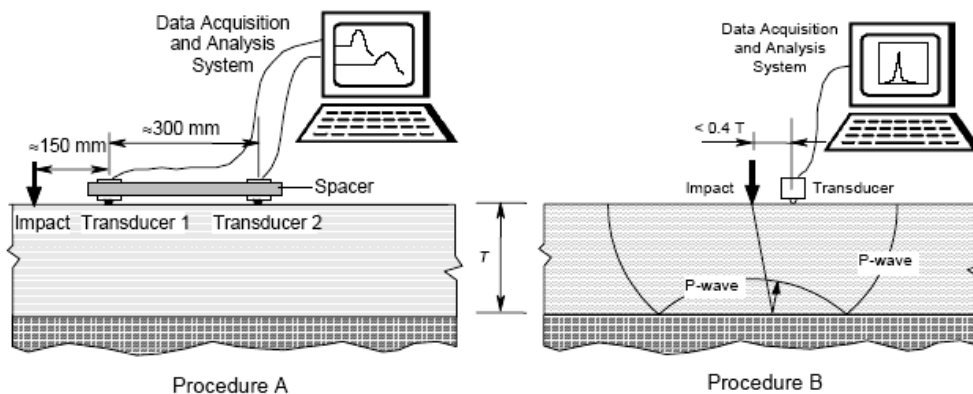
Figure 2.12 Procedure to be followed for impact-echo testing [16]
