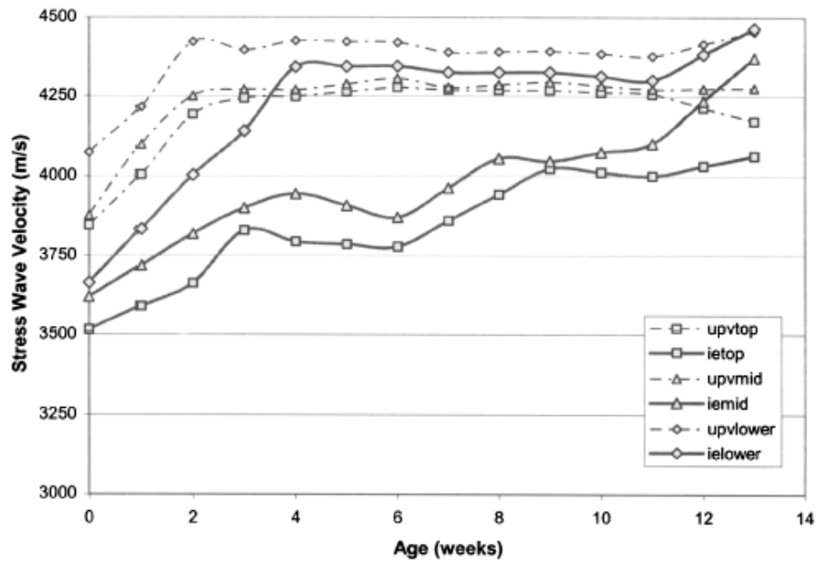
Figure 2.10 The increase in wave velocities with time in a concrete specimen with 0.45 W/C ratio. A comparison is also shown between the impact-echo and the ultrasonic pulse method. [11]
