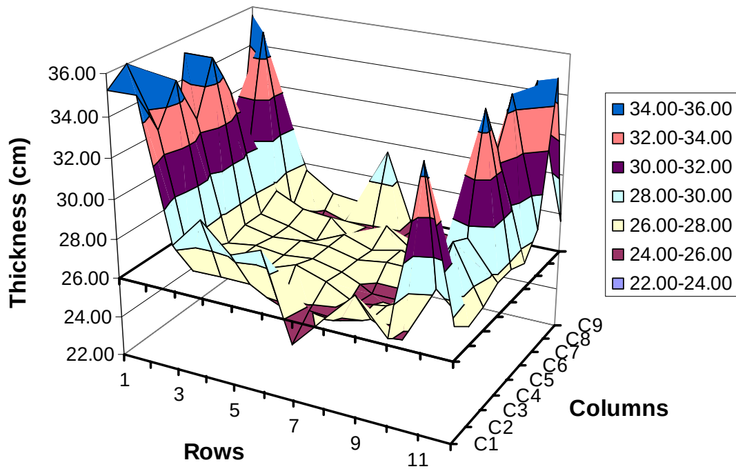
b-) Thickness values found by using impact-echo from IE-Deck25
