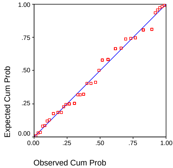
a-) Normal P-P plot of error percentages
