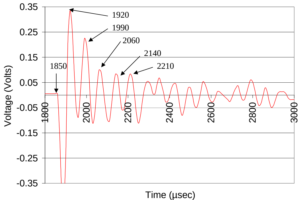
Figure 2.5 A sample waveform used for calculating the thickness frequency using the time domain approach
