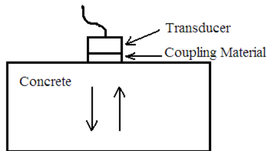
Figure 2.2 Working principle of pulse-echo method
