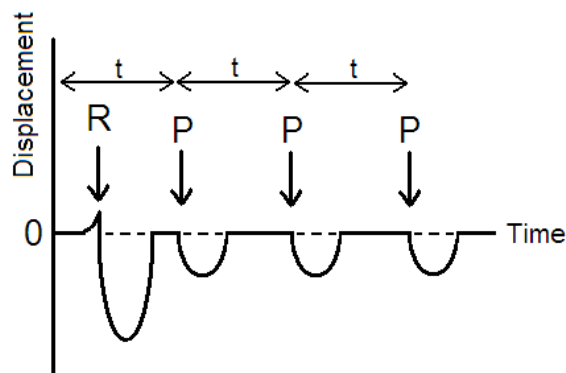
Figure 2.4 Illustration of an ideal waveform with the arrival of the R-wave and the multiple reflections of the P-wave
