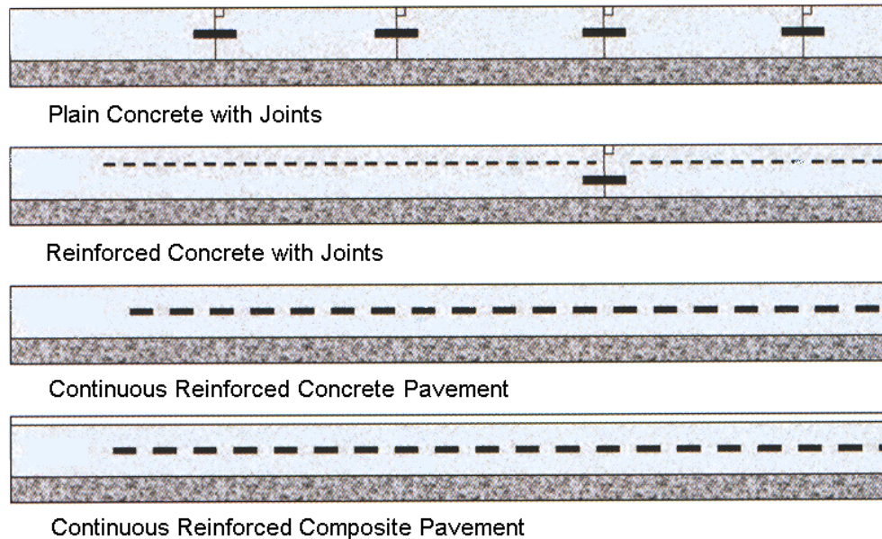
Figure 2.14 Several basic forms of concrete pavements and location of joints [17]
