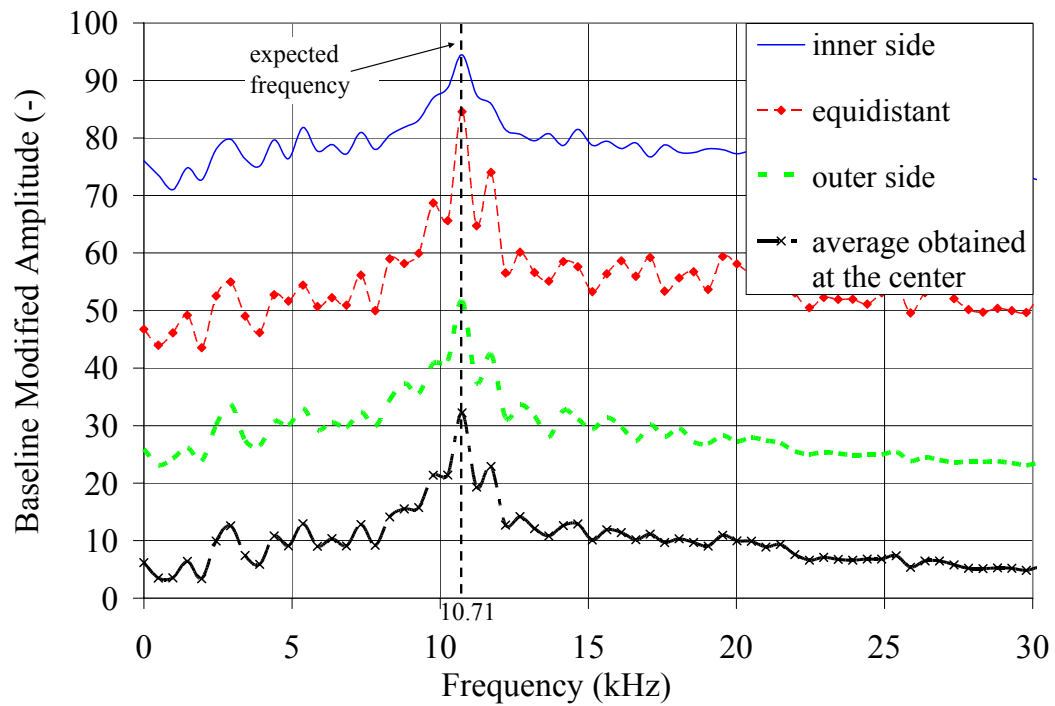
Figure 4.9 Results of data collected from the middle portion of the slab with 45 degree increments grouped into 3 categories
