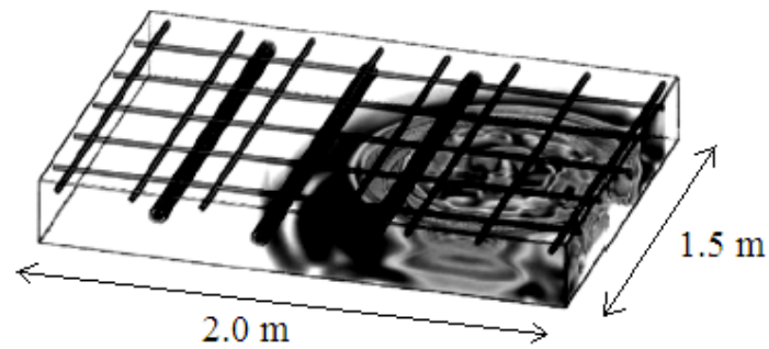
a-) 3-D view of the slab specimen used together with the reinforcing mesh and tendon ducts
