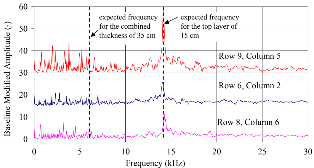
Figure 4.24 Sample resulting graphs while testing planar voids inside the concrete section
