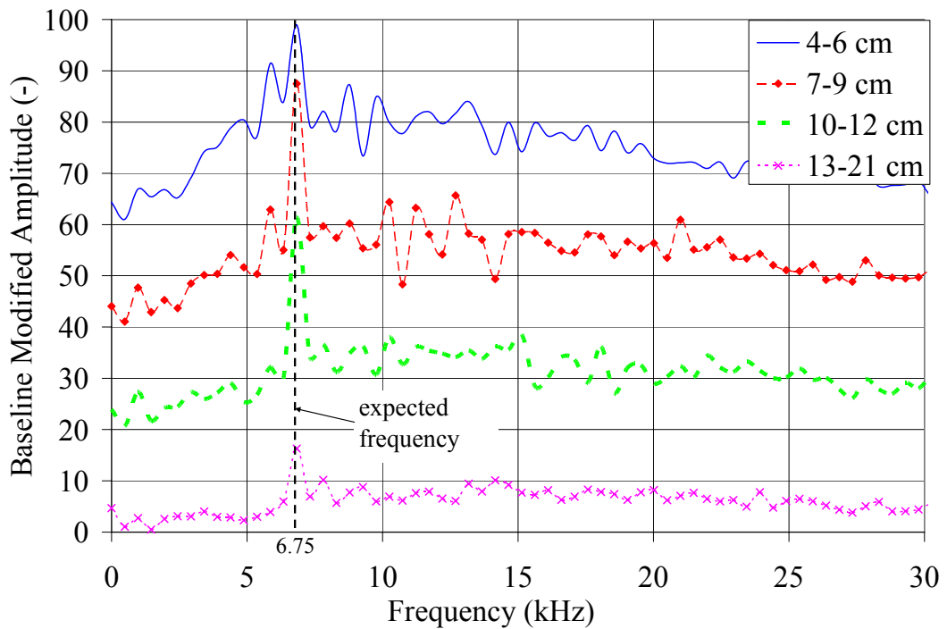
Figure 4.7 Illustration of the results of tests conducted to determine the effects of distance between the transducer and impact point on test results.
