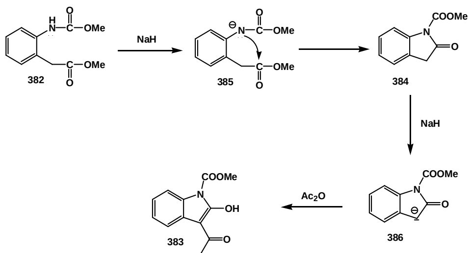
Scheme 15. Suggested mechanism for the formation of 383 .
