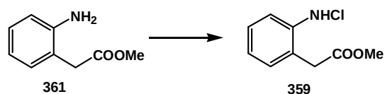
Scheme 10. Formation of the compound 359 .
