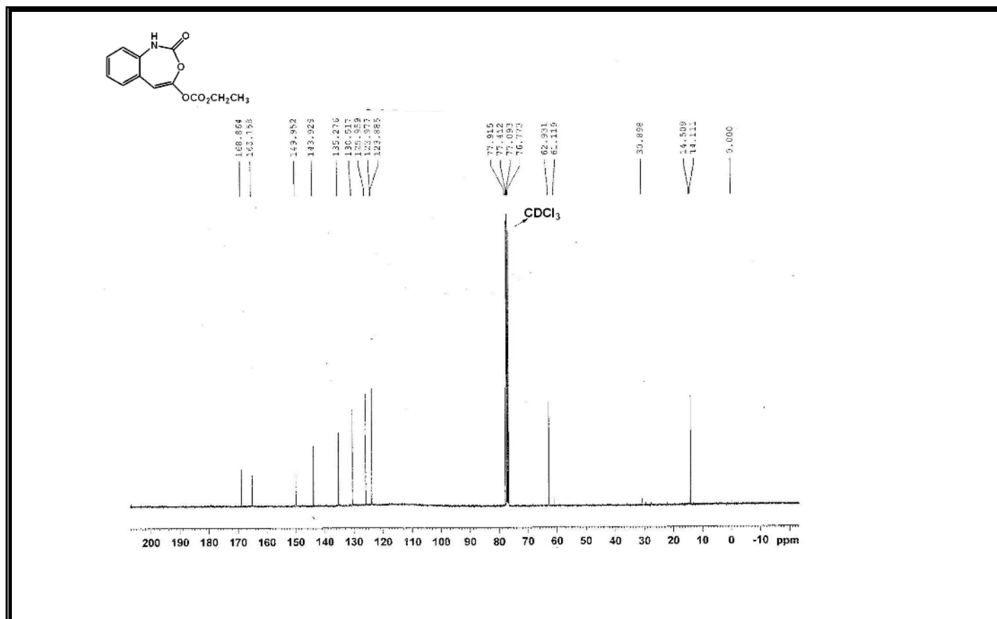
Figure A60 13 C-NMR Spectrum of Compound 335.
