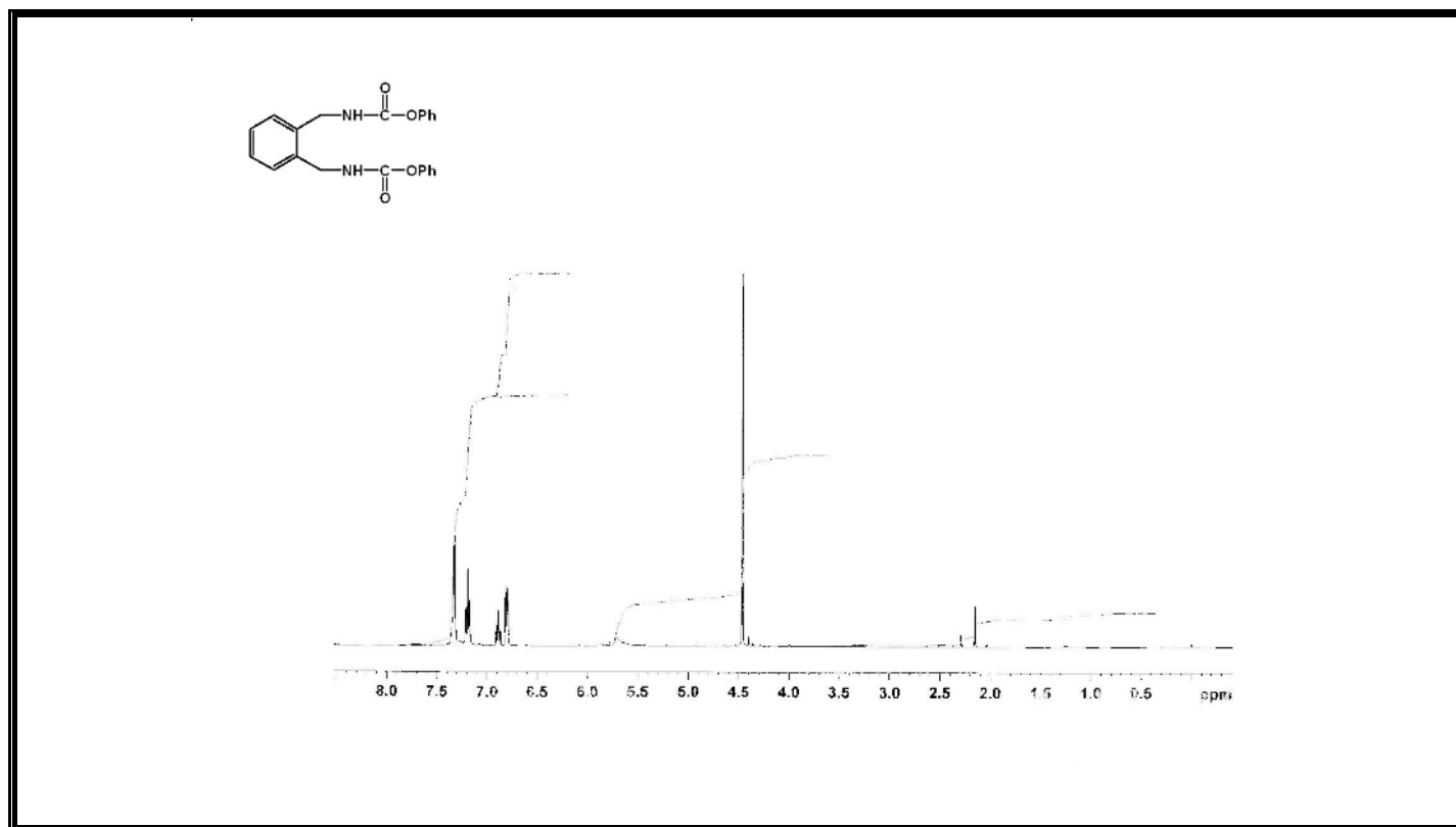
Figure A221 ^1\text{H} -NMR Spectrum of Compound 420.
