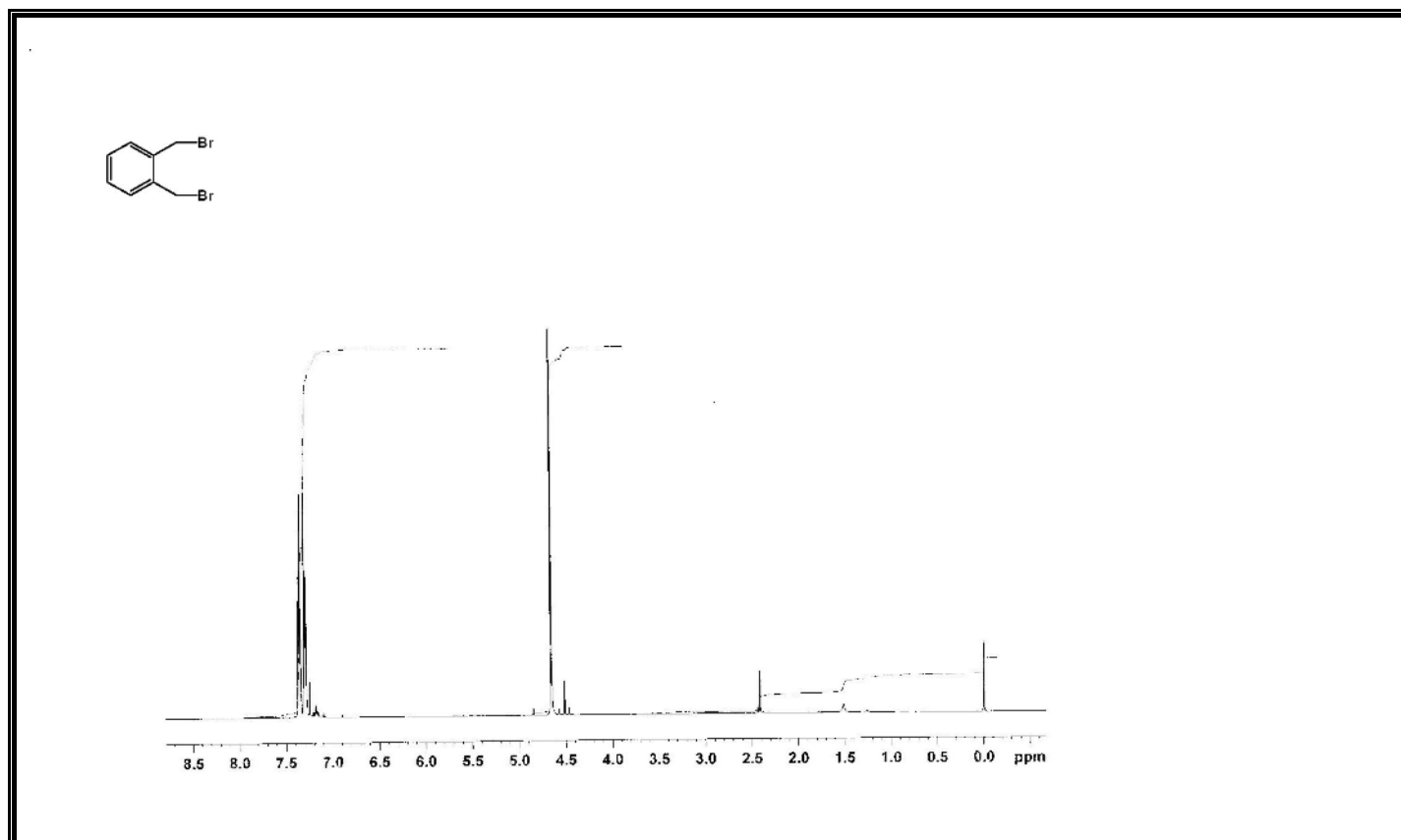
Figure A210 ^1\text{H} -NMR Spectrum of Compound 413.
