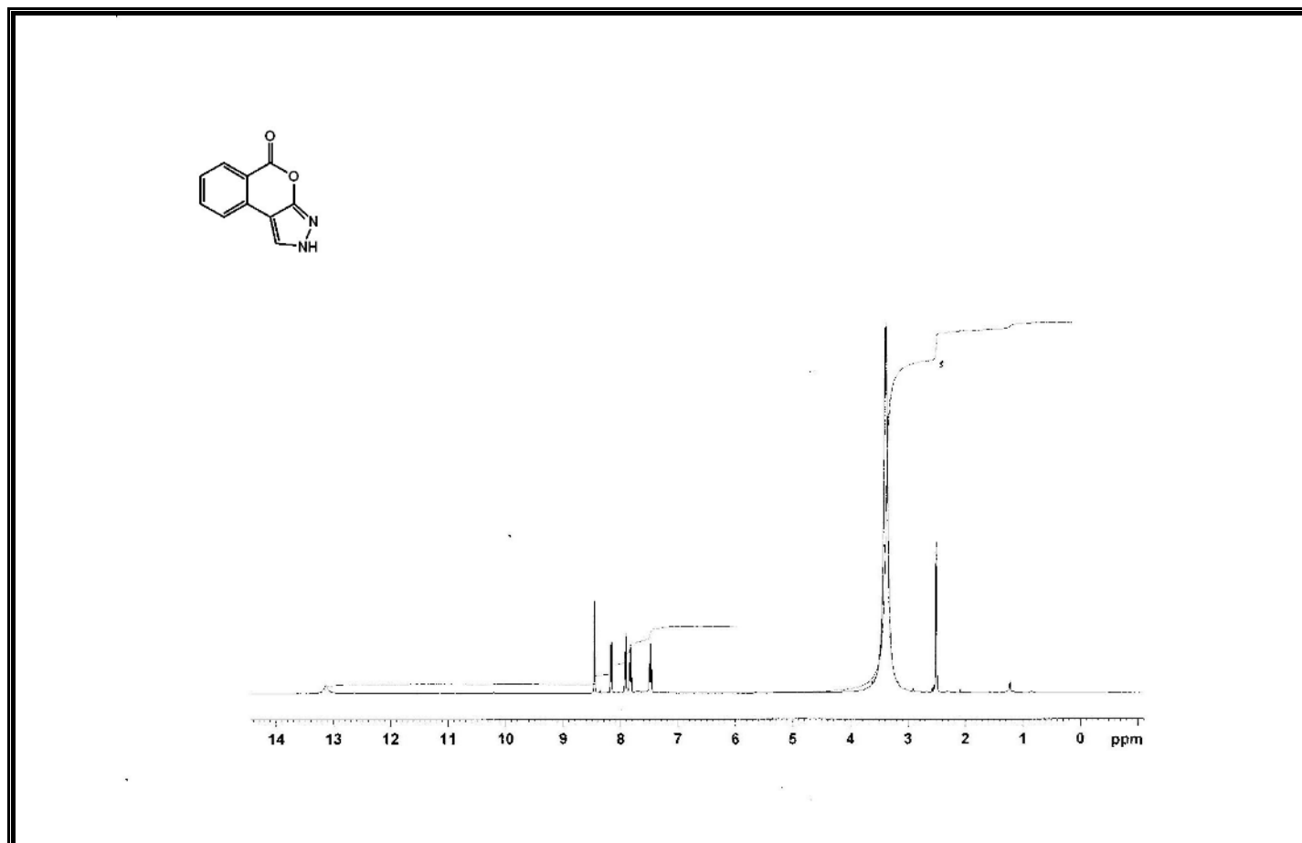
Figure A202 ^1\text{H} -NMR Spectrum of Compound 407.
