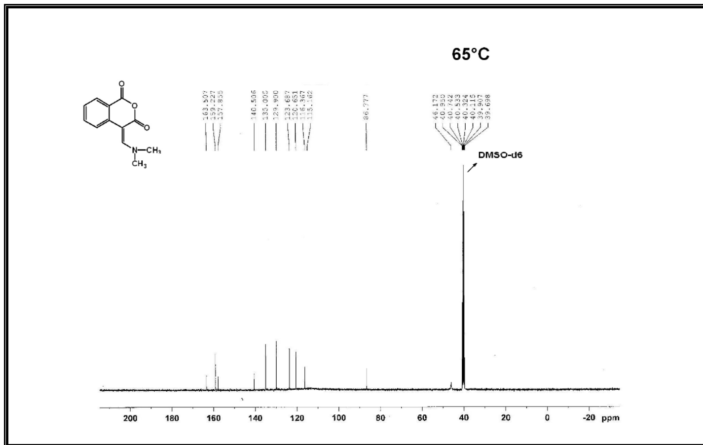
Figure A11 ^{13}\text{C} -NMR Spectrum of Compound 327.
