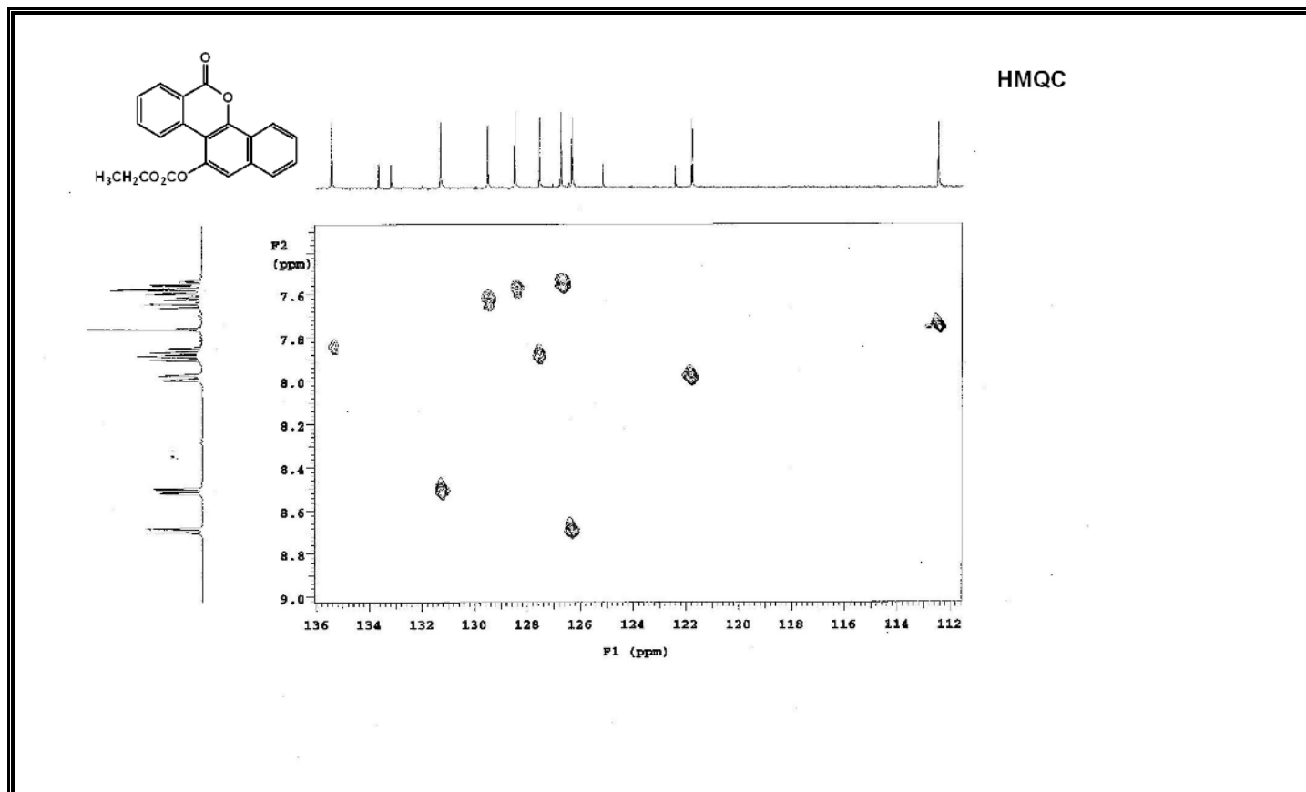
Figure A20 Expanded HMQC Spectrum of Compound 333.
