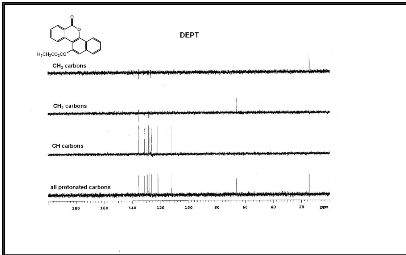
Figure A16 DEPT Spectrum of Compound 333.
