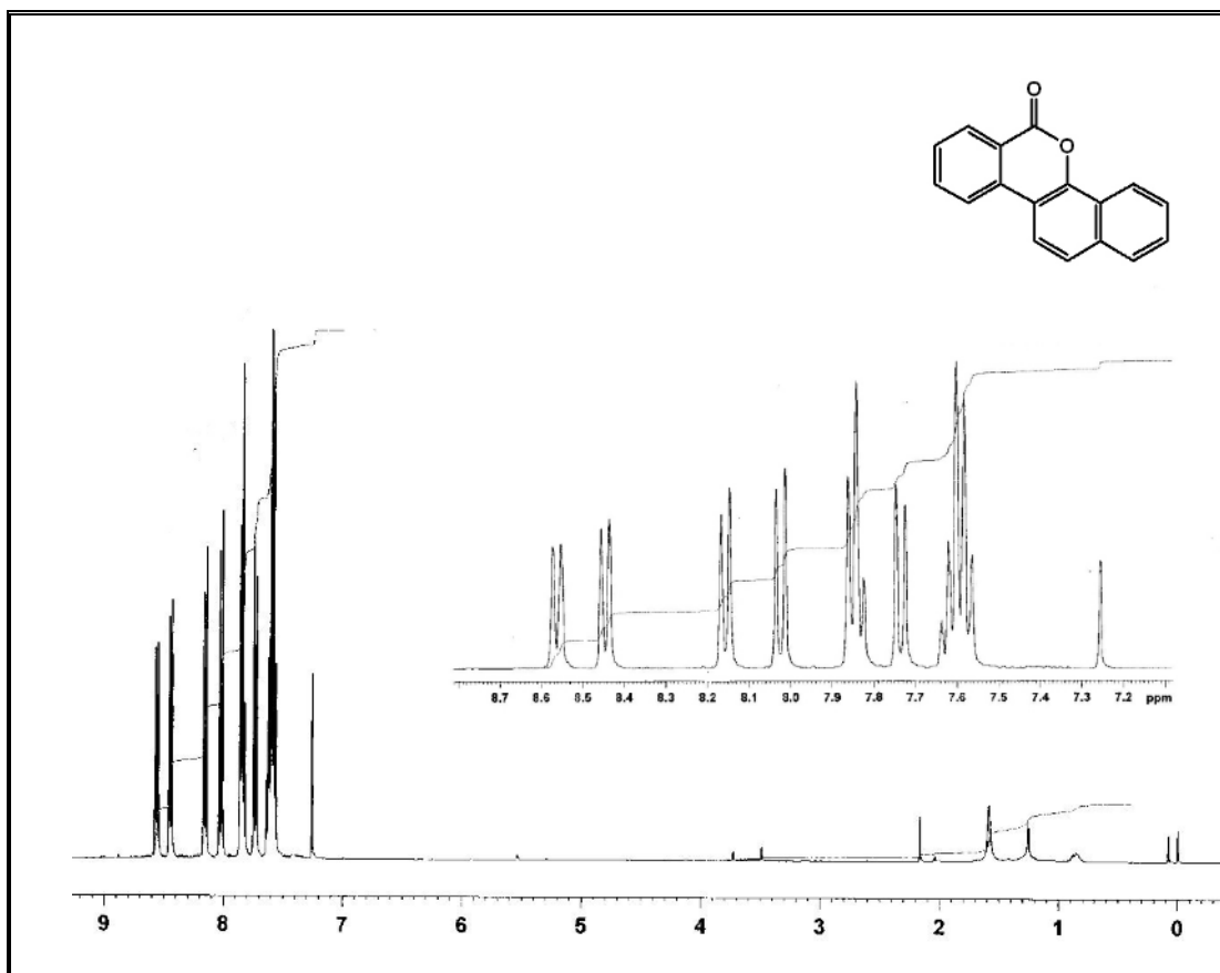
Figure 1. The ^1\text{H} -NMR spectrum of the compound 307 .
