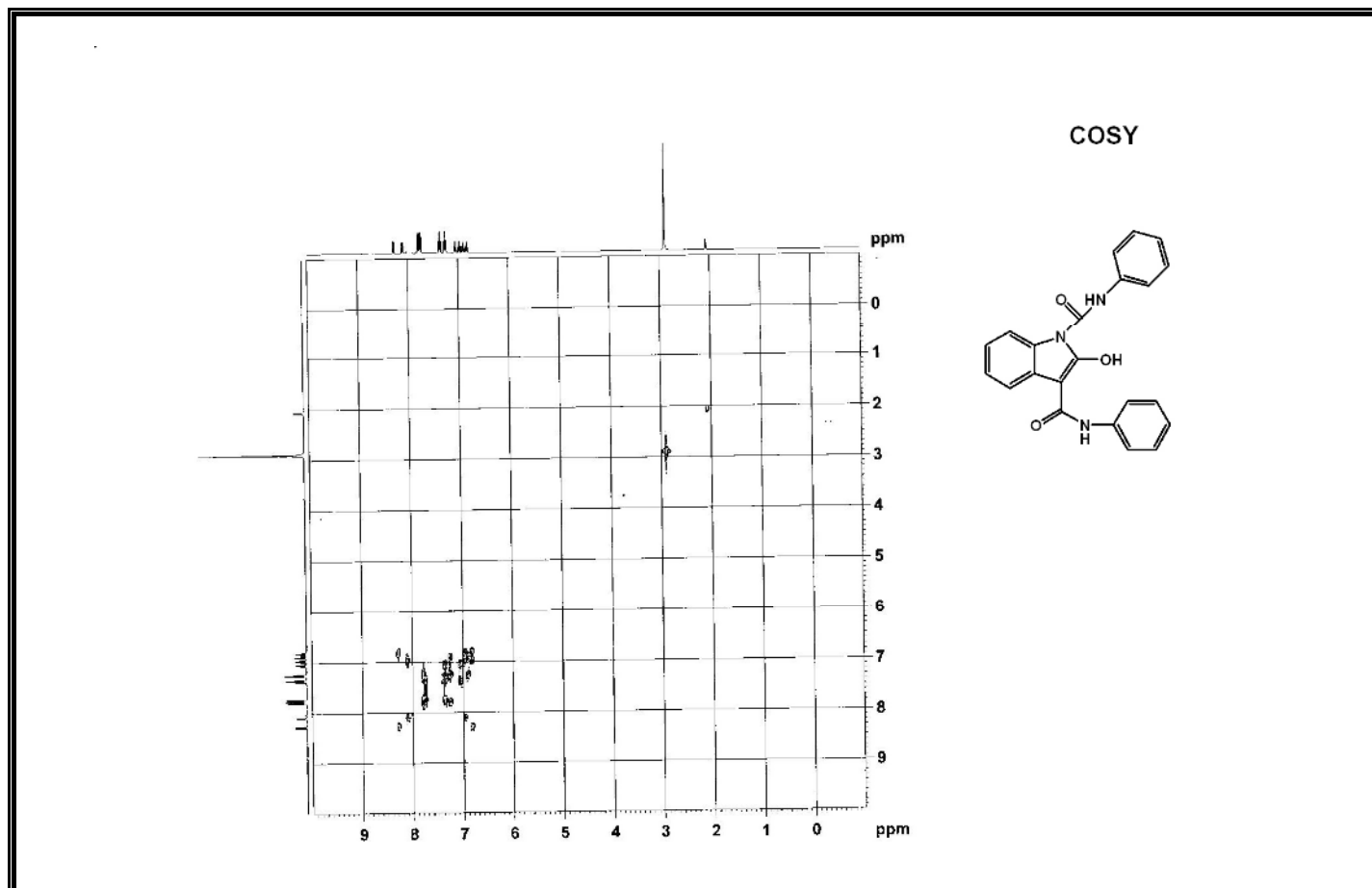
Figure A125 COSY Spectrum of Compound 379.
