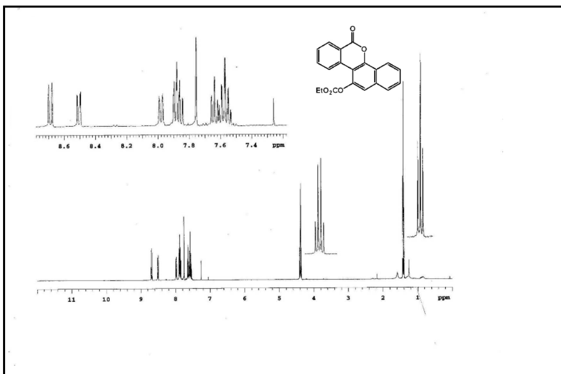
Figure 4. The ^1\text{H} -NMR spectrum of the compound 333 .
