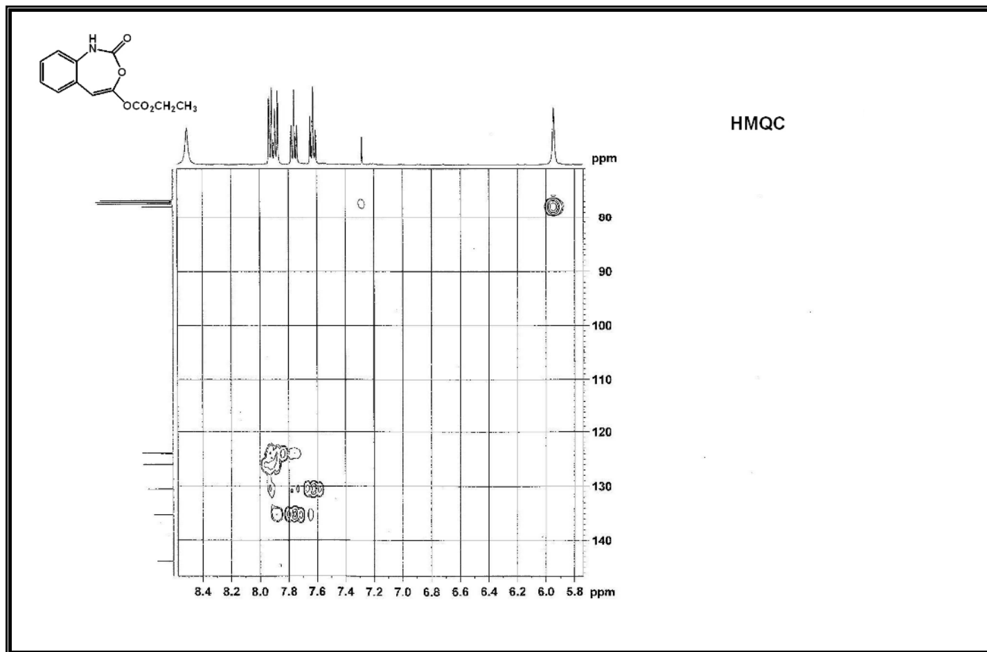
Figure A66 Expanded HMQC Spectrum of Compound 335.
