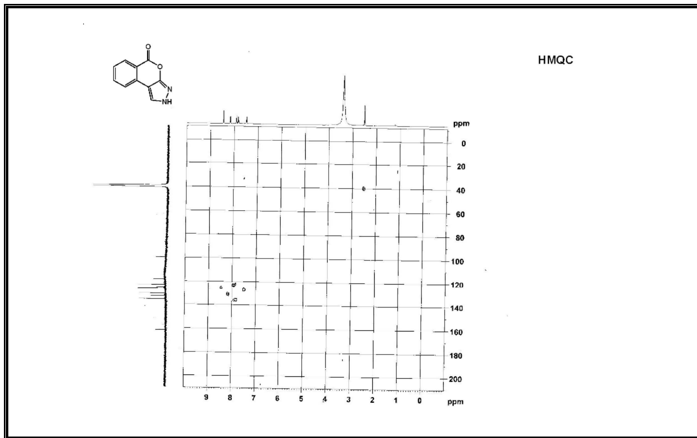
Figure A206 HMQC Spectrum of Compound 407.
