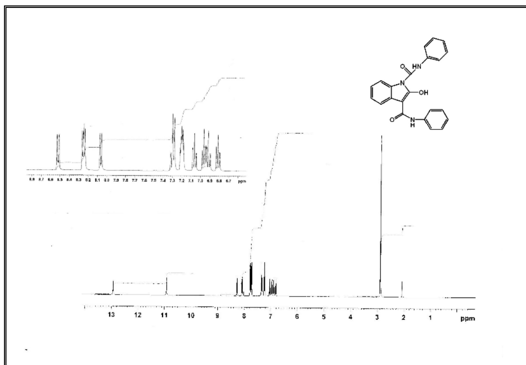
Figure 15. ^1\text{H} -NMR spectrum of the compound 379.
