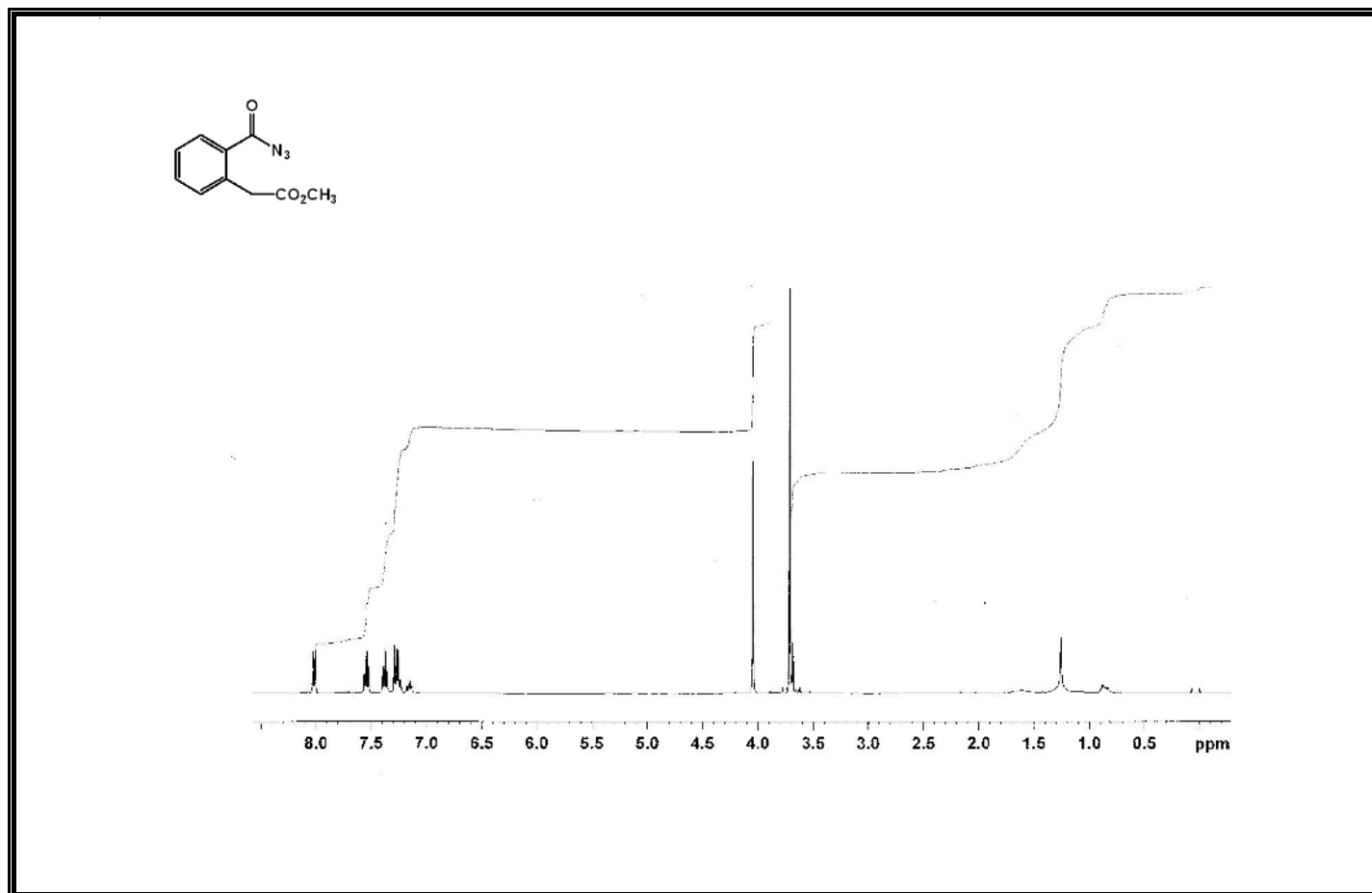
Figure A104 ^1\text{H} -NMR Spectrum of Compound 353.
