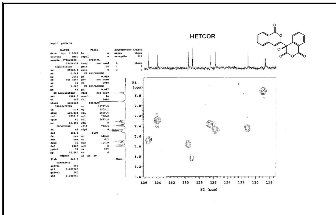
Figure A32 Expanded HETCOR Spectrum of Compound 332.
