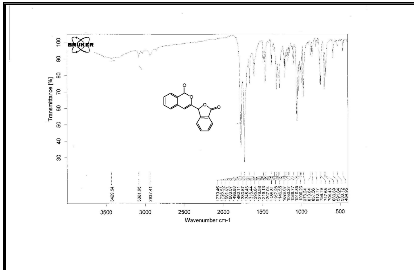
Figure A56 IR Spectrum of Compound 334.
