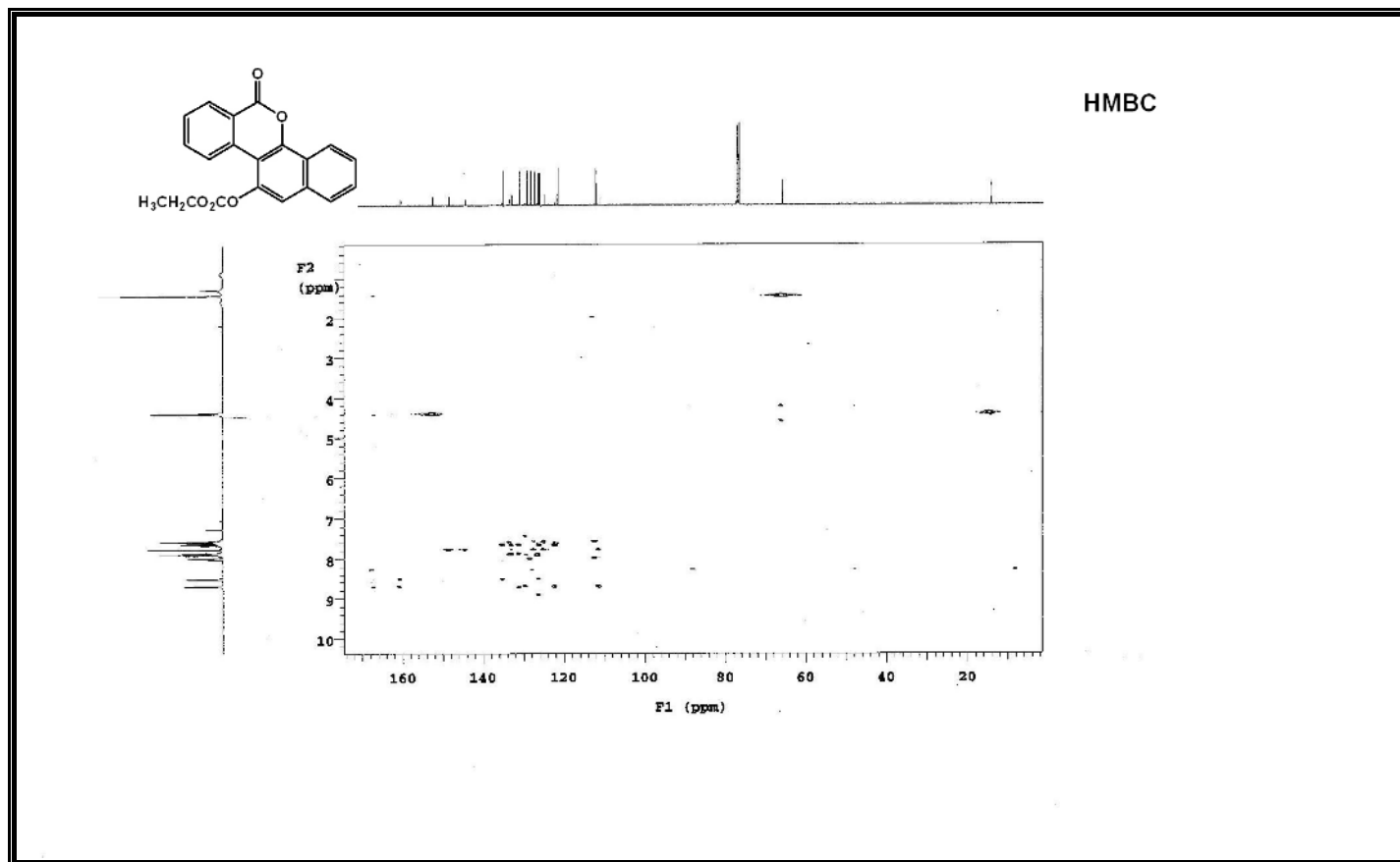
Figure A21 HMBC Spectrum of Compounds 333.
