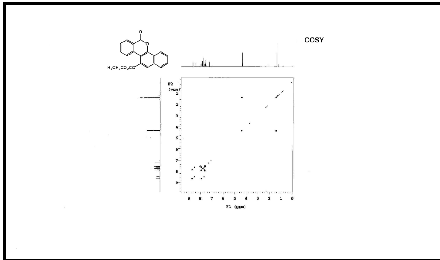
Figure A17 COSY Spectrum of Compound 333.
