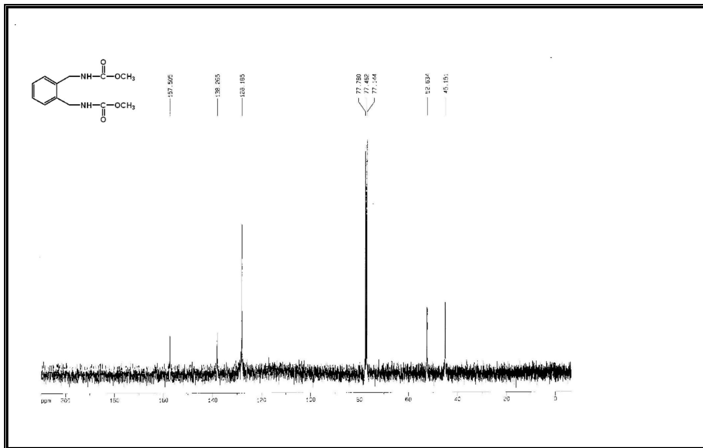
Figure A216 ^{13}\text{C} -NMR Spectrum of Compound 418.
