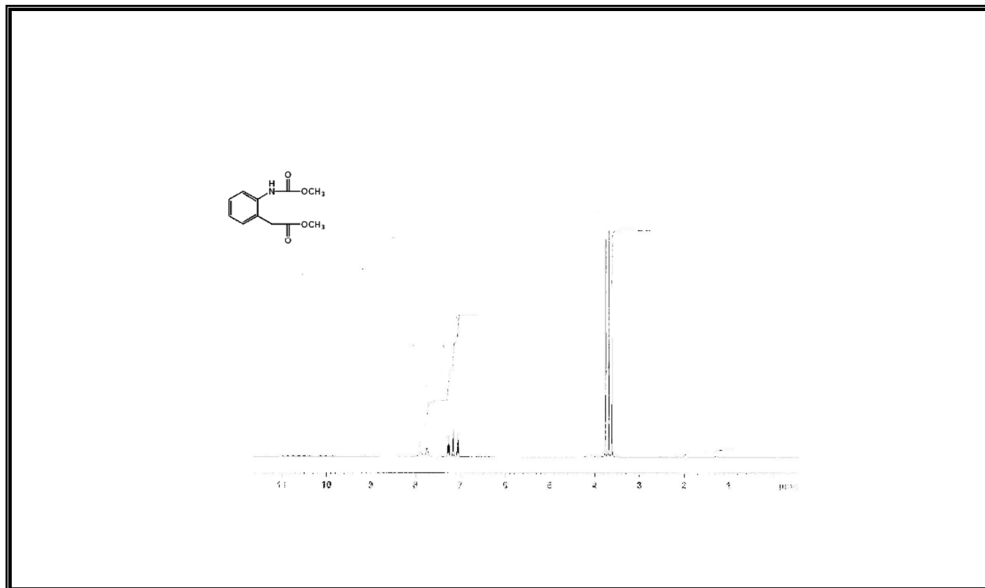
Figure A136 ^1\text{H} -NMR Spectrum of Compound 382.
