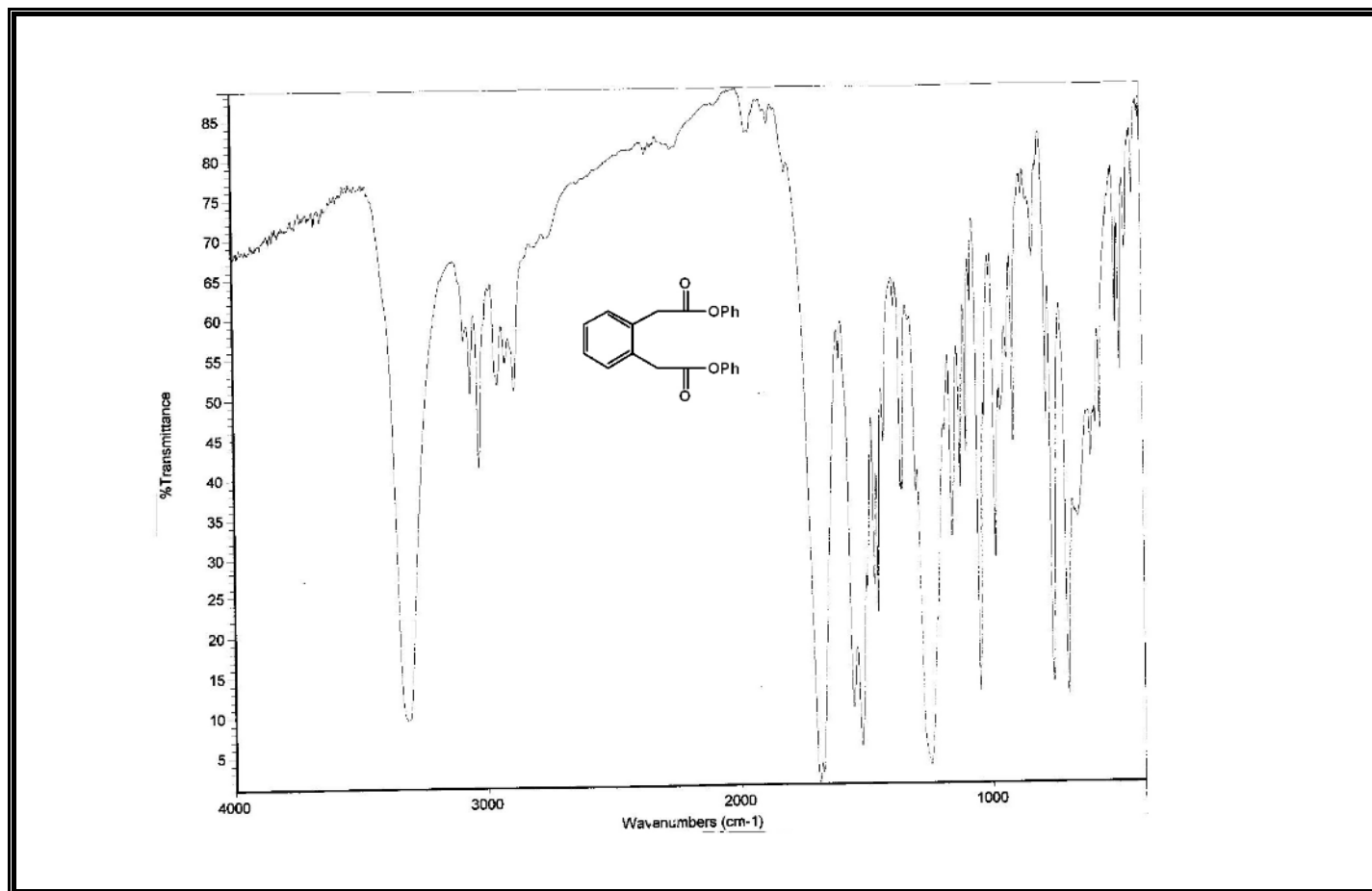
Figure A223 IR Spectrum of Compound 420.
