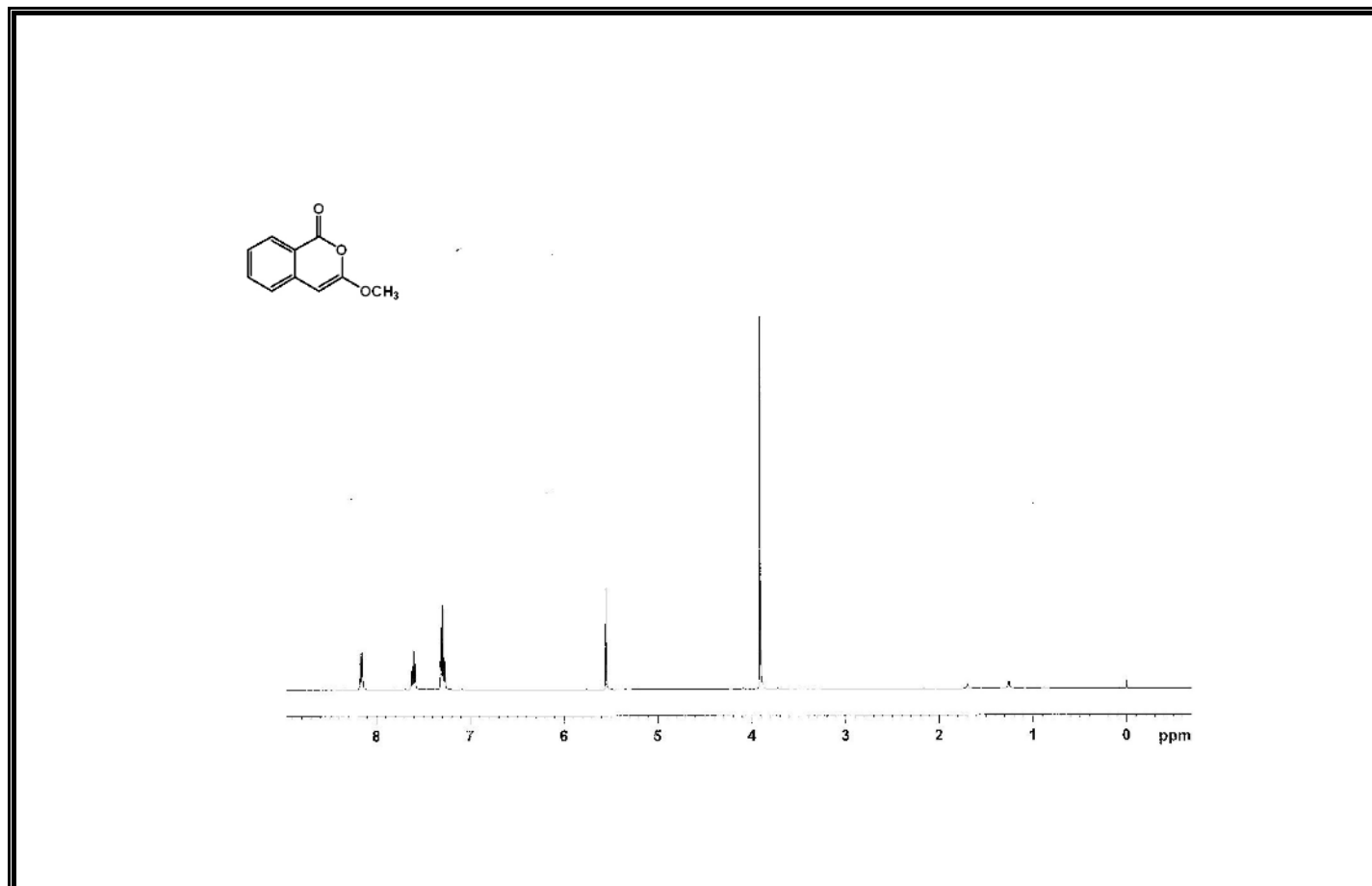
Figure A88 ^1\text{H} -NMR Spectrum of Compound 360.
