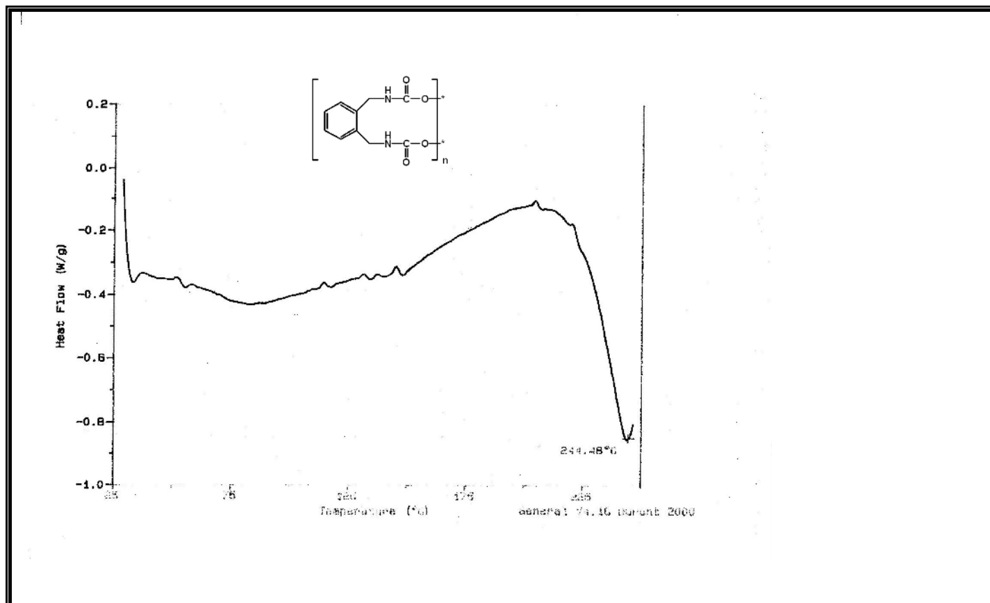
Figure A228 DSC Spectrum of Compound 427.
