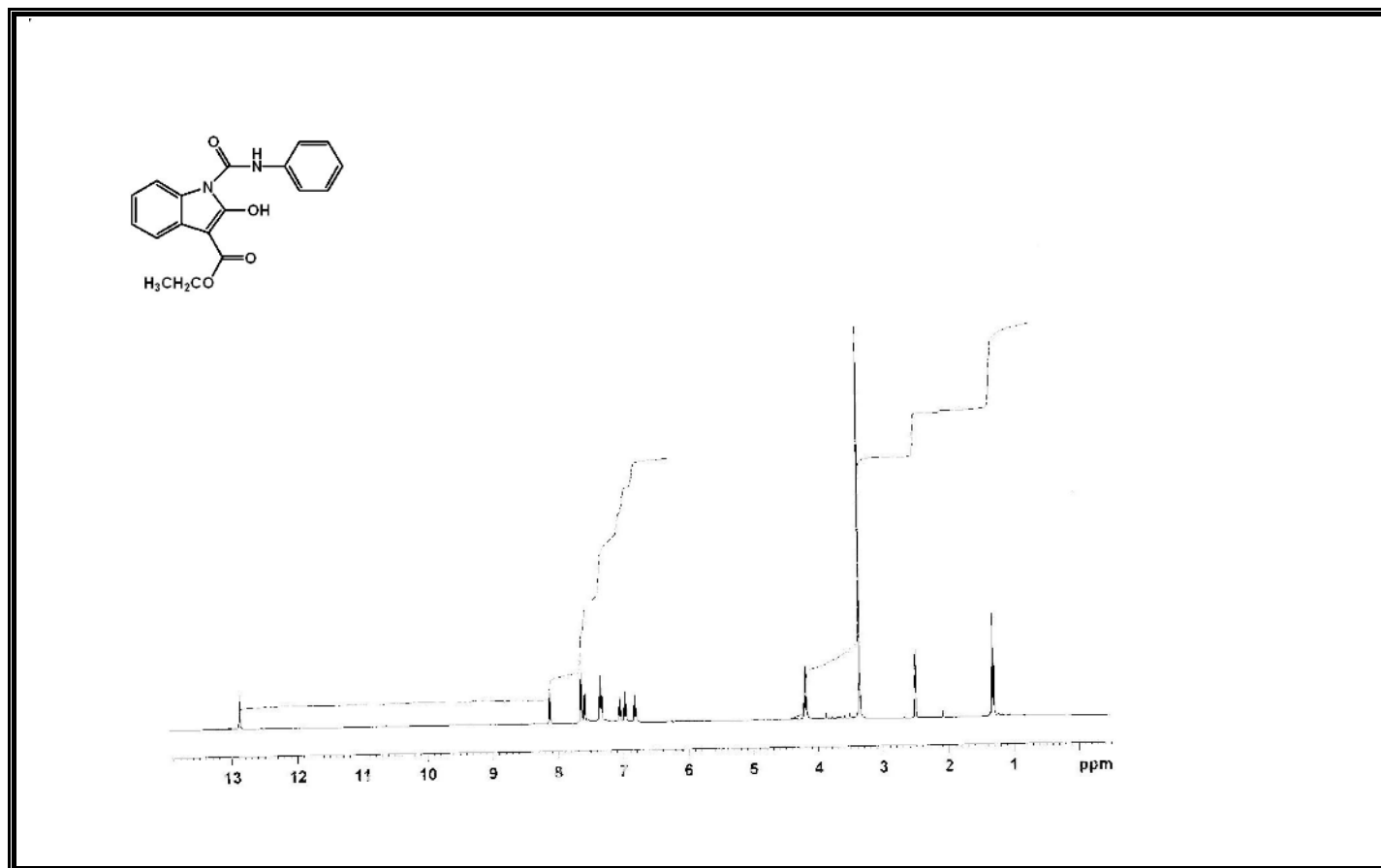
Figure A184 1 H-NMR Spectrum of Compound 396 .
