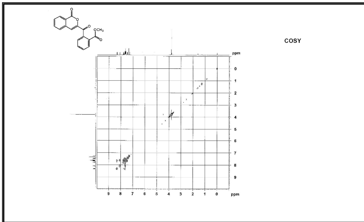
Figure A40 COSY Spectrum of Compound 340.
