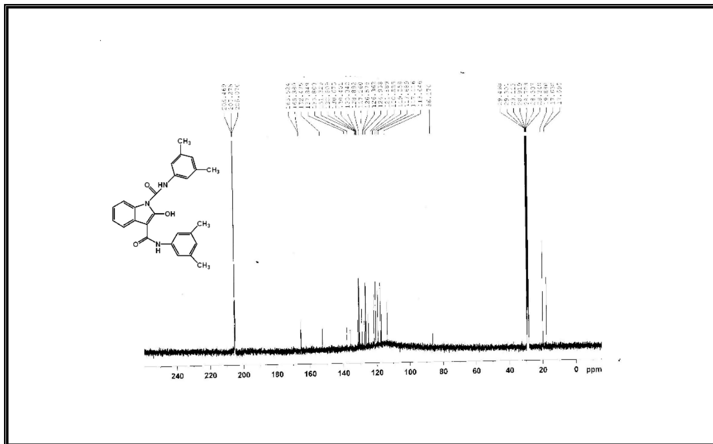
Figure A131 ^{13}\text{C} -NMR Spectrum of Compound 380.
