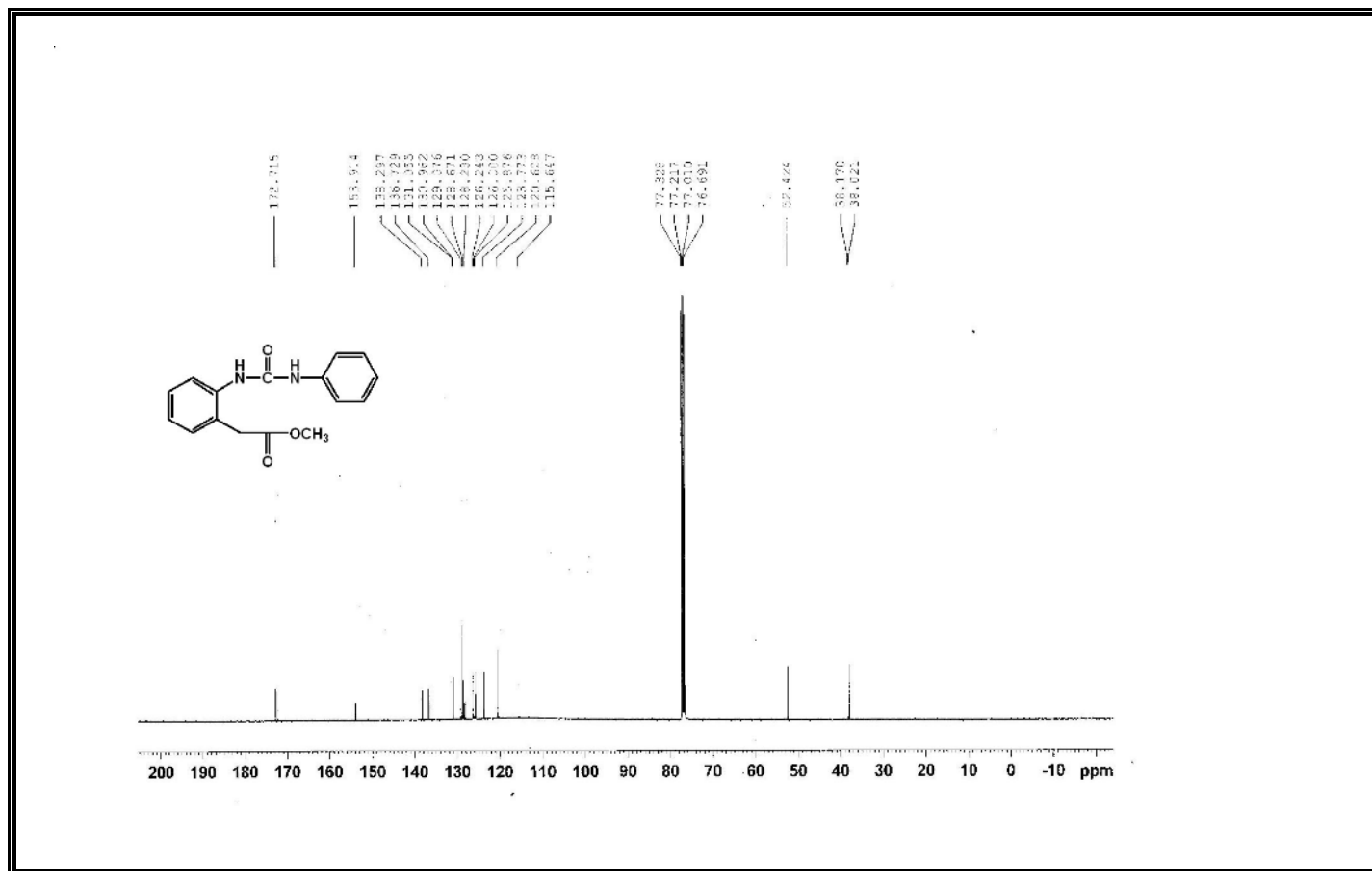
Figure A111 ^{13}\text{C} -NMR Spectrum of Compound 374.
