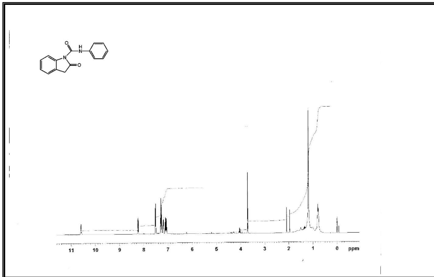
Figure A181 ^1\text{H} -NMR Spectrum of Compound 395.
