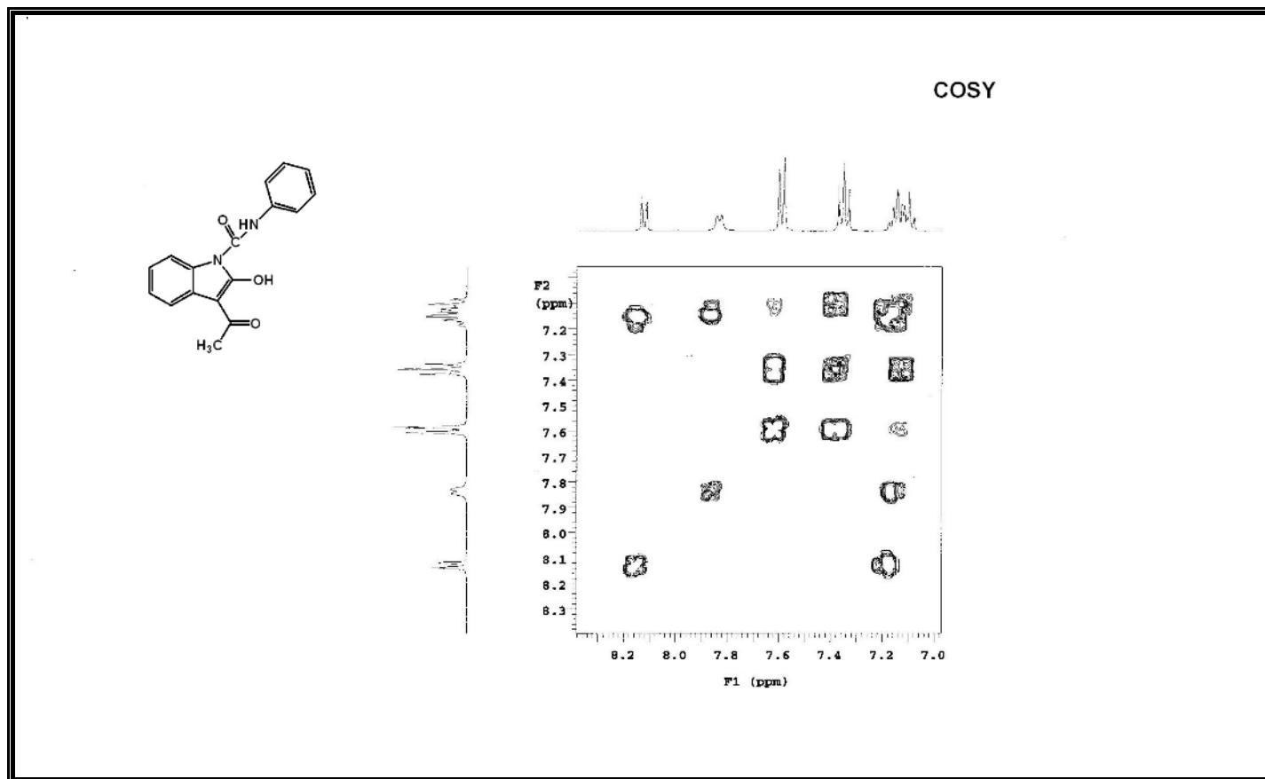
Figure A177 Expanded COSY Spectrum of Compound 394.
