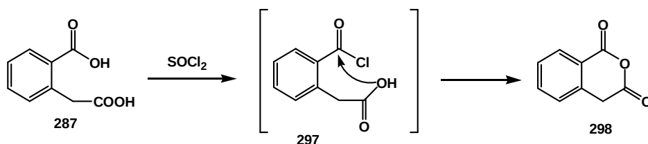
Scheme 1. Suggested mechanism for the formation of the compound 298 .
