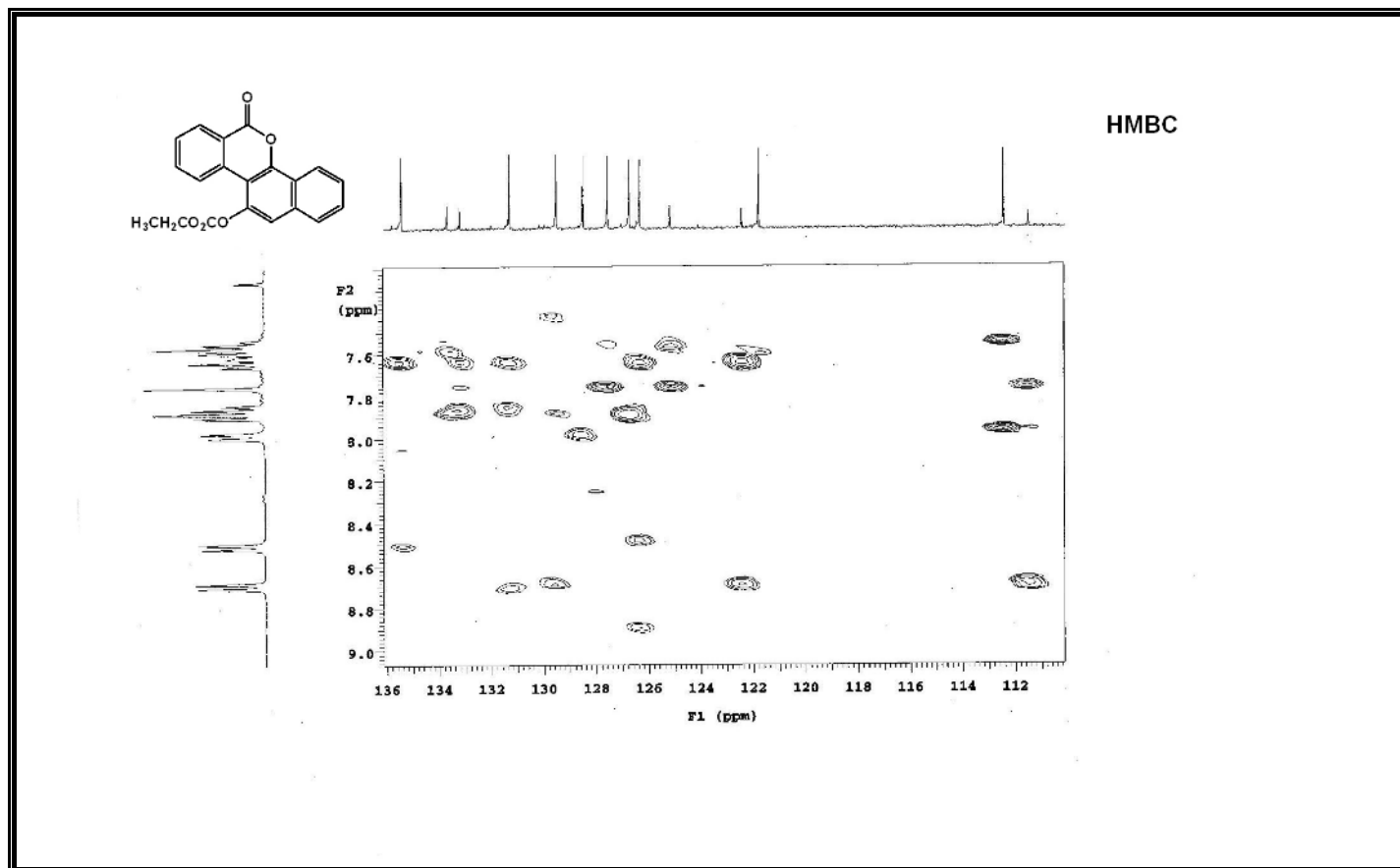
Figure A22 Expanded HMBC Spectrum of Compound 333.
