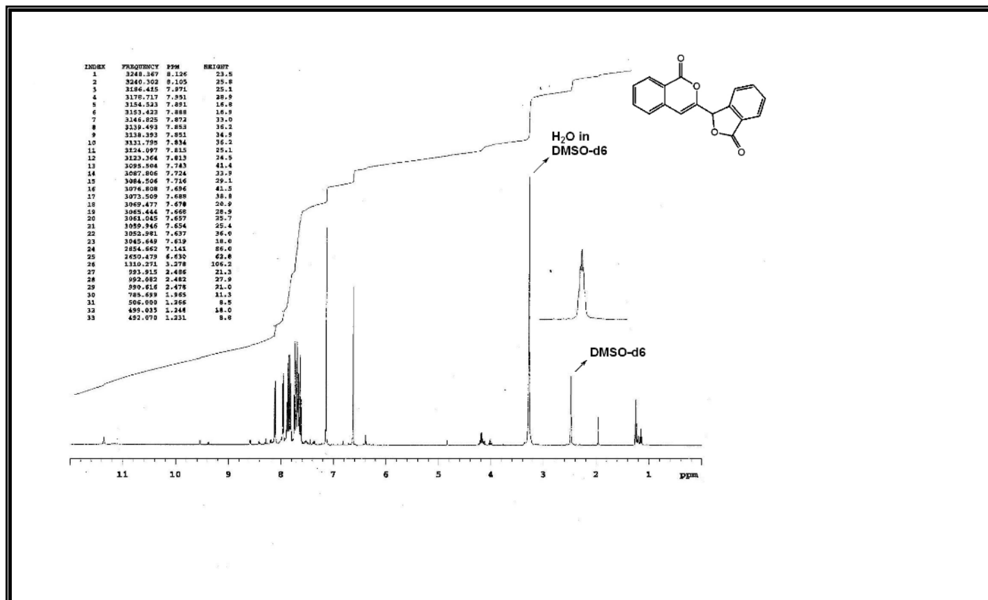
Figure A47 1 H-NMR Spectrum of Compound 334.
