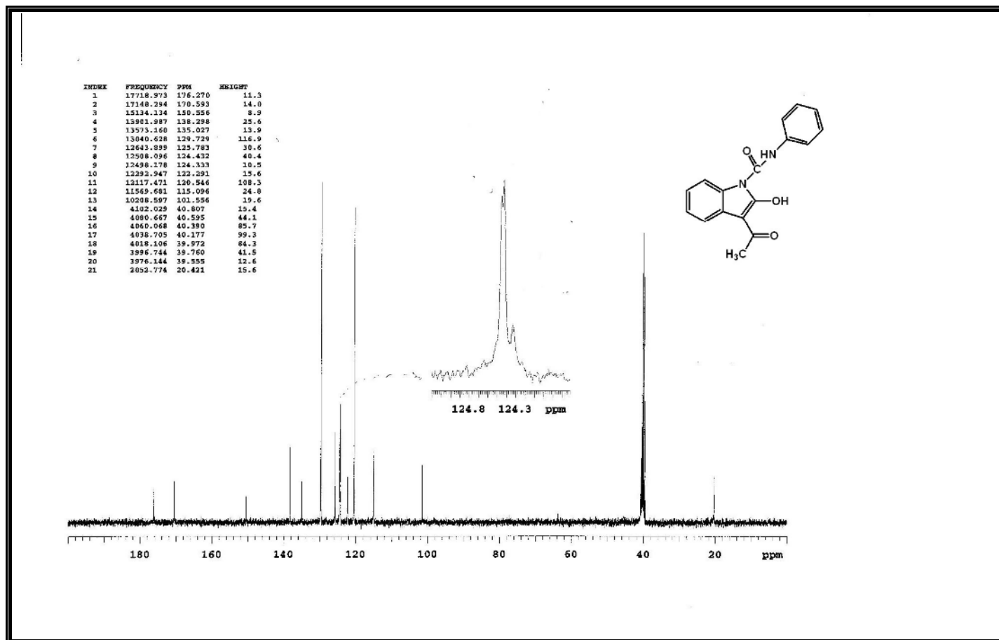
Figure A172 13 C-NMR Spectrum of Compound 394.
