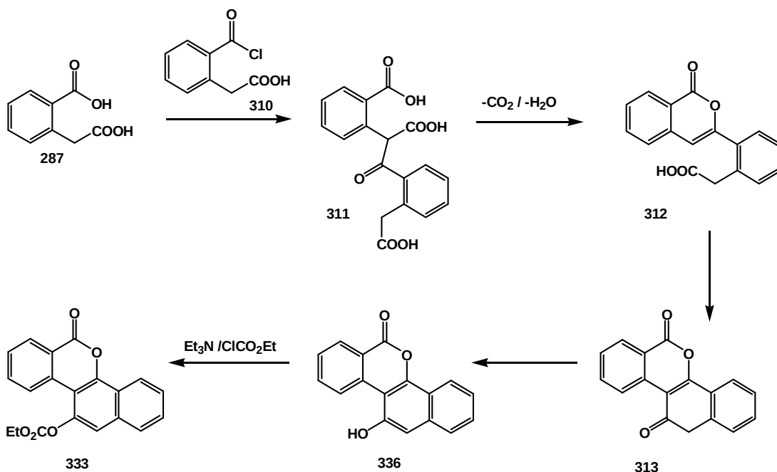
Scheme 4. Suggested mechanism for the formation of the compound 333 .
