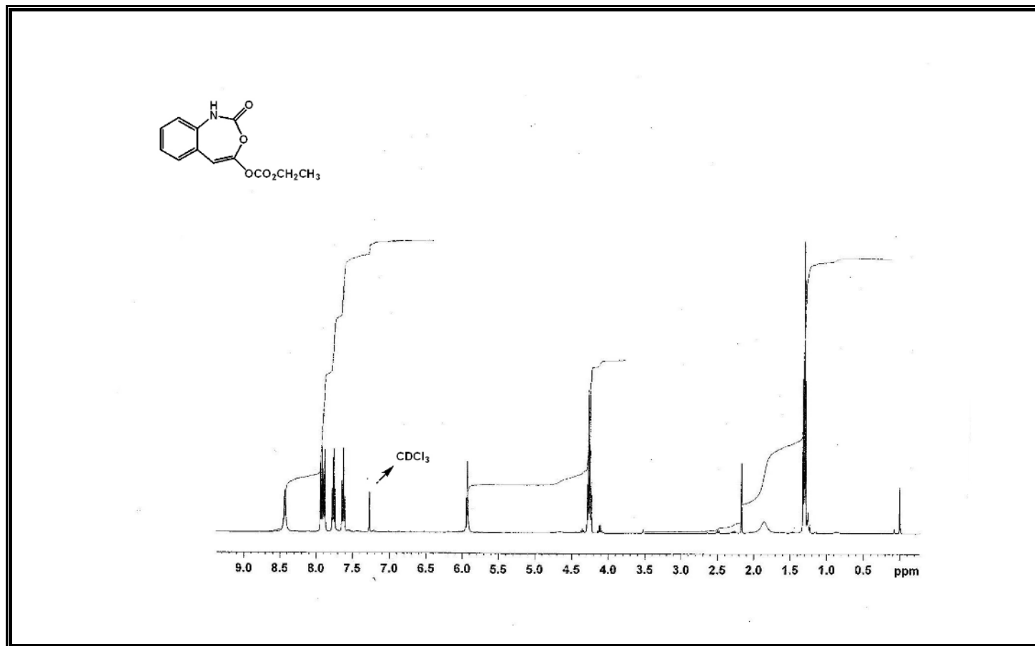
Figure A59 ^1\text{H} -NMR Spectrum of Compound 335.
