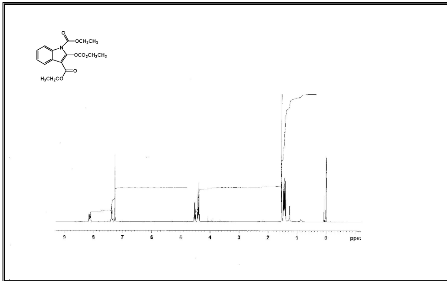
Figure A165 ^1\text{H} -NMR Spectrum of Compound 392.
