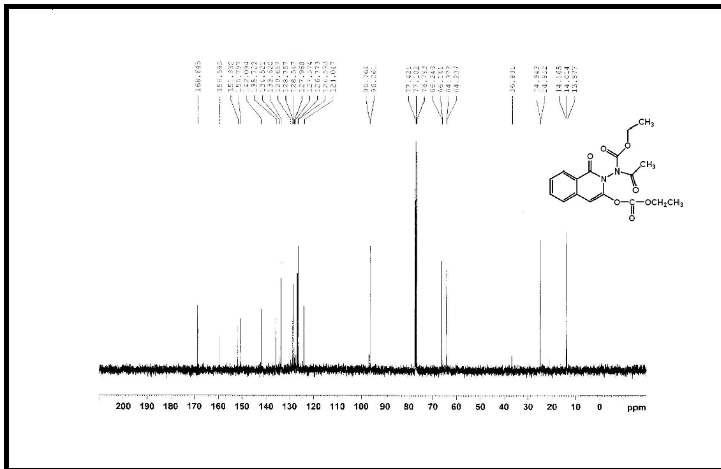
Figure A200 ^{13}\text{C} -NMR Spectrum of Compound 406.
