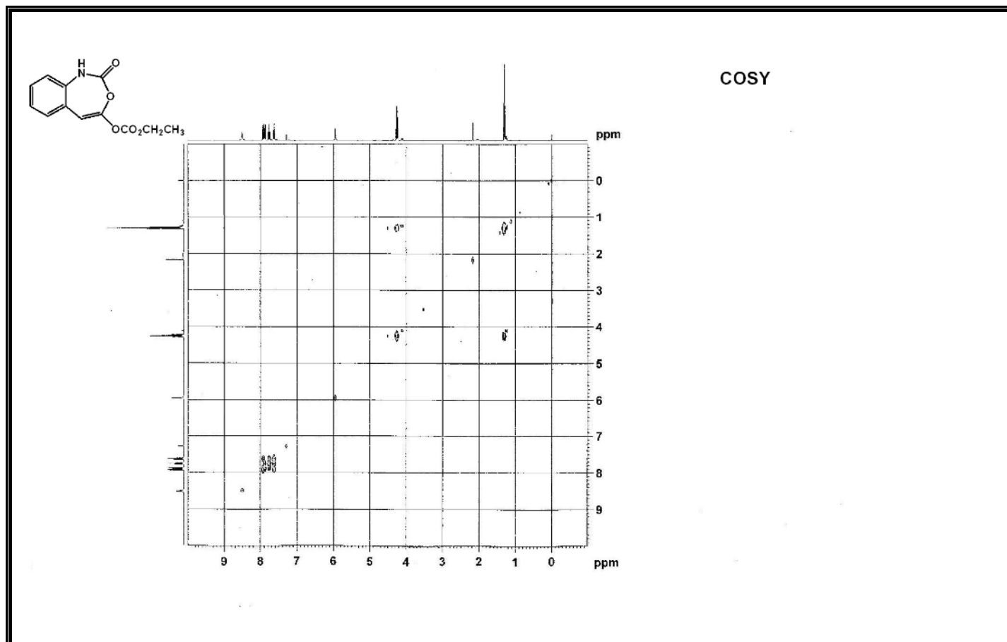
Figure A63 COSY Srectrum of Compound 335.
