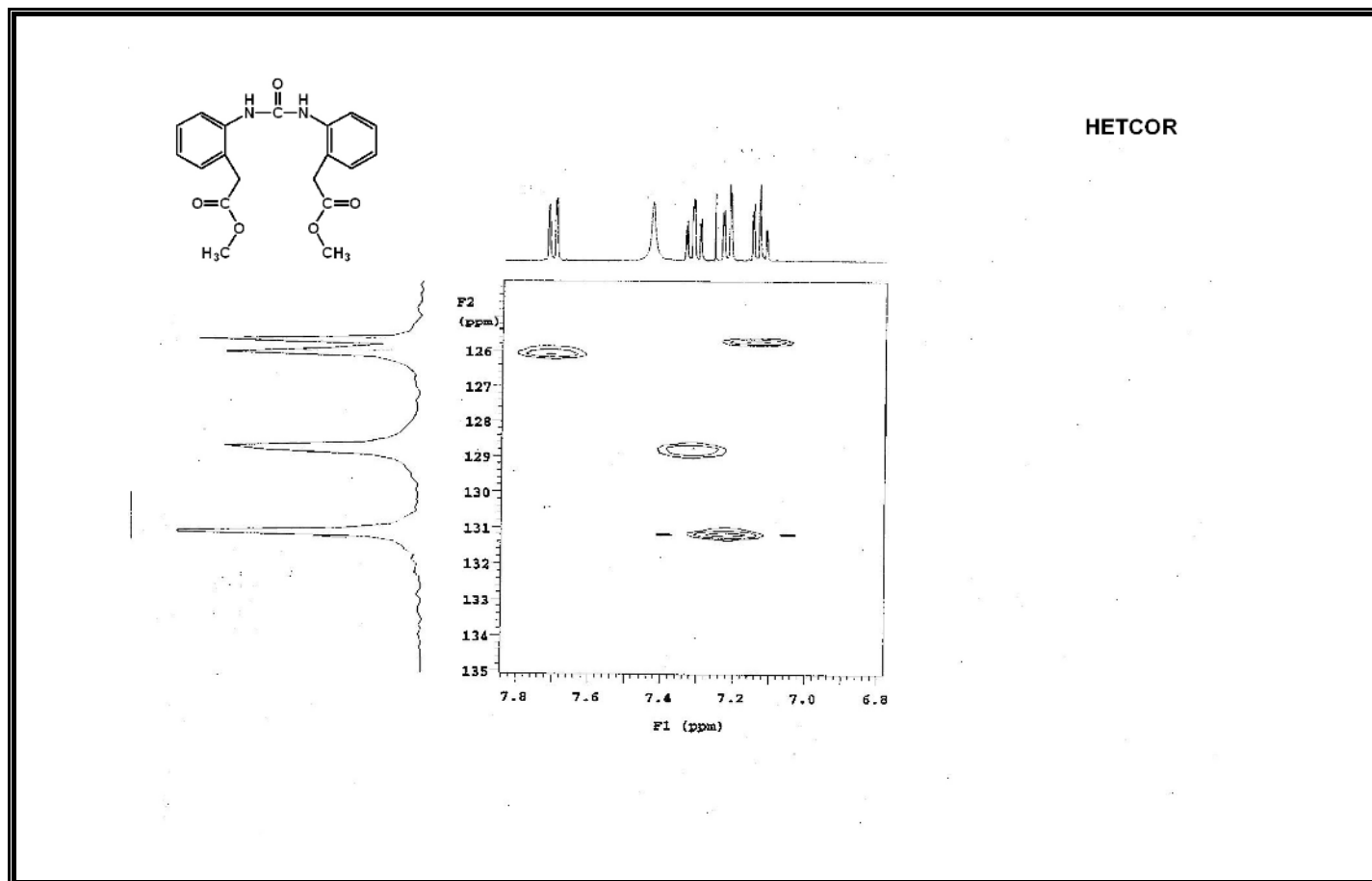
Figure A83 HETCOR Spectrum of Compound 358.
