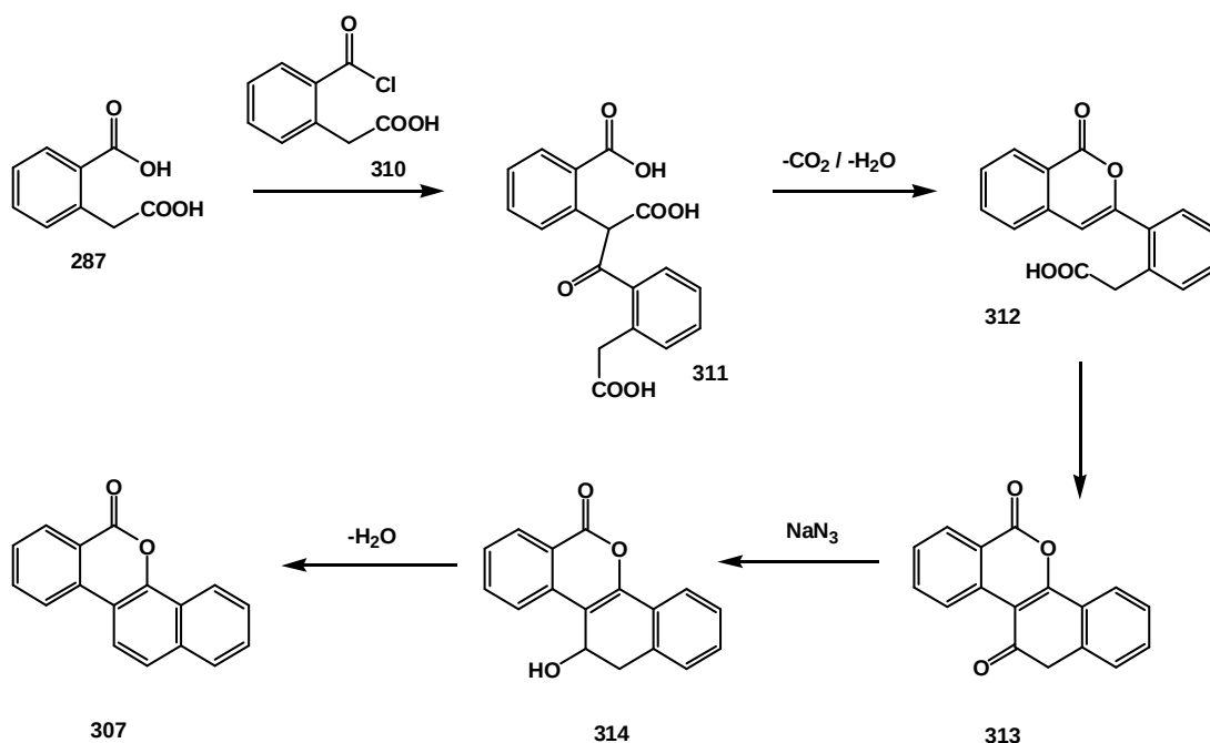
Scheme 2. Suggested mechanism for the formation of the compound 307 .
