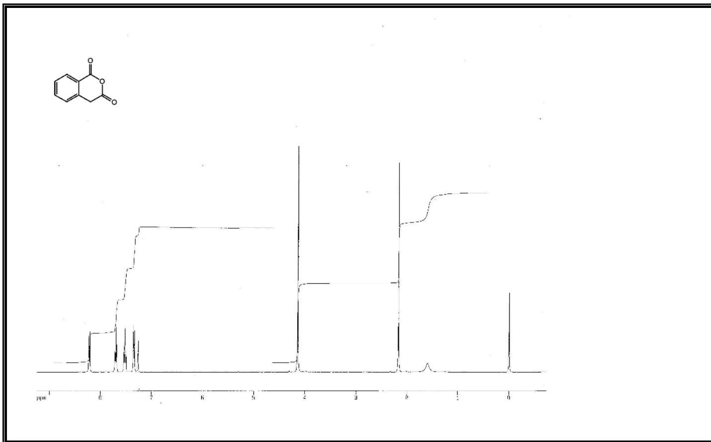
Figure A1 ^1\text{H} -NMR Spectrum of Compound 298.
