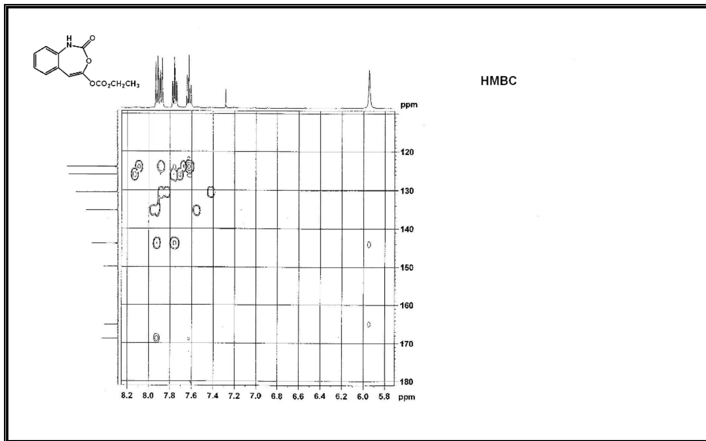
Figure A68 Expanded HMBC Spectrum of Compound 335.
