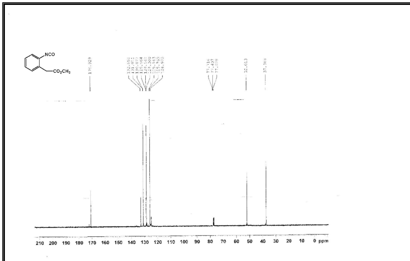
Figure A108 ^{13}\text{C} -NMR Spectrum of Compound 354.
