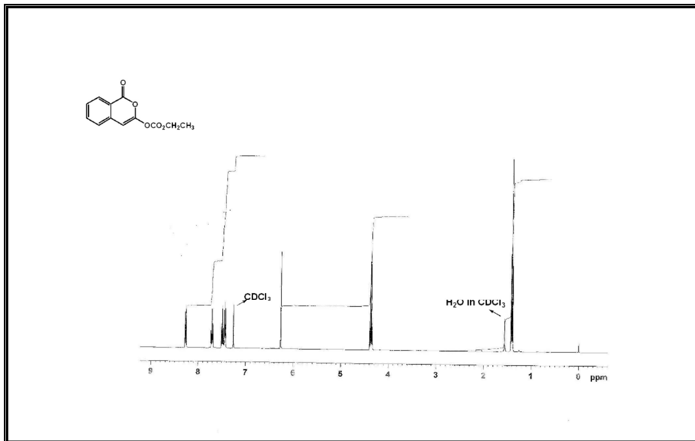
Figure A77 1 H-NMR Spectrum of Compound 352.
