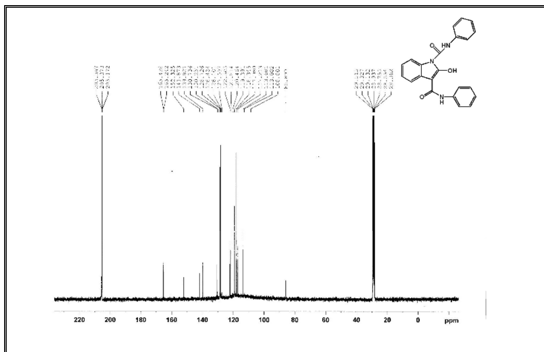
Figure 16. ^{13}\text{C} -NMR spectrum of the compound 379.
