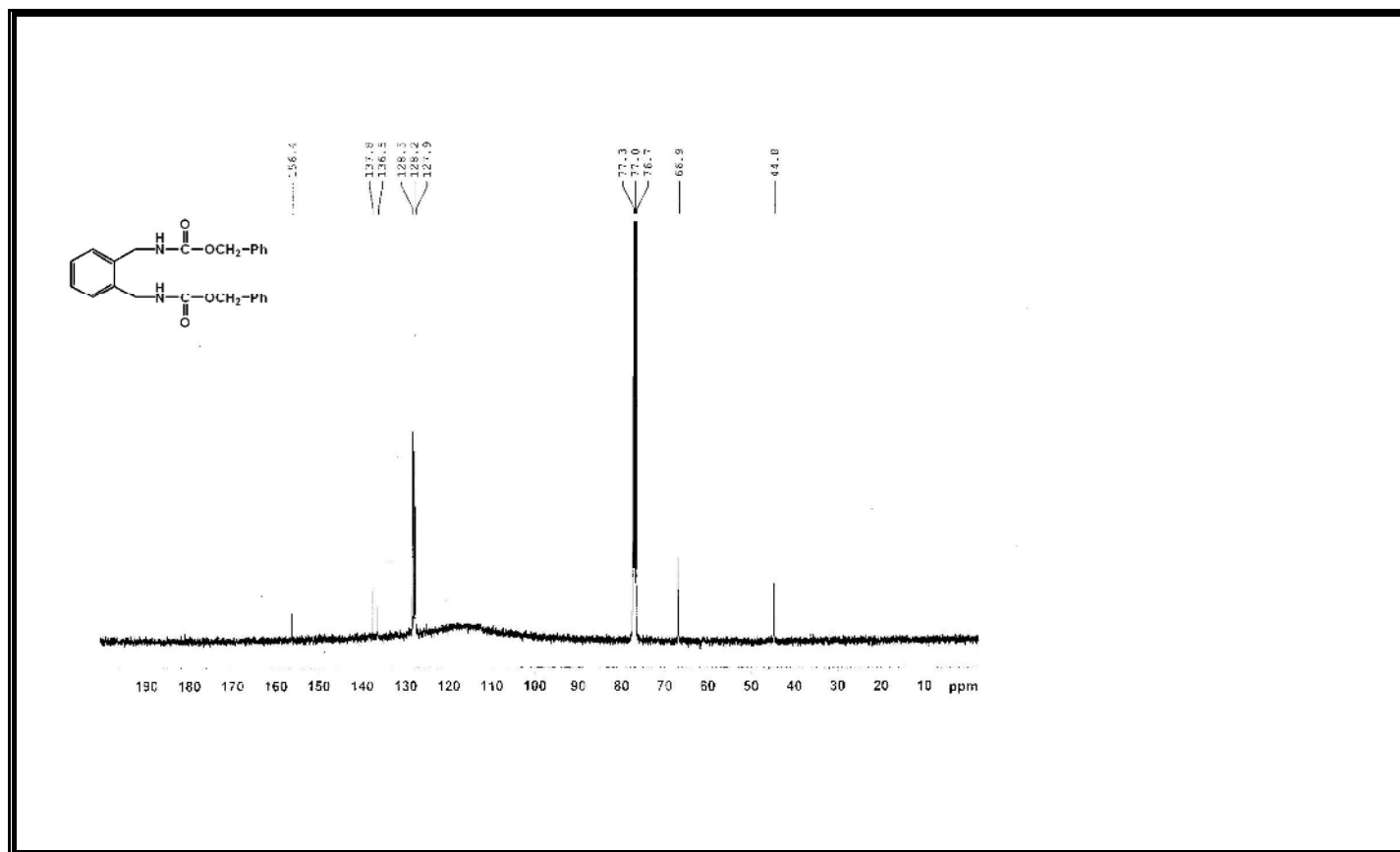
Figure A225 ^{13}\text{C} -NMR Spectrum of Compound 422.
