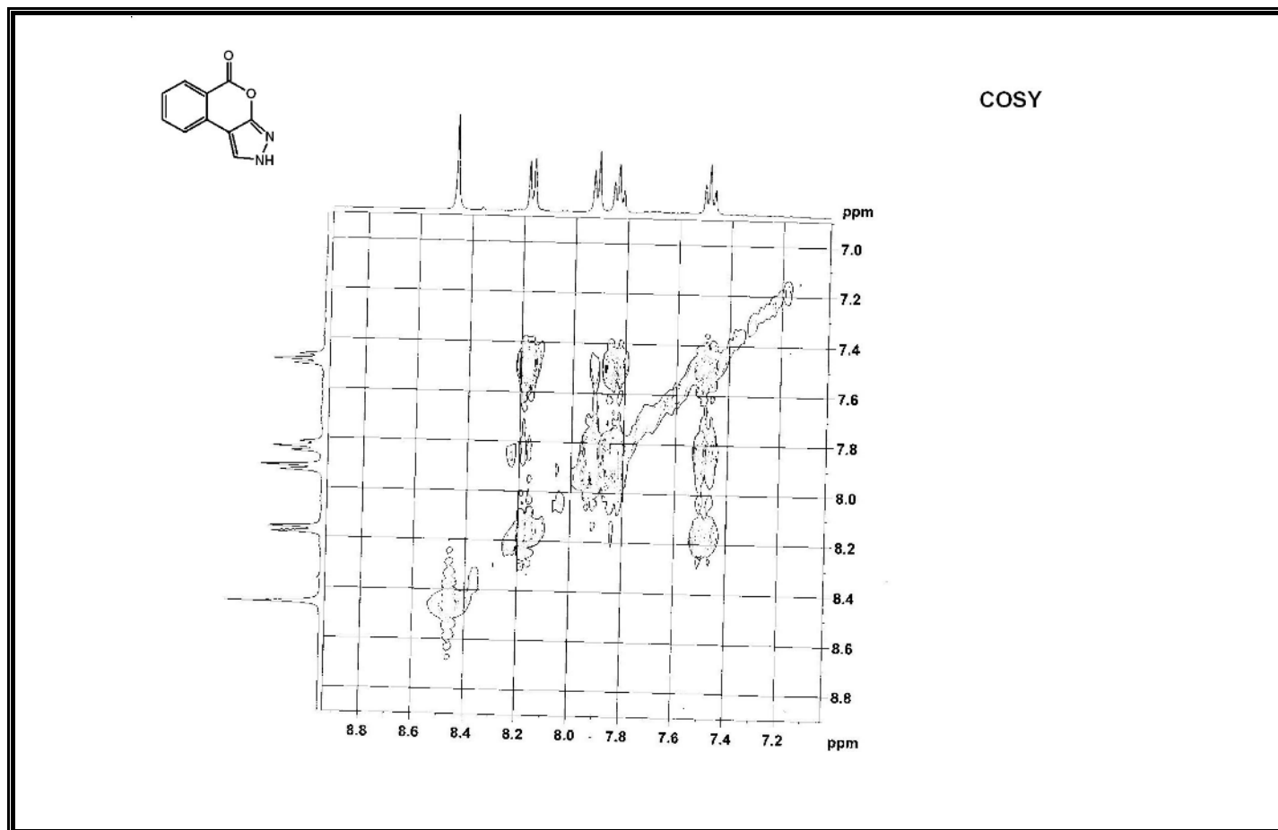
Figure A208 Expanded COSY Spectrum of Compound 407 .
