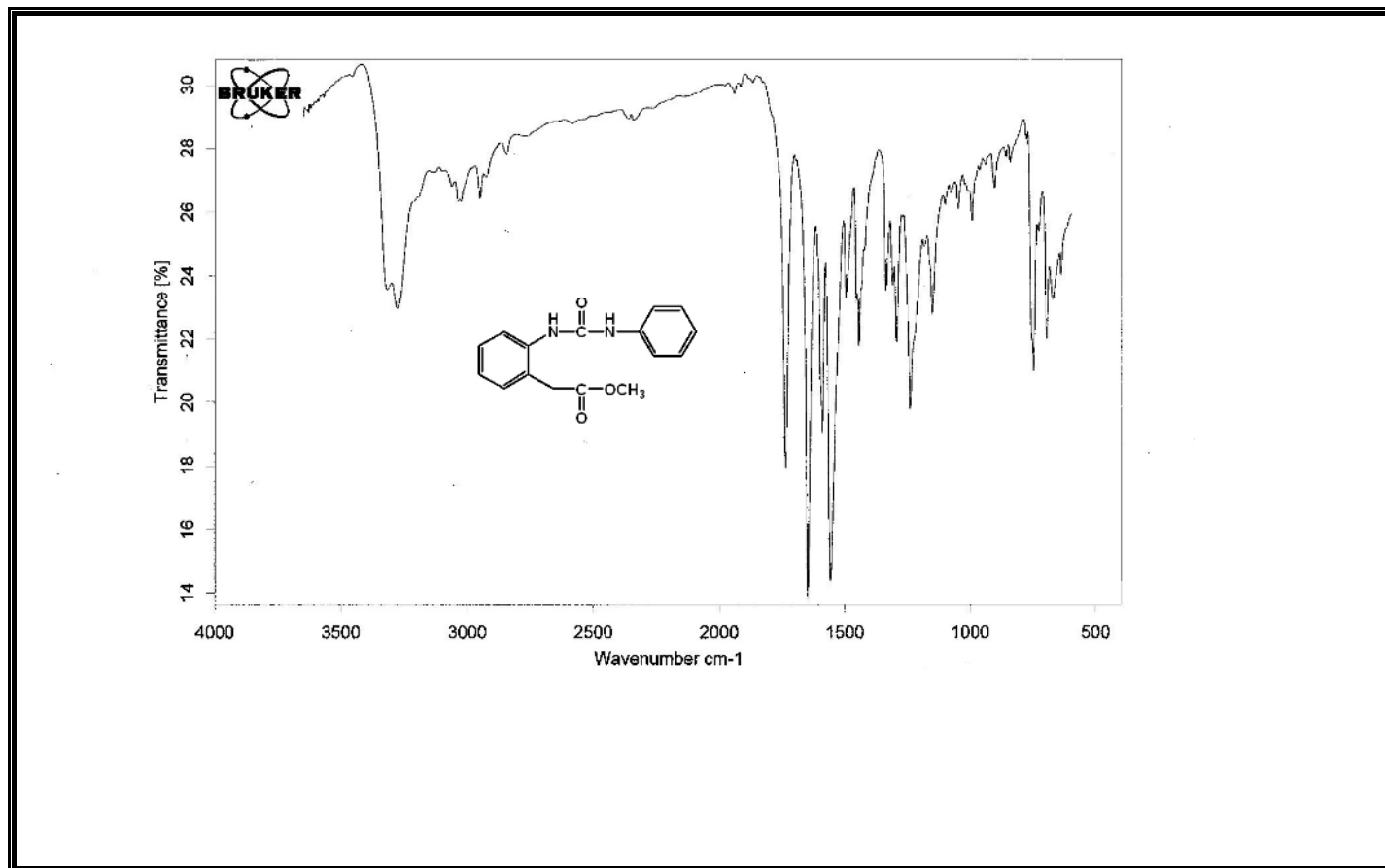
Figure A112 IR Spectrum of Compound 374.
