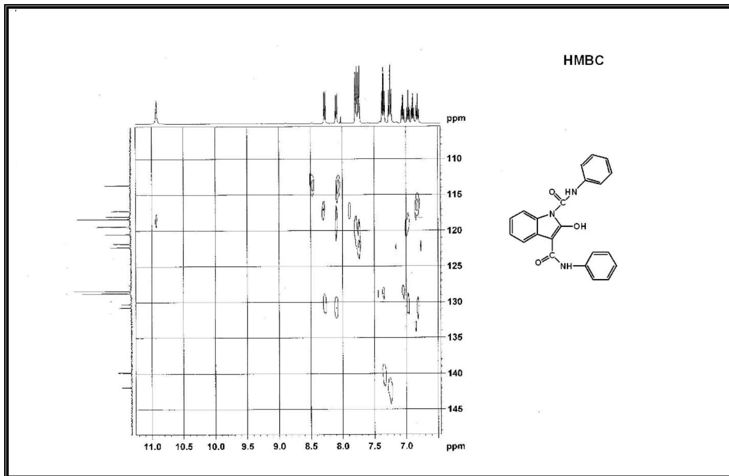
Figure A128 Expanded HMBC Spectrum of Compound 379 .
