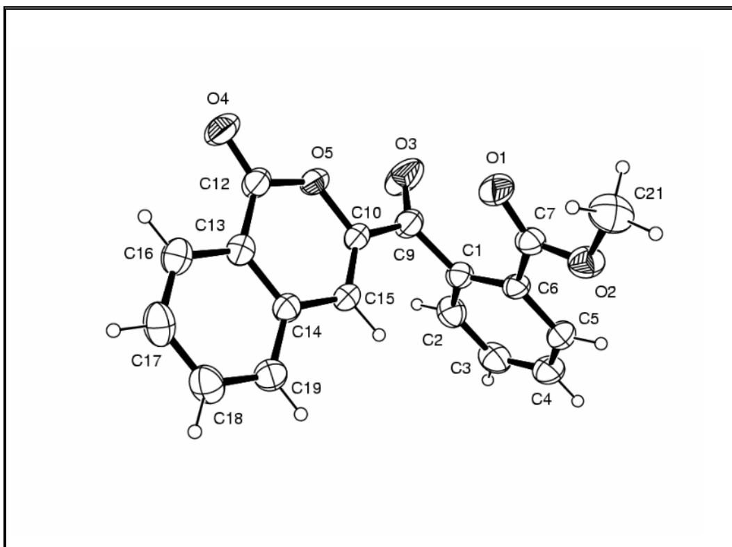
Figure 7. The X-ray crystal structure of the compound 340 .
