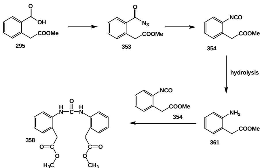
Scheme 9. Suggested mechanism for the formation of the compound 358 .
