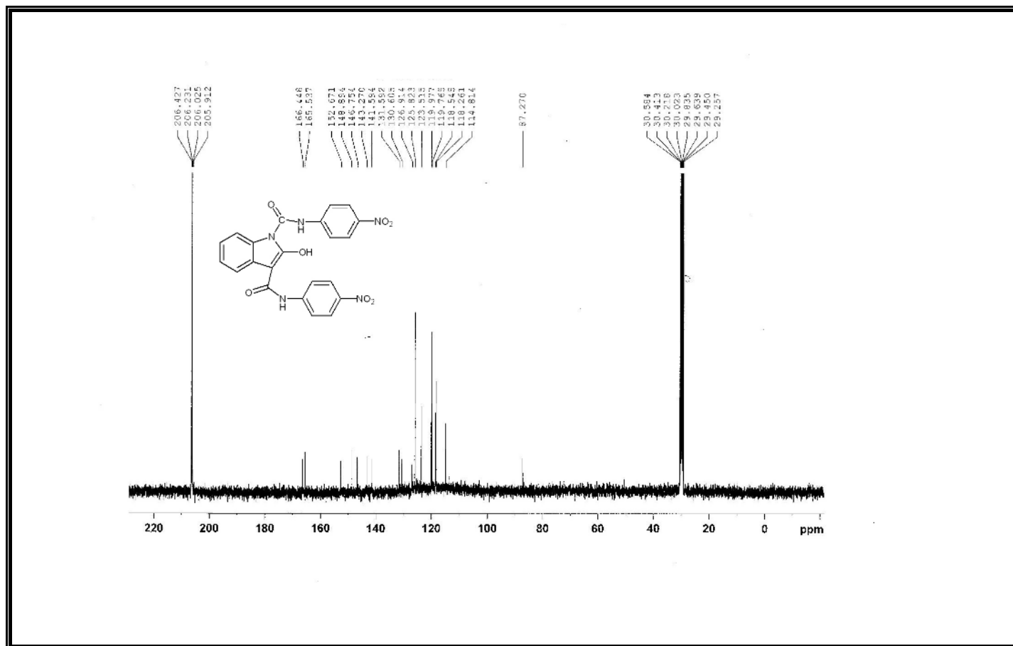
Figure A134 ^{13}\text{C} -NMR Spectrum of Compound 381.
