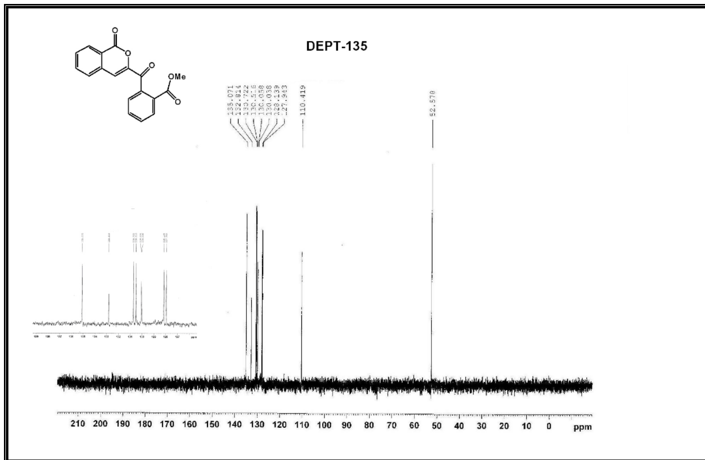
Figure A39 DEPT-135 Spectrum of Compound 340.
