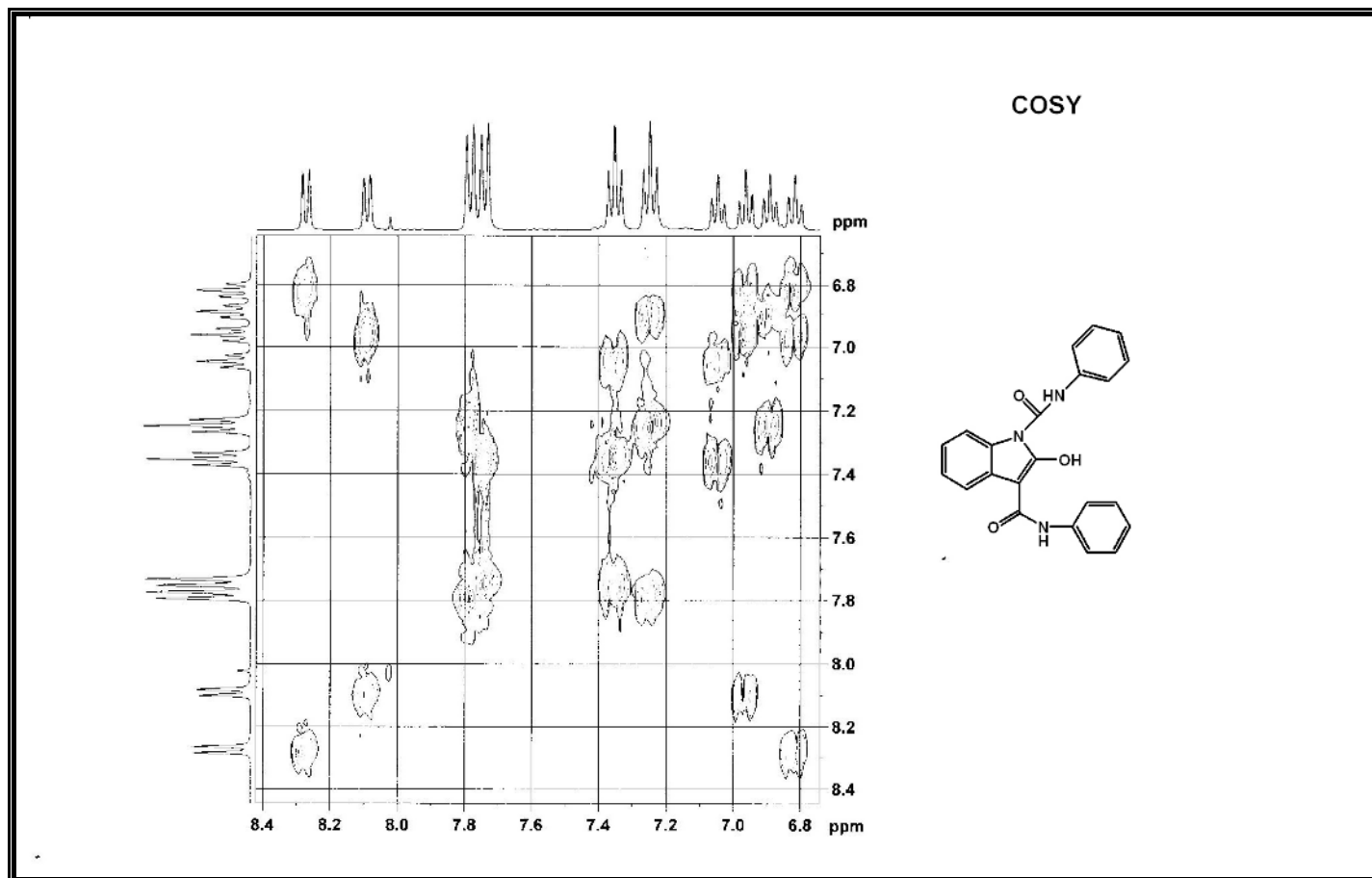
Figure A126 Expanded COSY Spectrum of Compound 379.
