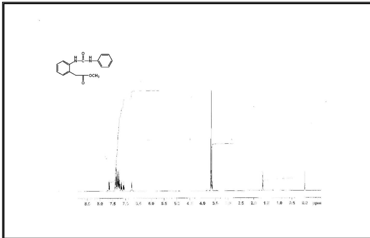
Figure A110 ^1\text{H} -NMR Spectrum of Compound 374.
