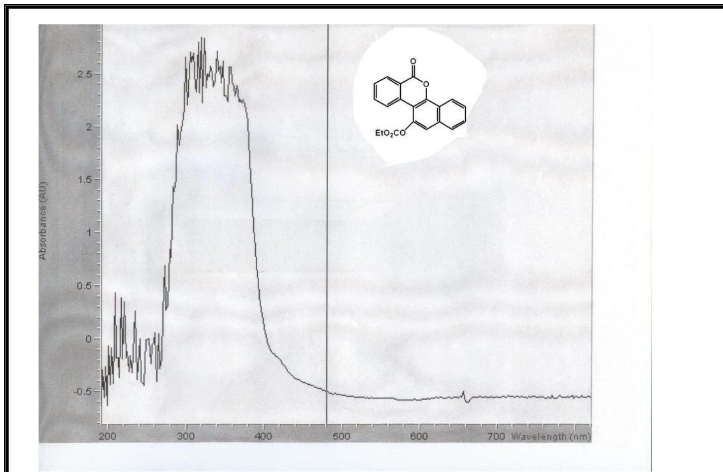
Figure A24 UV Spectrum of Compound 333.
