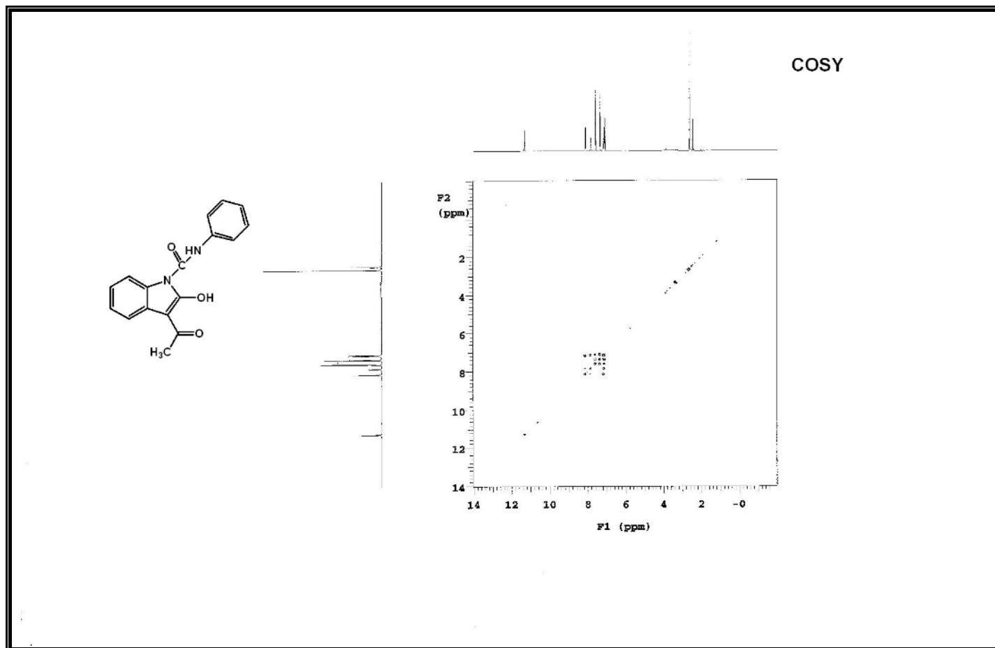
Figure A176 COSY Spectrum of Compound 394.
