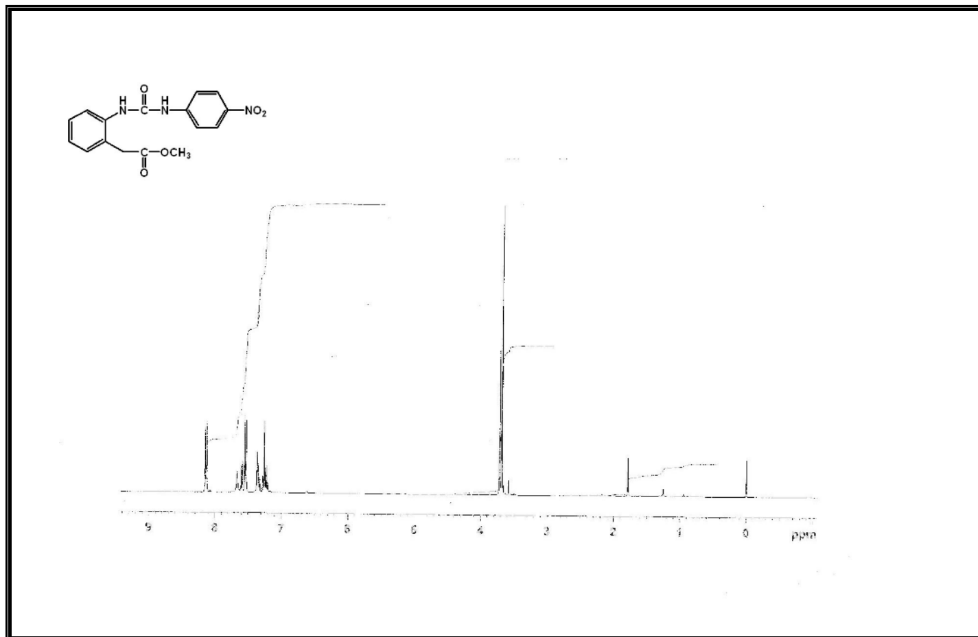
Figure A116 1 H-NMR Spectrum of Compound 378.
