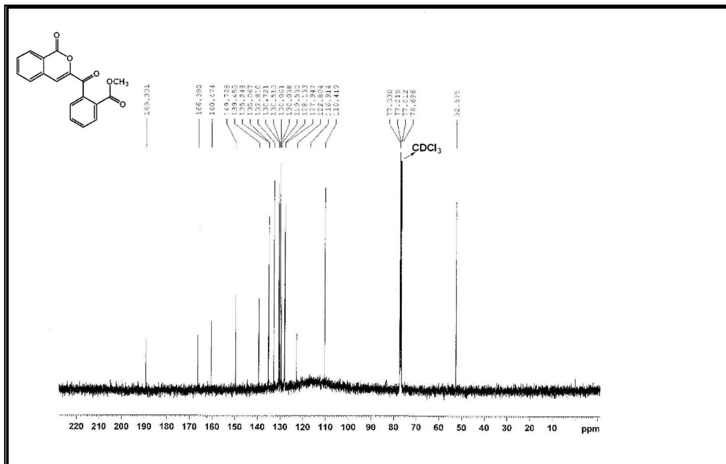
Figure A37 13 C-NMR Spectrum of Compound 340.
