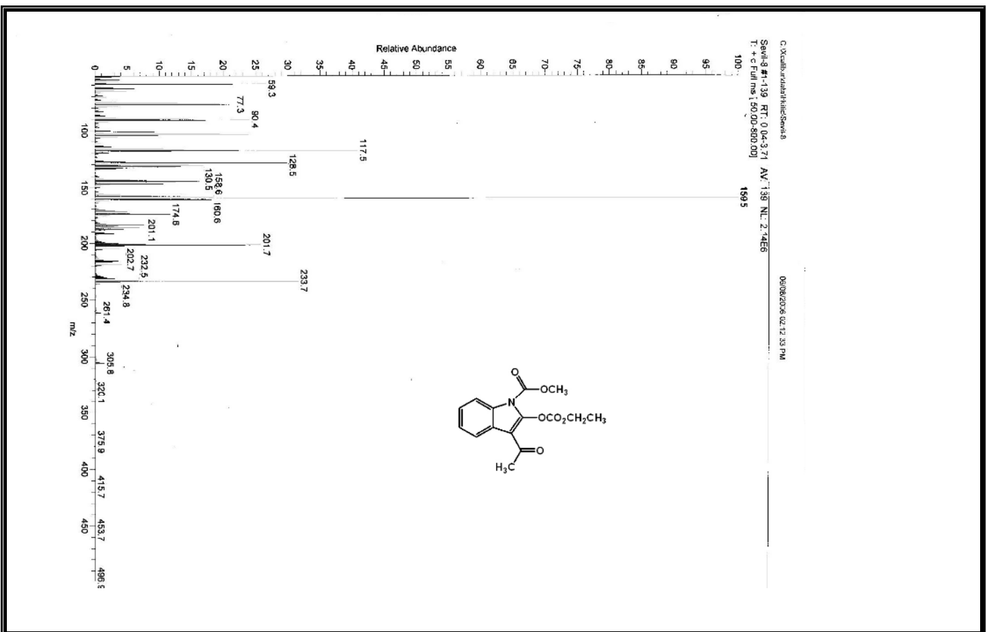
Figure A149 Mass Spectrum of Compound 387.
