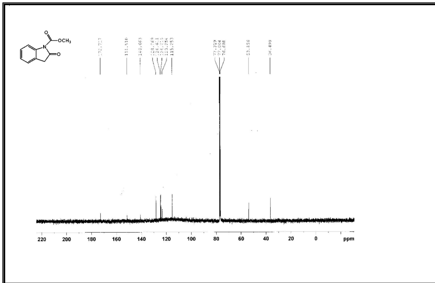
Figure A142 13 C-NMR Spectrum of Compound 384.
