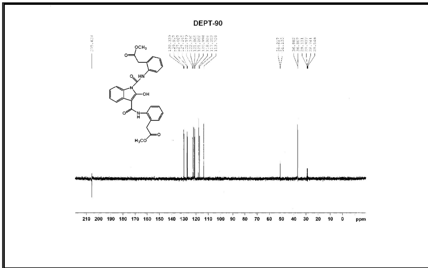
Figure A93 DEPT-90 Spectrum of Compound 368 .
