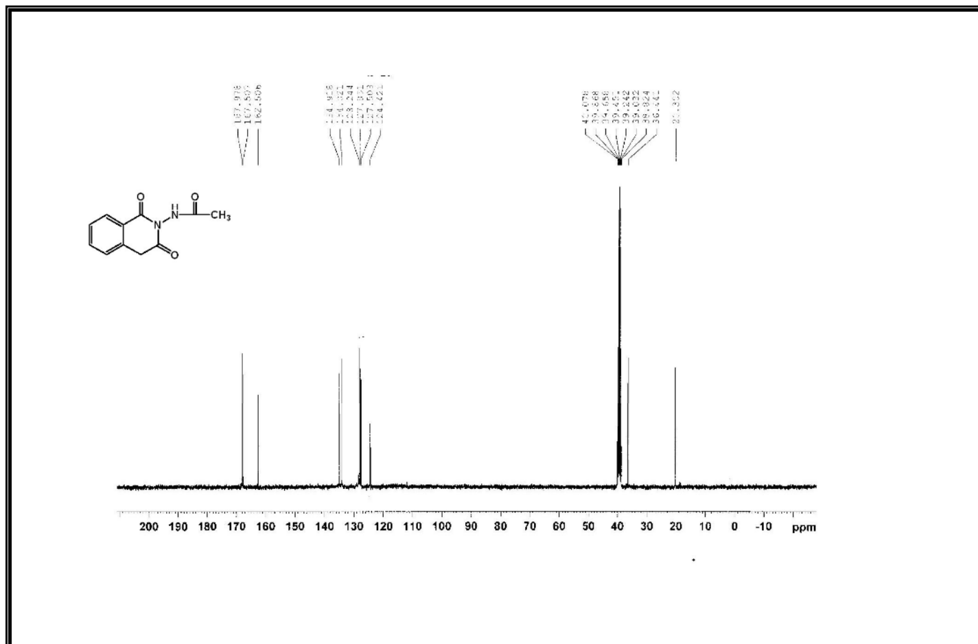
Figure A198 13 C-NMR Spectrum of Compound 405.
