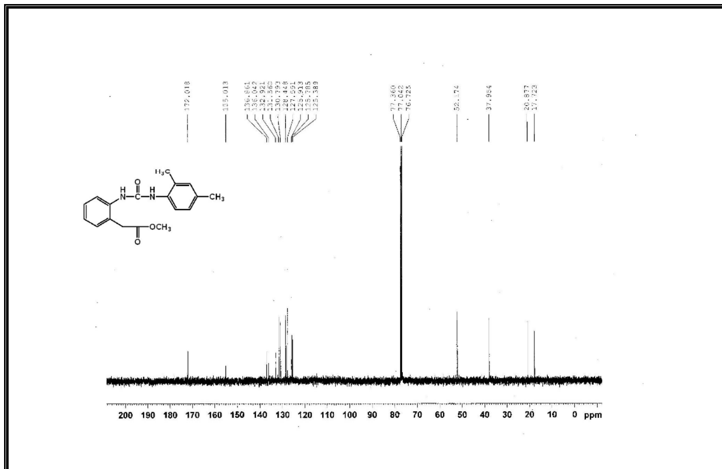
Figure A114 13 C-NMR Spectrum of Compound 376.
