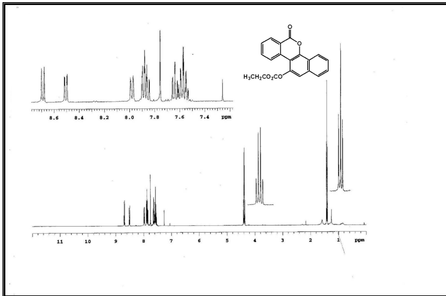
Figure A14 ^1\text{H} -NMR Spectrum of Compound 333.
