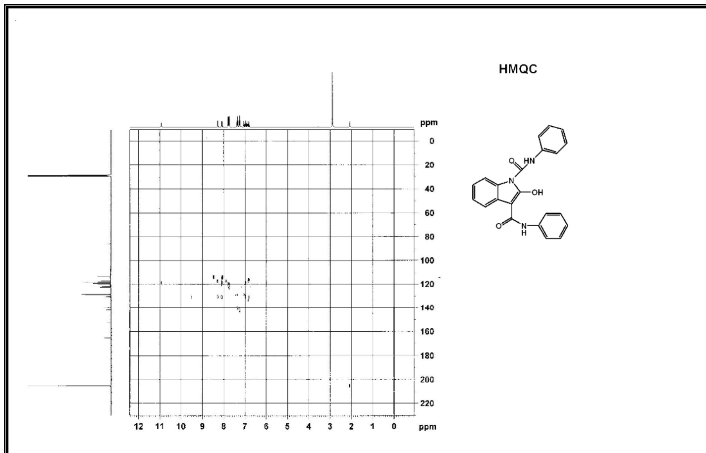
Figure A123 HMQC Spectrum of Compound 379.
