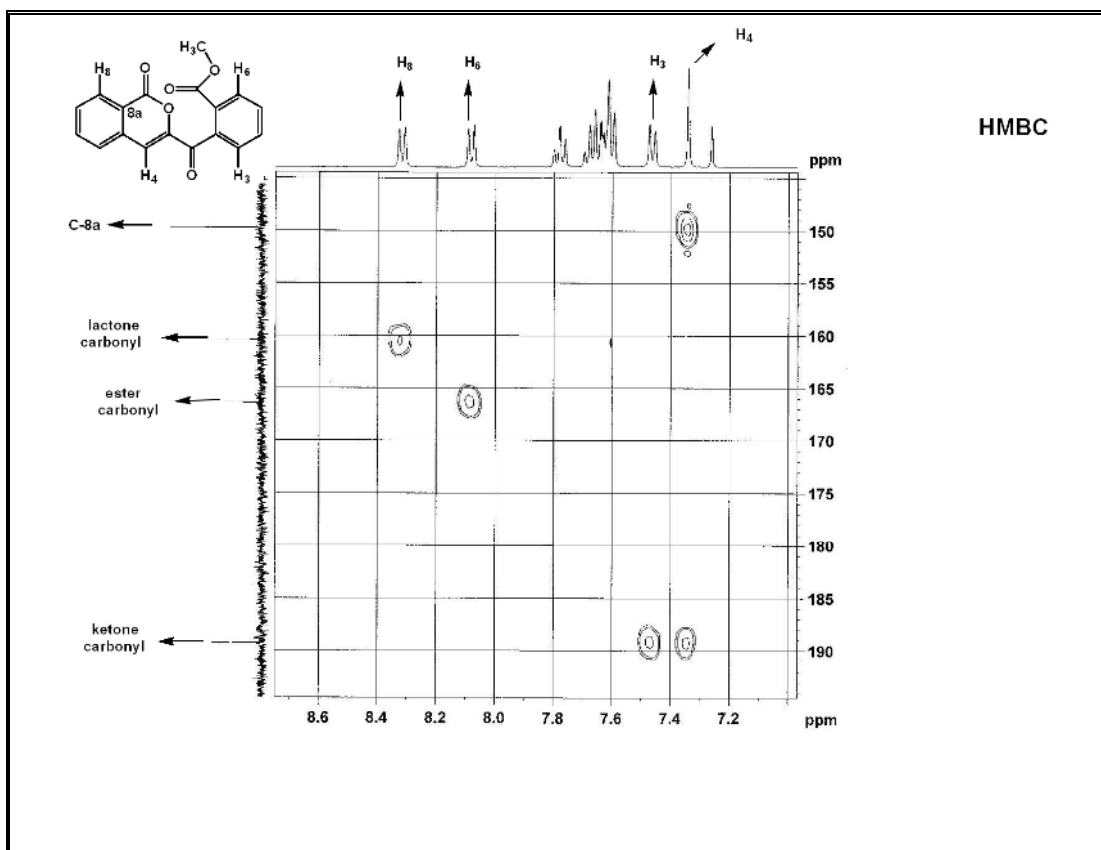
Figure 6. A part of HMBC experiment of 340 .
