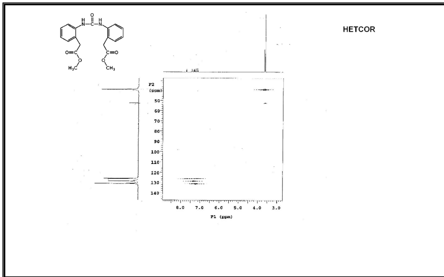
Figure A82 HETCOR Spectrum of Compound 358.
