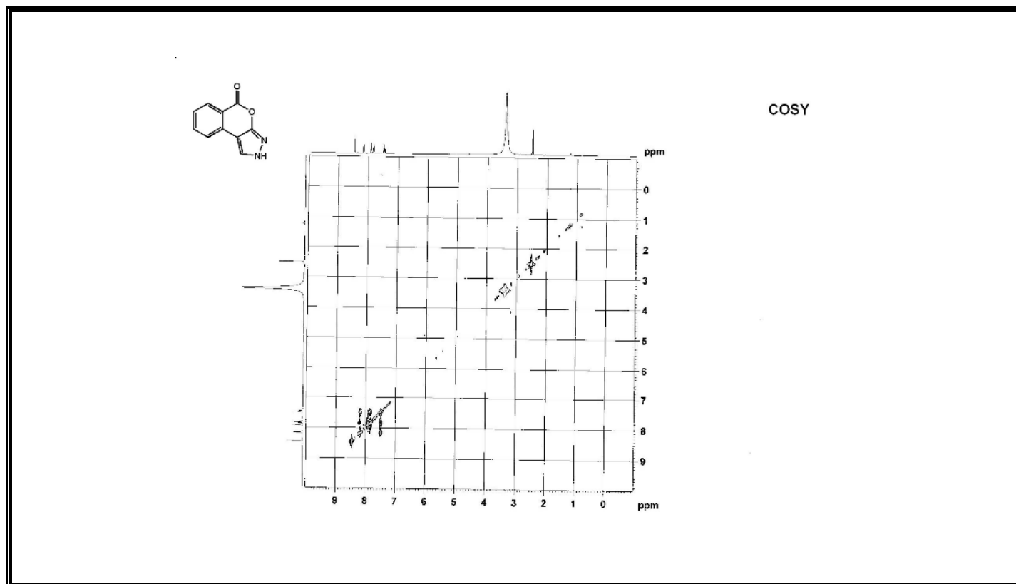
Figure A207 COSY Spectrum of Compound 407.
