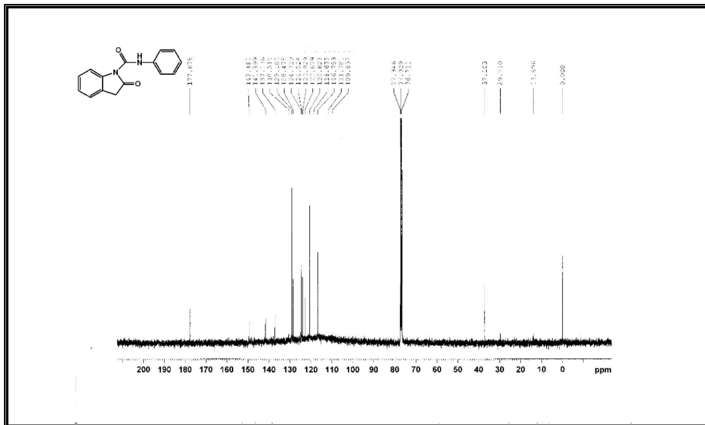
Figure A182 ^{13}\text{C} -NMR Spectrum of Compound 395.
