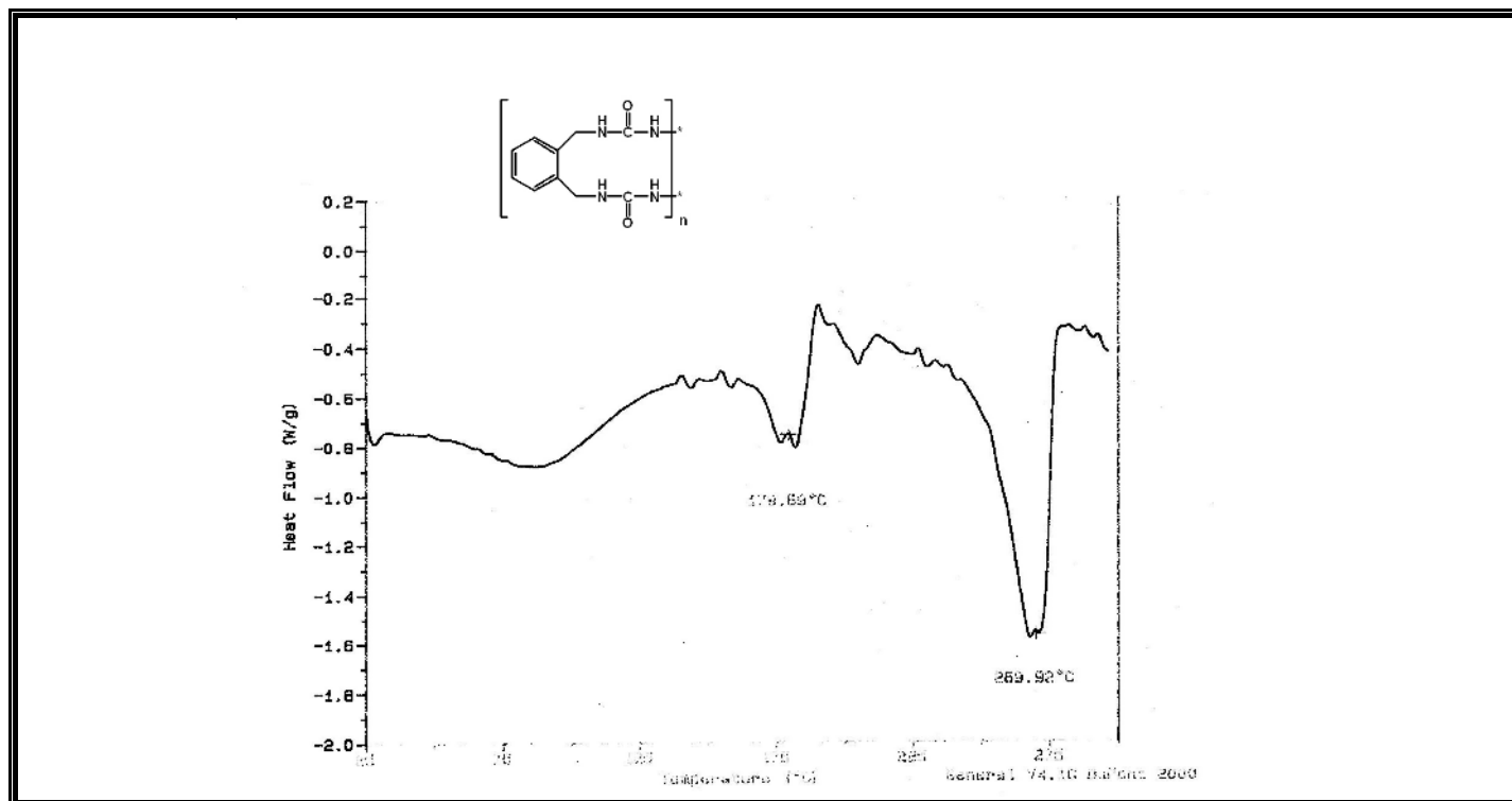
Figure A230 DSC Spectrum of Compound 424.
