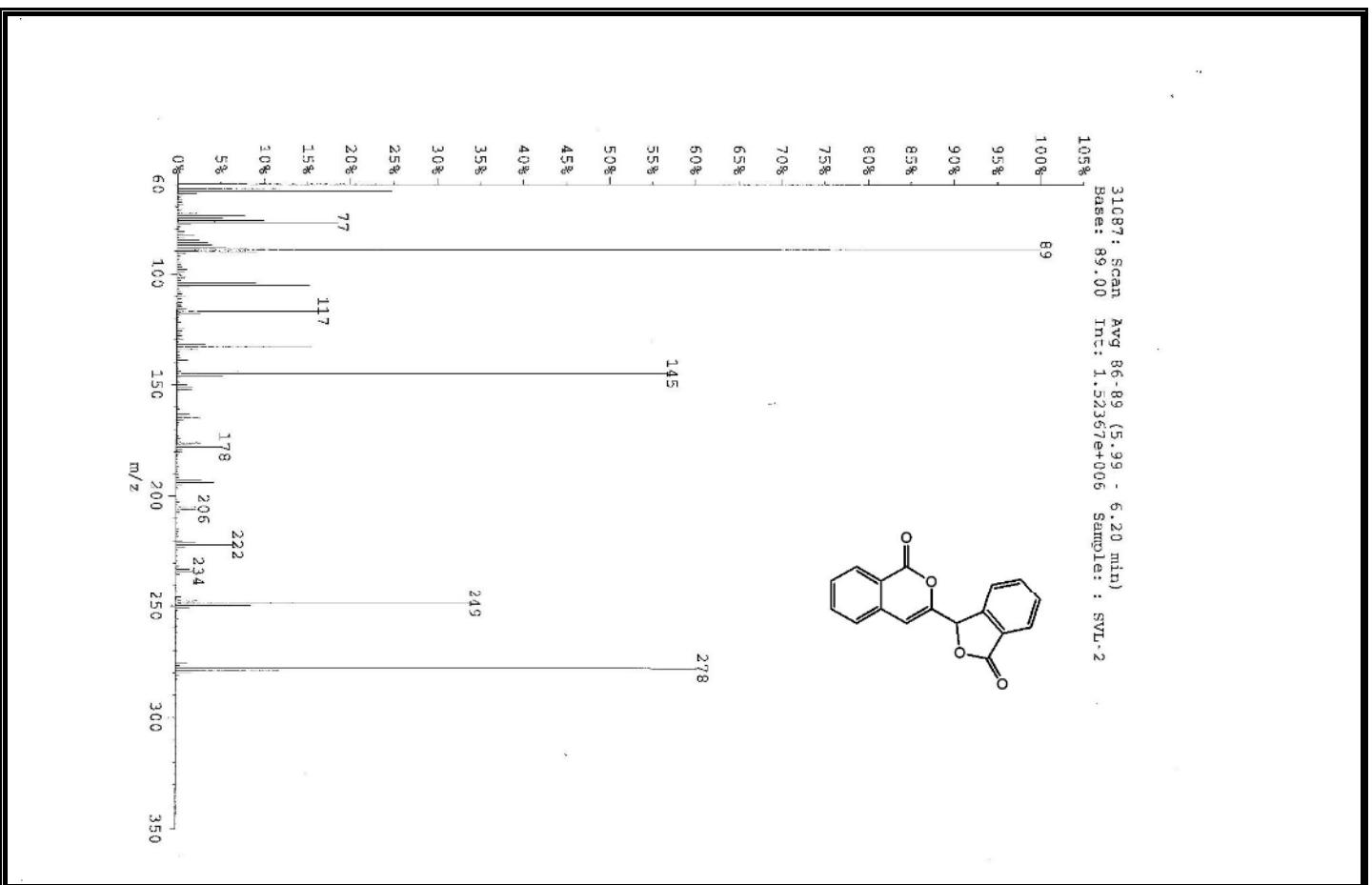
Figure A58 High Resolution Mass Spectrum of Compound 334 .
