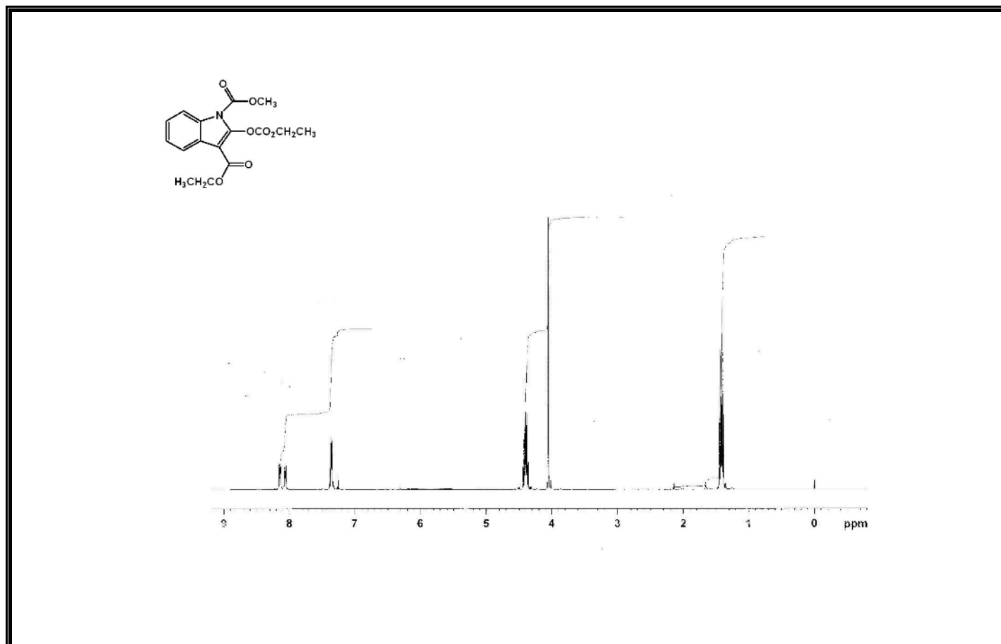
Figure A153 ^1\text{H} Spectrum of Compound 390.
