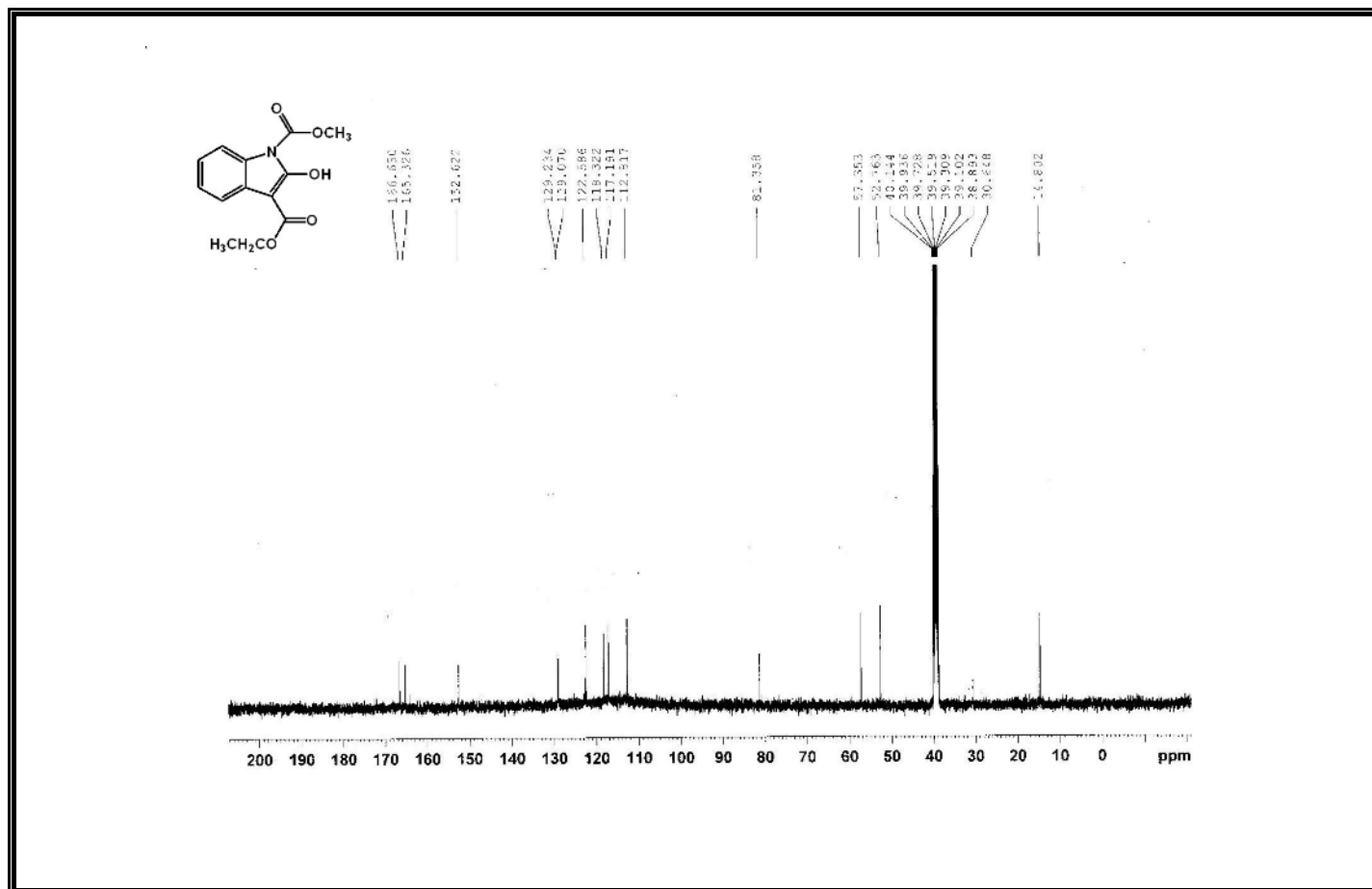
Figure A151 ^{13}\text{C} -NMR Spectrum of Compound 388
