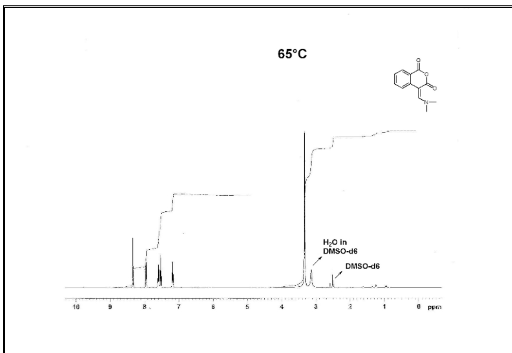
Figure 3. The 1 H-NMR spectrum of the compound 327 at 65°C.
