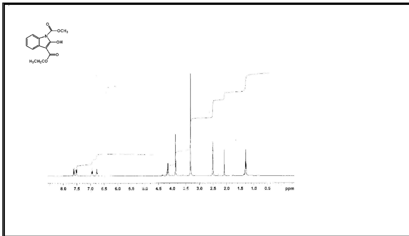
Figure A150 ^1\text{H} -NMR Spectrum of Compound 388.
