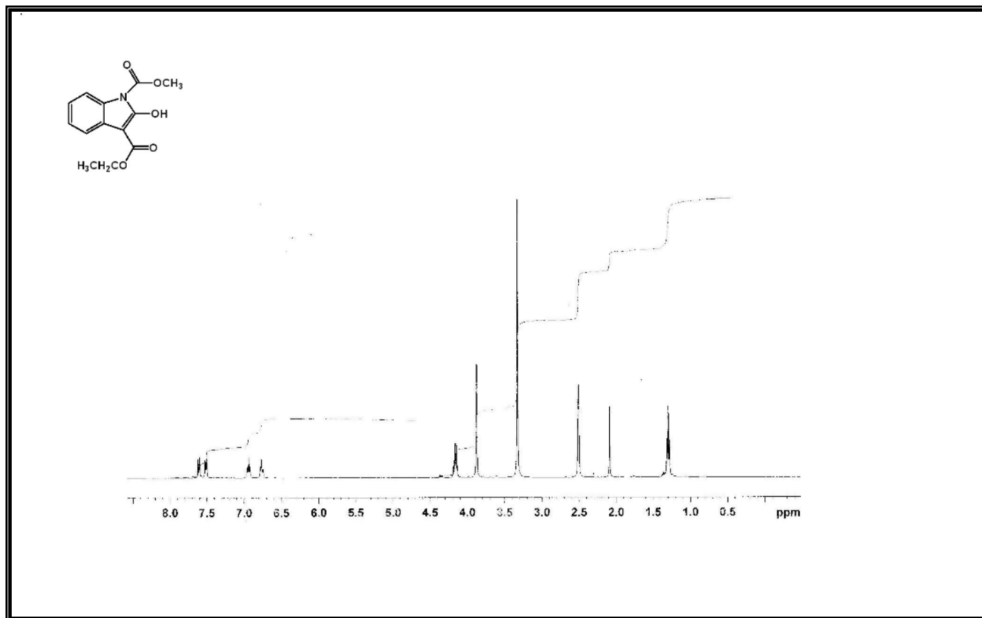
Figure A159 ^1\text{H} -NMR Spectrum of Compound 388 .
