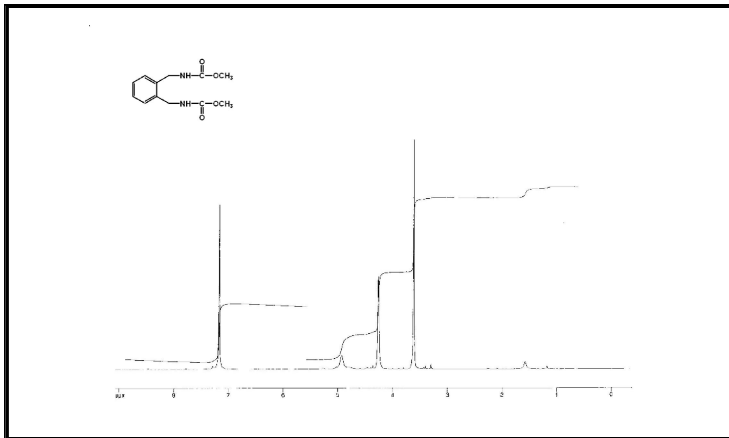
Figure A215 ^1\text{H} -NMR Spectrum of Compound 418.
