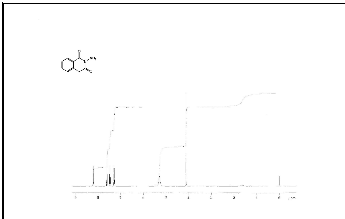
Figure A195 ^1\text{H} -NMR Spectrum of Compound 404.
