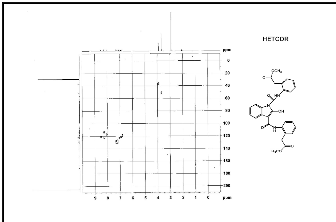
Figure A97 HETCOR Spectrum of Compound 368.
