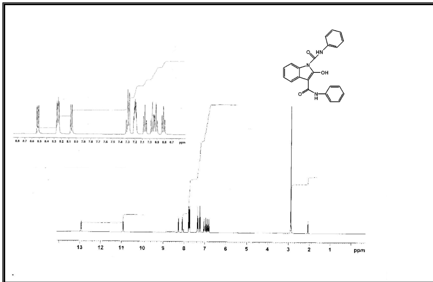
Figure A119 ^1\text{H} -NMR Spectrum of Compound 379.
