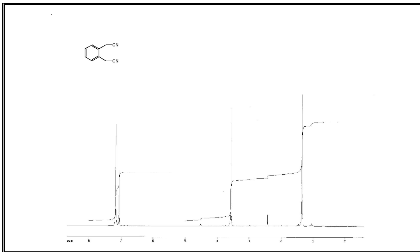
Figure A211 ^1\text{H} -NMR Spectrum of Compound 414 .
