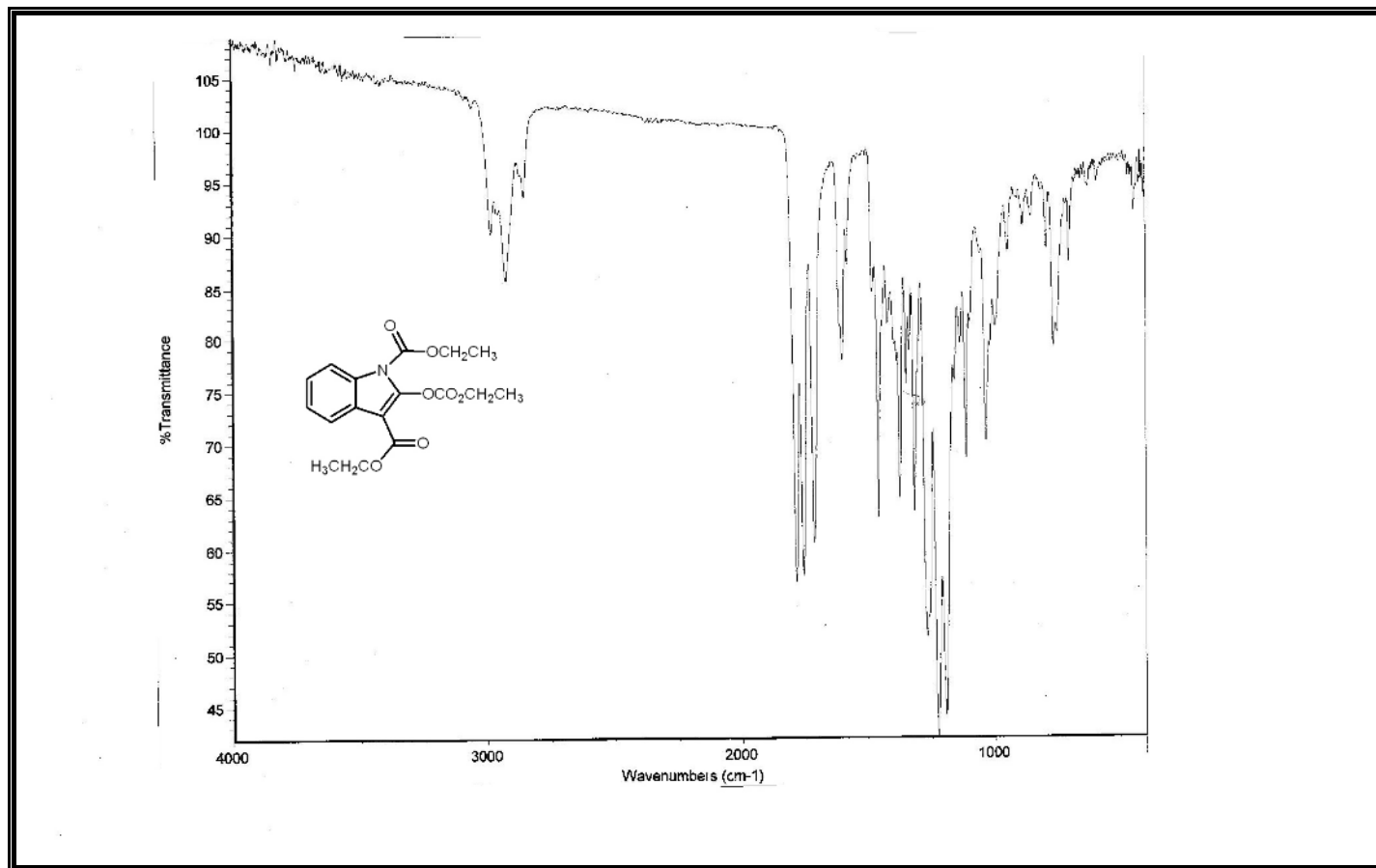
Figure A167 IR Spectrum of Compound 392.
