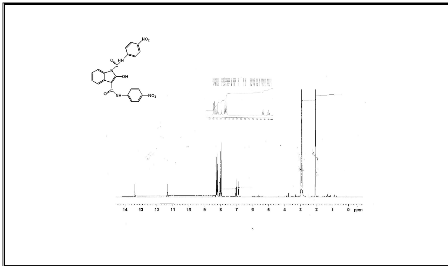
Figure A133 ^1\text{H} -NMR Spectrum of Compound 381.
