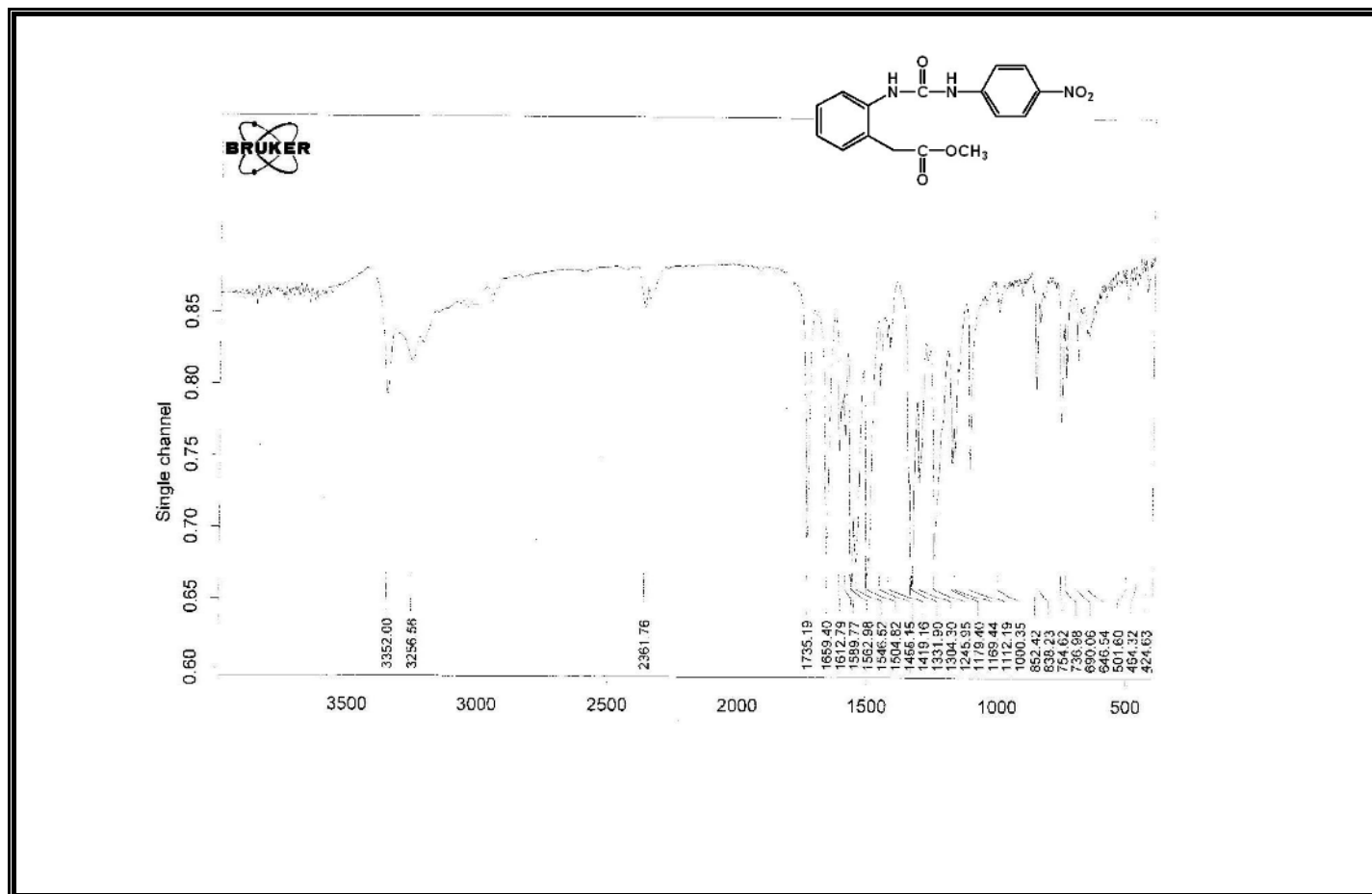
Figure A118 IR Spectrum of Compound 378.
