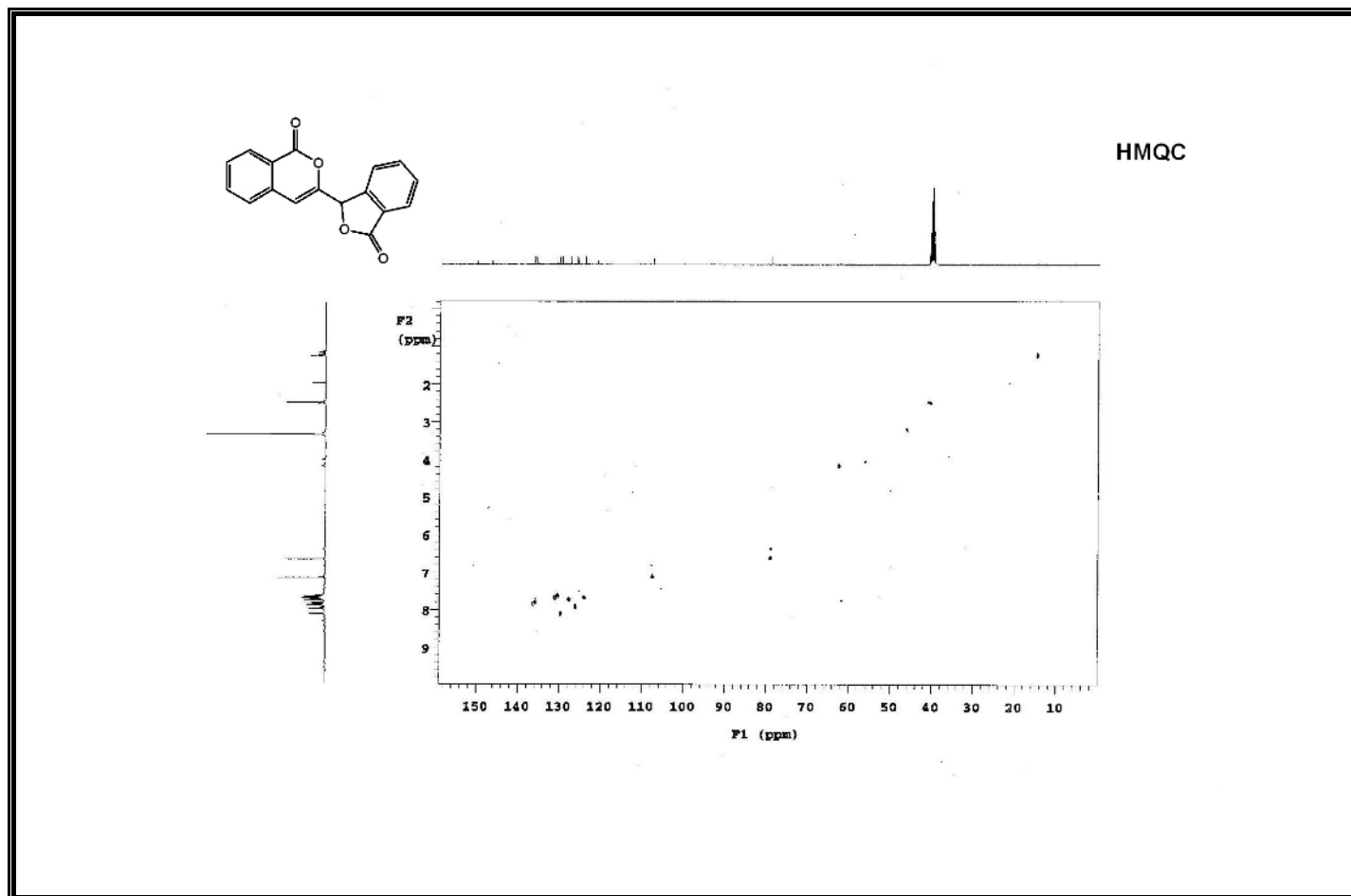
Figure A52 HMQC Spectrum of Compound 334.
