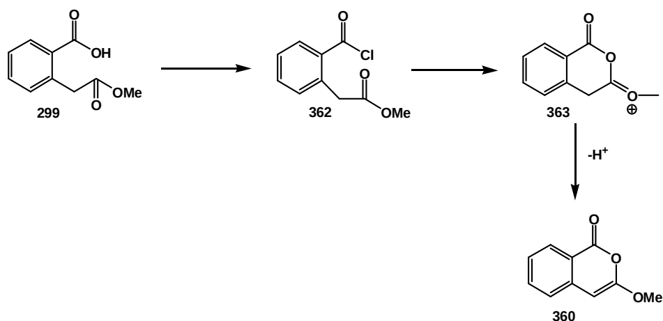
Scheme 11. Suggested mechanism for the formation of the compound 360 .
