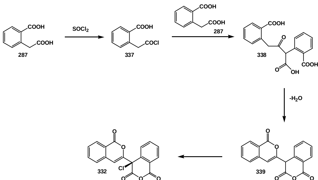
Scheme 5. Suggested mechanism for the formation of the compound 332 .
