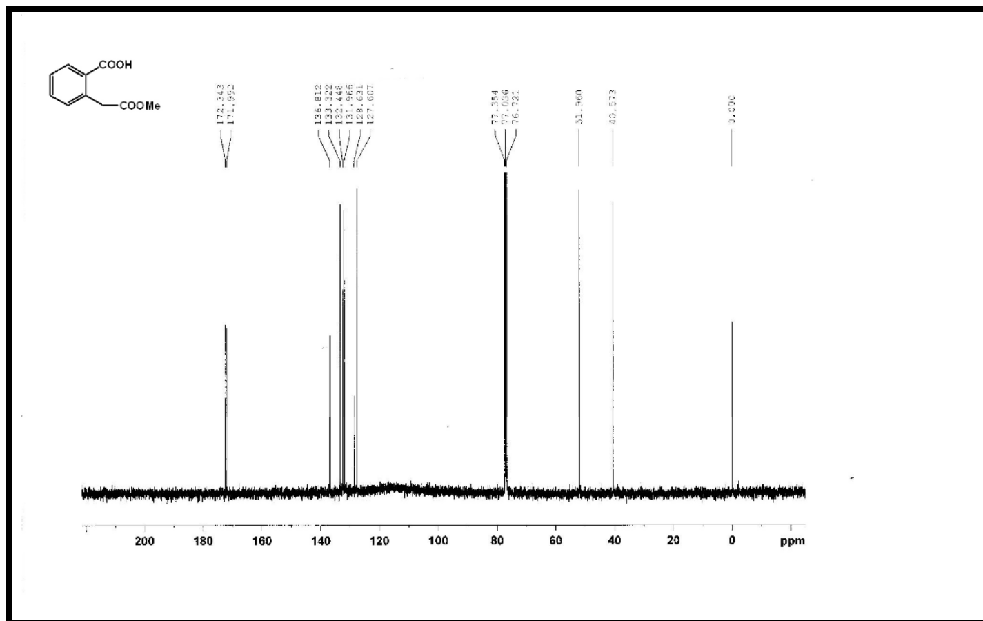
Figure A4 ^{13}\text{C} -NMR Spectrum of Compound 299.
