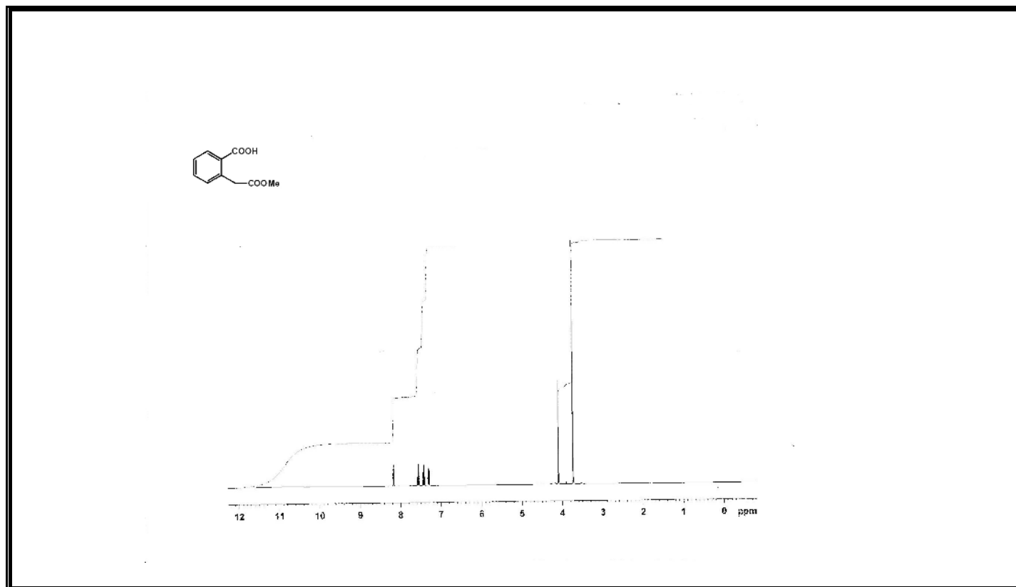
Figure A3 ^1\text{H} -NMR Spectrum of Compound 299.
