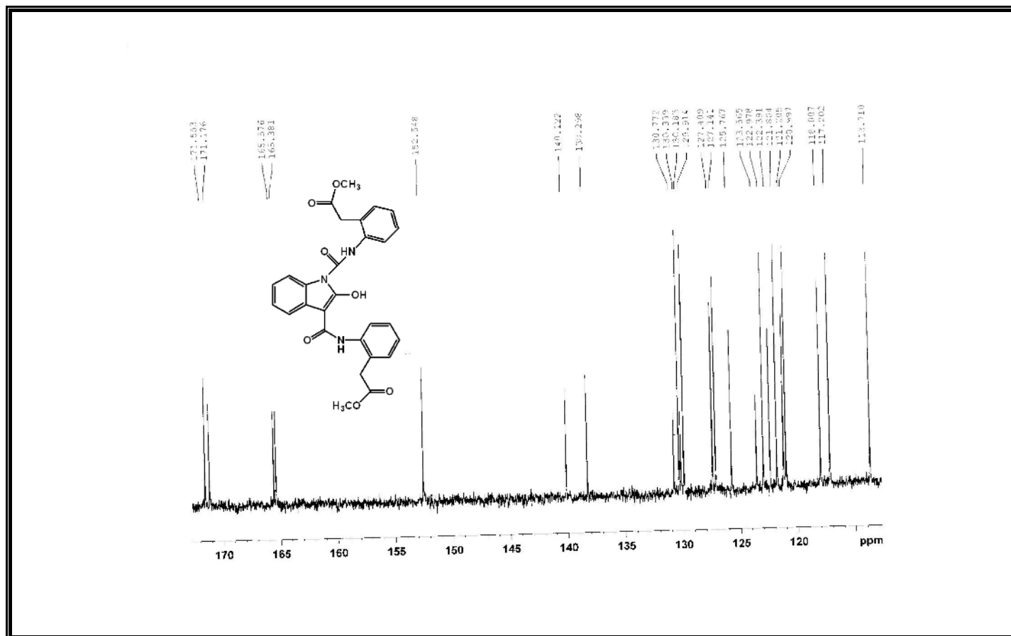
Figure A92 Expanded 13 C-NMR Spectrum of Compound 368.
