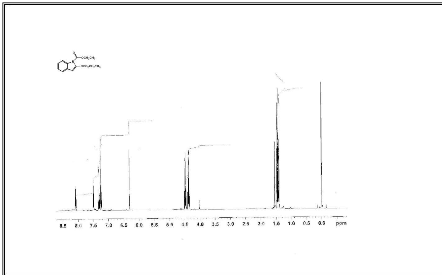
Figure A168 1 H-NMR Spectrum of Compound 393.
