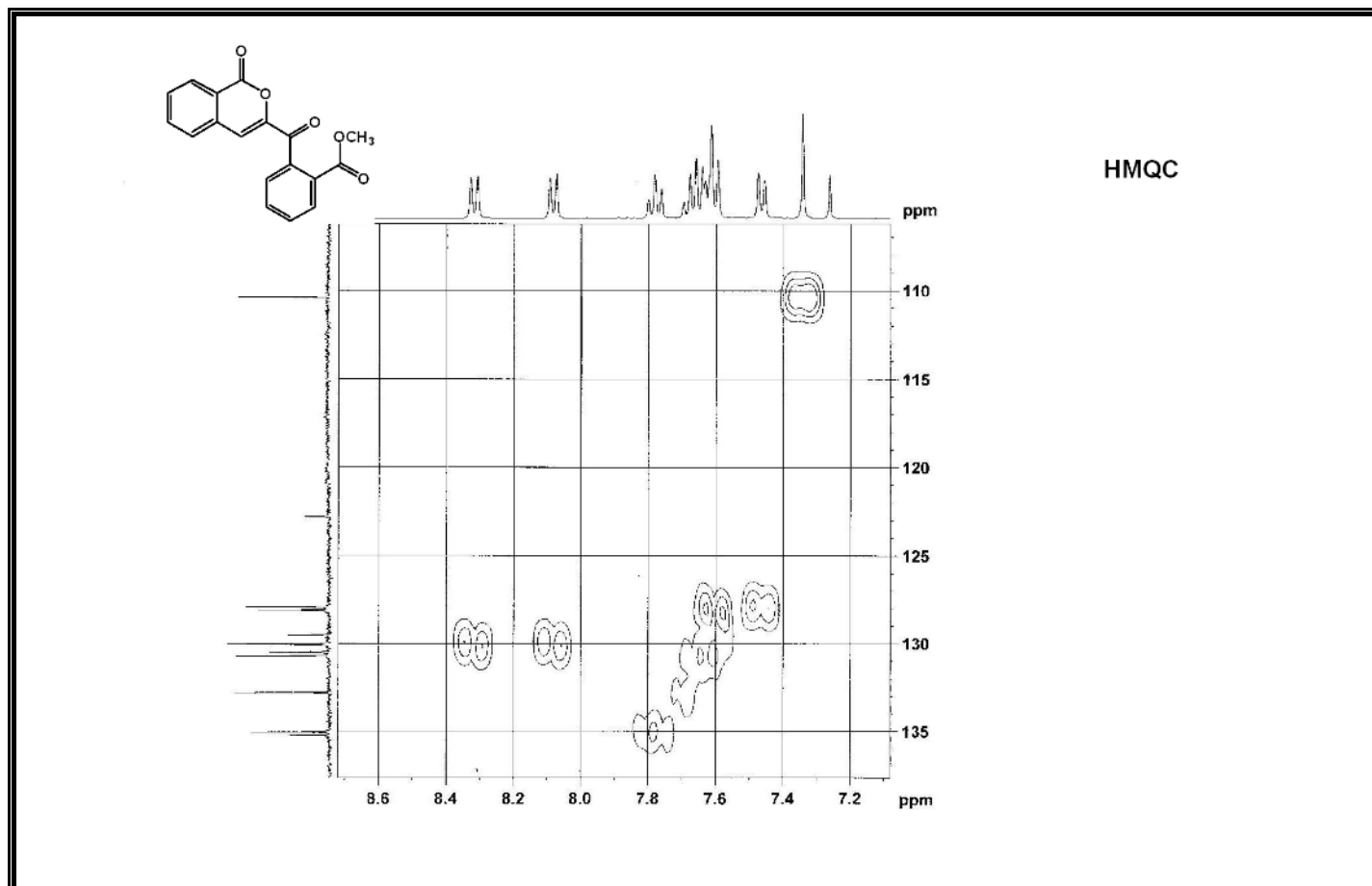
Figure A43 Expanded HMQC Spectrum of Compound 340.
