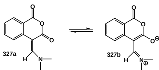
Scheme 3. The chemical equilibrium of compound 327 .
