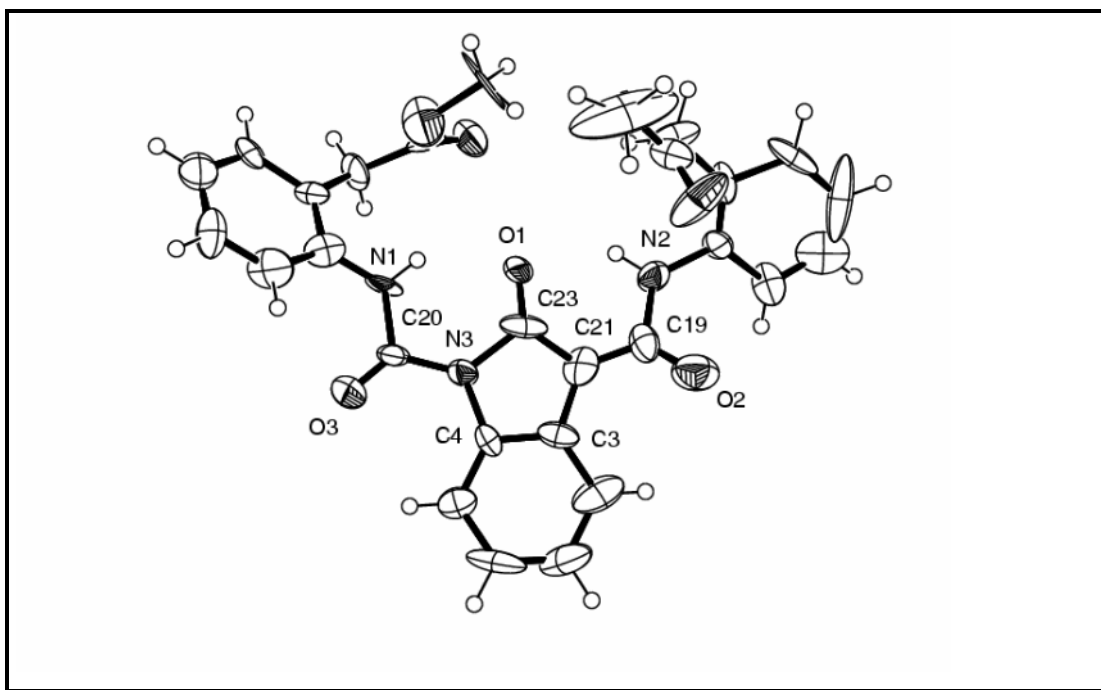
Figure 14. The X-ray crystal structure of the compound 368 .
