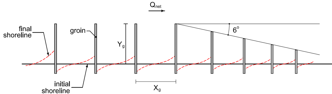
Figure 3.19 Definition sketch for a groin field
