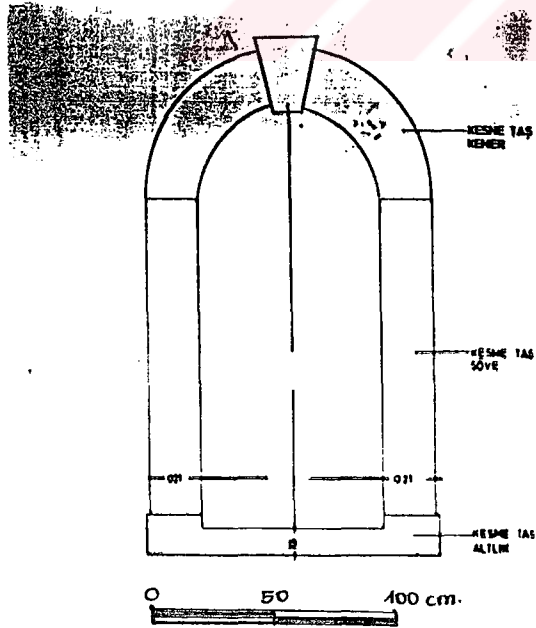
ÇİZİM.V.II.7.14-DAİRESEL, BASIK KEMERLİ PENCERE.
