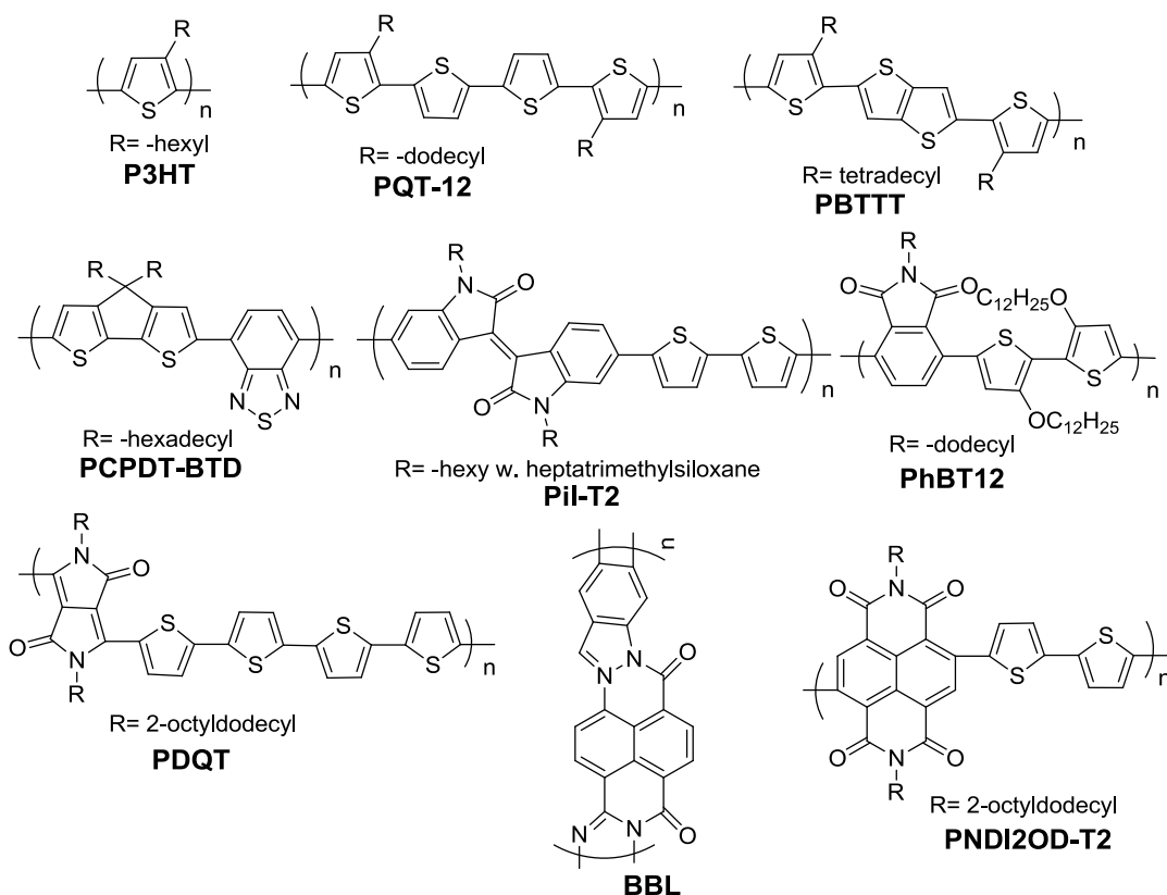
Figure 1-16. Representative hole and electron transporting polymers exceeding 0.1 \text{ cm}^2/\text{V.s.} mobilities in OFET devices.
