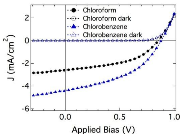
Figure 3-14. Solar cell characteristics of APFO-DOT processed from chloroform (black) and chlorobenzene (blue)(Adapted with permission from Reynolds, Copyright 2011 Royal Chemical Society)
