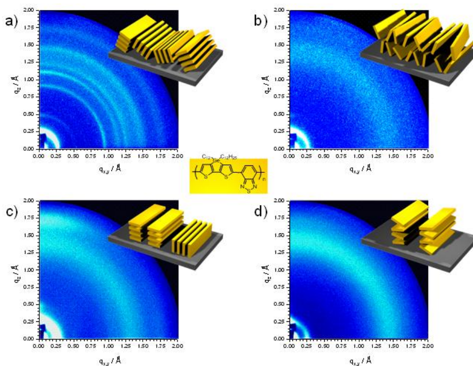
Figure 5-9. GIWAXS characterization of E(DTG-BTD) and NE(DTG-BTD) a) and c) patterns of drop-cast and spin-coated E(DTG-BTD), b) and d) patterns of drop-cast and spin-coated NE(DTG-BTD). Insets schematically illustrate the surface organization of the polymers.
