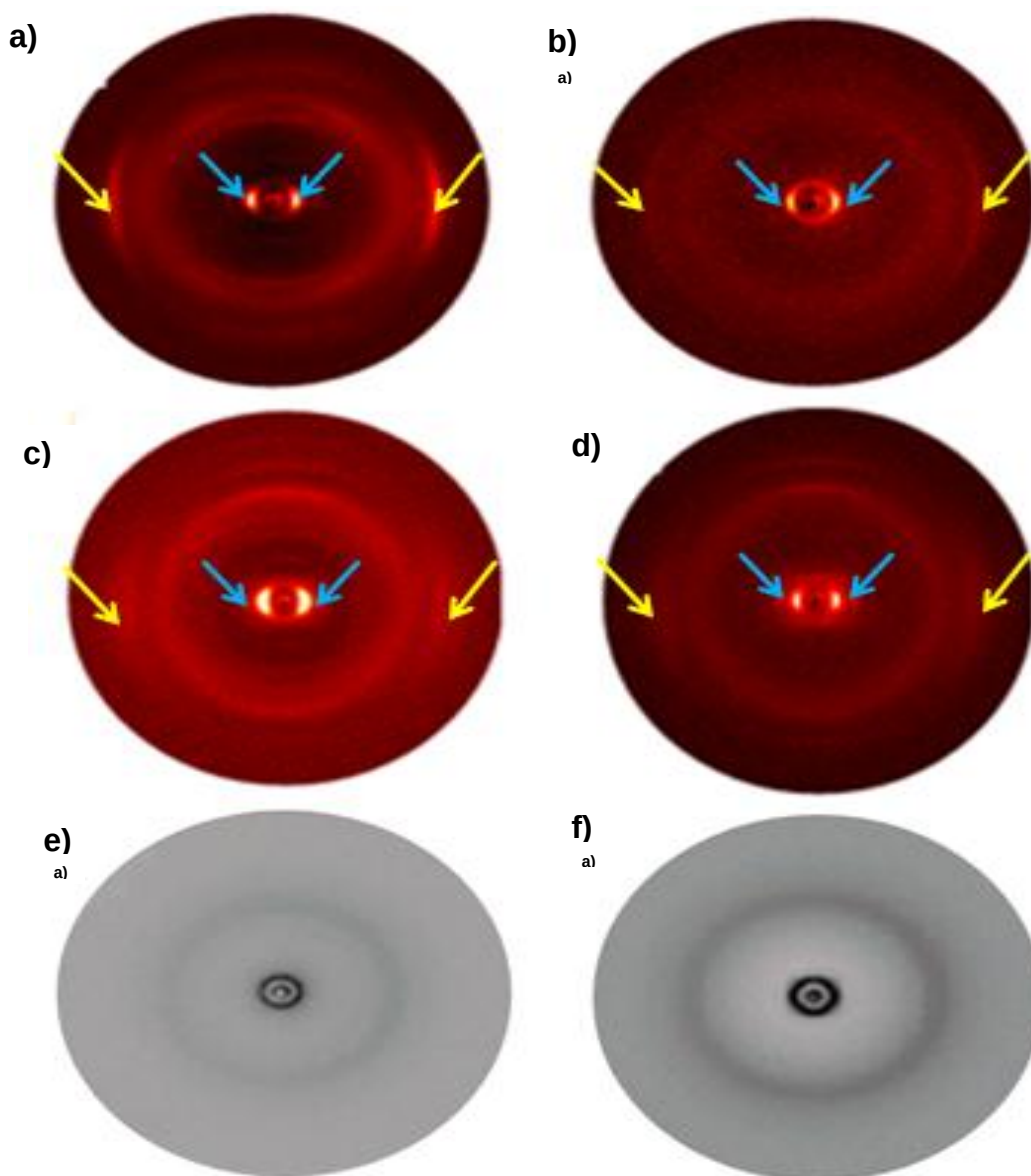
Figure 4-12. Extruded fiber 2D-WAXS patterns measured for DTS and DTG polymers. a) PGe12-BTD, b) PSi12-BTD, c) PGe12-TPD, d) PSi12-TPD, e) PGe12-PT and f) PSi12-PT at 30 °C after annealing the fibers at 200 °C. Yellow arrows show the reflections due to \pi - \pi stacking and blue arrows highlight the reflections due to lamellar interactions. The PGe12-PT and PSi12-PT patterns are shown in grayscale to increase the contrast.
