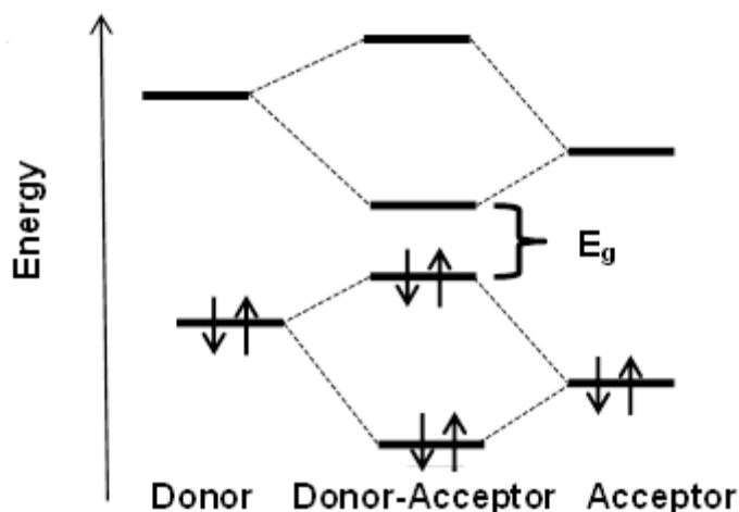
Figure 1-2. Reduction of the band gap in a donor-acceptor copolymer.
