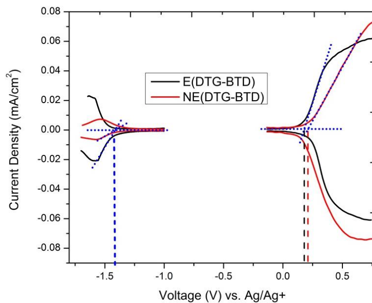
Figure 5-7. Differential Pulse Voltammograms of E(DTG-BTD) (black, solid line) and NE(DTG-BTD) (red, solid line) recorded in 0.1 M TBAPF 6 /PC electrolyte solution with a scan rate of 50 mV/s vs. Ag/Ag + reference electrode.
