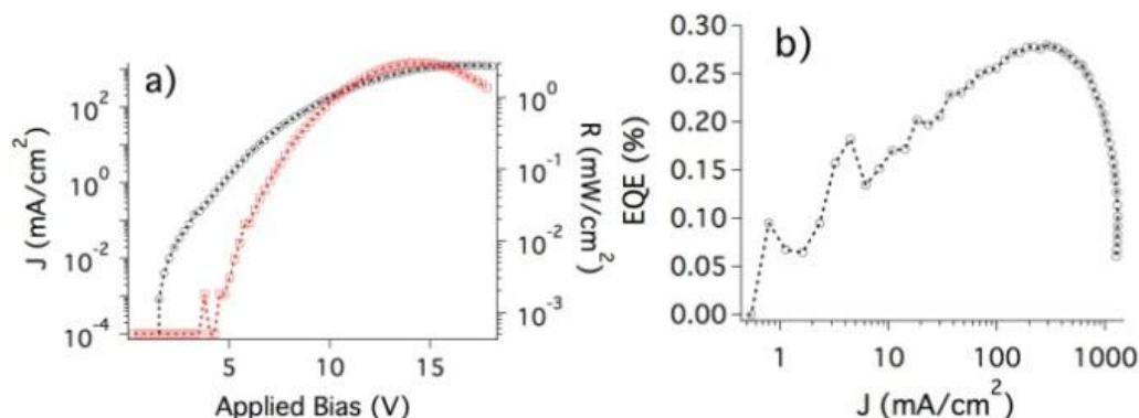
Figure 3-12. PLED properties of APFO-DOT. a) Current density and radiant emittance as a function of applied bias for APFO-DOT based PLED. b) The evaluation of EQE as a function of current density. (Adapted with permission from Reynolds, Copyright 2011 Royal Chemical Society)
