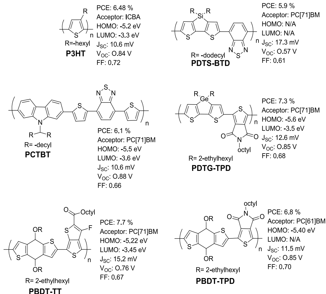
Figure 1-19. Representative high performing OPV polymers with their solar cell parameters.
