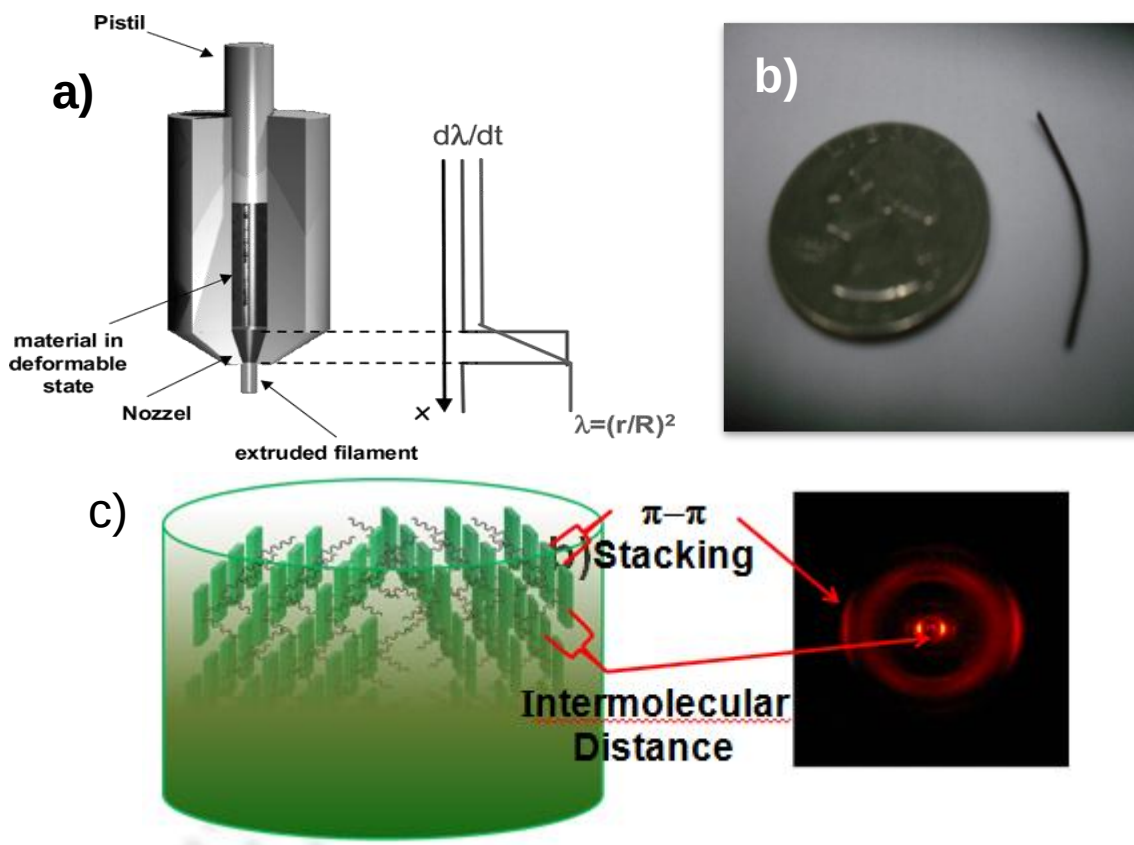
Figure 2-3. Preparation and analysis of a polymer via 2D-WAXS. a) Schematic illustration of extrusion process. (Adapted with permission from Muellen, Copyright 2005 American Chemical Society) b) The extruded polymer fiber prepared and comparison with a US quarter. c) Representation of an extruded fiber and the aligned polymer chains along the extrusion direction as well as relating \pi - \pi stacking and intermolecular distances in an obtained X-ray pattern.
