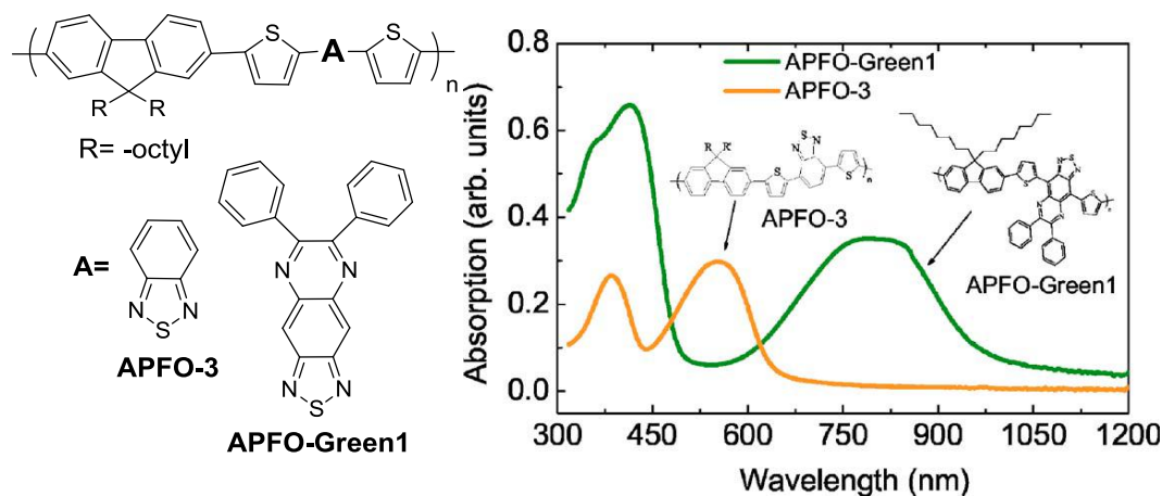
Figure 1-5. Repeat unit structures for the APFO type polymers displaying green and purple color along with their normalized absorption spectra. (Adapted with permission from Andersson)
