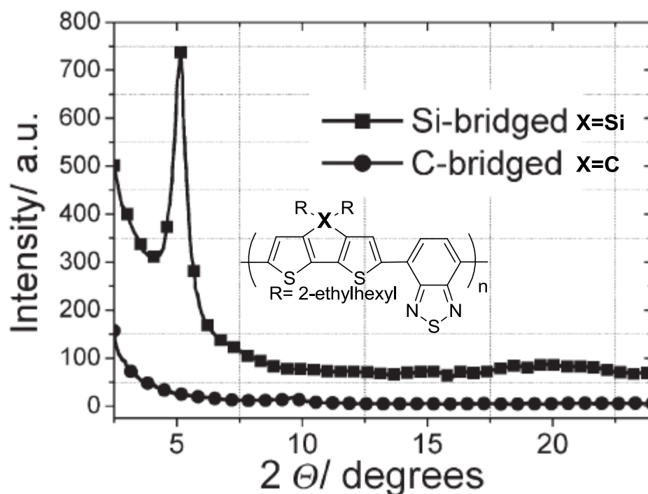
Figure 4-3. X-ray diffractograms of donor acceptor polymers of cyclopentadihiophene and dithiensilole. (Adapted with permission from Brabec.)
