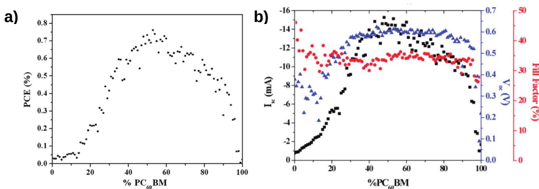
Figure 3-4. Performance of PGreen3 in large area solar cells. a) PCE optimization in 4.2 cm 2 solar cells as a function of PCBM content in the active layer blend. b) The variation of short circuit current ( I_{sc} ), open circuit voltage ( V_{oc} ) and FF (%) as a function of PCBM content. (Adapted with permission from Reynolds, Copyright 2012 American Chemical Society)
