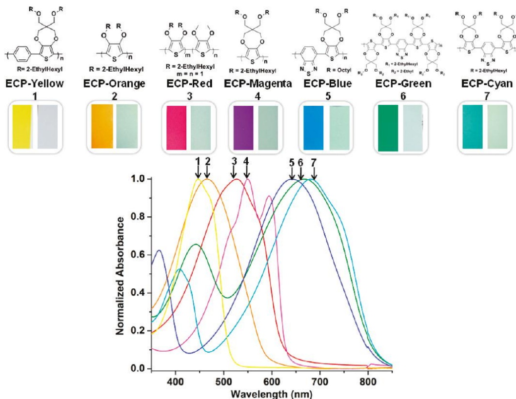
Figure 1-4. Colors obtained from 3,4- dioxothiophene based polymers along with their normalized absorption spectra. (Adapted with permission from Reynolds)
