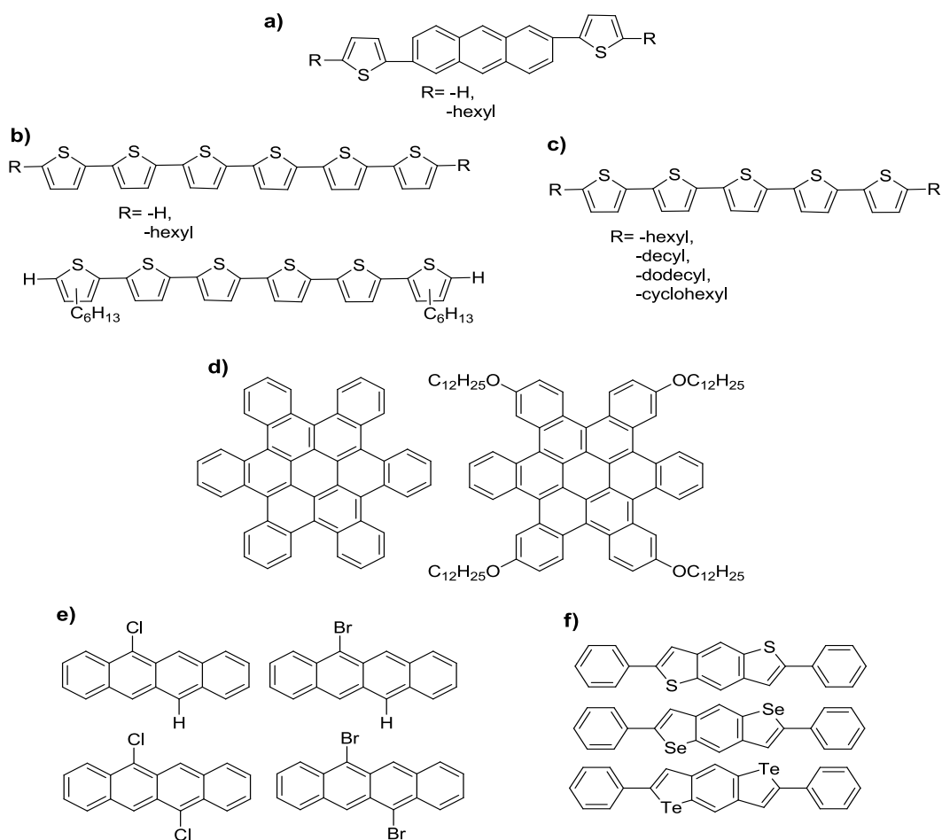
Figure 1-6. Examples of chemical modifications to study the molecular order. a-c) Alkyl chain substitution. d) Alkoxy substitution. e) Halogen atom substitution. f) Heavy atom substitution.
