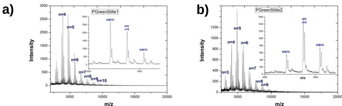
Figure 3-7. MALDI-MS of PGreenStille polymers. a) PGreenStille1 and b) PGreenStille2
