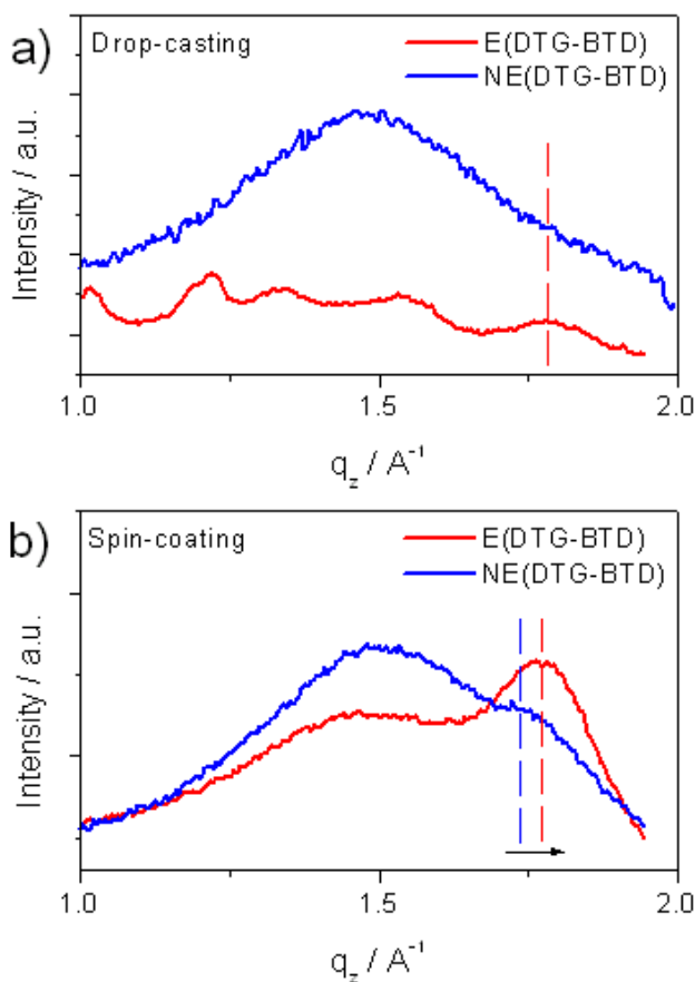
Figure 5-10. GIWAXS integrations of the wide-angle scattering region along q_z at q_{x,y} = 0 for E(DTG-BTD) and NE(DTG-BTD) a) after drop-casting and b) spin-coating. The dashed lines mark the position of the \pi -stacking peak maximum for E(DTG-BTD) (red) and NE(DTG-BTD) (blue). The arrow in b) indicates the shift of the \pi -stacking distance from 0.360 nm for NE(DTG-BTD) to 0.355 nm for E(DTG-BTD).
