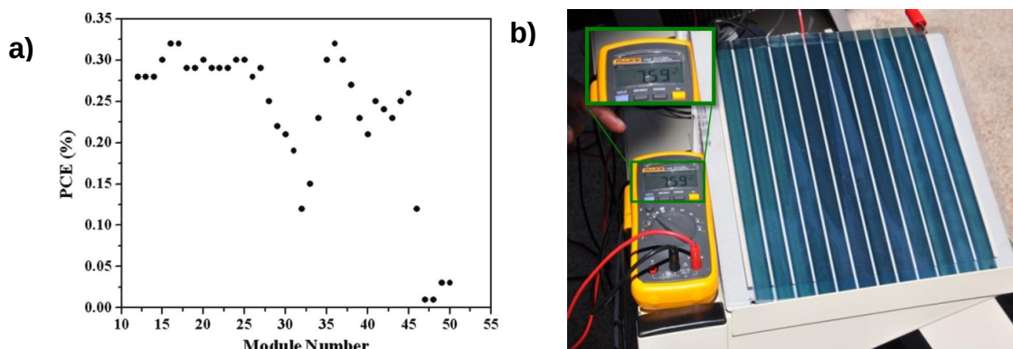
Figure 3-5. The performance of large scale processed blue-green cells. a) PCEs measured for each module. b) One of the slot die coated, inverted solar cell module in a Florida day sunshine. (Adapted with permission from Reynolds, Copyright 2012 American Chemical Society)
