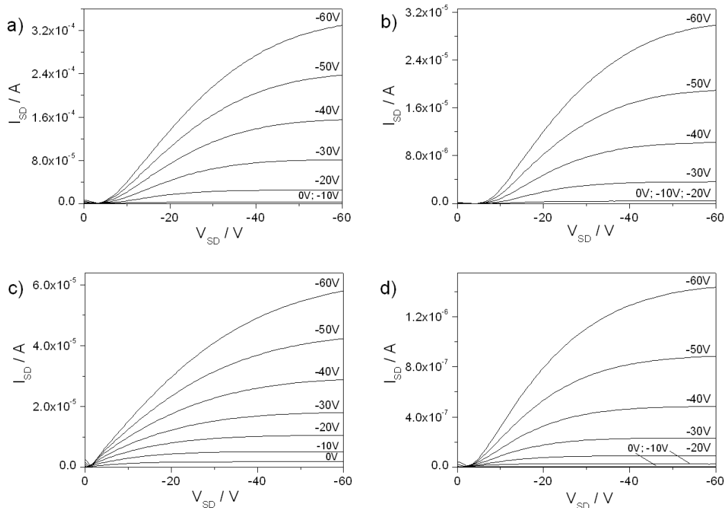
Figure 5-8. Transistor output curves for drop-cast and spin-coated a) and c) E(DTG-BTD), b) and d) NE(DTG-BTD) thin films.
