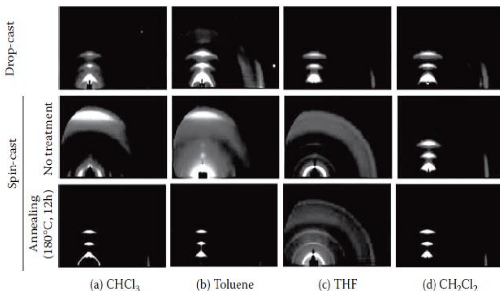
Figure 1-14. Two dimensional grazing incidence X-ray diffraction patterns for Poly(3-octylthiophene) processed from drop casting and spin coating from different solvents. (Adapted with permission from Locklin)
