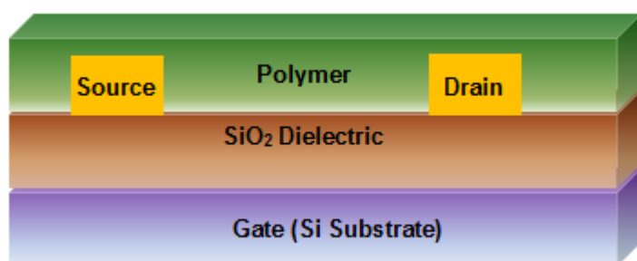
Figure 4-14. Bottom gate-bottom contact OFET architecture for charge transport measurements of the DTG and DTS polymers.
