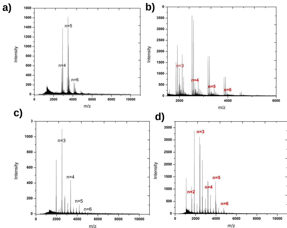
Figure 4-9. MALDI-MS of donor-acceptor polymers a) PGe12-BTD, b) PSi12-BTD, c) PG12-TPD and d) PSi12-TPD recorded using DCTB as matrix.
