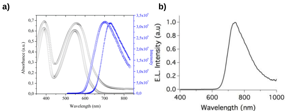
Figure 3-11. Absorption and emission characteristics for APFO-DOT. a) Absorption (in solution: circles, in film: triangles) and emission (in solution: diamond, in film: crosses) spectra of APFO-DOT. b) Electroluminescence spectrum of a PLED based on APFO-DOT at 12 V applied bias. (Adapted with permission from Reynolds, Copyright 2011 Royal Chemical Society)
