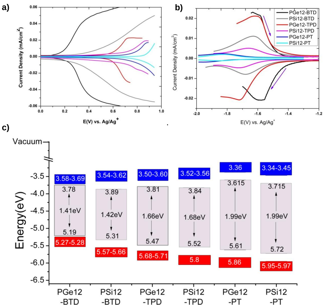
Figure 4-11. Electrochemical characterization of DTS and DTG polymers. a) Differential pulse voltammetry ((step size 2mV, step time 38 ms, pulse amplitude 100 mV) for thin films of PGe12-BTD (black), PSi12-BTD (gray), PGe12-TPD (red), PSi12-TPD (magenta), PGe12-PT (blue) and PSi12-PT (cyan) under a) positive voltage bias b) negative voltage bias c) The range of HOMO-LUMO energy levels estimated by CV and DPV measurements for the DTG&DTS series. The optically estimated band gaps of each polymer are placed at the center of the DPV estimated band gaps and a second approximated HOMO and LUMO levels are defined assuming the energy levels are equidistant from the center. These are highlighted in gray rectangle areas.
