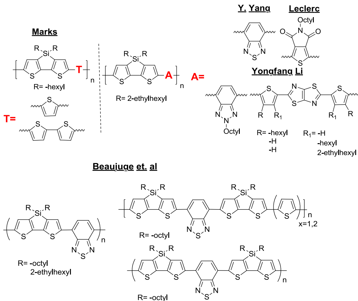
Figure 4-2. Copolymers based on dithienosilole and their chemical compositions.
