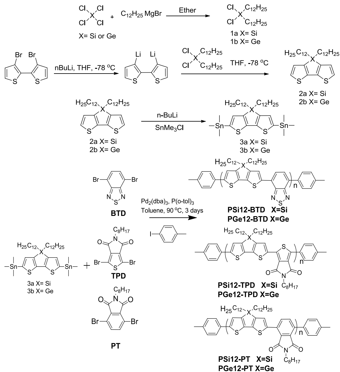
Figure 4-7. Schemes for the synthesis of n-dodecyl functionalized dithienosilole and dithienorgermole monomers and the six donor acceptor type polymers.
