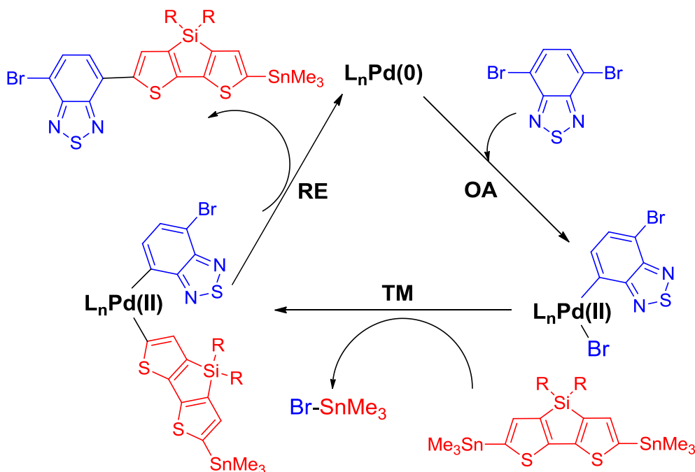
Figure 1-11. Catalytic cycle scheme as in Stille coupling.
