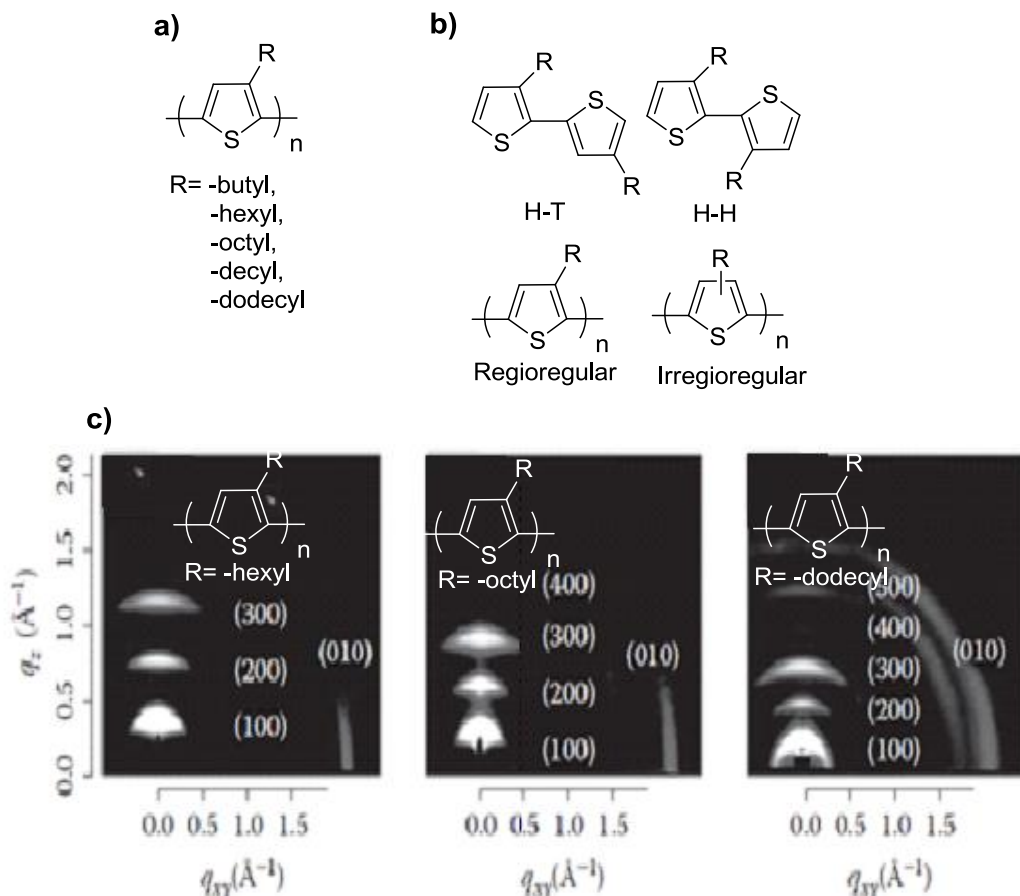
Figure 1-7. Control of molecular order in poly(3-alkylthiophenes). a) Poly(3-alkylthiophenes) functionalized with different length alkyl chains. b) Regioregular and irregular poly(3-alkylthiophenes) obtained from H-T and H-H couplings. c) Drop cast two dimensional grazing incidence X-ray diffraction patterns for drop cast poly(3-hexylthiophenes), poly(3-octylthiophenes) and poly(3-dodecylthiophenes). (Adapted with permission from Locklin)
