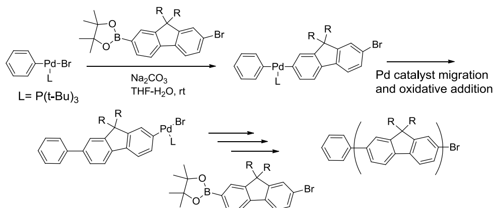
Figure 1-12. Proposed mechanism on the chain-growth Suzuki polymerizations.
