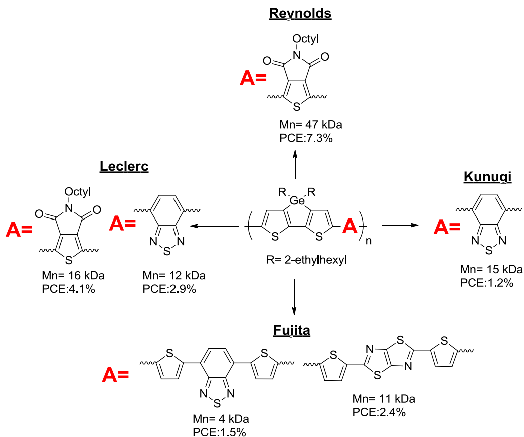
Figure 4-4. Dithiogermylene based donor-acceptor copolymers reported in 2011.
