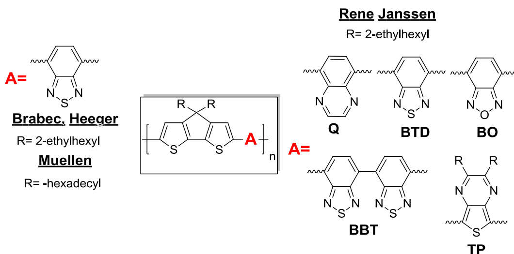
Figure 4-1. Various cyclopentadithiophene based copolymers and their chemical composition.
