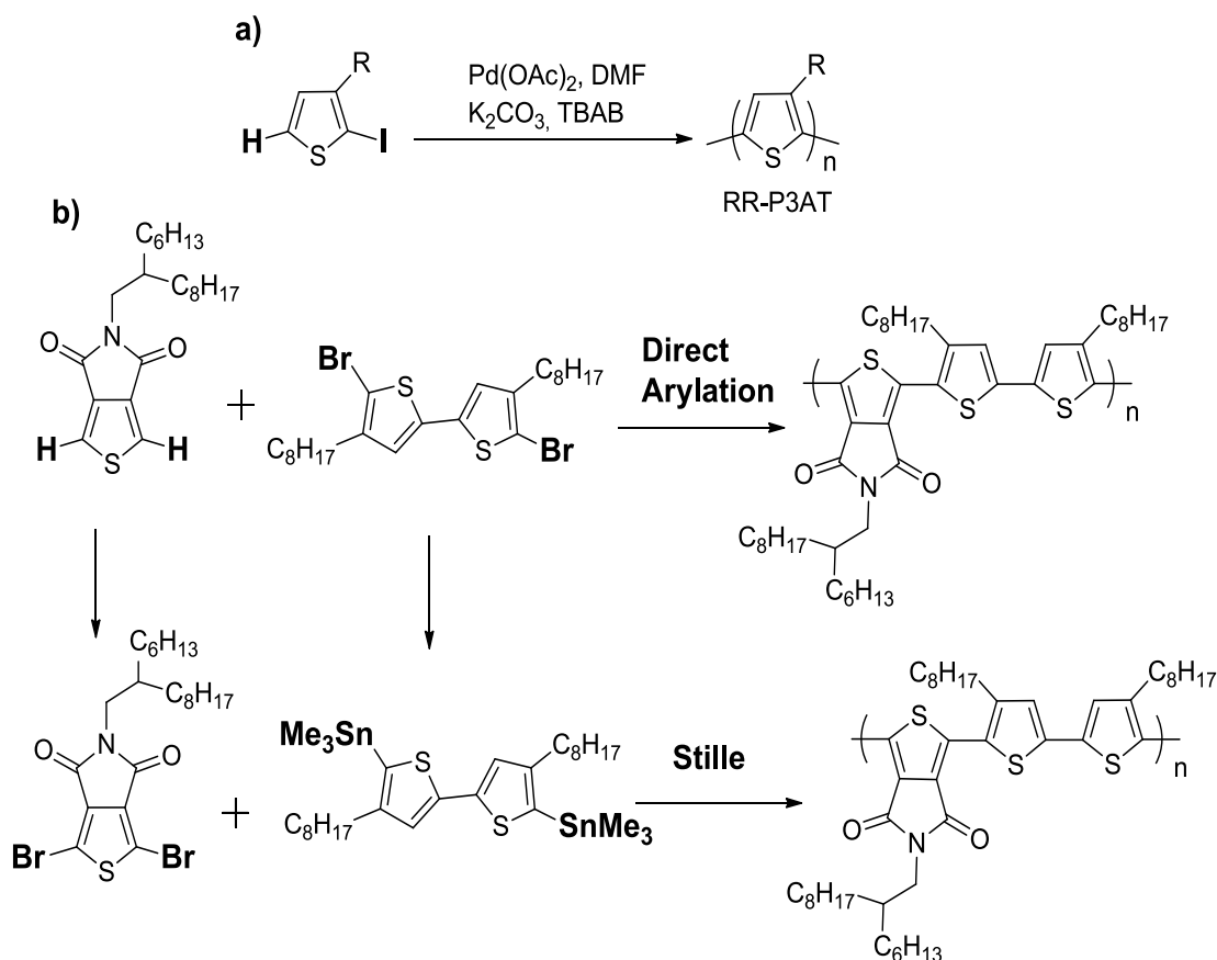
Figure 1-13. Direct arylation method for the synthesis of conjugated polymers.a) Direct arylation synthesis of poly(3-alkylthiophenes) b) Comparison of direct arylation and Stille polycondensation for generating the same thienopyrroledione based polymer.
