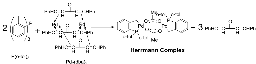
Figure 1-10. Formation of Herrmann complex with \text{Pd}_2(\text{dba})_3:\text{P(o-tol)}_3 catalyst system.
