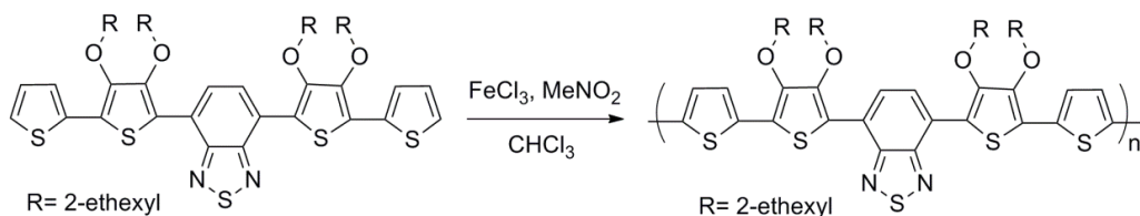
Figure 3-2. Synthesis of PGreen via oxidative polymerization.
