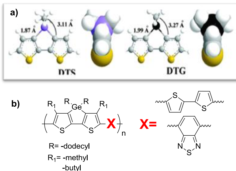
Figure 4-5. The literature examples studied the C-Ge bond lengths. a) Comparison of theoretical model structures dithienosilole and dithienogermole aromatic units. (Adapted with permission from Reynolds) b) Peripherally alkylated dithienogermole based copolymers.
