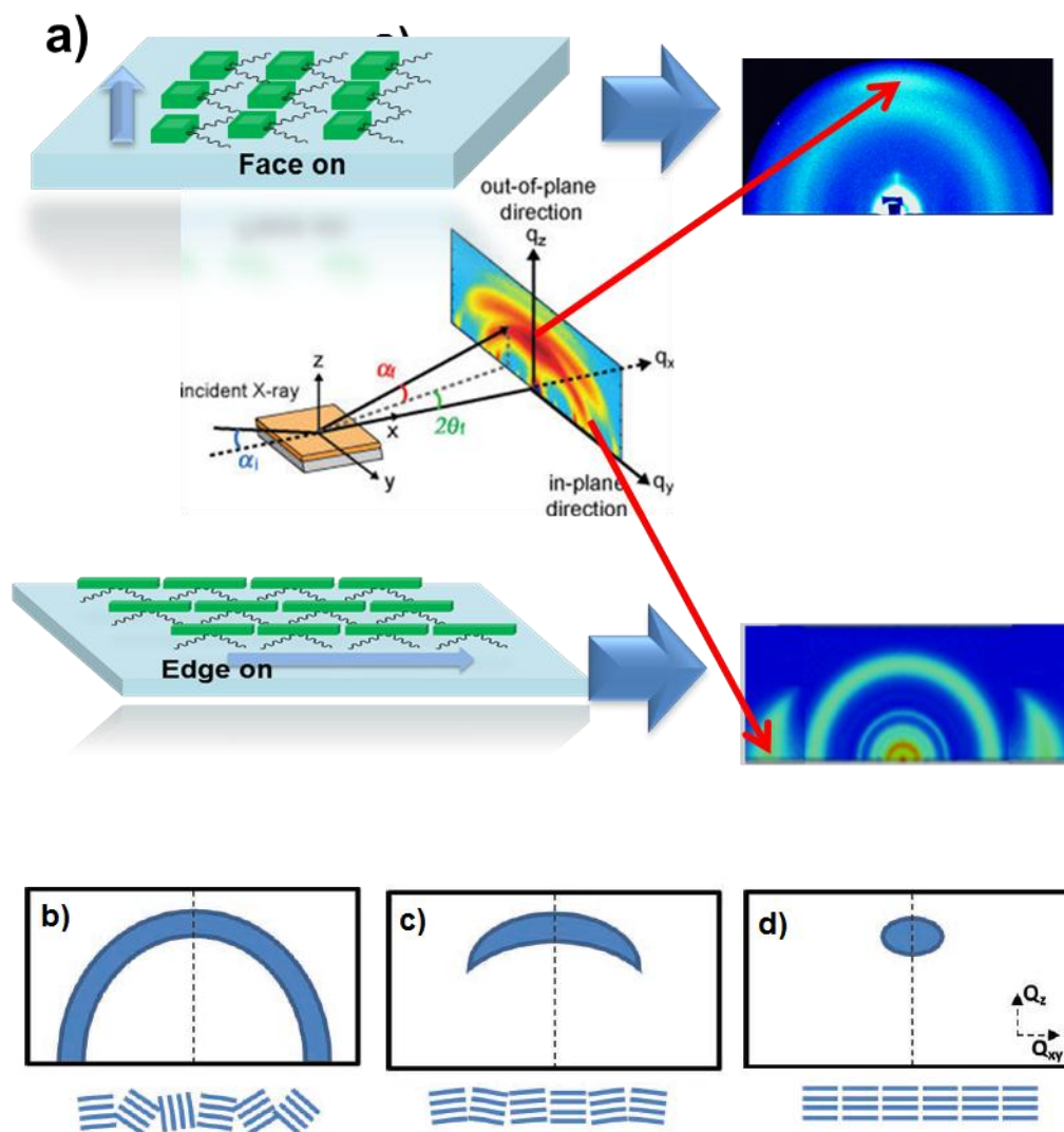
Figure 2-4. Analysis of GIWAXS patterns. a) Representation of the GIWAXS experiment and cartoons showing the X-ray pattern for face on and edge on arrangement on the substrate. b-d) The intensity and the shape of the arc at the q_z direction with the cartoons of representative ordering in the polymer chains.
