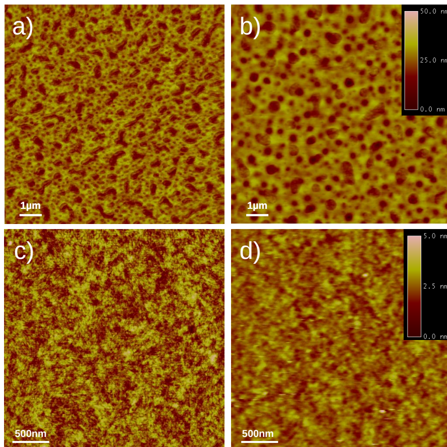
Figure 5-11. Tapping mode AFM height images of drop-cast and spin-coated a) and c) E(DTG-BTD), b) and d) NE(DTG-BTD). Height scale is identical for each processing methods.
