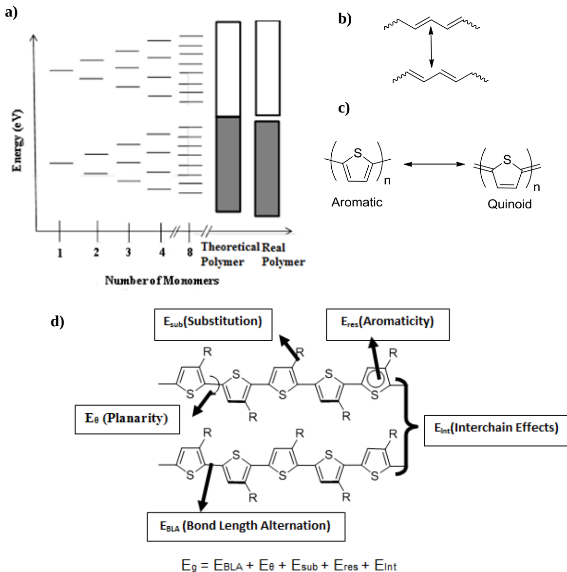
Figure 1-1. The concept of band gap as in conjugated polymers. a) Formation of bands in a conjugated polymer. b) Resonance forms of poly(acetylene). c) Aromatic and quinoid resonance structures for polythiophene. d) The structural factors affecting the energy of the band gap in an alkylated polythiophene. (Adapted and modified with permission from Roncali)
