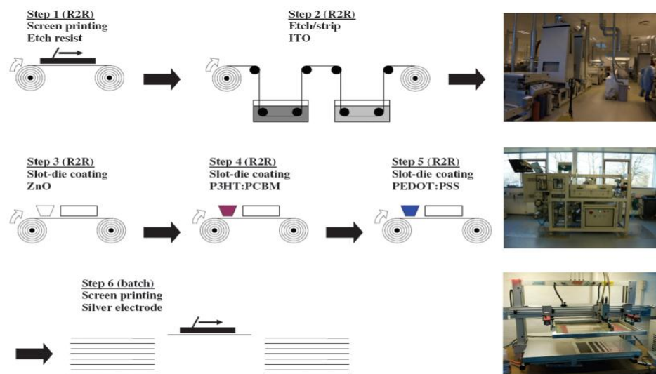
Figure 1-15. Illustration of six fabrication steps of deposition of organic solar cells components via roll-to-roll process. (Adapted with permission from Krebs)
