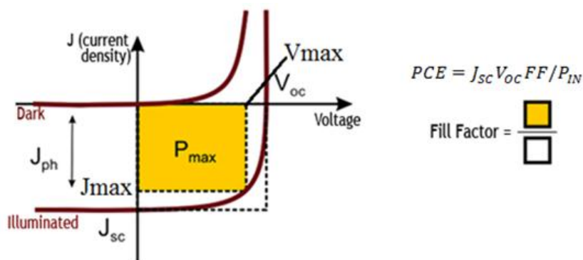
Figure 1-18. Representative J-V curve obtained from an organic solar cell and the evaluation of important parameters from the curve.
