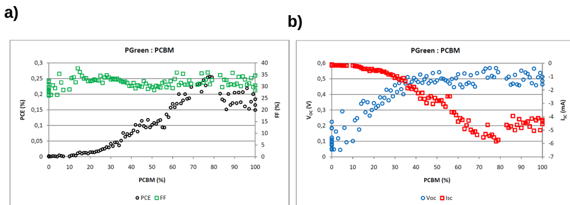
Figure 3-8. Performance of PGreenStille polymer in large area solar cells. a) PCE optimization and FF (%) results in 4.2 cm 2 solar cells as a function of PCBM content in the active layer blend. b) The variation of short circuit current ( I_{SC} ) and open circuit voltage ( V_{OC} ) as a function of PCBM content.
