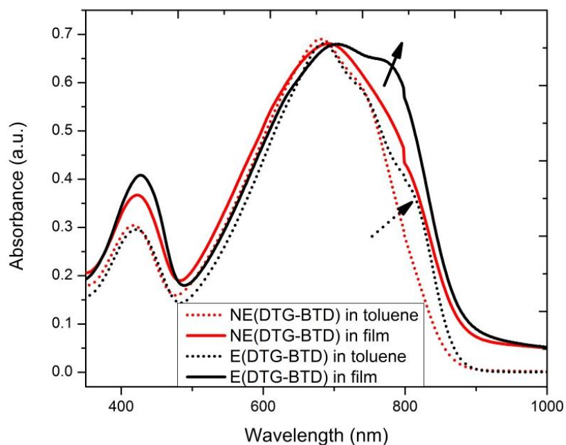
Figure 5-6. Absorption spectra for dilute solutions of E(DTG-BTD) and NE(DTG-BTD) in toluene and for thin film. Arrows highlight the aggregation bands.
