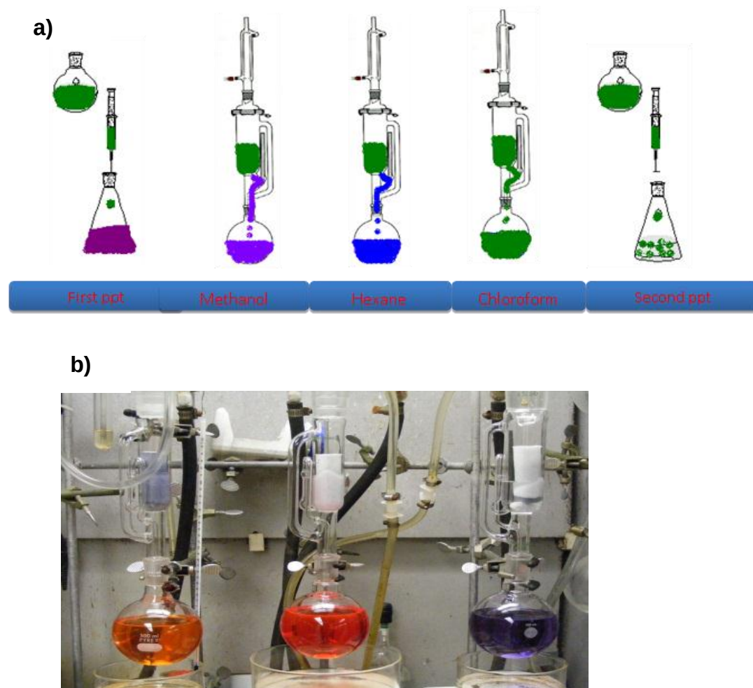
Figure 2-2. Demonstration of soxhlet extraction process. a) Soxhlet extraction sequence b) Different colors of washings for the low molecular weight polymers
