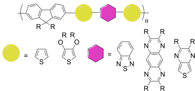
Figure 3-9. Chemical composition of APFO copolymers with different donor and acceptor units employed in the repeat unit structure. (Adapted with permission from Reynolds, Copyright 2011 Royal Chemical Society)
