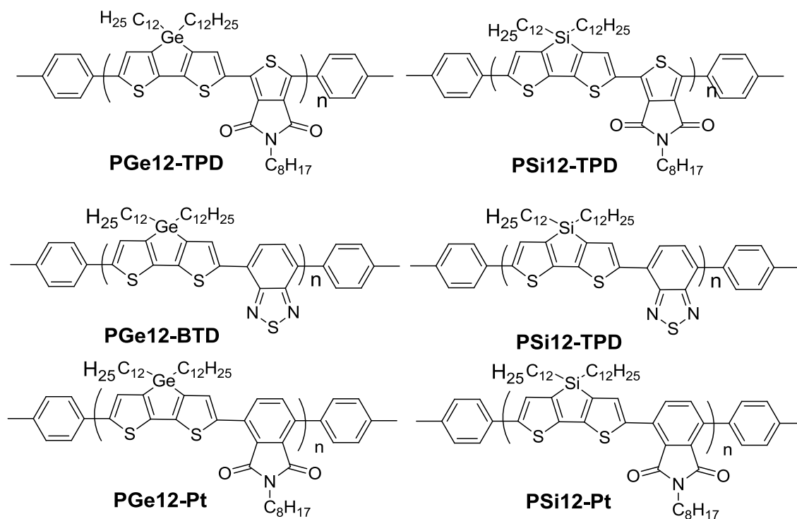
Figure 4-6. Repeat unit structures for the discussed n-dodecyl functionalized dithienogermole and dithienosilole based donor acceptor copolymers in Chapter 4.
