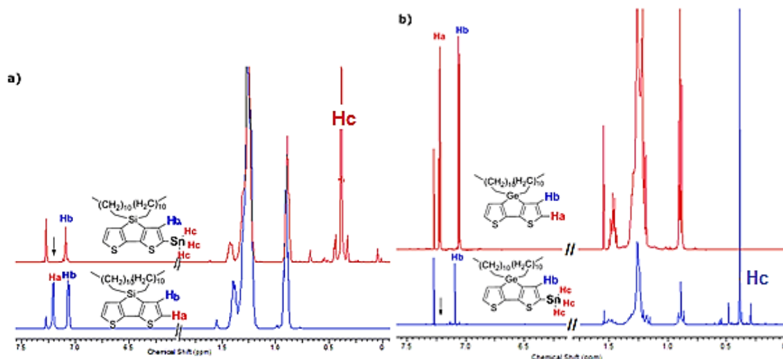
Figure 4-8. Comparison of ^1\text{H} -NMR spectra of the distannylated monomers and their precursors. a) dithienosilole and distannylated dithienosilole, b) dithienogermole and distannylated dithienogermole. Black arrows show the absence of Ha protons.
