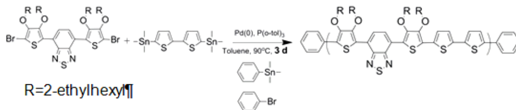
Figure 3-6. PGreen synthesis through Stille polycondensation.
