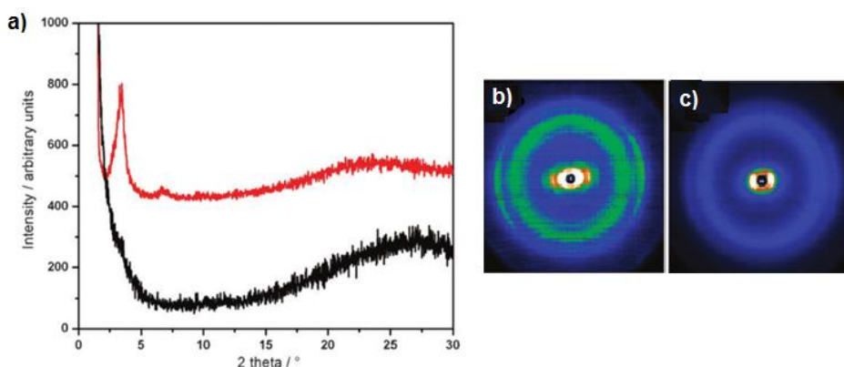
Figure 1-9. X-ray analyses of PCPDT-BTD for different molecular weights. a) X-ray diffraction pattern for high molecular weight (56 kDa) PCPDT-BTD (red line) and low molecular weight (13 kDa) PCPDT-BTD (black line). Two dimensional wide angle X-ray scattering patterns for b) high molecular weight (65 kDa) PCPDT-BTD c) low molecular weight (13 kDa) PCPDT-BTD. (Adapted with permission from Muellen)
