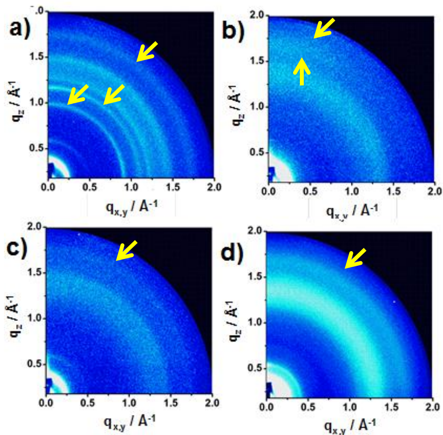
Figure 4-13. GIWAXS patterns recorded for thin films of DTS and DTG polymers. a) PGe12-BTD, b) PGe12-TPD c) PSi12-BTD and d) PSi12-TPD. Yellow arrows highlight the important reflections due to molecular organization.
