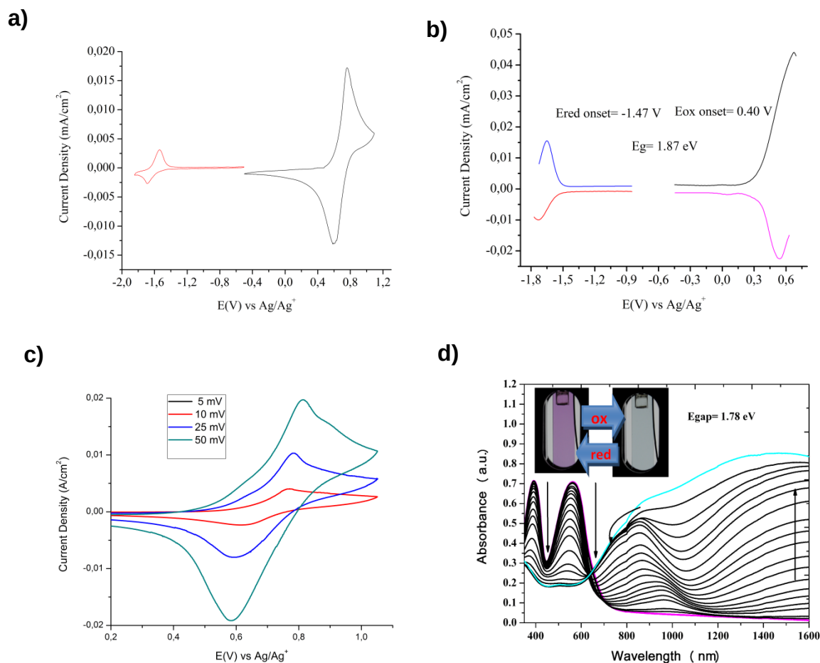
Figure 3-13. Electrochemical characterization of APFO-DOT. a) Cyclic voltammetry of APFO-DOT in 0.1 TBAPF6/PC with a 50 mV/s scan rate. b) Differential Pulse Voltammetry of APFO-DOT in 0.1 TBAPF6/PC. c) Scan Rate Dependant Cyclic Voltammetry of APFO-DOT in 0.1 TBAPF6/PC. d) The spectroelectrochemistry of APFO-DOT films coated on ITO glass in 0.2 M LiBTI/PC supporting electrolyte between -0.5 V and 0.82 V versus \text{Ag}/\text{Ag}^+ reference electrode. Inset shows photographs of neutral and oxidized states. (Adapted with permission from Reynolds, Copyright 2011 Royal Chemical Society)
