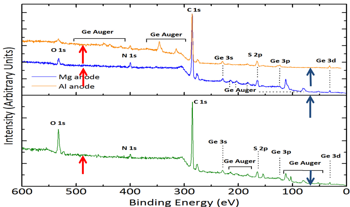
Figure 5-5. XPS spectra of NE(DTG-BTD) with two different X-ray sources of Mg and Al and E(DTG-BTD) with Mg source. The expected Br 3d and Sn 3d 5/2 orbital energies are highlighted as blue and red arrows respectively.
