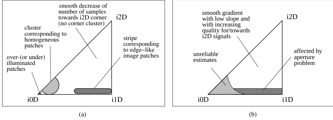
Figure 3.1: a) Schematic representation of the distribution of local image patches in natural images according to their intrinsic dimension. b) Schematic representation of the quality of optic flow estimation according to the intrinsic dimension of the underlying signal.
