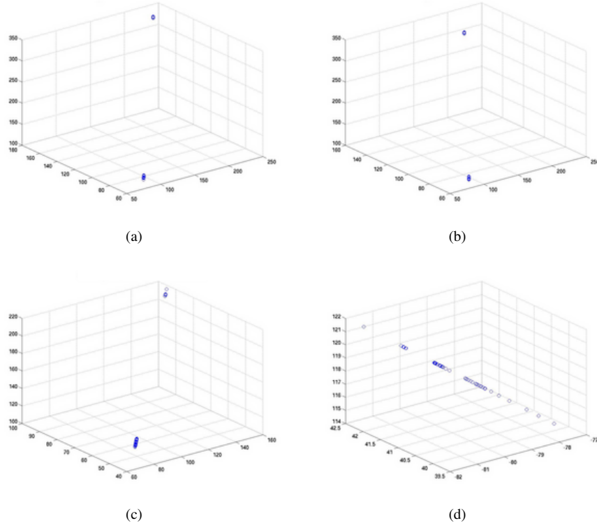
Figure 7.10: The distribution of the votes for a few monos shown in the 3D Euclidean space. Sub-figures (a)-(c) are clear examples where there are two clusters. However, such clear clusters do not always exist (d).
