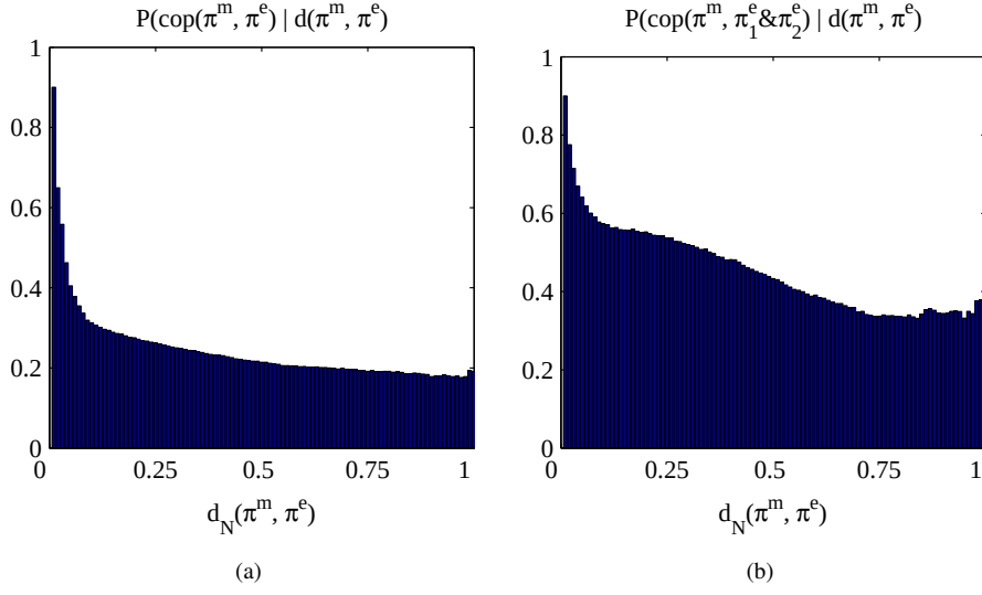
Figure 6.7: Likelihoods from figures 6.6(a) and 6.6(b) with a more strict coplanarity relation (namely, we set the thresholds T_p and T_d to 10 degrees and 0.2, respectively. See Appendix for more information about these thresholds). (a) Figure 6.6(a) with more strict coplanarity relation. (b) Figure 6.6(b) with more strict coplanarity relation.
