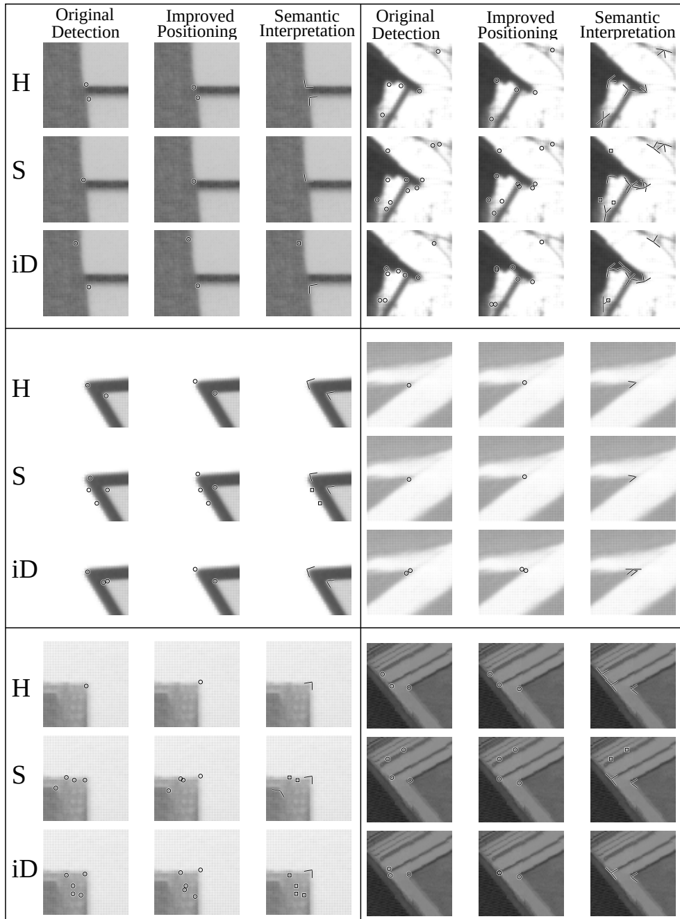
Figure 4.5: A set of example junctions and the results of junction detectors and the results of IC and SI on these results. For each example, S, H and iD denote SUSAN, Harris and iD respectively. In each example, the first column shows the original detections of the algorithms; the second column shows the effect of improved positioning via IC ; and, the third column shows the estimated SI and how it can be used to get rid of spurious junctions. Spurious junctions that are estimated with SI are marked in small squares.
