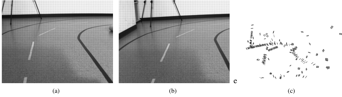
Figure 7.1: (a-b) An input stereo pair. (c) Results of a feature-based stereo algorithm taken from [Pugeault and Krüger, 2003]. This is a view from our 3D displaying software which shows the 3D edge features as rectangles for the sake of simplicity. Note that stereo information can contain outliers.
