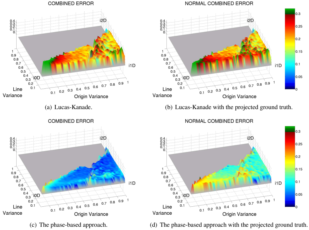
Figure 3.9: Qualities of the optic flow algorithms depending on iD. Left column shows the errors between computed flow and the ground truth. Right column shows the errors between computed flow and the ground truth projected orthogonal to the orientation of signals. Color bars show the error values for corresponding colors of corresponding graphs. (a,b) The Lucas-Kanade. (c,d) The phase-based approach.
