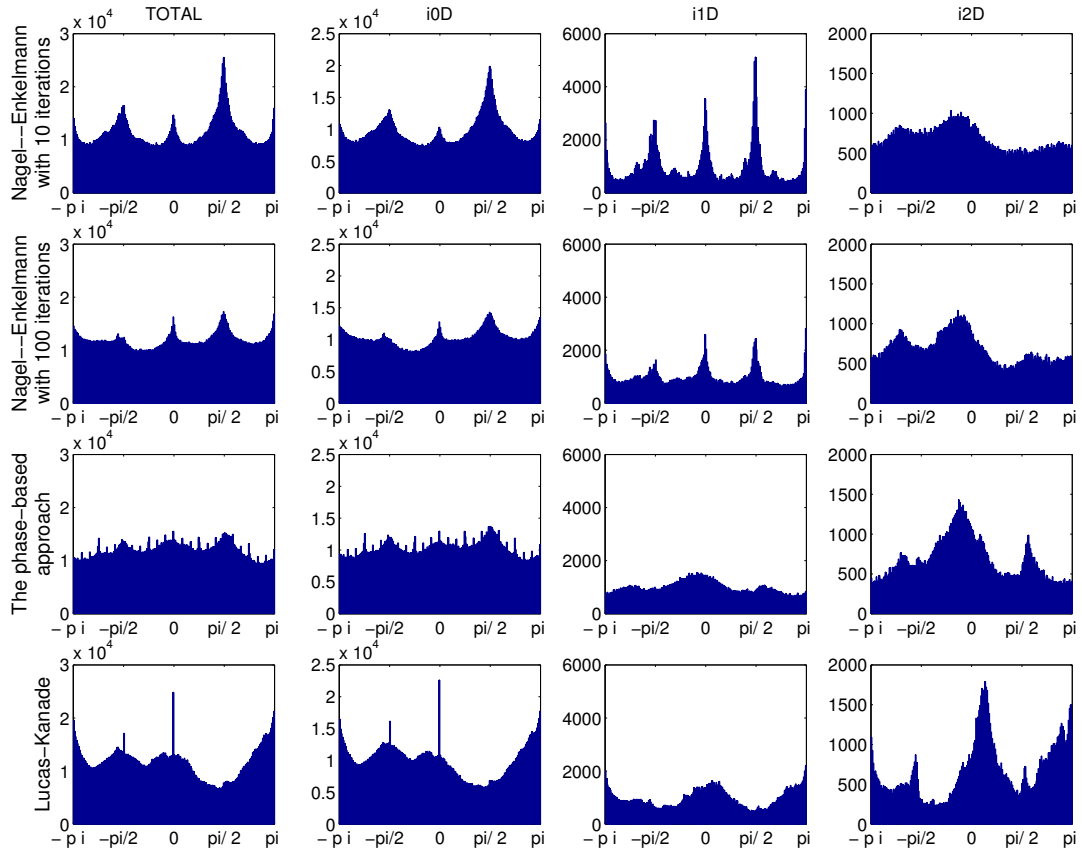
Figure 3.6: Distribution of direction of optic flow vectors depending on the intrinsic dimension. The histograms show the summed up distributions over the sequences which are introduced in section 3.1. From top to bottom: The Nagel-Enkelmann algorithm with 10 iterations; The Nagel-Enkelmann algorithm with 100 iterations; The phase-based approach; The Lucas-Kanade algorithm. From left to right: The total distribution; The distribution for i0D signals; The distribution for i1D signals; The distribution for i2D signals.
