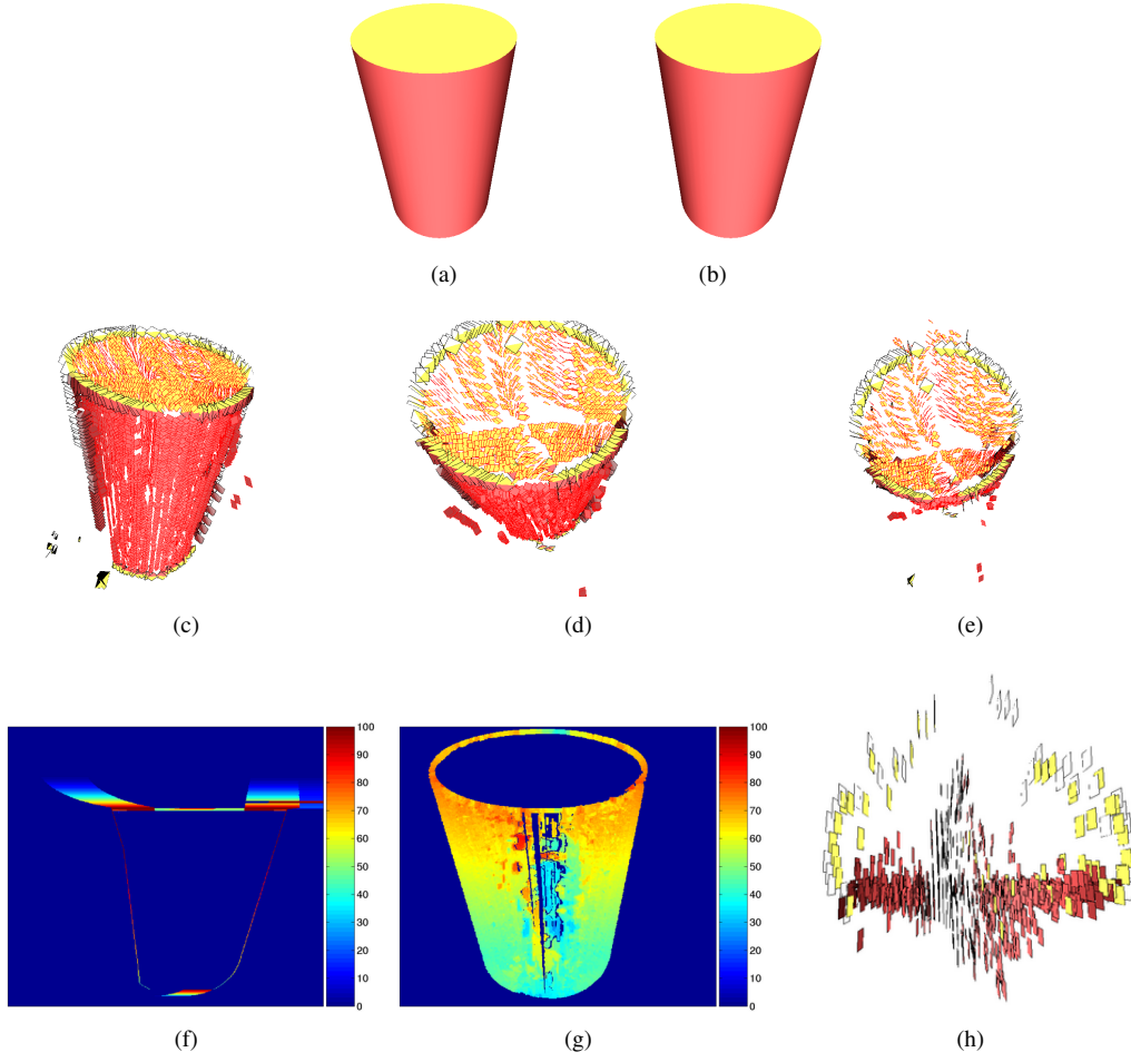
Figure 7.17: Experiment results on a cylinder. (a,b) Input stereo pair. (c-e) The predictions of our model shown as snapshots from our 3D displaying software. As surface fitting for curved surfaces in case of outliers is not trivial, we are unable to provide disparity maps for our results. (f) Disparity map from DP. (g) Disparity map from PB. (h) Top view of the results of PB.
