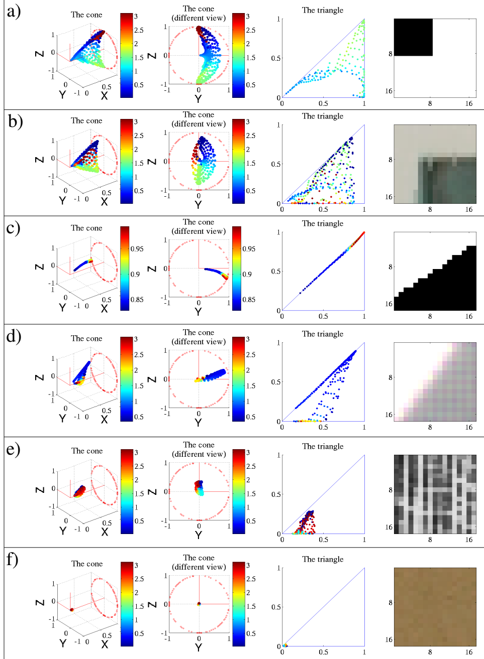
Figure A.2: Illustration of how the points in some image patches taken from real scenes map to the triangle and the cone. The patches are illustrated in the right-most column. The color of the points inside the triangle and the cone encode different orientations, whose values can be accessed using the color-bars.
