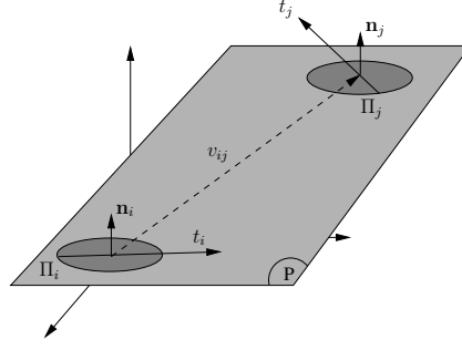
Figure 7.4: Co-planarity of two 3D primitives \Pi_i^e and \Pi_j^e .
