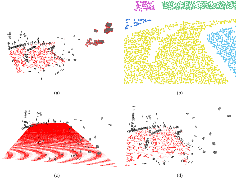
Figure 7.11: (a) The predictions on the surface of the road for the input images shown in figure 7.1 (predictions are marked with red boundaries). The predictions are scattered around the plane of the road, and there are wrong predictions due to possible outliers in the computed stereo. The figure is a snapshot from our 3D displaying software. (b) Segmentation of one of the input images given in figure 7.1 into areas using region-growing based on primitives. (c) The surface extracted from the predictions shown in (a). (d) The predictions from (a) that are corrected using the extracted surface shown in sub-figure (c).
