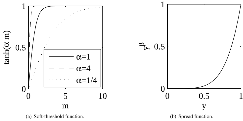
Figure A.3: (a) Function s_1(m) = \tanh(\alpha m) for soft-thresholding the magnitude with different values of \alpha . (b) Spread function, y^\beta for \beta = 5 .
