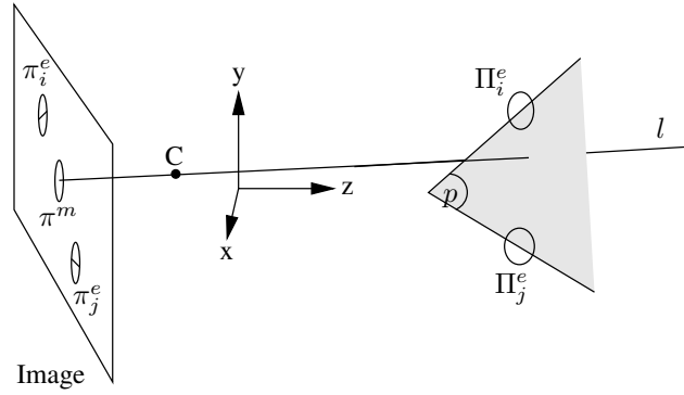
Figure 7.9: Illustration of how the vote of a pair of edge primitives is computed. The 3D primitives \Pi_i^e and \Pi_j^e corresponding to the 2D primitives \pi_i^e and \pi_j^e define the plane p . The intersection of p with the ray l that goes through the 2D mono \pi^m and the camera center C then determines the position of the estimated 3D mono \Pi^m . The 3D orientation of \Pi^m is set to be the orientation of the plane p .
