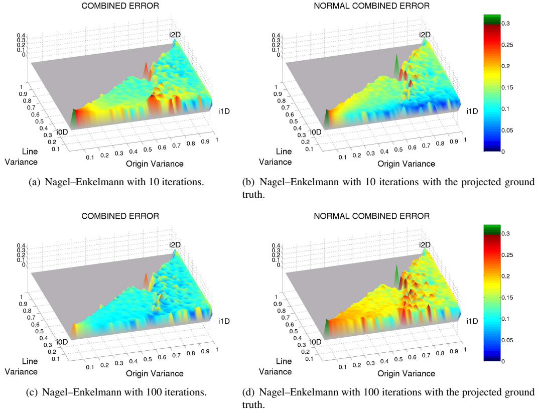
Figure 3.8: Qualities of the optic flow algorithms depending on iD. Left column shows the errors between computed flow and the ground truth. Right column shows the errors between computed flow and the ground truth projected orthogonal to the orientation of signals. Color bars show the error values for corresponding colors of corresponding graphs. (a,b) Nagel-Enkelmann with 10 iterations. (c,d) Nagel-Enkelmann with 100 iterations.
