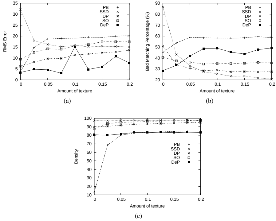
Figure 7.19: Performance of the different algorithms on the artificial scene in figure 7.18 for different amount of texture using RMS (a), BMP (b) measures. The densities are shown in (c).
