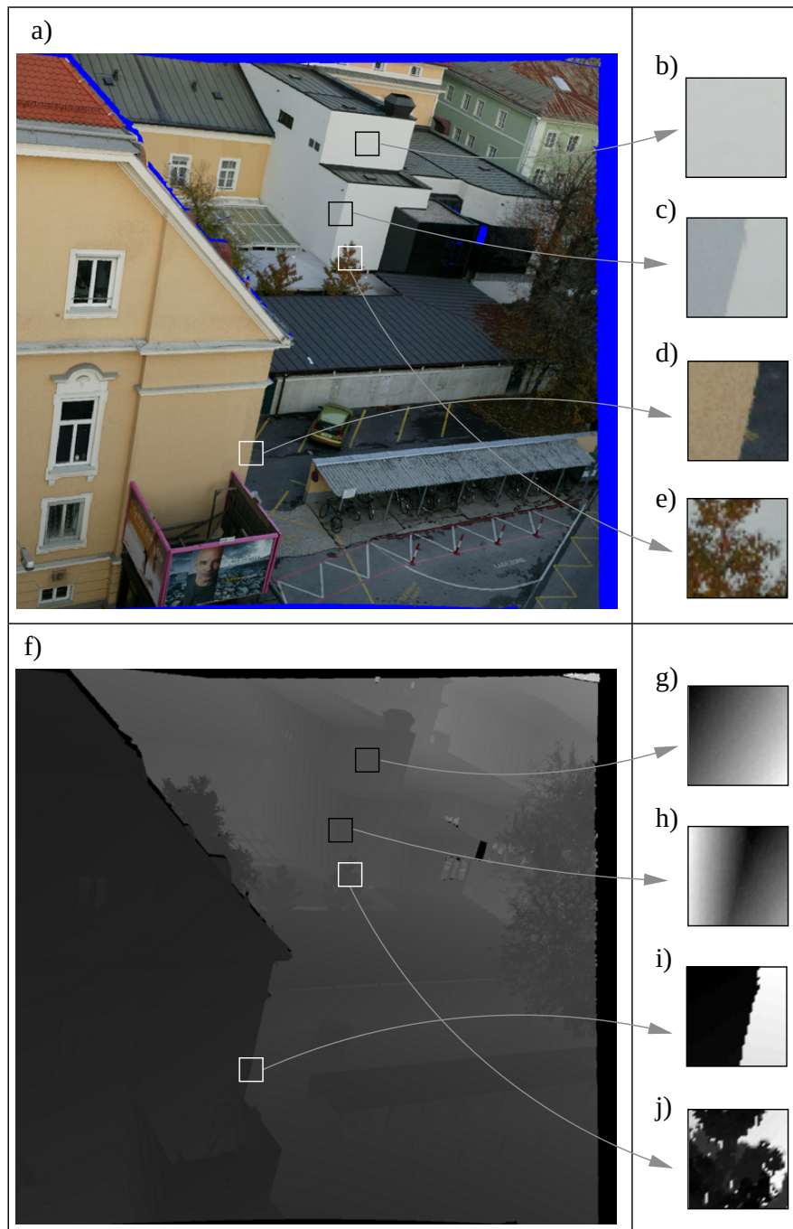
Figure 5.1: Illustration of the types of 3D discontinuities. (a) 2D image. (b) Continuity. (c) Orientation discontinuity. (d) Gap discontinuity. (e) Irregular gap discontinuity. (f)-(j) The range images corresponding to (a)-(e). Note that the range images are scaled independently for better visibility.
