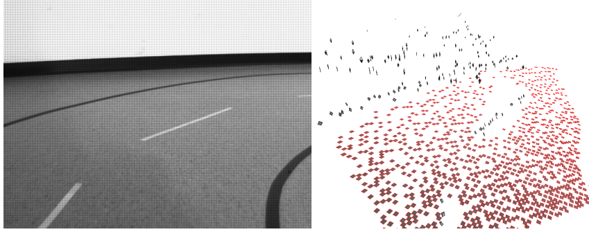
Figure 7.15: Experiment results on a lab road scene. Left: Left image of the input stereo pair. Right: The predictions of our model shown in our 3D displaying software.
