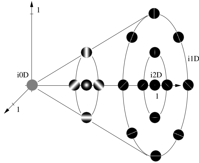
Figure A.1: The cone constructed from the magnitude and the orientation of signals. Taken from [Felsberg et al., 2007a].
