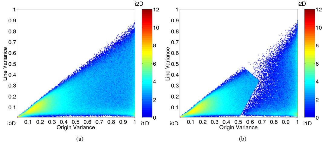
Figure 3.2: Logarithmic plot of the distribution of intrinsic dimensionality. (a) The distribution for regularly sampled points. (b) The distribution when the positions are modified according to iD (See the text for details of this modification).
