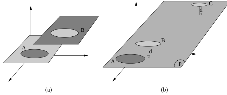
Figure C.1: Criteria for coplanarity of two planes. (a) According to the angular-difference criterion of coplanarity, entities A and B will be measured as coplanar although they are on different planes. In (b), P is the plane defined by entity A. According to the distance-based coplanarity definition, entities B and C have the same measure of coplanarity. However, entity C which is more distant to entity A should have a higher measure of coplanarity than entity B although they have the same distance to plane P (see the text).
