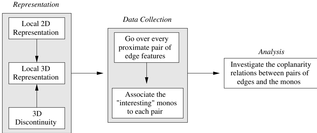
Figure 6.2: Overview of the analysis process. First, local 2D and 3D representations of the scene are extracted from the chromatic range data. Second, a data set is constructed out of each pair of edge features, associating the monos that are likely to be coplanar ( i.e. , "interesting") to them (see section 6.1.2 for what is meant by relevance). Third, the coplanarity between the monos and the edge features that they are associated to are investigated.
