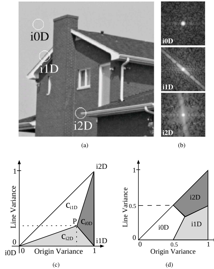
Figure 2.1: Illustration of iD (Sub-figures (a,b) are taken from [Felsberg and Krüger, 2003]). (a) Three image patches for three different intrinsic dimensions. (b) The 2D spatial frequency spectra of the local patches in (a), from top to bottom: i0D , i1D , i2D . (c) The topology of iD . Origin variance is variance from a point, i.e., the origin. Line variance is variance from a line, measuring the junctionness of the signal. c_{iND} for N = 0, 1, 2 stands for confidence for being i0D , i1D and i2D , respectively. Confidences for an arbitrary point P is shown in the figure which reflect the areas of the sub-triangles defined by P and the corners of the triangle. (d) The decision areas for local image structures.
