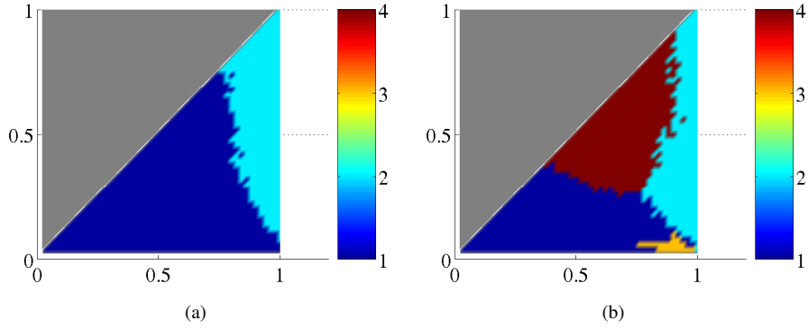
Figure 5.7: Maximum likelihood estimates of local 3D structures given local 2D structures. Numbers 1, 2, 3 and 4 represent continuity, gap discontinuity, orientation discontinuity and irregular gap discontinuity, respectively. (a) Raw maximum likelihood estimates. Note that the estimates are dominated by continuities and gap discontinuities. (b) Maximum likelihood estimates from normalized likelihood distributions: the triangles provided in figure 5.6 are normalized within themselves so that the maximum likelihood of P(X | 2D \text{ Structure}) is 1 for X being continuity, gap discontinuity, irregular gap discontinuity and orientation discontinuity.
