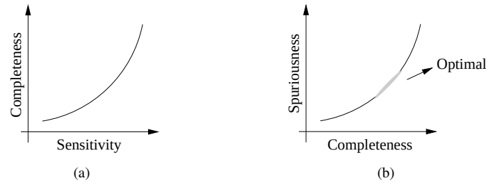
Figure 4.1: The relations between sensitivity, completeness and spuriousness.
