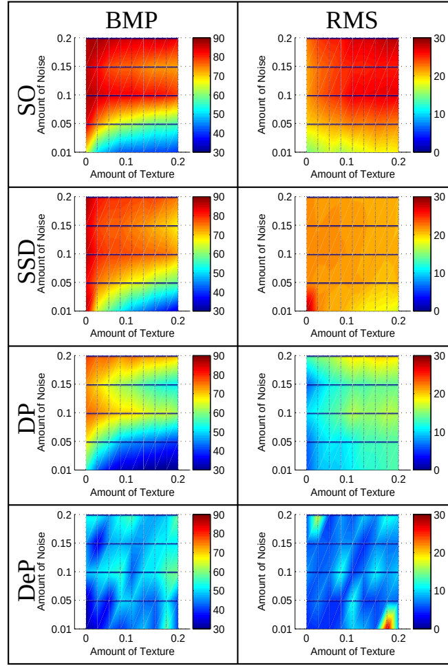
Figure 7.22: Performance of the different algorithms as a function of white noise and texture (white noise). Results of PB are skipped due to page limits.
