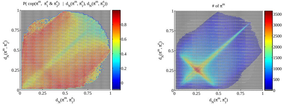
Figure 6.9: The likelihood of the coplanarity of a mono against the distance to \pi_1^e and \pi_2^e . Left-plot shows the likelihood distribution whereas right-plot shows the frequency distribution.
