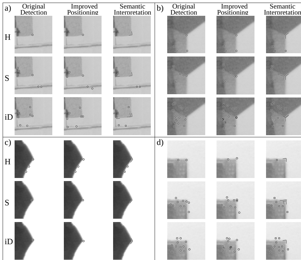
Figure 4.6: The effect of high 'sensitivity' on the performance of junction detectors. Junction detectors can now detect low contrast junctions that they miss with low sensitivity. H and S denote Harris and SUSAN respectively. For each subfigure, the first column shows original detection results, the second the results of improved positioning with IC and the third the SI . Spurious junctions that are estimated with SI are marked in small squares.
