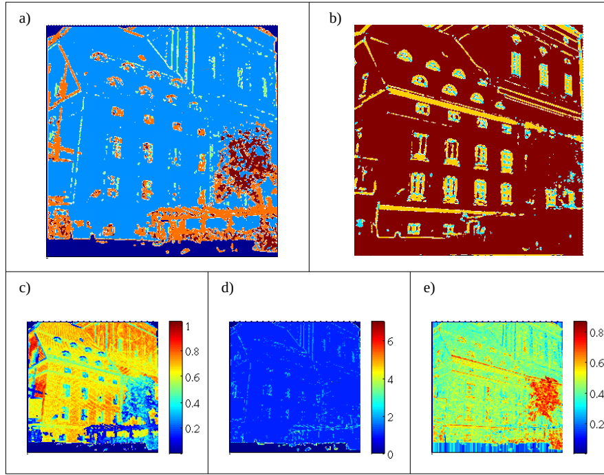
Figure 5.5: The 3D and 2D information for one of the scenes shown in figure 5.2. Dark blue marks the points without range data. (a) 3D discontinuity. Blue: continuous surfaces, light blue: orientation discontinuities, orange: gap discontinuities and brown: irregular gap discontinuities. (b) Intrinsic Dimensionality. Homogeneous patches, edge-like and corner-like structures are encoded in colors brown, yellow and light blue, respectively. (c) Gap discontinuity measure \mu_{GD} . (d) Orientation discontinuity measure \mu_{OD} . (e) Irregular gap discontinuity measure \mu_{IGD} .
