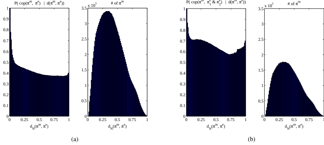
Figure 6.6: Likelihood distribution of coplanarity of monos. In each sub-figure, left-plot shows the likelihood distribution whereas right-plot shows the frequency distribution. (a) The likelihood of the coplanarity of a mono with \pi_1^e or \pi_2^e against the distance to \pi_1^e or \pi_2^e . This is the unconstrained case; i.e. , the case where there is no information about the coplanarity of \pi_1^e and \pi_2^e . (b) The likelihood of the coplanarity of a mono with \pi_1^e and \pi_2^e against the distance to \pi_1^e or \pi_2^e .
