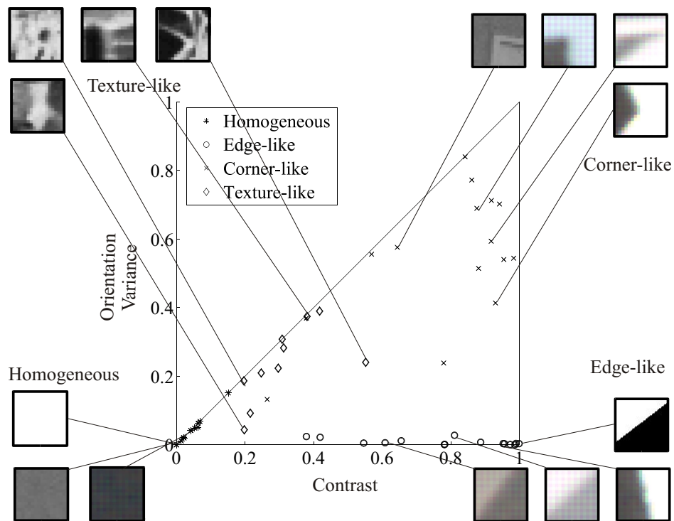
Figure 2.3: How a set of 54 patches map to the different areas of the intrinsic dimensionality triangle. Some examples from these patches are also shown. The horizontal and vertical axes of the triangle denote the contrast and the orientation variances of the image patches, respectively.
