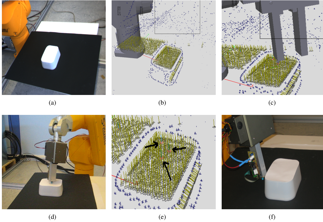
Figure 7.25: Surface Verification Experiment (taken from [Kjargaard et al., 2007]). (a) Setup of the scene. (b) View of the 3 predicted surfaces. (c) The robot moving in position to verify the surface on the box. (d) The sensor in contact with the surface on the box. (e) The 3 detected haptic primitives shown as small red squares. (f) The robot moving through the wrongly predicted surface without detecting a contact.
