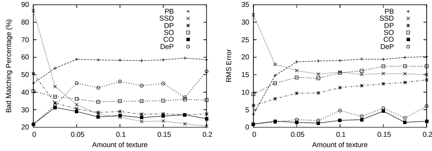
Figure 7.24: The results of combination (CO) with dense stereo (namely, DP) on the artificial data set from figure 7.18. (a) Bad matching performance. (b) RMS errors.
