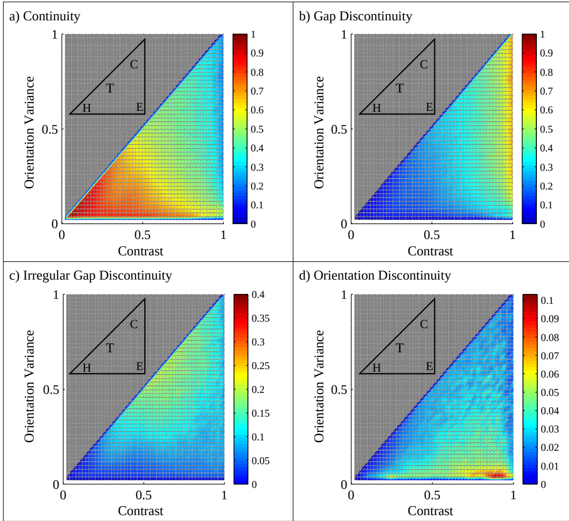
Figure 5.6: P(3D \text{ Discontinuity} | 2D \text{ Structure}) . The distribution of local image structures is schematized for easy reference in the upper-left part of each subfigure (the letters C, E, H, T represent corner-like, edge-like, homogeneous and texture-like structures). (a) P(\text{Continuity} | 2D \text{ Structure}) . (b) P(\text{Gap Discontinuity} | 2D \text{ Structure}) . (c) P(\text{Irregular Gap Discontinuity} | 2D \text{ Structure}) . (d) P(\text{Orientation Discontinuity} | 2D \text{ Structure}) .
