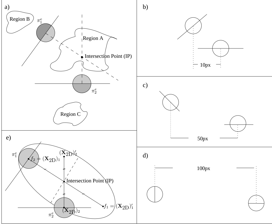
Figure 6.4: (a) Given a pair of edge features, coplanarity relation can be investigated for homogeneous image patches inside regions A, B and C. However, due to computational intractability reasons, this chapter is concerned in making the analysis only in region A (see the text for more details). (b)-(d) A few different configurations of edge features that might be encountered in the analysis. The difficult part of the investigation is to make these different configurations comparable, which can be achieved by fitting a shape (like square, rectangle, circle, parallelogram, ellipse) to these configurations. (e) The ellipse, among the alternative shapes ( i.e. , square, rectangle, circle, parallelogram) turns out to describe the different configurations shown in (b)-(d) better. For this reason, ellipse is for analyzing coplanarity relations in the rest of the chapter.
