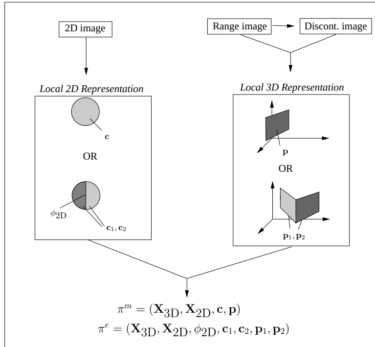
Figure 6.3: Illustration of the representation of a 3D entity. From the 2D and 3D information, local 2D and 3D representation is extracted.
