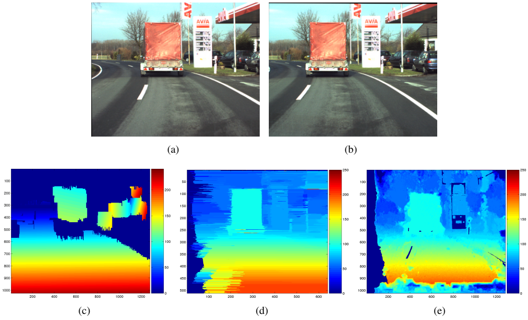
Figure 7.16: Experiment results on a road scene. (a,b) Input stereo pair. (c) The predictions of our model as a disparity map. (d) Disparity map from DP. (e) Disparity map from PB.
