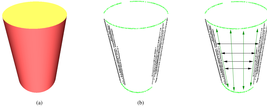
Figure 7.13: Detected curved groups (b) which are extracted from (a). The edges of a curved group are shown in green. There are several 'layers' of groups at the vertical edges of the cylinder due to shading. The vertical groups (associated with horizontal arrows) shown in (c) predict a planar surface, and in order to predict a round surface, the curved groups need to be used.
