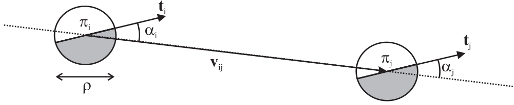
Figure B.1: Illustration of the values used for the collinearity computation. If we consider two primitives \pi_i and \pi_j , then the vector between the centres of these two primitives is written \mathbf{v}_{ij} , and the orientations of the two primitives are designated by the vectors t_i and t_j , respectively. The angle formed by \mathbf{v}_{ij} and t_i is written \alpha_i , and between \mathbf{v}_{ij} and t_j is written \alpha_j . \rho is the radius of the image patch used to generate the primitive.
