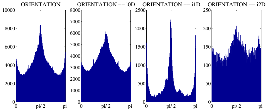
Figure 3.4: Orientation distribution depending on iD. The first image shows the total distribution. The sequences that have been used for this analysis are introduced in section 3.1.
