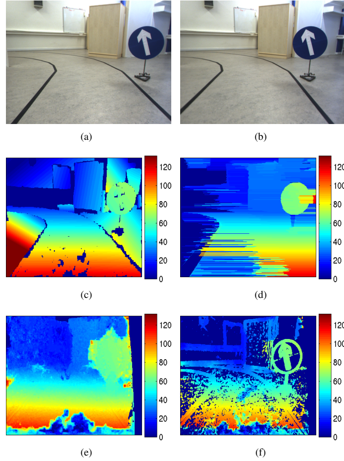
Figure 7.14: Experiment results on a road scene. (a,b) Input stereo pair. (c) The predictions of our model as a disparity map. (d) Disparity map from DP. (e) Disparity map from PB. (f) Subfigure (e) after a small threshold (0.001).
