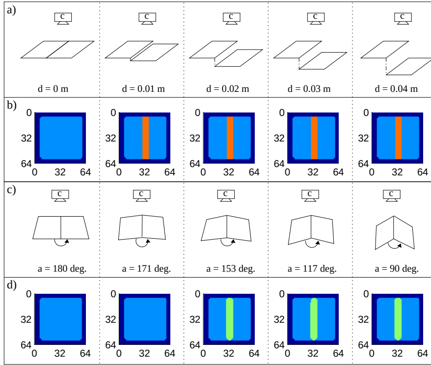
Figure 5.4: Results of the combined measures on artificial data. The camera and the range scanner are denoted by c. (a) Gap discontinuity tests. There are two planes which are separated by a distance d where d = 0, 0.01, 0.02, 0.03, 0.04 meters. (b) The detected discontinuities. Dark blue marks the boundary points where the measures are not applicable. Blue and orange respectively correspond to detected continuities and gap discontinuities. (c) Orientation discontinuity tests. There are two planes which are connected but separated with an angle a where a = 180, 171, 153, 117, 90 degrees. (d) The detected discontinuities. Dark blue marks the boundary points where the measures are not applicable. Blue and green respectively correspond to detected continuities and orientation discontinuities.
