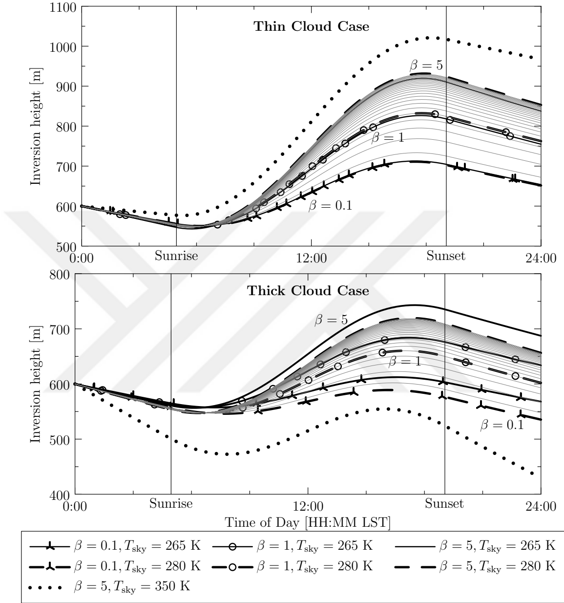
Figure 3.5: Inversion height trend ( z_i(t) ) with respect to different Bowen Ratios and T_{\text{sky}} radiative temperatures for the thin cloud case ( [0, 200] m, top) and the thick cloud case ( [200, 400] m, bottom). Other variables are fixed at T_{\text{srf}} = 289 K, T_{\text{cld}} = 285 K, \zeta_D = 51 K, D = -3.75 \times 10^{-6} \text{ s}^{-1} . Simulations with T_{\text{sky}} = 265 K (solid) and T_{\text{sky}} = 280 K (dashed) are shown. Simulations for Bowen Ratios between 0.1 and 5 are shown as thin gray lines for the T_{\text{sky}} = 280 K case with 0.2 increments. The dotted line is an admittedly unrealistic parameter choice to show a case where z_i(t) decreases. For this and all future graphs a latitude equal to 32.85^\circ N and Julian day of 196 were used for solar zenith angle calculations.
