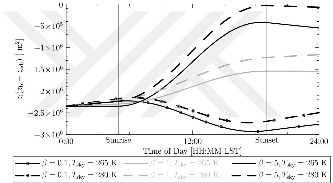
Figure 3.6: z_i(z_b - z_{\text{adj}}) (proxy for cloud base height) timeseries for different Bowen Ratios and T_{\text{sky}} radiative temperatures. Cases for T_{\text{sky}} = 265 \text{ K} (solid) and T_{\text{sky}} = 280 \text{ K} (dashed) are shown. Other variables are fixed at T_{\text{srf}} = 289 \text{ K} , T_{\text{cld}} = 285 \text{ K} , \zeta_D = 51 \text{ K} , D = -3.75 \times 10^{-6} \text{ s}^{-1} .
