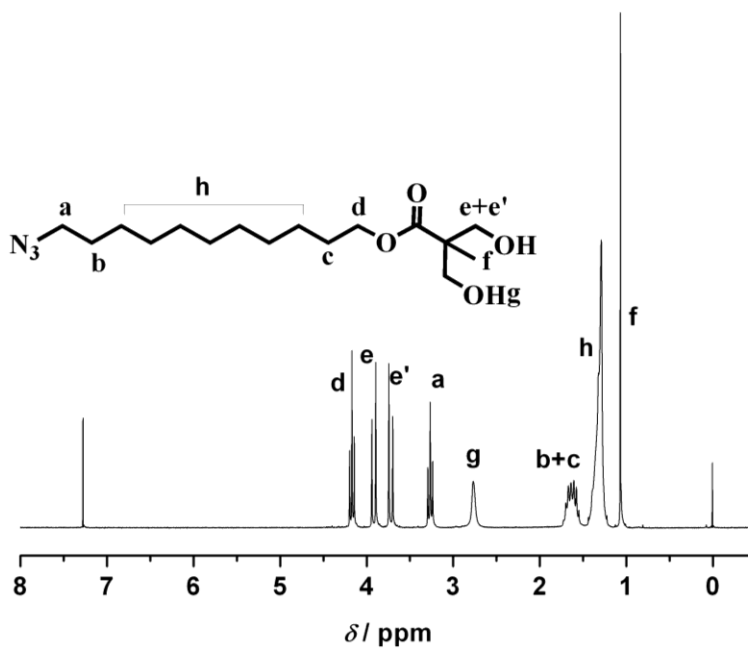
Figure 5.3 ^1\text{H} -NMR spectrum of 11-azidoundecyl 3-hydroxy-2-(hydroxymethyl)-2-methylpropanoate ( 4 ) in \text{CDCl}_3 .
