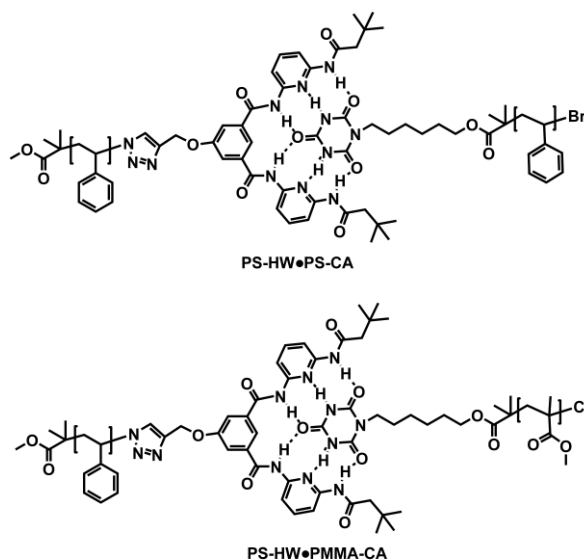
Scheme 5.1 Formation of poly(styrene)-Hamilton Wedge and poly(styrene)-cyanuric acid (PS-HW•PS-CA) as well as poly(styrene)-Hamilton Wedge and poly(methyl methacrylate)-cyanuric acid (PS-HW•PMMA-CA) block copolymers through H-bonding of Hamilton Wedge and cyanuric acid motifs.
