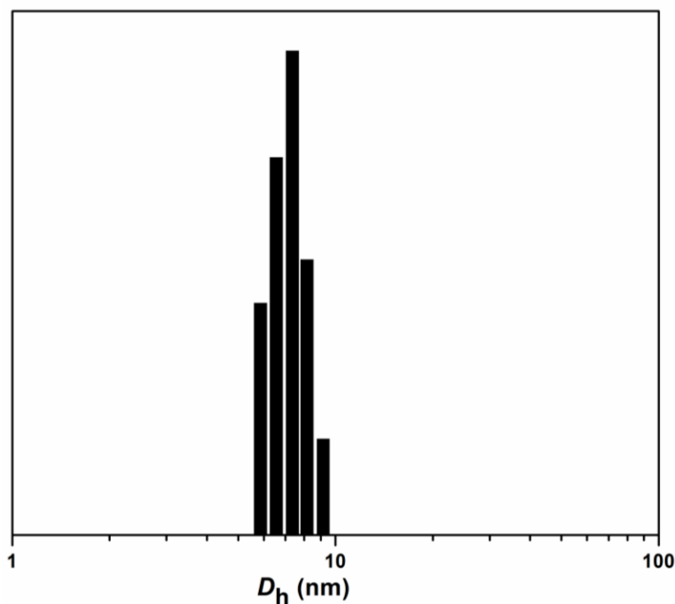
Figure 5.29 The mean hydrodynamic diameter of supramolecular grafted star-shaped macromolecules ( PS- g -PS ) 4 ( 30b ) determined at 90° in dichloromethane at ambient temperature.
