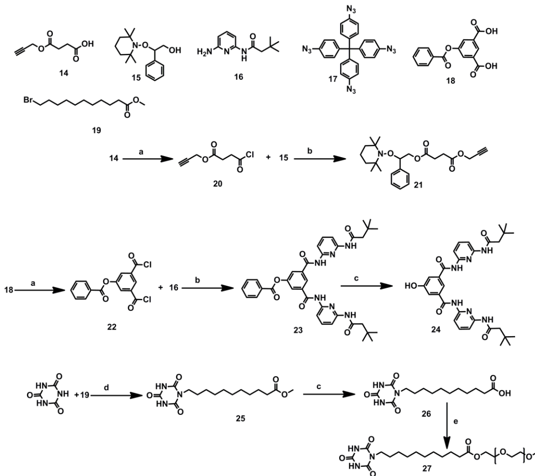
Scheme 5.6 Chemical structures used in current section and general strategy for the preparation of the alkyne functional NMP initiator, the hydroxyl functional Hamilton wedge, and cyanuric acid functional poly(ethylene glycol) ( CA-PEG ). Experimental conditions: (a) Oxalyl chloride, DMF, THF, 6h, r.t; (b) TEA, THF, overnight, r.t; (c) \text{NaOH}_{(\text{aq})} , MeOH/THF, 5h, r.t; (d) DBU, DMF, 24 h, 70 °C; (e) DCC, DMAP, DCM, MeO-PEG-OH.
