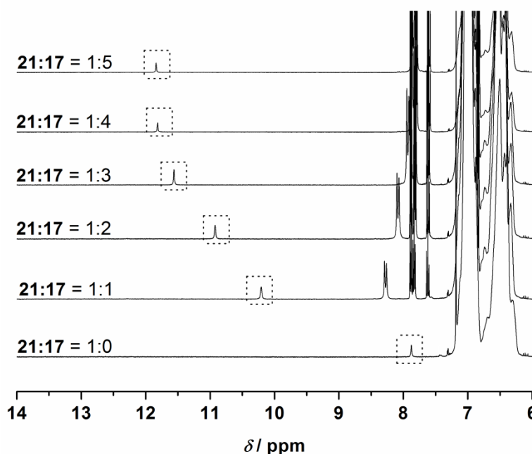
Figure 3.21 Expanded ^1\text{H} NMR spectra of the 21•17 self-assembly system with varied concentration ratios in \text{CD}_2\text{Cl}_2 at ambient temperature. The concentration of 21 was kept constant at 3 mM.
