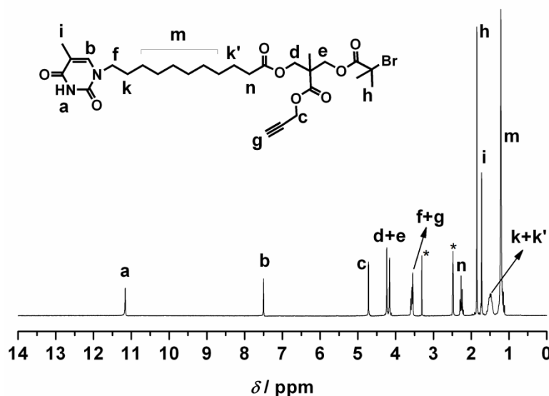
Figure 4.5 ^1\text{H} NMR spectrum of 2-((2-bromo-2-methylpropanoyloxy)methyl)-2-methyl-3-oxo-3-(prop-2-ynoxy)propyl 11-(5-methyl-2,4-dioxo-3,4-dihydropyrimidin-1(2H)-yl)undecanoate ( 6 ) in \text{DMSO}-d_6 . The resonances marked with an asterisk are associated with solvent/water.
