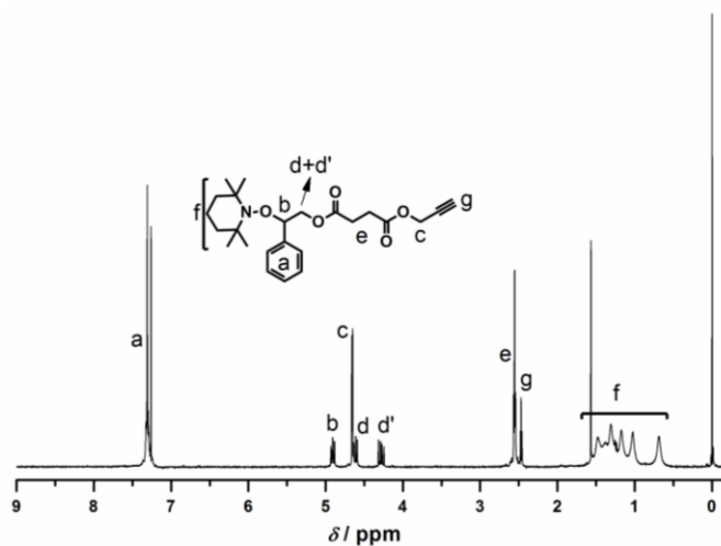
Figure 5.20 ^1\text{H} NMR spectrum of 2-phenyl-2-((2,2,6,6-tetramethylpiperidin-1-yl)oxy)ethyl prop-2-yn-1-yl succinate ( 21 ) in \text{CDCl}_3 at ambient temperature. The non-assigned resonance refers to solvent/water.
