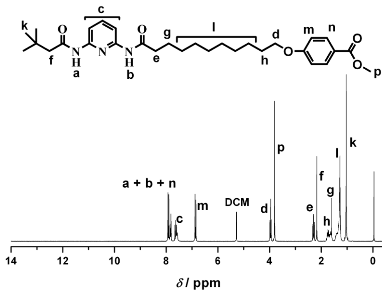
Figure 3.23 1 H-NMR spectrum of methyl 4-(11-(6-(3,3-dimethylbutanamido)pyridin-2-ylamino)-11-oxoundecyloxy) benzoate ( 17 ) in CD 2 Cl 2 .
