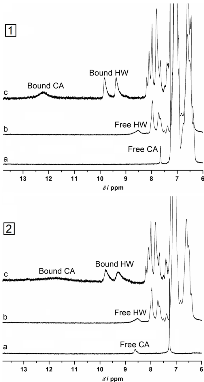
Figure 5.27 Expanded 1 H NMR spectrum of (1a) PS-CA (1b) (PS-co-HWS) 4 (1c) (PS-g-PS) 4 (2a) PMMA-CA (2b) (PS-co-HWS) 4 (2c) (PS-g-PMMA) 4 in CD 2 Cl 2 at ambient temperature. Equimolar amounts with respect to the HW and CA binding motifs were employed. The NMR data for the poly(ethylene glycol) system can be found in the Figure 5.27.
