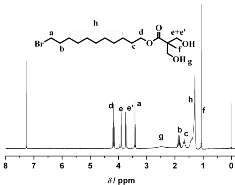
Figure 5.2 ^1\text{H} -NMR spectrum of 11-bromoundecyl 3-hydroxy-2-(hydroxymethyl)-2-methylpropanoate ( 3 ) in \text{CDCl}_3 .
