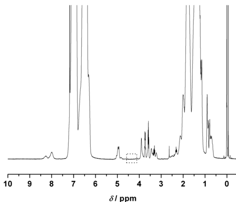
Figure 4.11 1 H NMR spectrum of 10 with azide functionality in CDCl 3 at ambient temperature. The dashed box within the figure shows that CH-Br of polymer 10 was quantitatively converted to its azide functionality.
