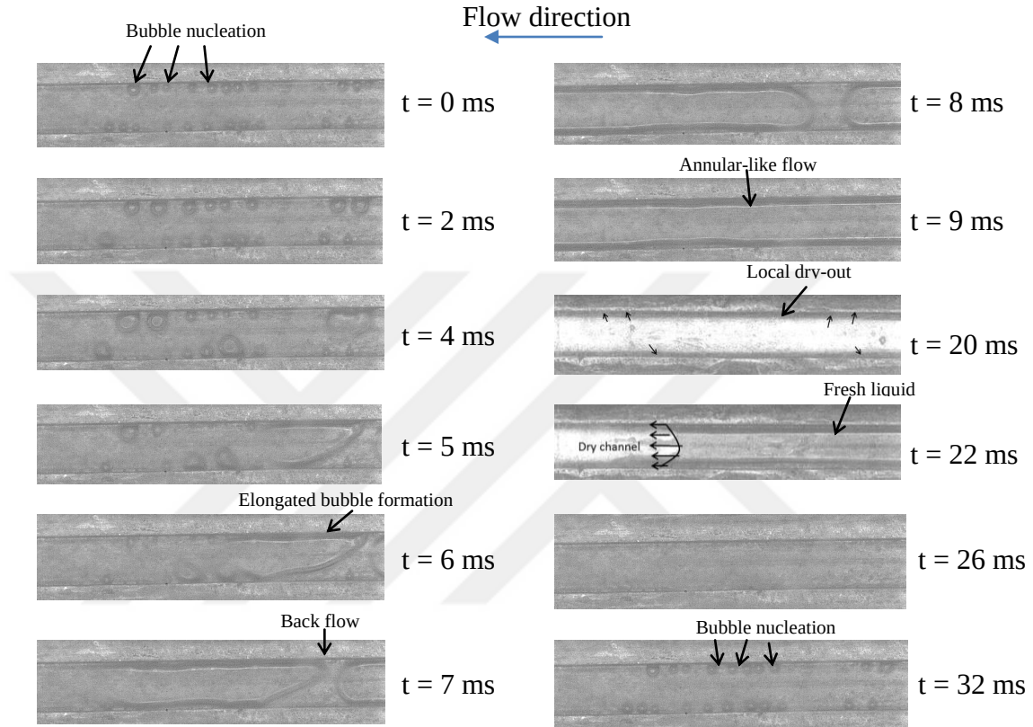
Figure 5.2 Sequence of flow images at the middle of the channel at periodic flow regime for the \beta = 2.56 and microchannel (TS1) at q'' = 99.15 \text{ kW/m}^2 and G = 400 \text{ kg/m}^2\text{s} .
