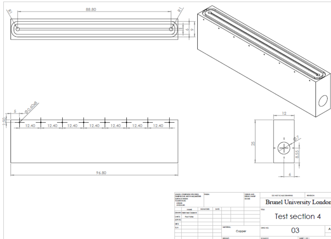
Figure 3.11 Engineering drawing of the microchannel test section 4 (TS4), dimensions in mm.
