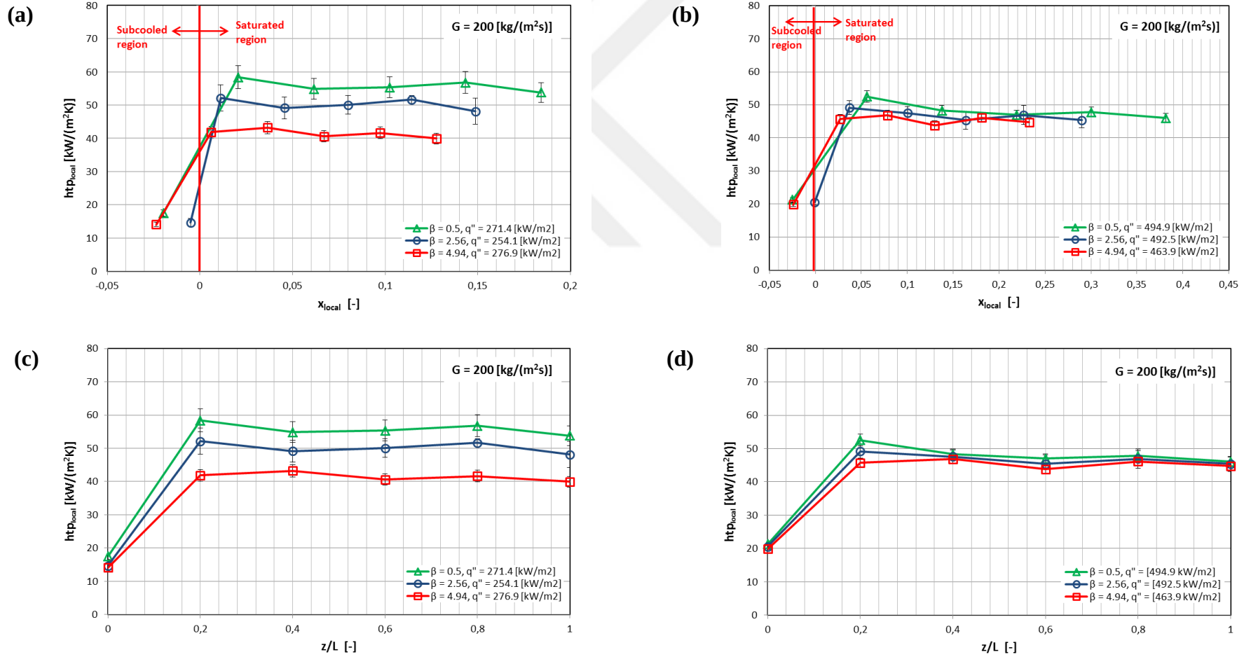
Figure 5.26 Effect of channel aspect ratio on the local heat transfer coefficient; (a) versus local vapour quality at G = 200 \text{ kg/m}^2\text{s} and low heat flux input, (b) versus local vapour quality at G = 200 \text{ kg/m}^2\text{s} and high heat flux input, (c) versus dimensionless distance at G = 200 \text{ kg/m}^2\text{s} and low heat flux input, (d) versus dimensionless distance at G = 200 \text{ kg/m}^2\text{s} and high heat flux input.
