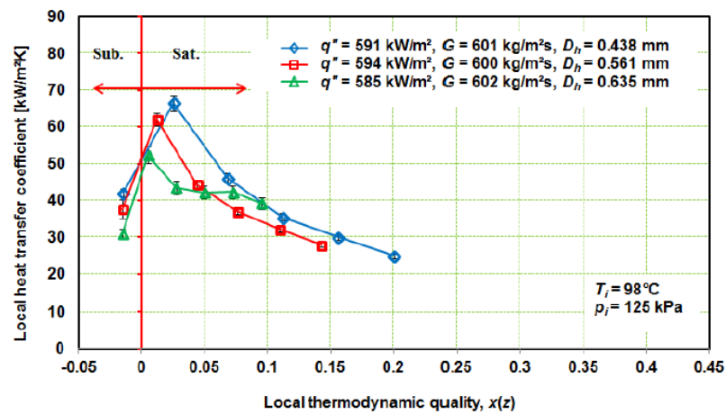
Figure 2.33 Effect of hydraulic diameter on the local heat transfer coefficient with increasin quality at G = 600 \text{ kg/m}^2\text{s} and similar heat flux values, Mirmanto (2012).
