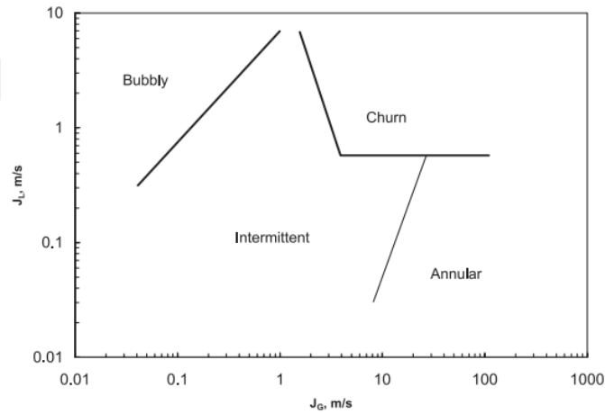
Figure 2.22 Flow map for horizontal channels having hydraulic diameter less than 1 mm based on air-water flow, Hassan et al. (2005).
