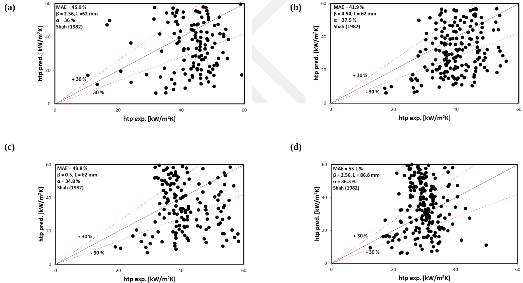
Figure 5.31 Comparison of the experimental heat transfer data with the Shah (1982) correlation: (a) TS1, (b) TS2, (c) TS3 and (d) TS4 microchannels.
