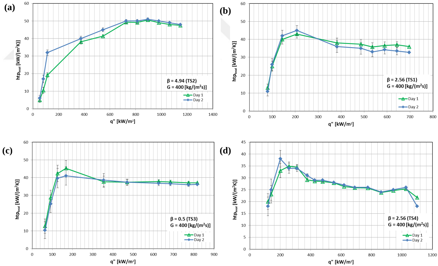
Figure 5.29 Repeatability of the local heat transfer data at a mass flux of G = 400 \text{ kg/m}^2\text{s} at z/L = 0.6 : (a) TS2, (b) TS1, (c) TS3 and (d) TS4 at z/L = 0.71 .
