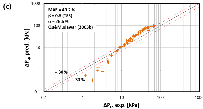
Figure 6.13 Comparison of experimental flow boiling pressure drop data with the Qu and Mudawar (2003b) correlation: (a) TS2, (b) TS1, (c) TS3 and (d) TS4.
