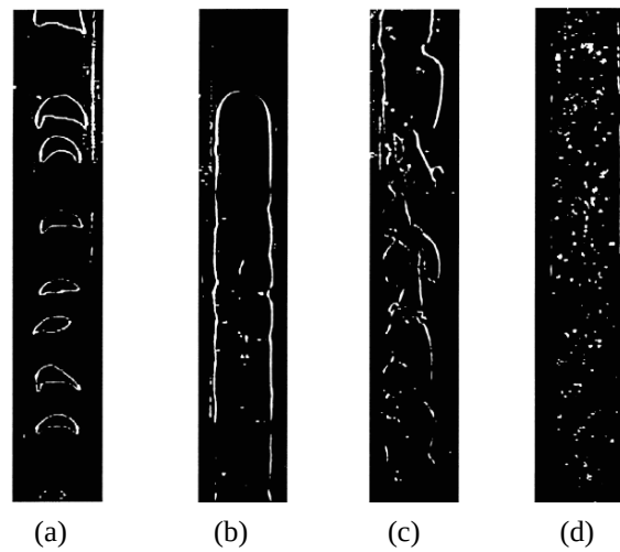
Figure 2.16 The flow patterns in vertical rectangular channel with 0.59 mm hydraulic diameter: (a) cap-bubbly; (b) slug-droplet; (c) churn; (d) annular-droplet, Xu et al. (1999).
