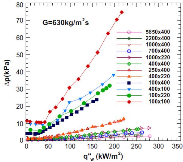
Figure 2.39 Effect of microchannel cross-sectional area on the pressure drop for FC-77 at G = 630 \text{ kg/m}^2\text{s} , Harirchian and Garimella (2009b).
