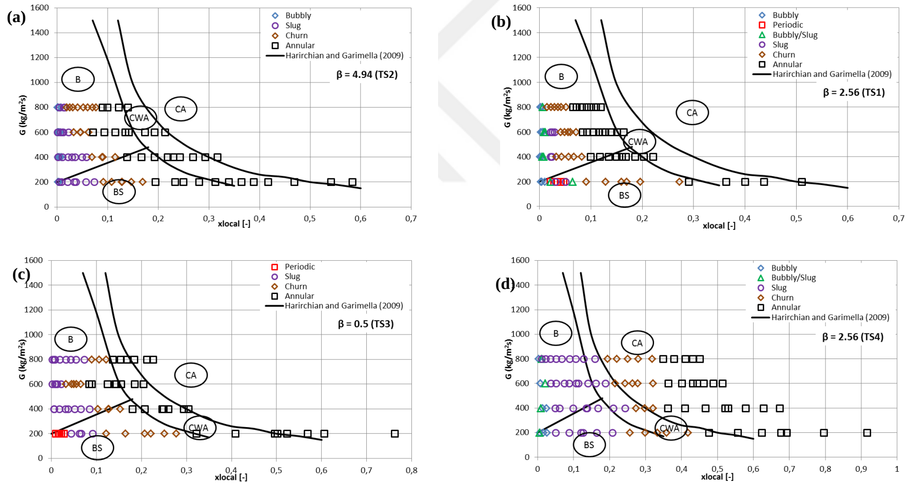
Figure 5.12 Comparison of the experimental flow patterns at the outlet region with flow pattern map of Harirchian and Garimella (2009a): (a) TS2, (b) TS1, (c) TS3 and (d) TS4. B: Bubbly incipience, BS: Bubbly-Slug flow, CWA: Churn-Wispy annular flow and CA: Churn-Annular flow.
