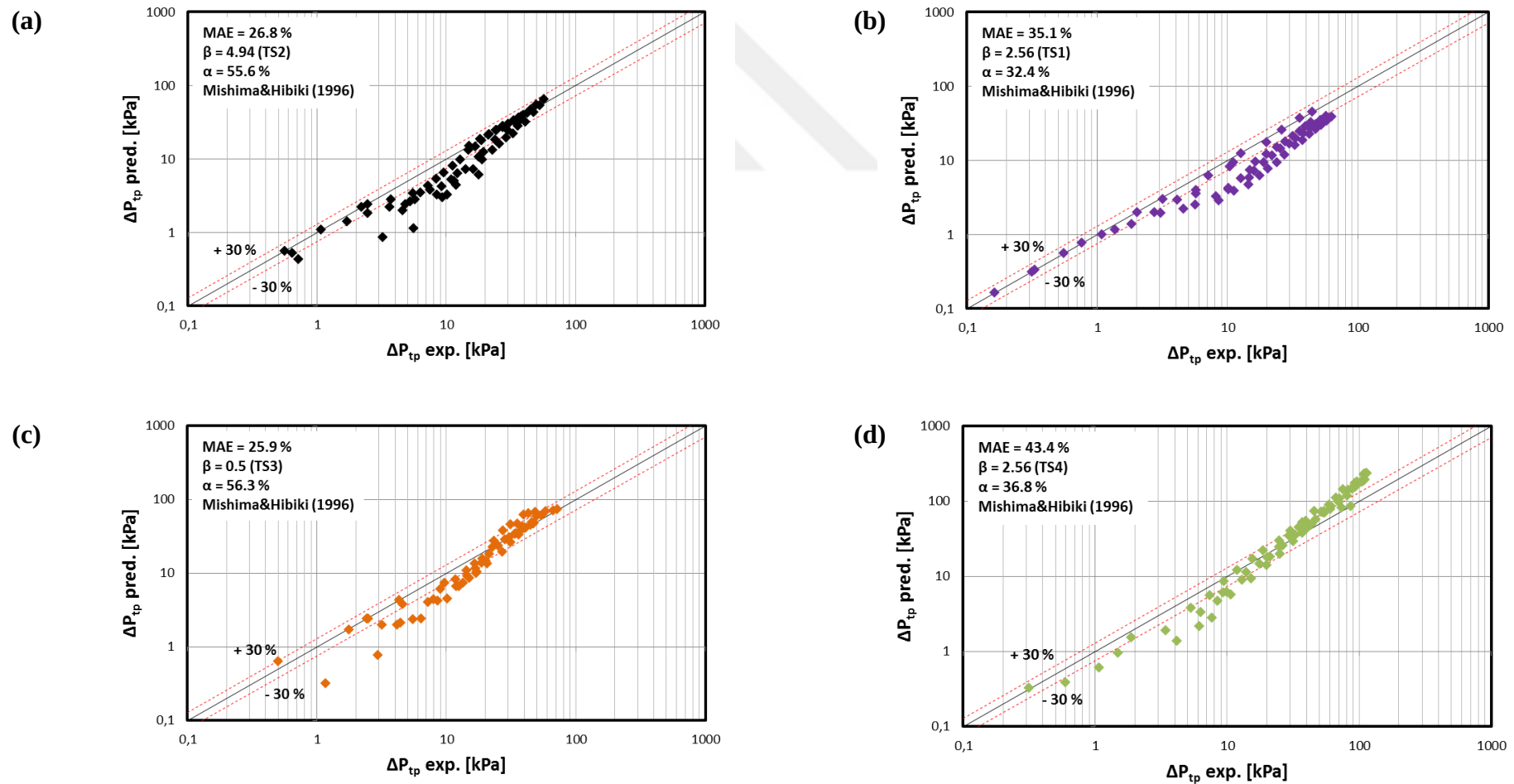
Figure 6.10 Comparison of experimental flow boiling pressure drop data with the Mishima-Hibiki (1996) correlation: (a) TS2, (b) TS1, (c) TS3 and (d) TS4.
