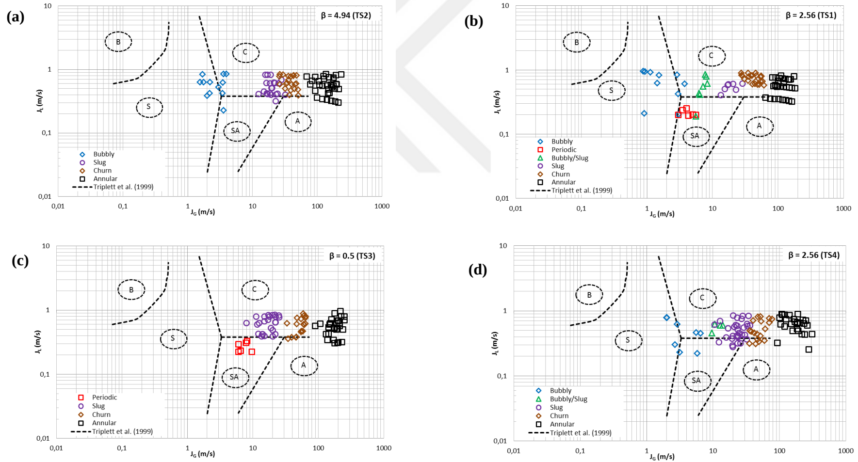
Figure 5.9 Comparison of the experimental flow patterns at the outlet region with flow pattern map of Triplett et al. (1999): (a) TS2, (b) TS1, (c) TS3 and (d) TS4. B: Bubbly flow, S: Slug flow, C: Churn flow, SA: Slug-Annular flow and A: Annular flow.
