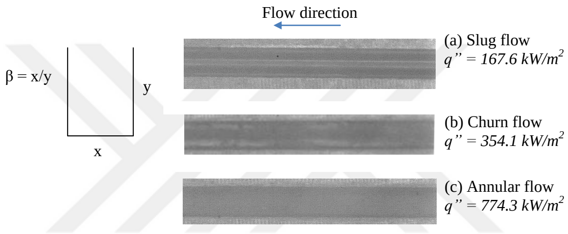
Figure 5.8 Flow patterns in the TS3 at the outlet region, for several heat fluxes at G = 400 \text{ kg/m}^2\text{s} .
