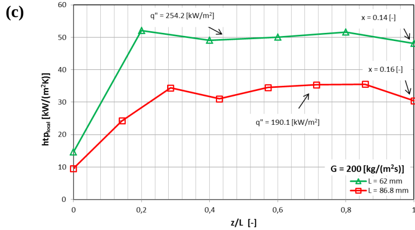
Figure 5.28 Effect of heated length on the local heat transfer coefficient; (a) versus local vapour quality at G = 200 kg/m²s and constant exit quality, (b) versus local vapour quality at G = 200 kg/m²s constant heat flux, (c) versus dimensionless distance at G = 200 kg/m²s and constant exit quality, (d) versus dimensionless distance at G = 200 kg/m²s and constant heat flux.
