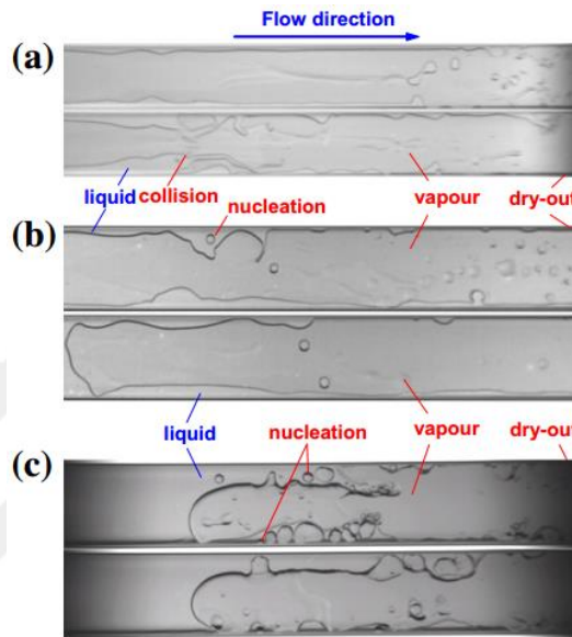
Figure 2.20 Flow regimes of FC-72 in three horizontal borosilicate glass microchannels at G = 44.8\ \text{kg/m}^2\text{s}^1 : (a) D_h = 571\ \mu\text{m} at q'' = 6\ \text{kW/m}^2 , (b) D_h = 762\ \mu\text{m} at q'' = 5.95\ \text{kW/m}^2 and (c) D_h = 1454\ \mu\text{m} at q'' = 7.56\ \text{kW/m}^2 , Wang and Sefiane (2012).
