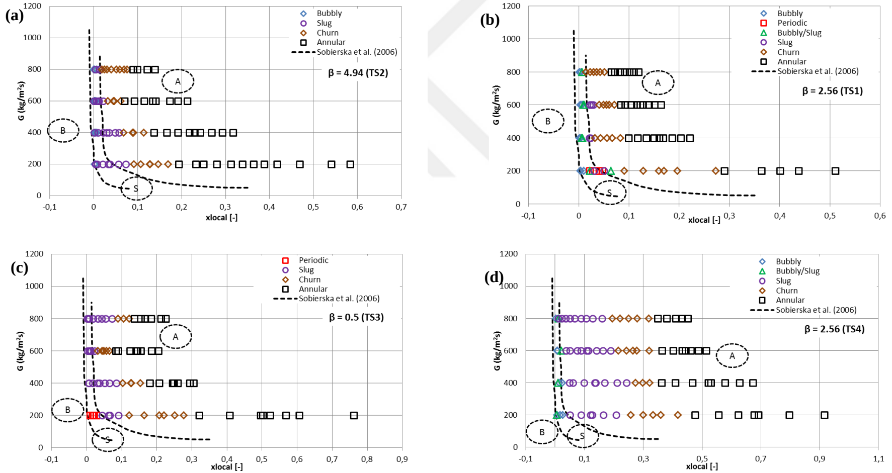
Figure 5.13 Comparison of the experimental flow patterns at the outlet region with flow pattern map of Sobierska et al. (2006): (a) TS2, (b) TS1, (c) TS3 and (d) TS4. B: Bubbly flow, S: Slug flow and A: Annular flow.
