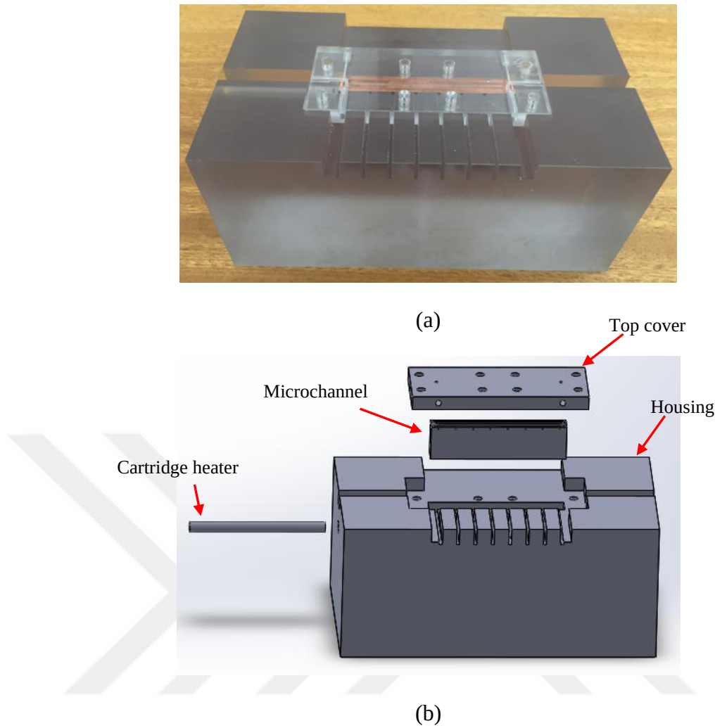
Fig 3.14 Assembly of the housing, top cover and microchannel test section; (a) Photograph, (b) Exploded view.
