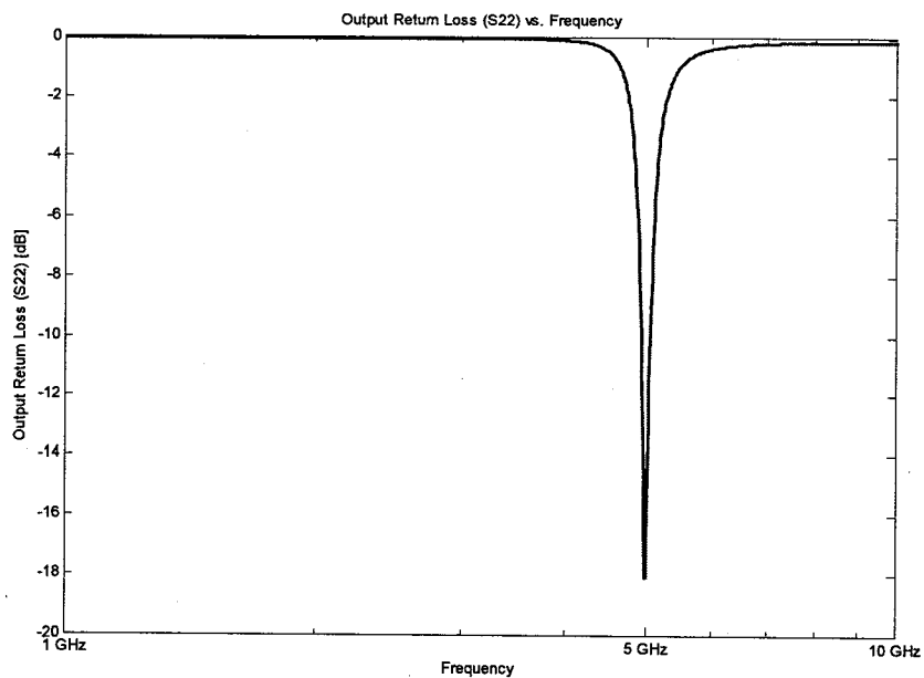
Figure 18: Output Return Loss vs. Frequency
