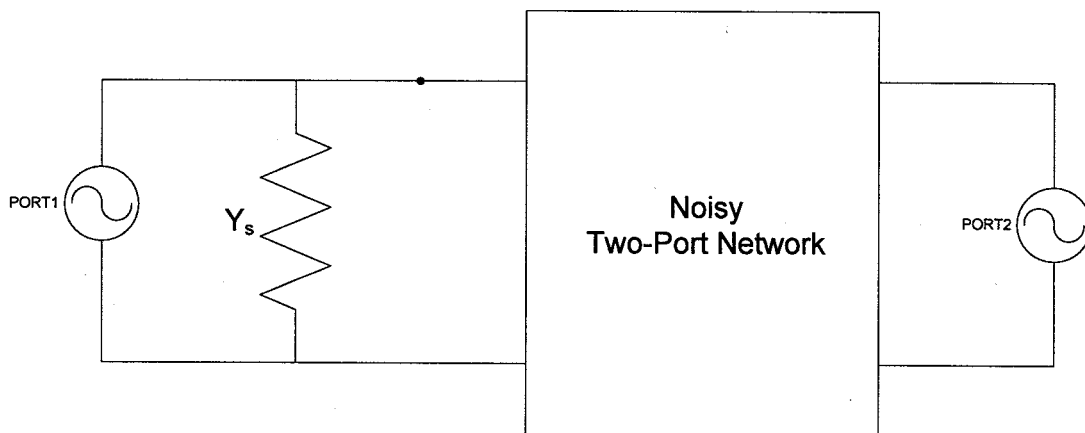
Figure 3: An example of a two-port noisy network
