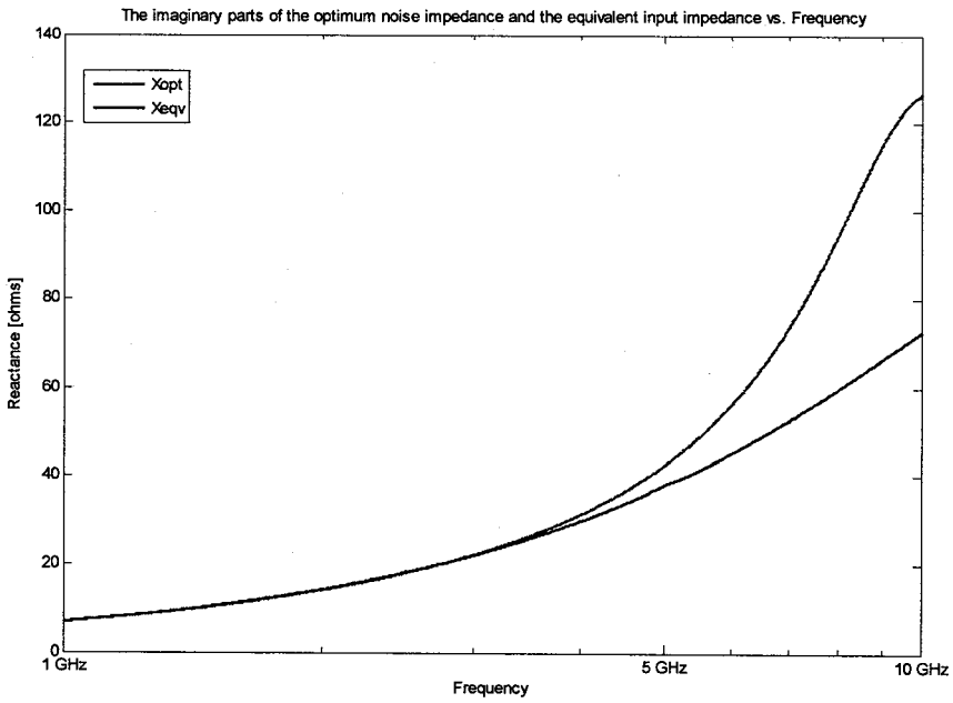
Figure 15: Xopt and Xeqv vs. Frequency
