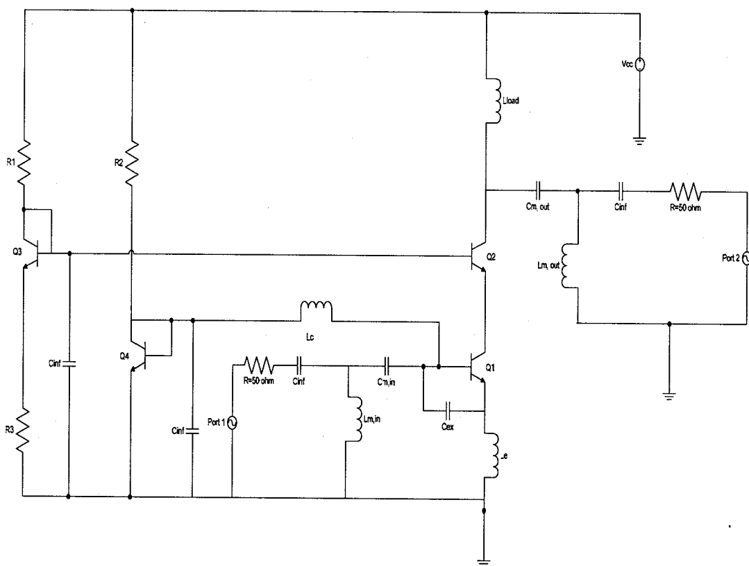
Figure 11: The designed circuit topology
