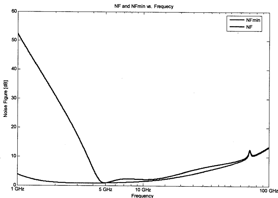
Figure 16: NF and \text{NF}_{\min} vs. Frequency
