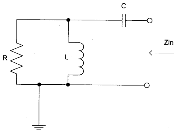
Figure 44: Basic L-type high-pass matching network
