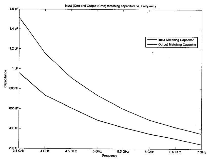
Figure 39: Variation in the values of the Input and Output Matching Capacitor (realistic)
