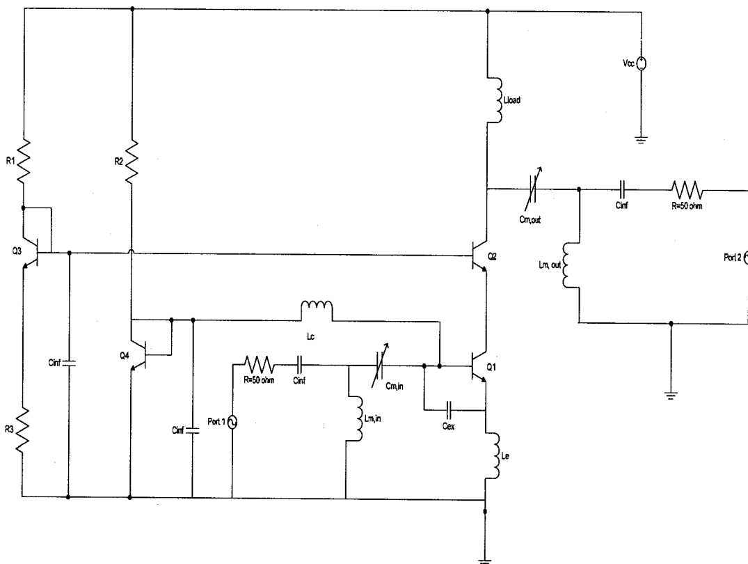
Figure 33: Suggested topology for tunable low noise amplifier
