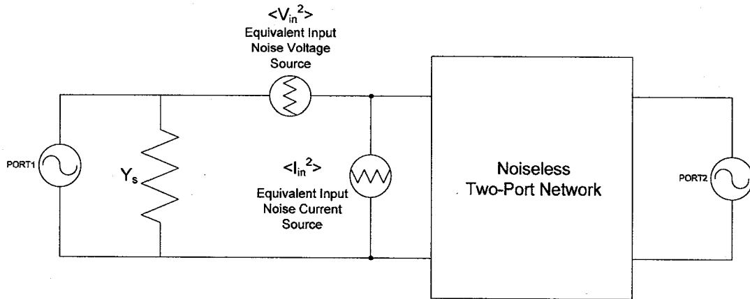
Figure 4: Noiseless two-port network with the equivalent noise sources
