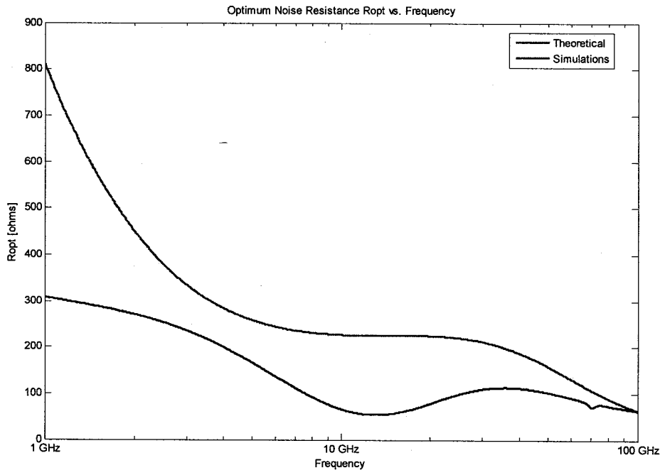
Figure 10: Optimum Noise Resistance R_{opt} vs. Frequency
