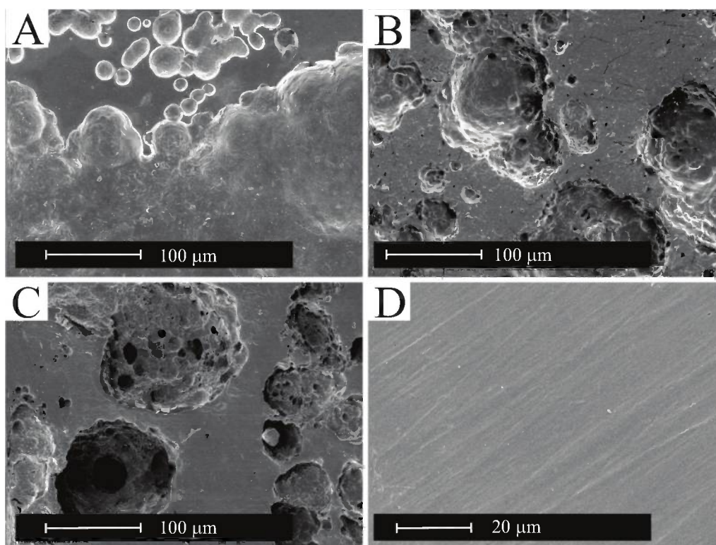
Figure 5. SEM micrographs showing the surfaces of the (co)polymer network films containing 100 % (A, from reference 22 ) 39 % (B), 18 % (C), 0 % (D) TMC after 5 days of subcutaneous implantation in rats.
