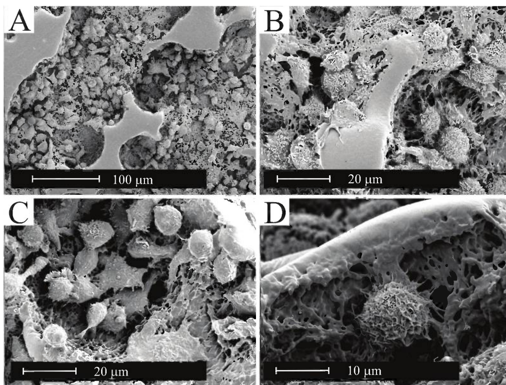
Figure 3. SEM micrographs of J774A macrophages on PTMC films after 14 days of culturing at magnifications of 250X (A), 1000X (B), 1000X (C), 2000X (D).
