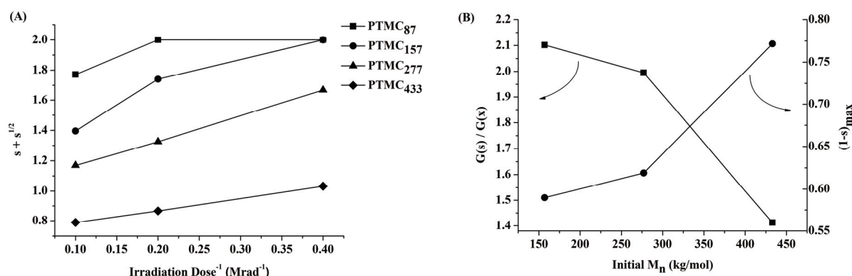
Figure 2. Charlesby-Pinner plots for networks prepared by gamma-irradiation of PTMC films of different initial molecular weights (A), and the effect of initial polymer molecular weight on the ratio of the radiation chemical yield of chain scission to crosslinking ( G(s)/G(x) ) and on the maximum gel percentage that can be obtained (1-s)_{\max} (B).
