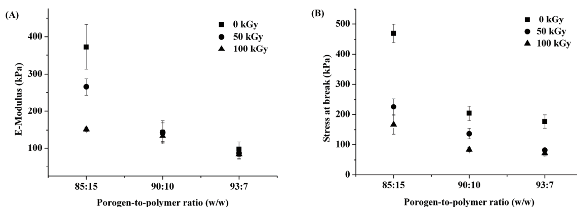
Figure 2. Effect of the porogen-to-polymer ratio and the gamma irradiation dose on the elastic modulus (A) and stress at break (B) values of porous PTMC structures.
