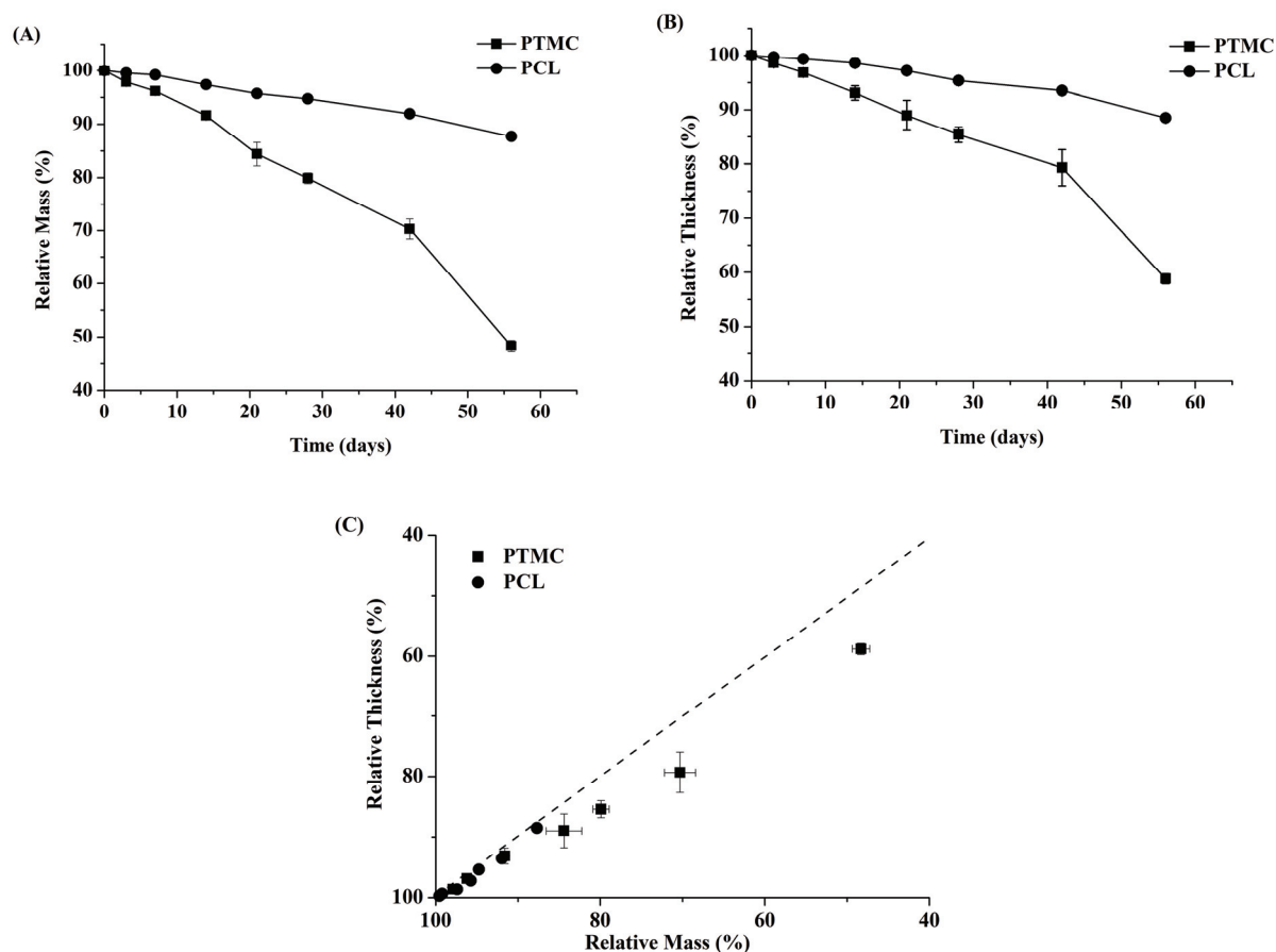
Figure 7. Erosion of PTMC films and PCL films in buffer (pH=13) containing 1.0 M KO 2 in time. The figure shows changes in mass (A), changes in thickness (B), and the relationship between the relative thickness and relative mass of PTMC and PCL films during erosion (C).
