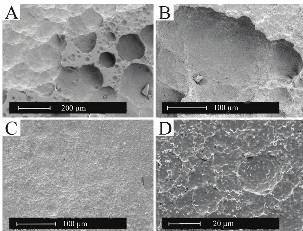
Figure 6. SEM micrographs showing the surface of PTMC films after incubation for 14 days in CE solutions (A, B), and in LPL solutions (C,D).
