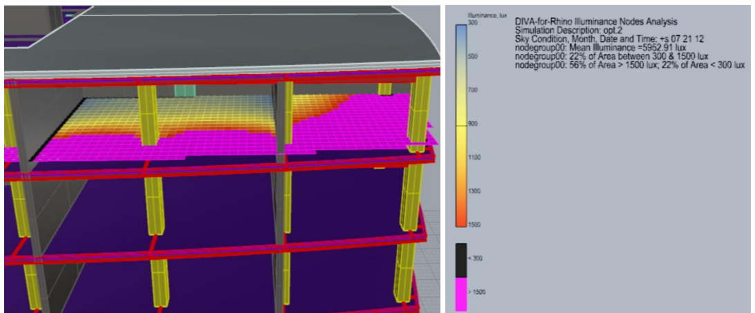
Figure 4.26 : The analysis result of the luminance levels for 21st of July at 12:00.
