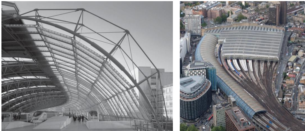
Figure 2.12 : International Terminal Waterloo in London by Nicholas Grimshaw, 1993 (Url-5).
