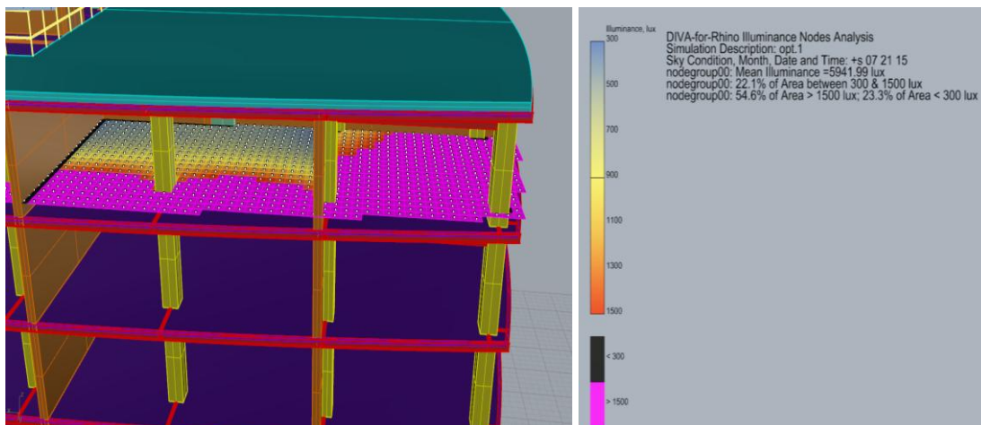
Figure 4.27 : The analysis result of the luminance levels for 21st of July at 15:00.
