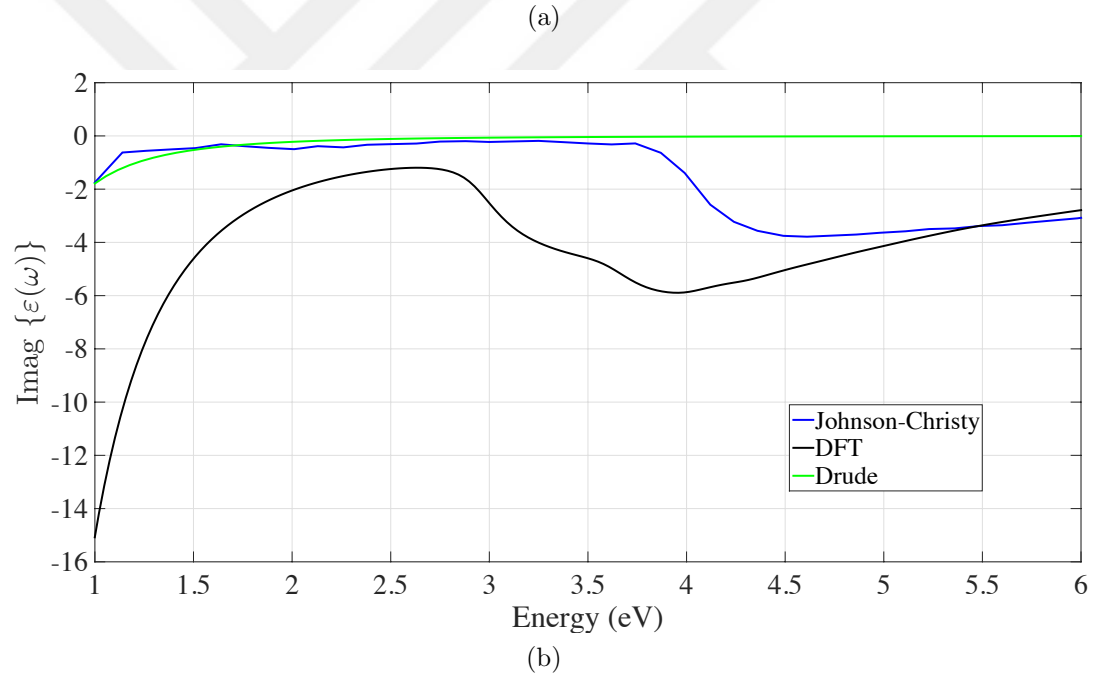
Figure 4.7: (a) Real and (b) imaginary parts of \varepsilon(\omega) for bulk silver.
