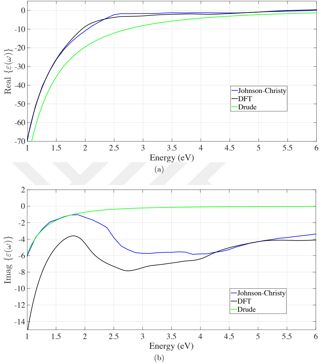
Figure 4.6: (a) Real and (b) imaginary parts of \varepsilon(\omega) for bulk gold.
