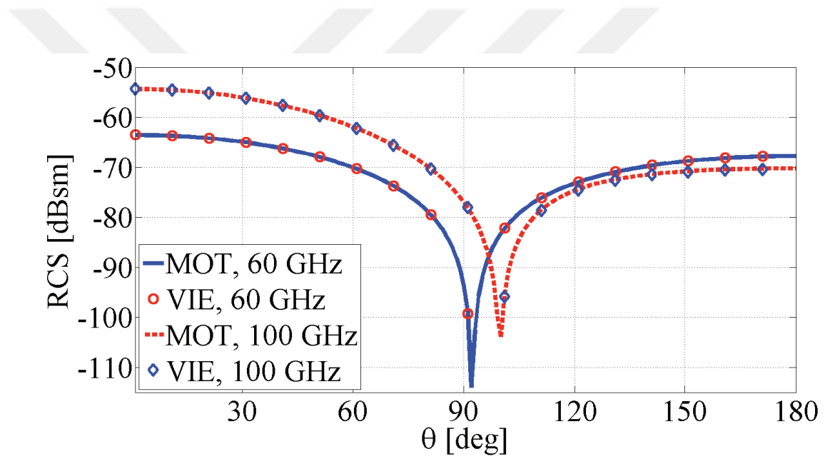
Figure 2.3: RCS obtained from the MOT and FD-VIE solutions for \phi = 0^\circ and 0^\circ \leq \theta < 180^\circ at 60 GHz and 100 GHz.
