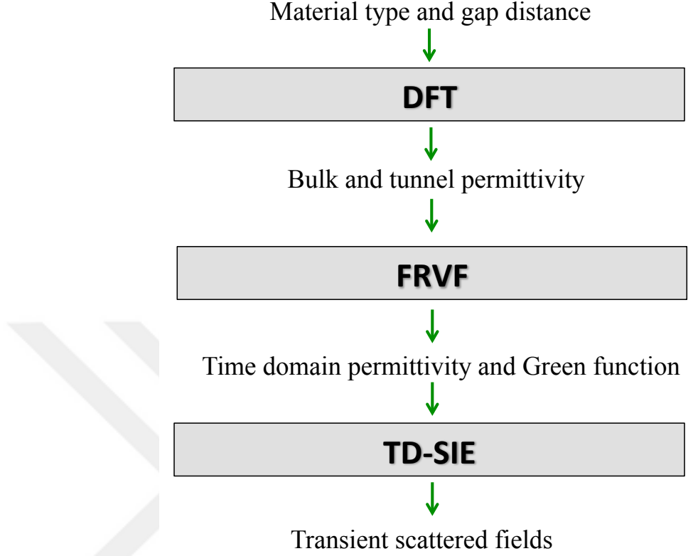
Figure 4.1: Steps of the quantum corrected transient electromagnetic analysis
