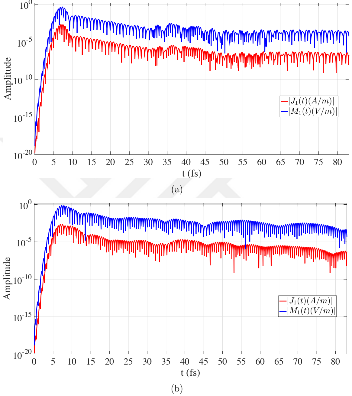
Figure 3.4: Amplitude of J_1(t) and M_1(t) induced on (a) the gold sphere and (b) the silver sphere.
