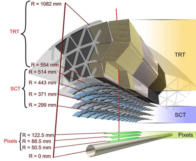
Figure 3.2. Inner Detector [4].
