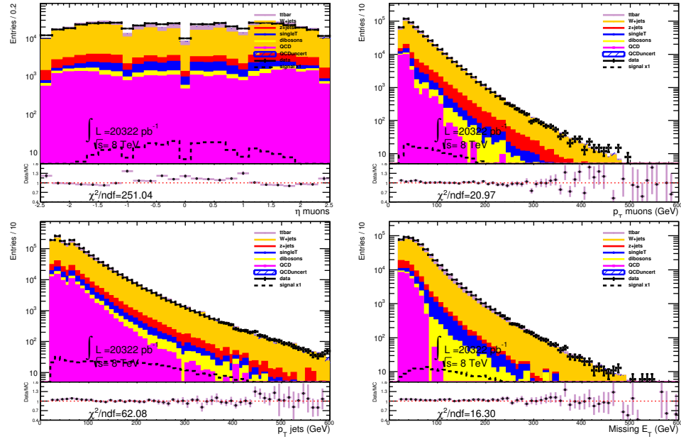
Figure B.2. P_T and \eta of muons, P_T of jets, E_T^{miss} distribution in muon channel only with 3 jets.
