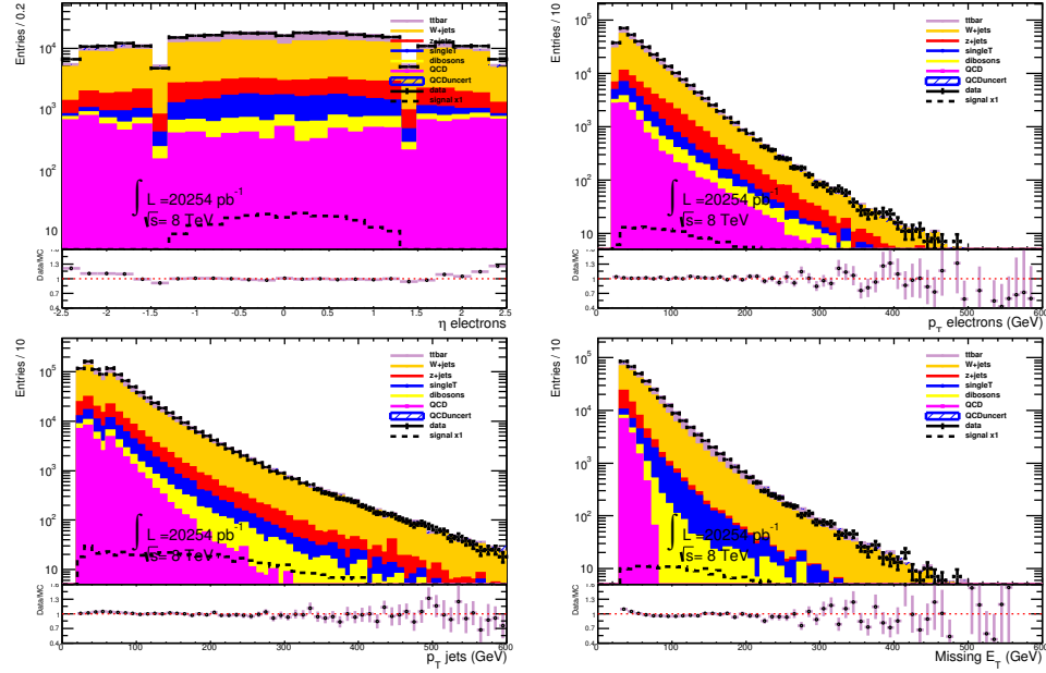
Figure B.1. P_T and \eta of electrons, P_T of jets, E_T^{miss} distribution in electron channel only with 3 jets.
