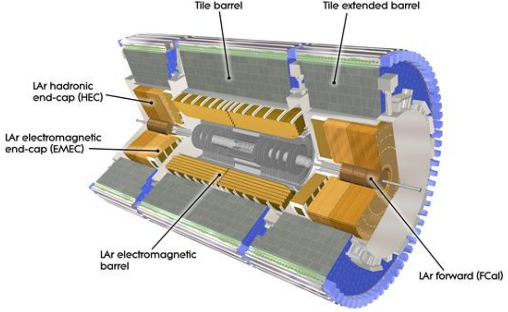
Figure 3.3. ATLAS Calorimeters [4].
