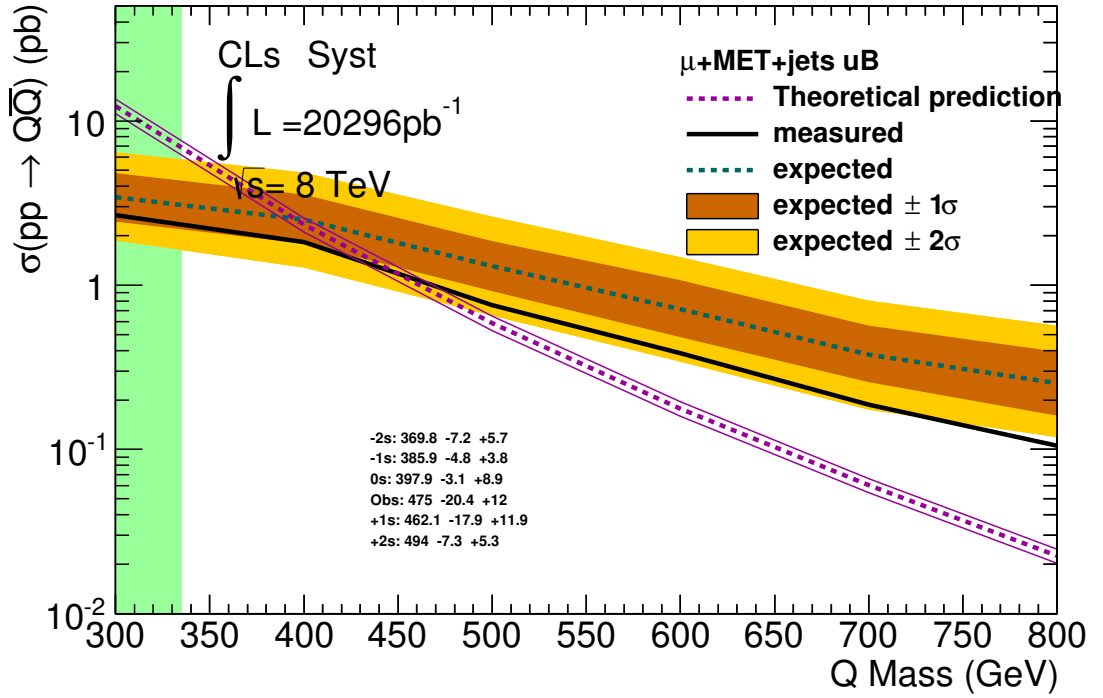
Figure 8.6. Limit with 95% confidence level for muon channel only.
