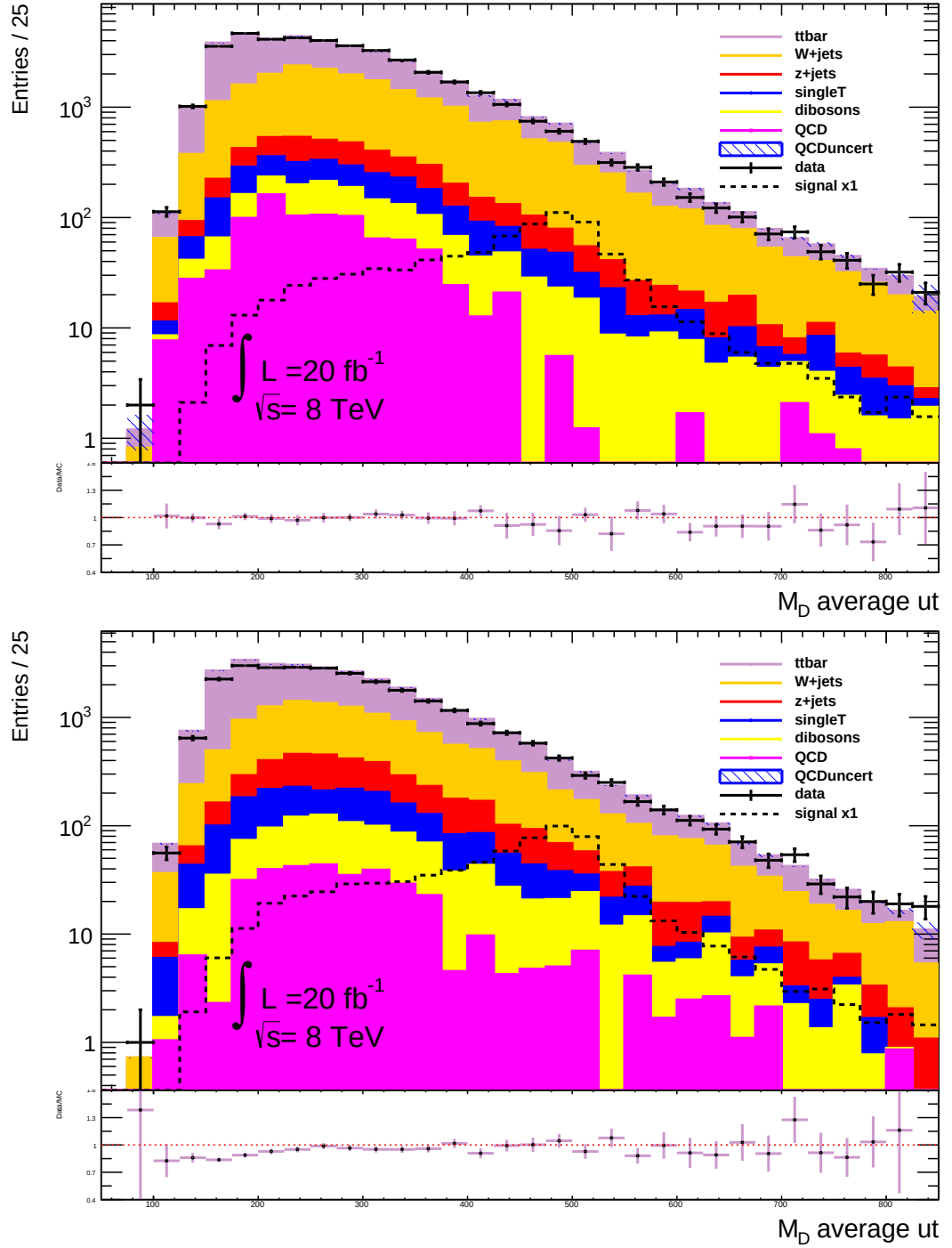
Figure 8.4. Average invariant mass of Q in muon (top) and electron (bottom) channels.
