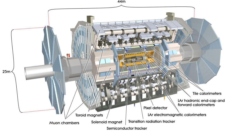
Figure 3.1. Atlas Detector [4].
