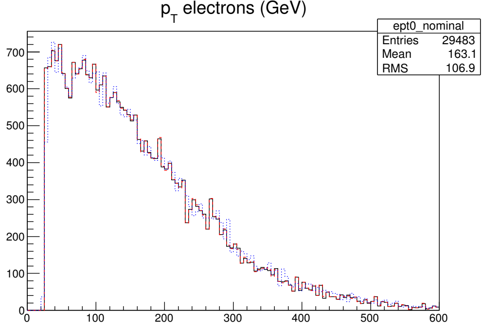
Figure 7.2. The effect of the \pm 1\sigma variations of electron energy smearing on electron P_T distribution of 600 GeV signal sample.
