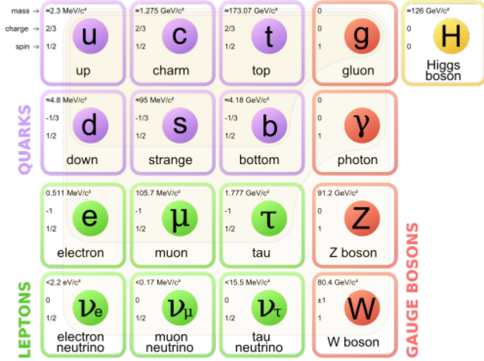
Figure 2.1. Fundamental particles [1].
