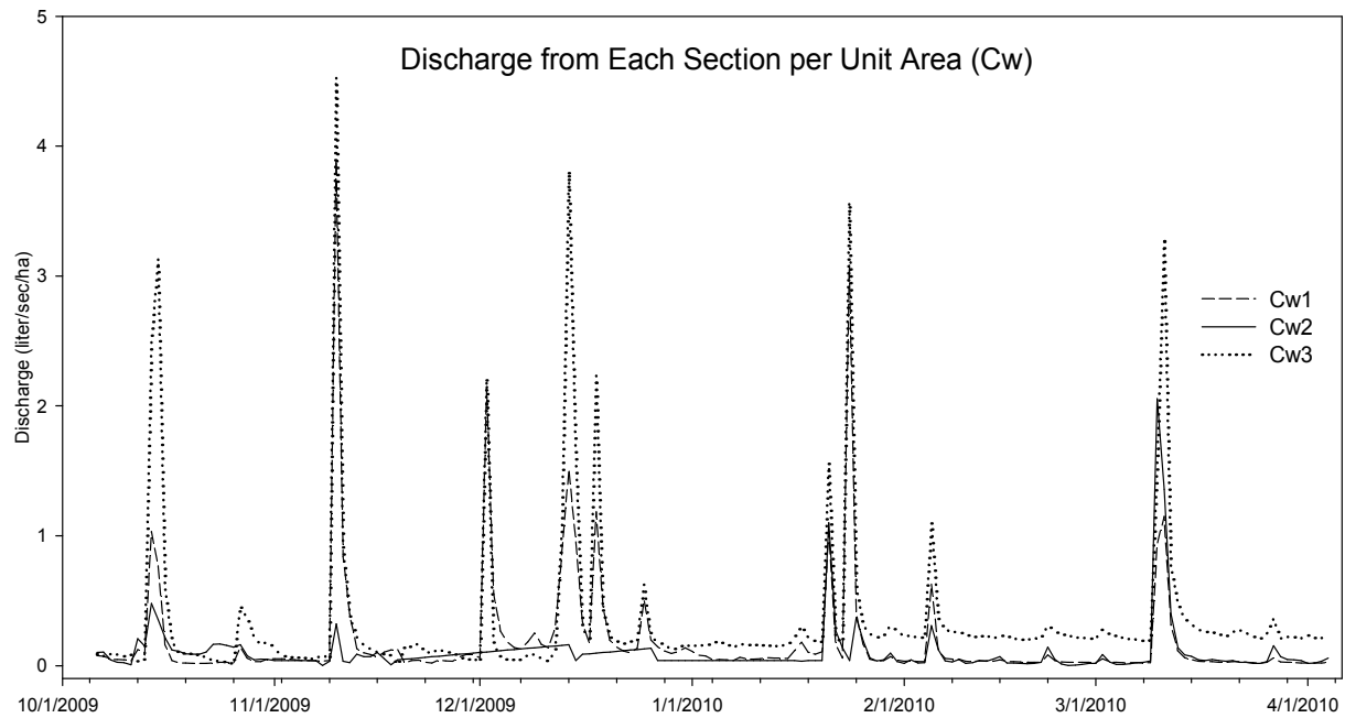
Figure 4.15: Discharge per unit area on the control watershed for post-harvest conditions
