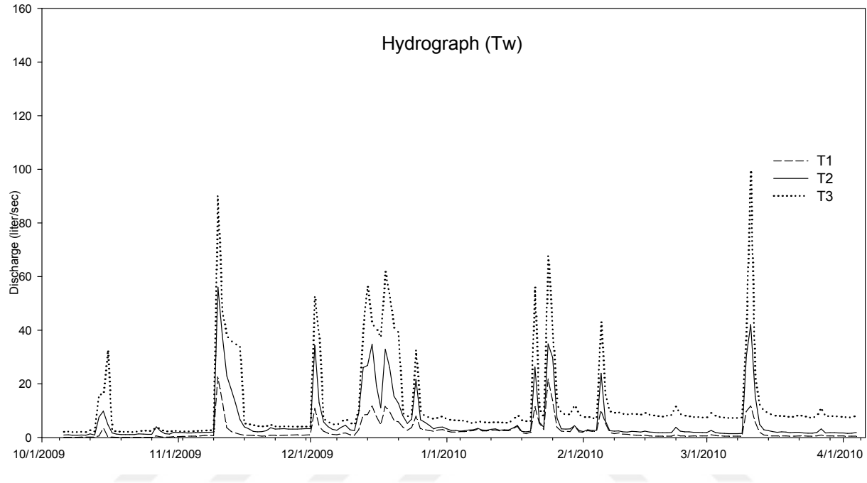
Post-treatment hydrograph of the treatment watershed
