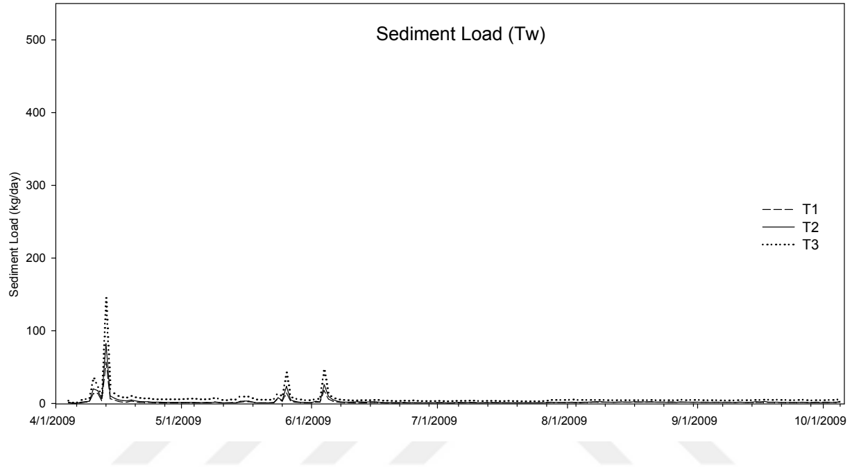
Sediment yield on the control watershed for pre-harvest conditions
