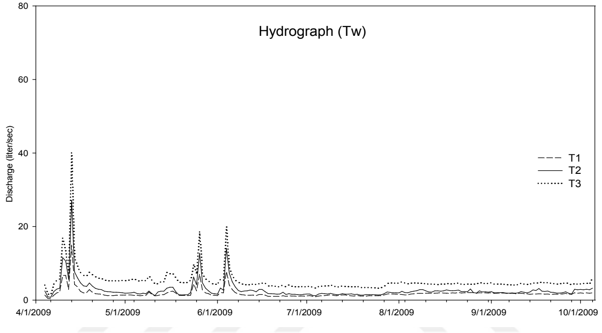
Pre-treatment (Calibration) hydrograph of the treatment watershed
