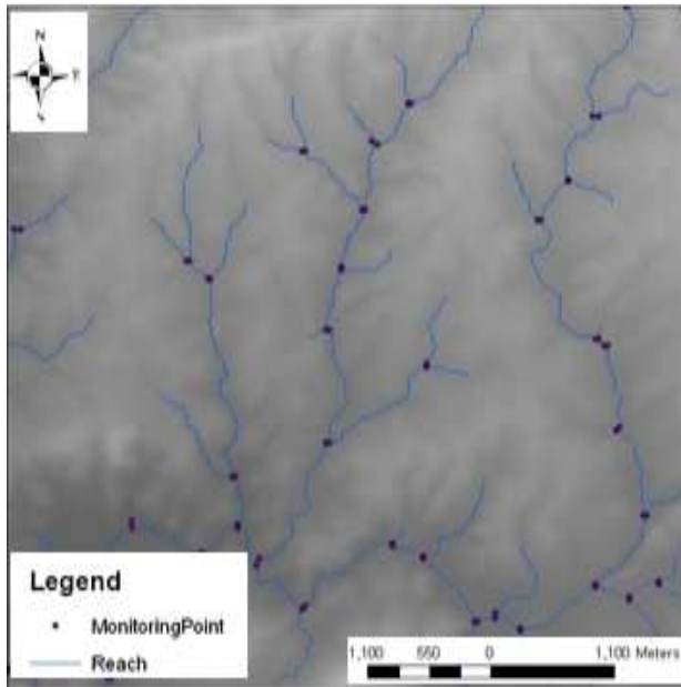
Figure 3.3: Stream processing
