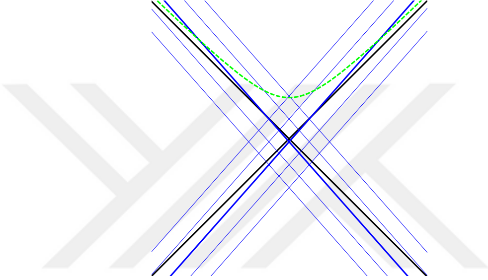
Figure A.1: Light-cone picture of the interaction of two nuclei. The thick black lines show the light-cone coordinates x^+ and x^- . Note that the transverse direction \mathbf{x}_\perp does not appear in this two-dimensional plot. The nuclei are comprised of partons shown as blue lines. The partons are not parallel to the light-cone because, in our treatment, the nuclei have speed \beta < c . The thick blue lines correspond to the partons exactly at the center of the nuclei ( x_\parallel = 0 ). Each parton from a nucleus interacts with all of the partons from the other nucleus, albeit at different times. One such time \tau' > 0 is shown with the green dashed line. The latest interaction occurs on the green hyper-surface by the partons from the rear of both the nuclei. The partons in the front of the nuclei interact even before \tau = 0 . Imposing the \tau = 0 as the interaction hyper-surface, we find boundary condition for the partons that interact on \tau = 0 . These two partons interact at the vertex, and they are shown with thick blue lines.
