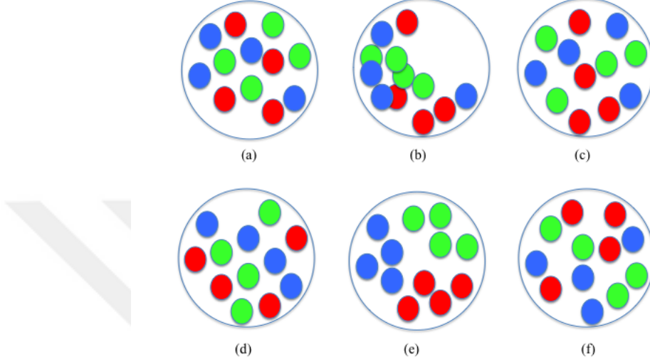
Figure 3.3: Some members of the charge configuration ensemble. In each collision, quarks with color red, green or blue in a nucleus are positioned differently. The positions of the color charges are encoded in the color charge density \rho^a(\mathbf{x}) , however, it cannot be known for a particular collision. Therefore, a statistical approach using an ensemble averaged quantities becomes inevitable. The configuration in (b) does not contribute much to the weight function since it is very unlikely for quarks in a nucleus to gather on one side of the nucleus. The configuration in (e) is also unlikely since there is high order in the way colors gather in specific locations.
