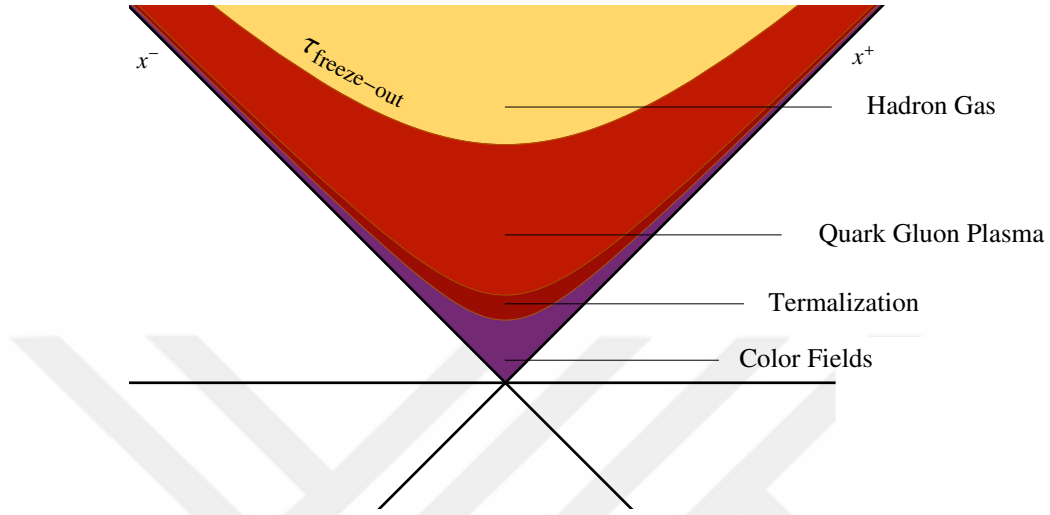
Figure 2.5: Formation and evolution of QGP. Collision of two nuclei occurs at the vertex where x^+ = x^- = 0 . On the hyperbolic boundaries the proper time \tau is constant.
