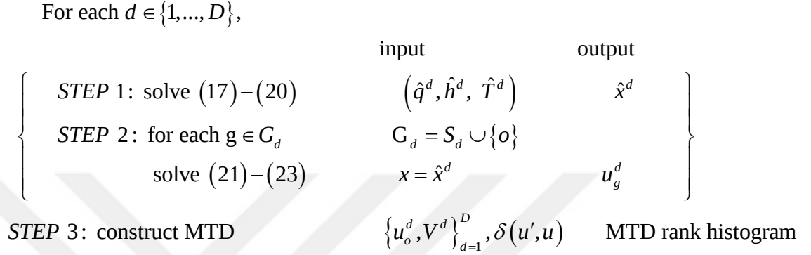
Figure 4.1 Generic scenario assessment
