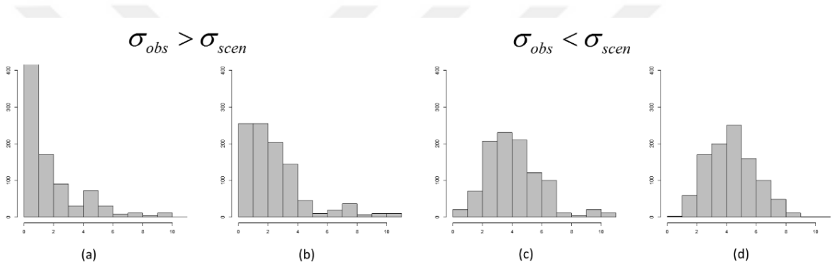
Figure 4.11 MTD rank histograms obtained by PI based scenario assessment when applied to SUC for \sigma_{obs} = 100 and \frac{\sigma_{obs}}{\sigma_{scen}} = (a) 4 (b) 2 (c) \frac{1}{2} (d) \frac{1}{4} .
