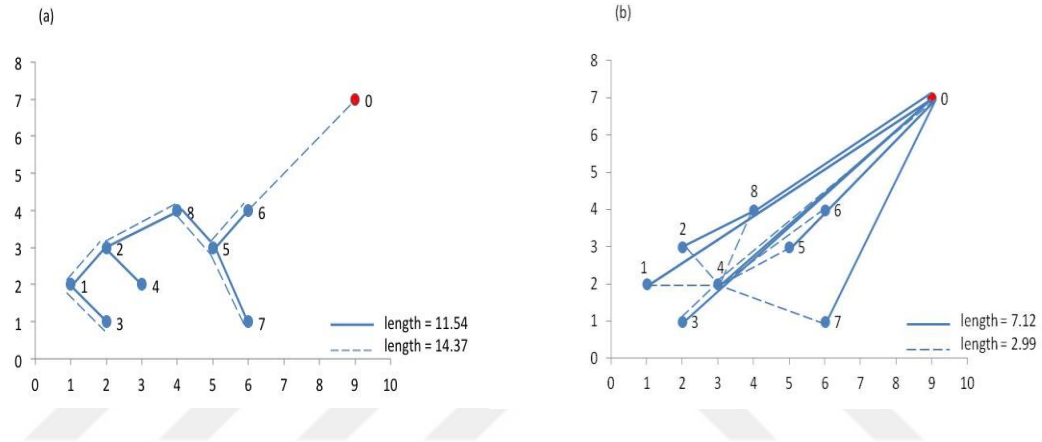
Figure 2.2 The observation 0, is moved to point (9,7) from point (4,2) to obtain an under-dispersed and/or biased ensemble, whereas the 8 scenarios labeled 1-8, have been kept at their same coordinates. The observation becomes exterior to the convex hull of the scenarios. (a) The solid lines indicate an MST for the scenarios labeled 1-8, and the dashed lines indicate an MST that results from the observation being substituted for scenario 4. (b) Similarly, solid edges are used to transport probability from the scenarios to the observation, and dashed edges are used to transport probability to scenario 4 from all other scenarios plus the observation.
