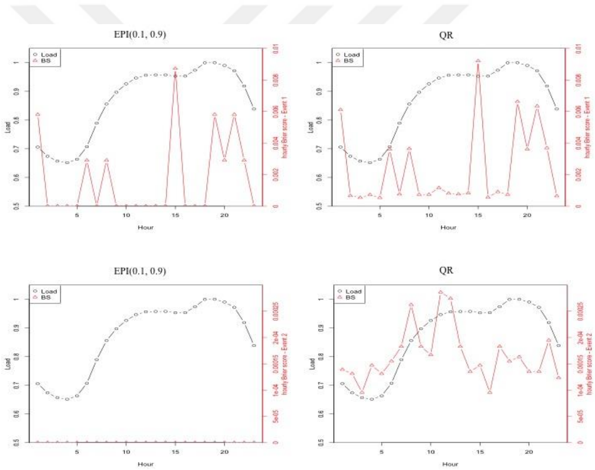
Figure 3.6 Hourly average load and average hourly Brier scores for Event 1 and 2
