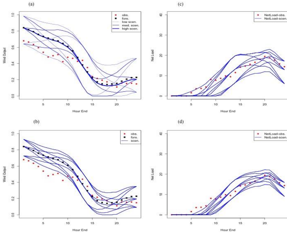
Figure 3.9 Wind power scenarios and net load scenarios for day 2013/04/14. (a) EPI(0.1, 0.9), (b) EPI(0.33, 0.66), (c) Net load scenarios for EPI(0.1, 0.9), (d) Net load scenarios for EPI(0.33, 0.66)
