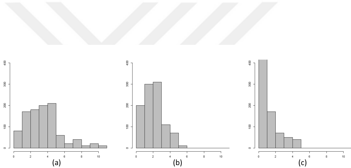
Figure 4.9 Possible MTD rank histograms obtained by PI-based scenario assessment when we try different combinations of parameters while keeping \mu_{obs} = \mu_{scen} , \sigma_{obs} = \sigma_{scen} , and \rho_{obs} = \rho_{scen} with (a) (s_{obs} = 70, m_{obs} = 2500, r_{obs} = .75) (b) (s_{obs} = 300, m_{obs} = 1500, r_{obs} = .50) and (c) (\sigma_{obs} = 800, \mu_{obs} = 800, \rho_{obs} = .50) .
