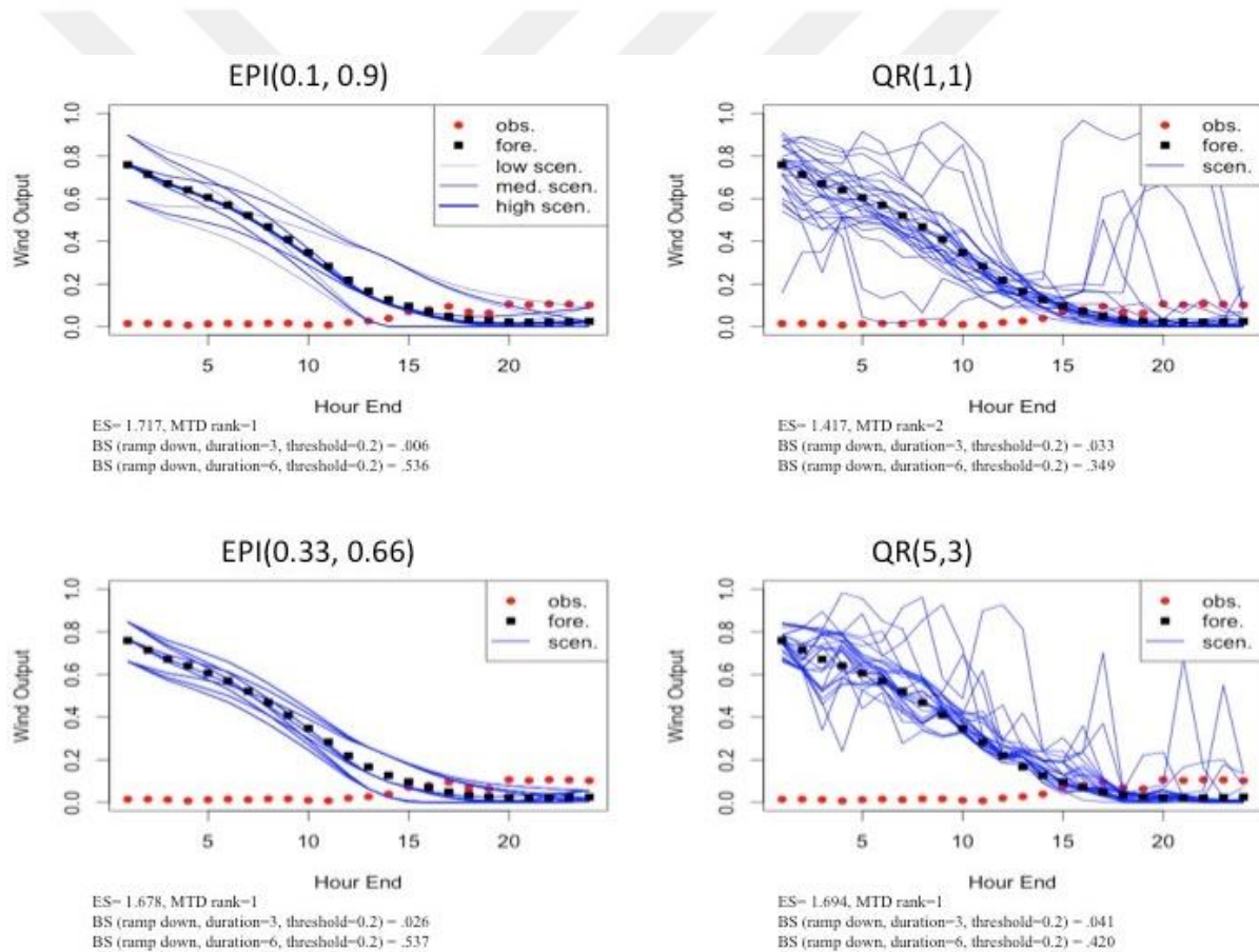
Figure 2.11 Wind power scenarios generated for day 2012-11-08
