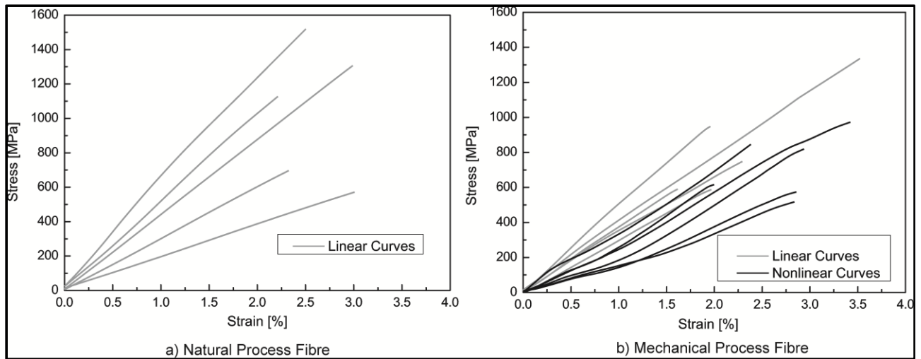
Figure 4.5. Stress strain behaviour of single flax fibres: a) naturally processed fibres, and b) mechanically processed fibres
