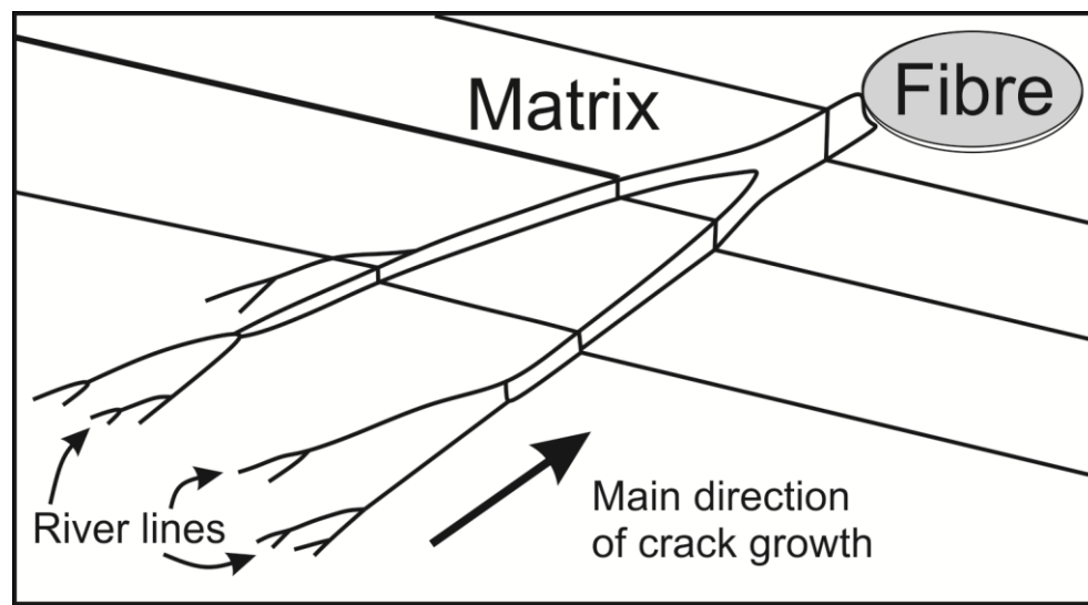
Figure 5.9. Schematic river line patterns showing sequence of steps into larger steps in matrix area after (Hull, 1999).
