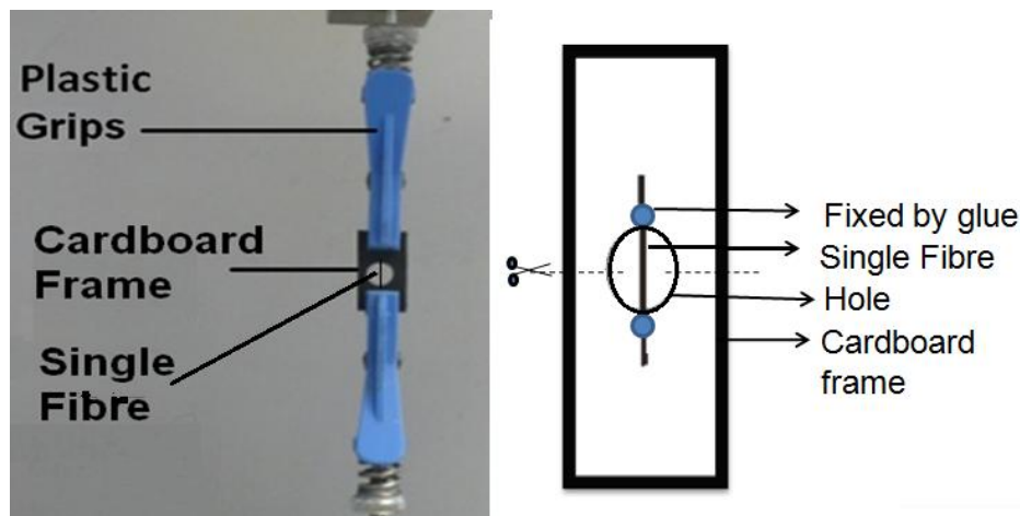
Figure 3.3. Experimental set-up for tensile testing of single flax fibres
