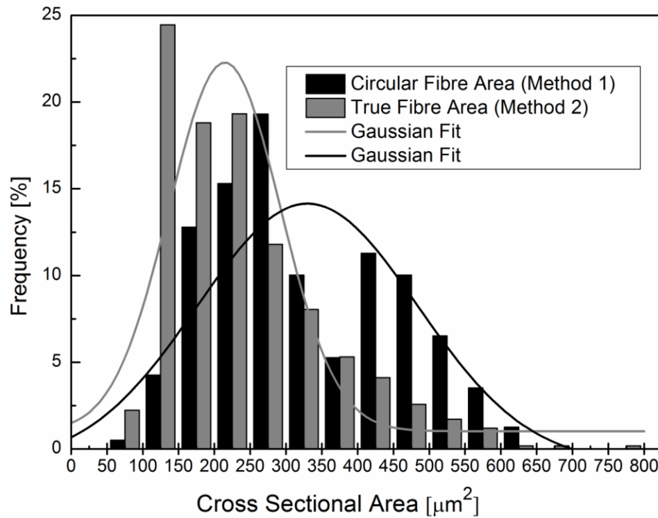
Figure 4.4. Frequency distribution of the cross sectional area of fibres determined by two methods of circular fibre area and true fibre area.
