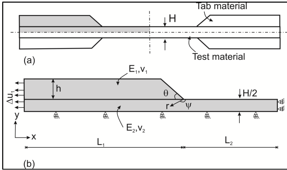
Figure 5.14. The straight sided tensile test specimen along the cross section (a) and modelled part of the quarter of tensile specimen (b) shown with defined boundary conditions.
