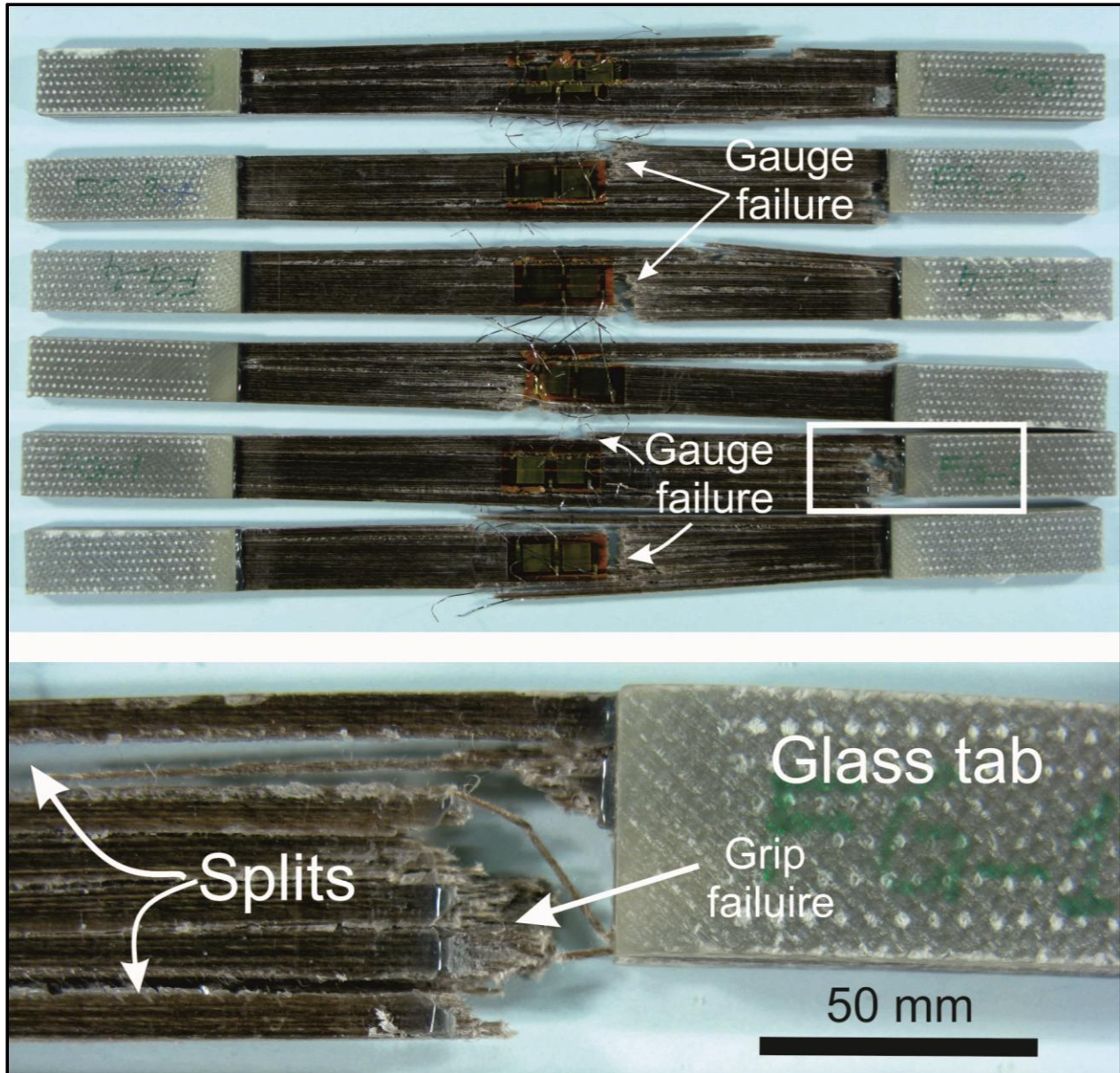
Figure 5.6. Typical specimen-tab edge failure for the unidirectional Flax/LPET composites.
