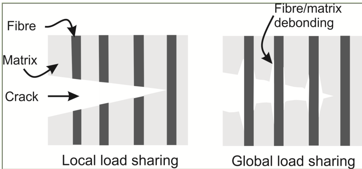
Figure 5.8. A sketch of load transfer mechanisms in fibre composites.
