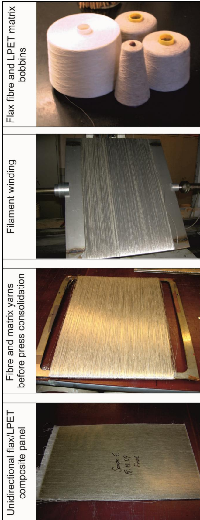
Figure 3.1. The applied fabrication route for unidirectional flax/LPET composites.
