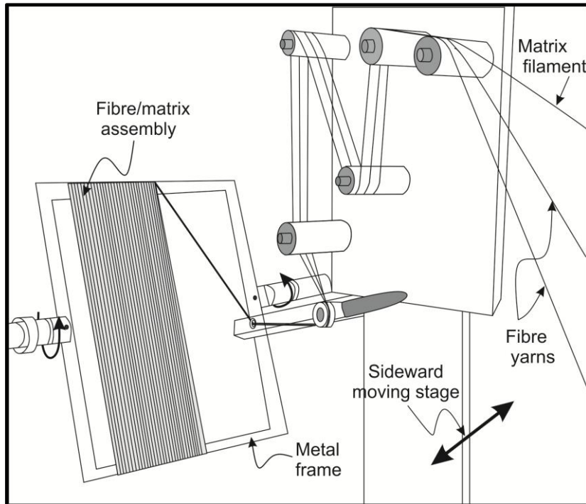
Figure 3.2. Commingled fibre/matrix winding set-up for unidirectional flax fibre/LPET assemblies.
