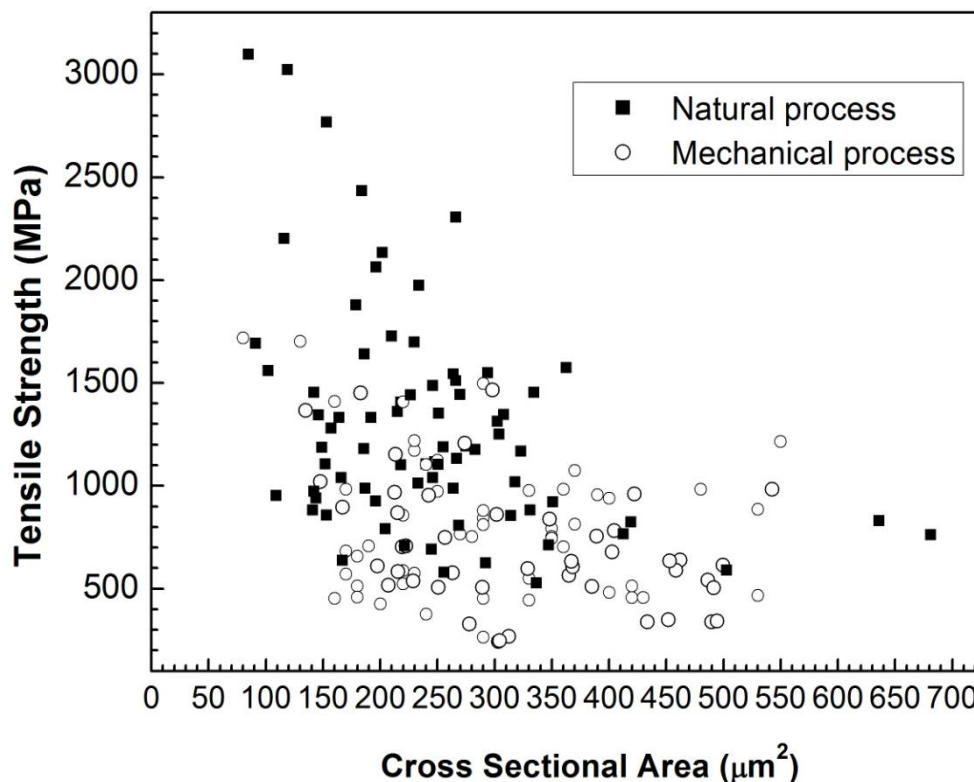
Figure 4.6. Tensile strength of single flax fibres as a function of cross sectional area for naturally and mechanically processed flax fibres.
