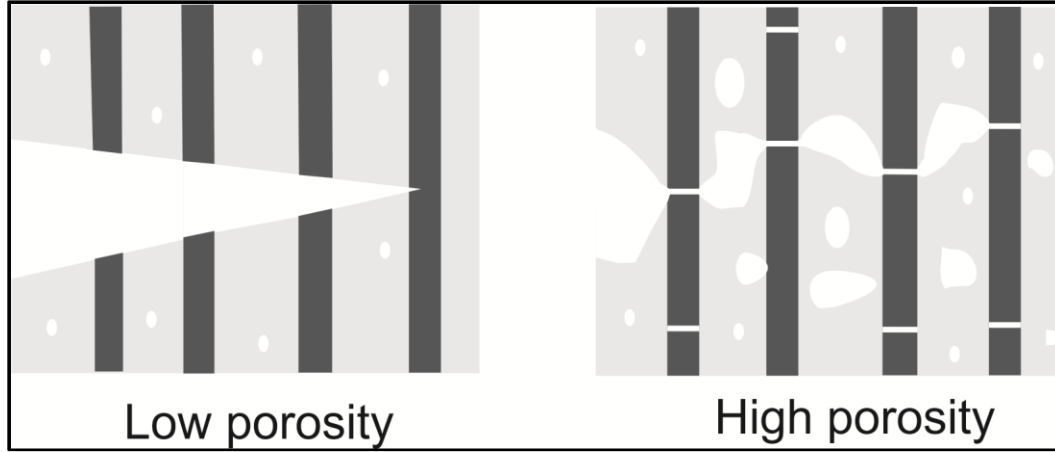
Figure 5.13. A sketch of load transfer mechanisms in low and high porous microstructure.
