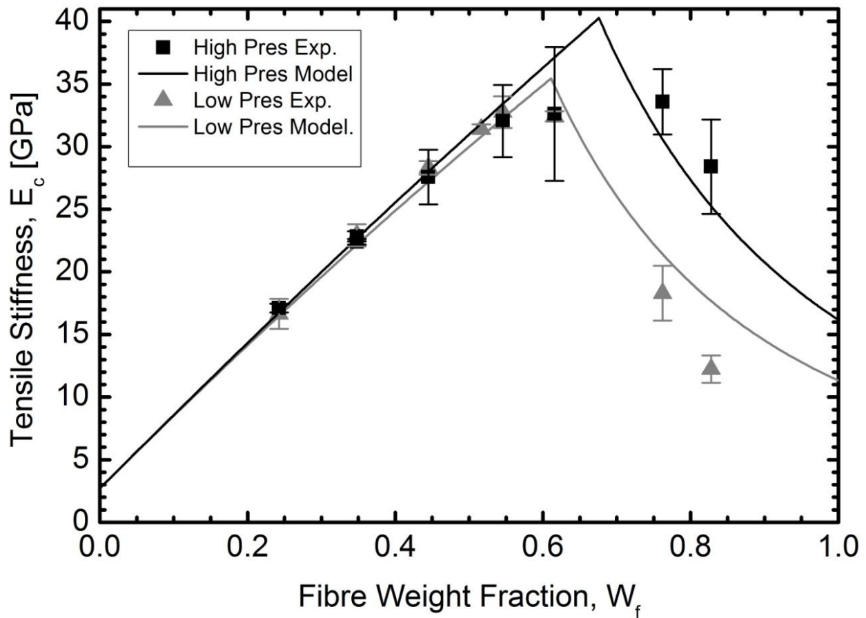
Figure 5.4. Composite stiffness as a function of the fibre weight fraction in unidirectional flax/LPET composites manufactured by a low and a high consolidation pressure.
