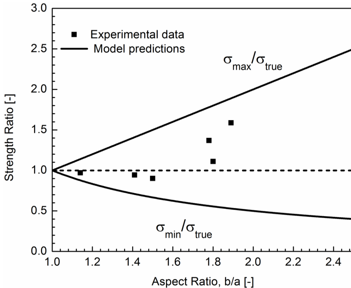
Figure 4.9. Experimental and model predictions of the tensile strength of fibres using the circular assumption method (maximum or minimum cross sectional area) and the true cross sectional method, as a function of the fibre cross sectional aspect ratio.
