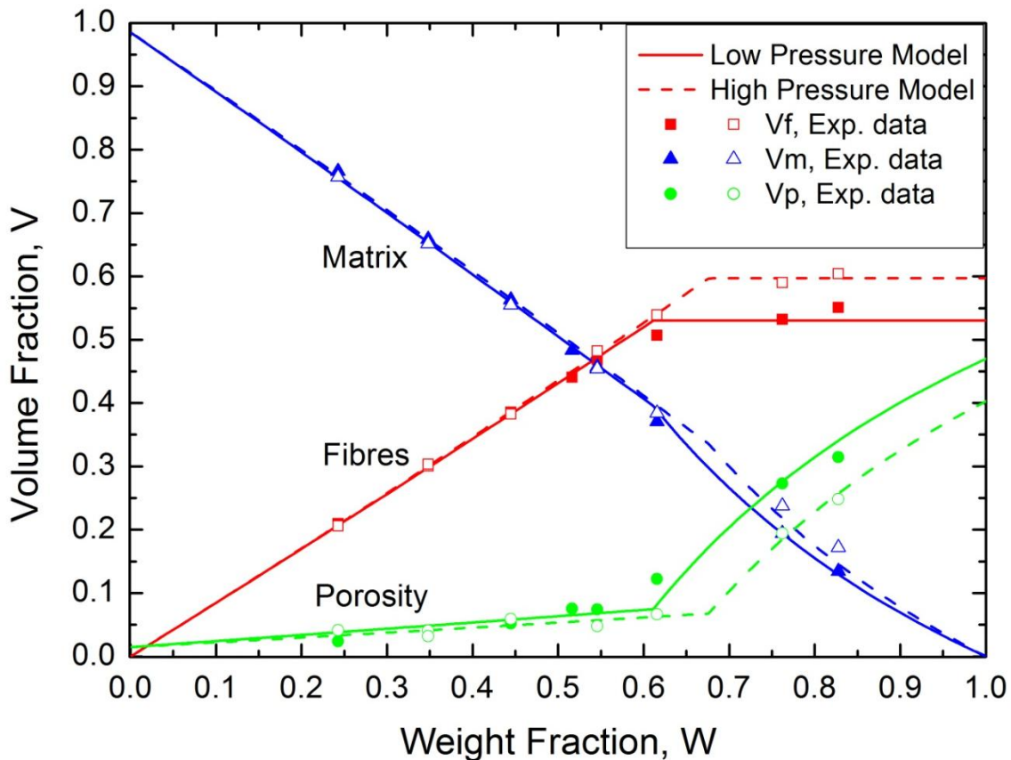
Figure 5.3. Model lines and experimental data points for volume fractions ( V_p : porosity, V_f : fibres, V_m : matrix) of flax/LPET composites shown as a function of the fibre weight fraction. Full lines and dotted lines are used for model calculations of low and high pressure composites, respectively.
