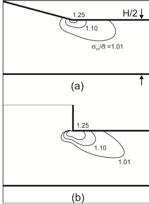
Figure 5.15. The stress distribution (a) as a function of the distance from the wedge tip of the tab and test material are presented with the axial stress \sigma_{xx} contours (b) for \theta = 15^\circ and \theta = 90^\circ .
