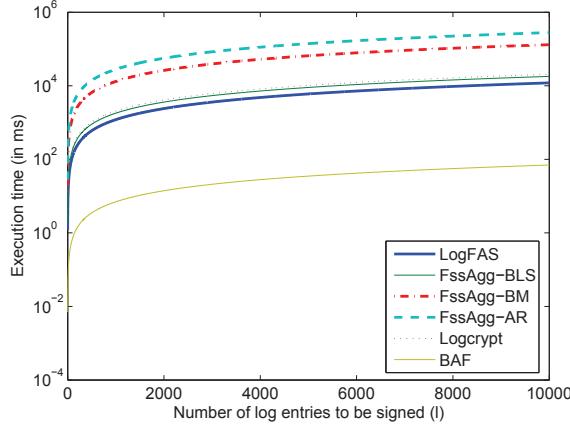
Figure 5.1: Signing time comparison of LogFAS and Figure 5.2: Verification time comparison of LogFAS and its counterparts (in ms)
