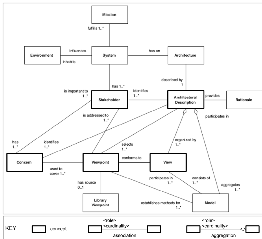
Figure 2.4: Basic concepts of architecture description (IEEE 1471 [78])
