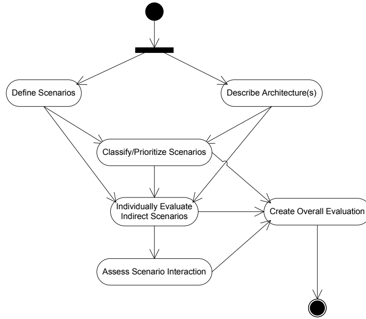
Figure 3.1: SAAM activities [19]
