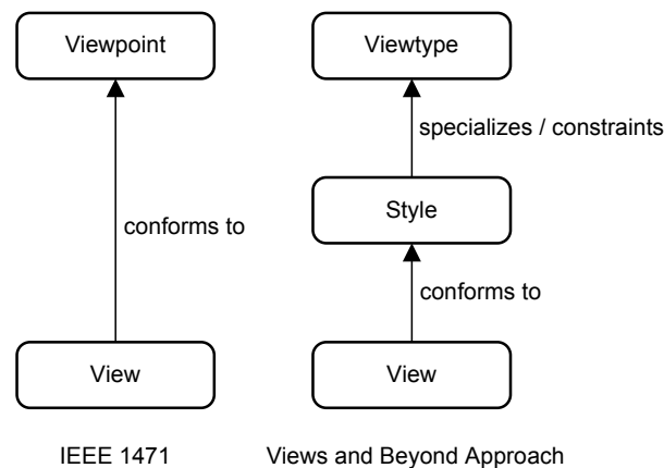
Figure 4.1: Viewpoint, view, viewpoint and style
