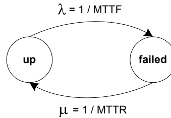
Figure 5.1: An example CTMC as a simple availability model
