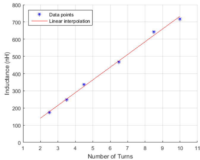
Figure 3.5. Simulated inductance values of tilted helical coils with 10 mm diameter.
