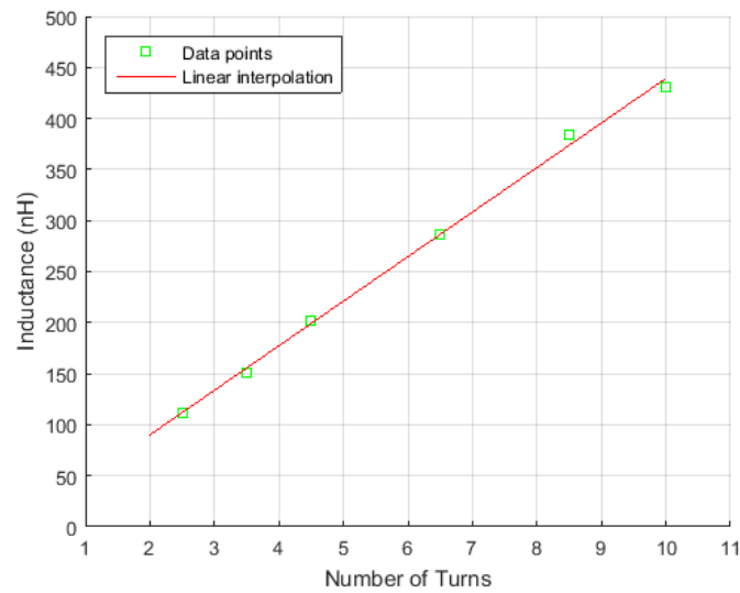
Figure 4.14. Measured inductance values for 10 mm diameter straight helical coils.
