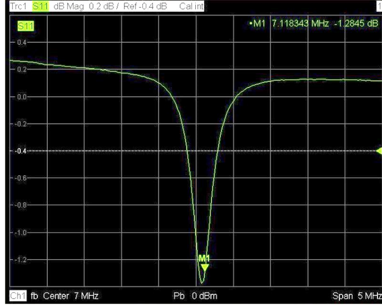
Figure 4.8. Resonance frequency caption for 8.5 turn and 10 mm diameter coil.
