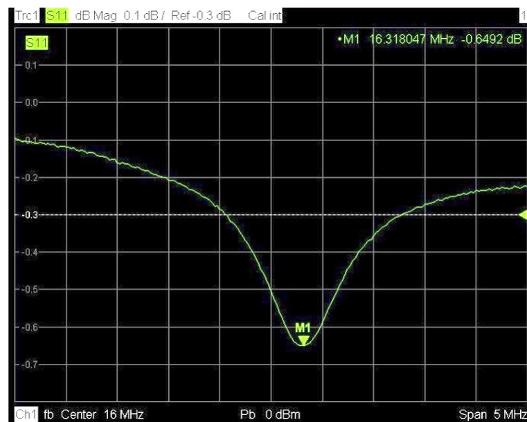
Figure 4.17. Resonance frequency caption of 6.5 turn 5 mm straight helical coil.
