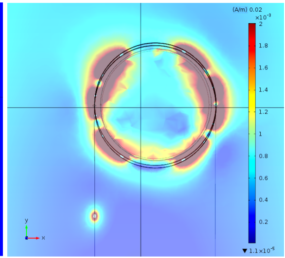
(b) Tilted coil in XY plane
