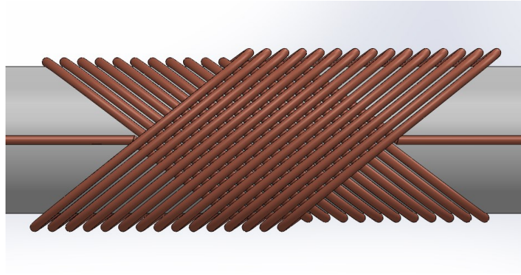
Figure 5.7. Overlap capacitor.
