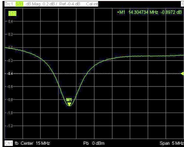
Figure 4.12. Resonance frequency caption of 6.5 turn 5 mm tilted helical coil.
