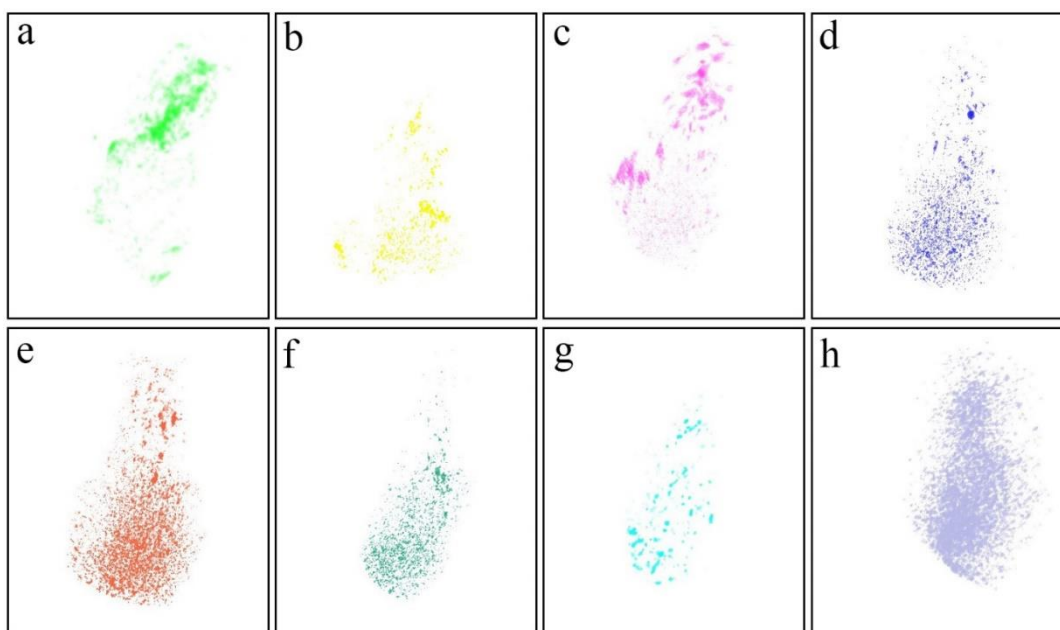
Figure 29: Images of three-dimensional reconstructions of organics and minerals. a: Si-O stretch in silicates, b: S-O stretch in sulfates, c: C-H bend in aliphatics, d: C=O stretch in carbonates, e: O-H bend in water, f: C=O stretch in carbonyls, g: C-H stretch in aliphatics, h: O-H stretch in water.
