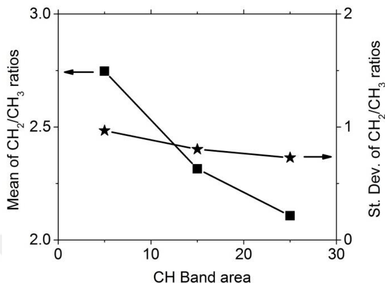
Figure 11: Mean and standard deviation of the \text{CH}_2 / \text{CH}_3 ratios.
