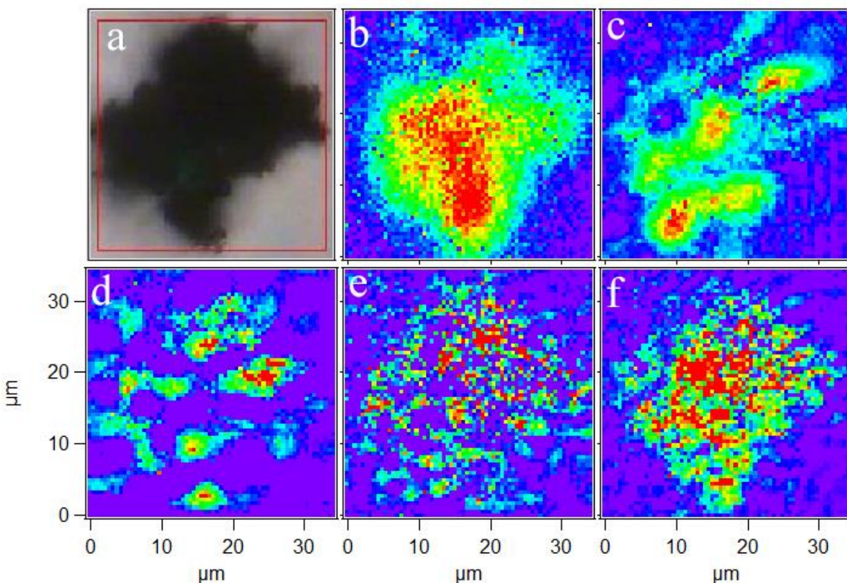
Figure 26: Spatial distributions of characteristic absorbance in SM12 grain #12: a) Visible micrograph; b) Silicates, c) Carbonates, d) \text{H}_2\text{O} + aromatic C=C stretch, e) Aliphatic C-H stretch, f) OH.
