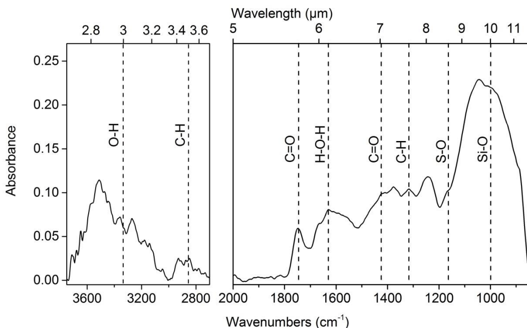
Figure 28: Infrared spectrum of the Murchison grain studied in this work. Vertical dashed lines represent positions of specific vibrational modes.
