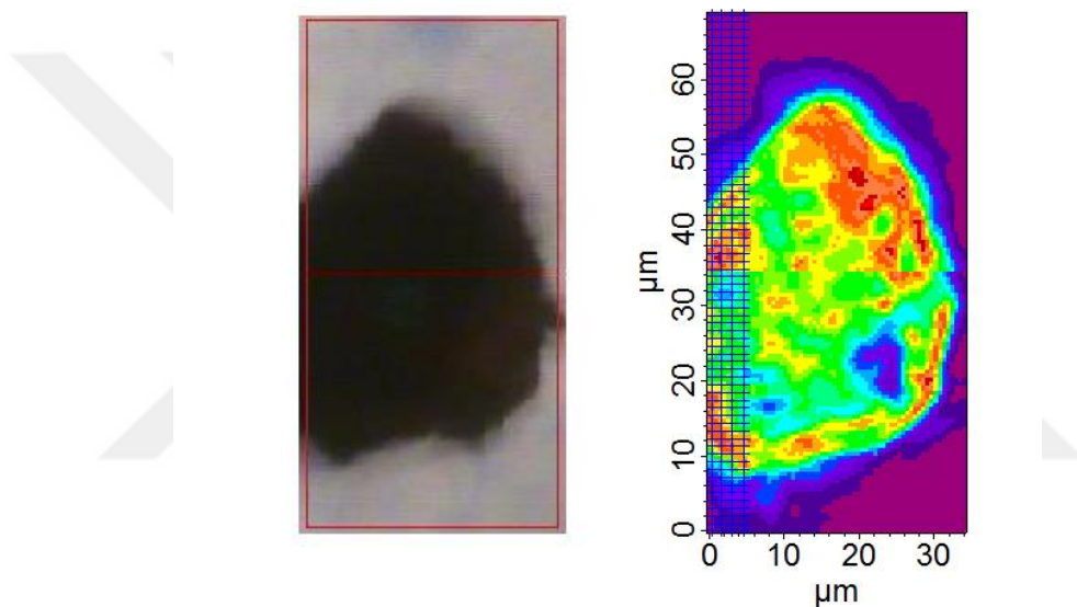
Figure 18: Visible micrograph (left), and infrared image of the Orgueil grain at 2921\text{ cm}^{-1} (right).
