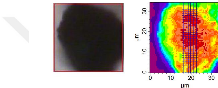
Figure 6: Visible micrograph (left), and infrared image of the NWA 852 grain at 2921\text{ cm}^{-1} (right).
