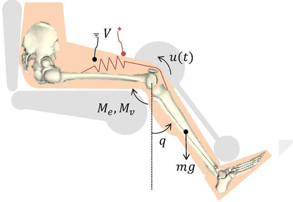
Figure 5-1. Schematic [1] of the knee-joint dynamics and the torque production about the knee caused by the voltage potential V applied to the of the quadriceps muscle group.
