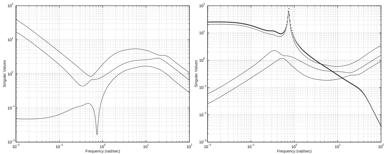
Figure 5.19: a) Actuator activity due output disturbance b) Maximum allowable additive uncertainty vs. \bar{\sigma}(G)
