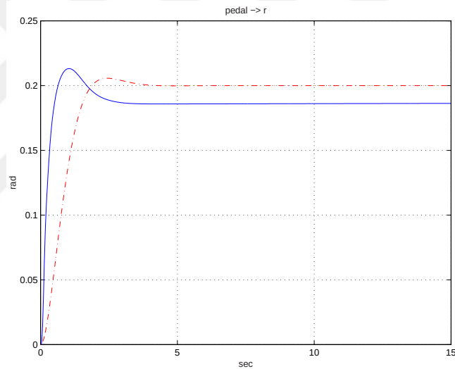
Figure 6.58: Linear response to pedal demand of 0.2 rad/sec: system response , ideal model
