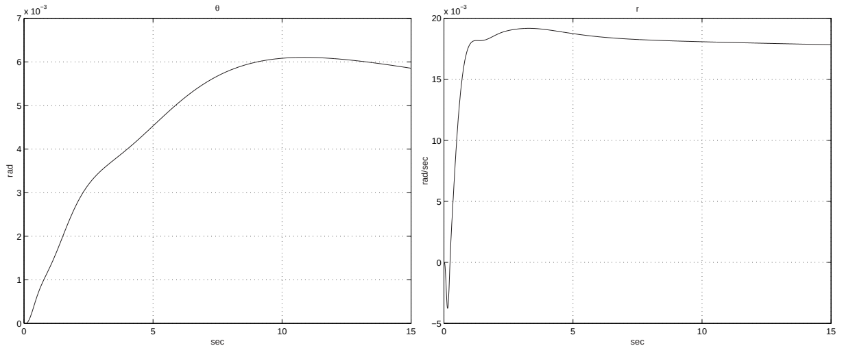
Figure 6.23: Coupling to lateral cyclic step demand of 0.2 rad
