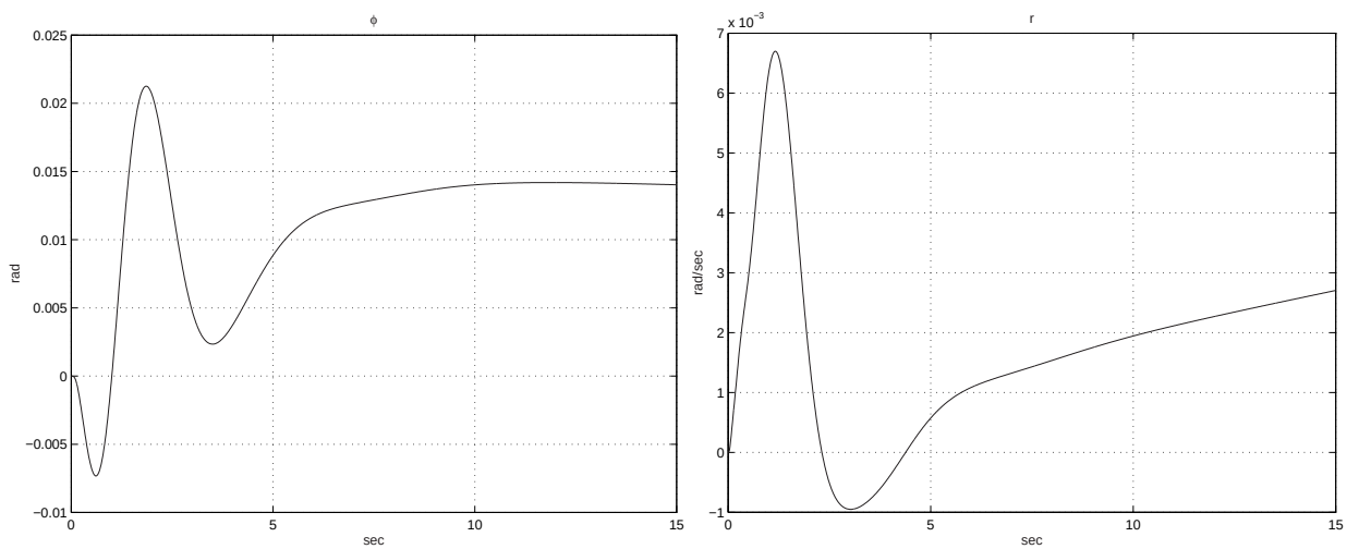
Figure 6.4: Couplings to longitudinal cyclic step demand of 0.2 rad a) \phi b) r
