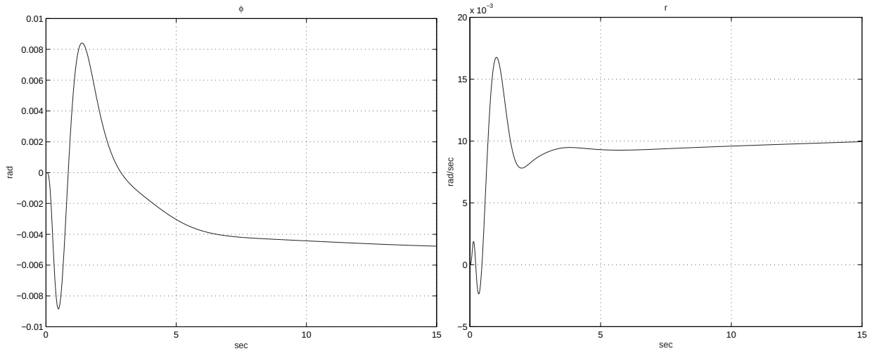
Figure 6.25: Coupling to longitudinal cyclic step demand of 0.2 rad a) \theta b) \phi
