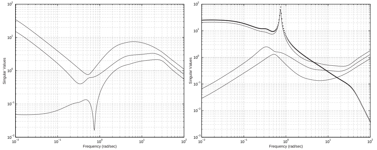
Figure 5.43: a) Actuator activity due output disturbance b) Maximum allowable additive uncertainty vs. \bar{\sigma}(\mathbf{G})
