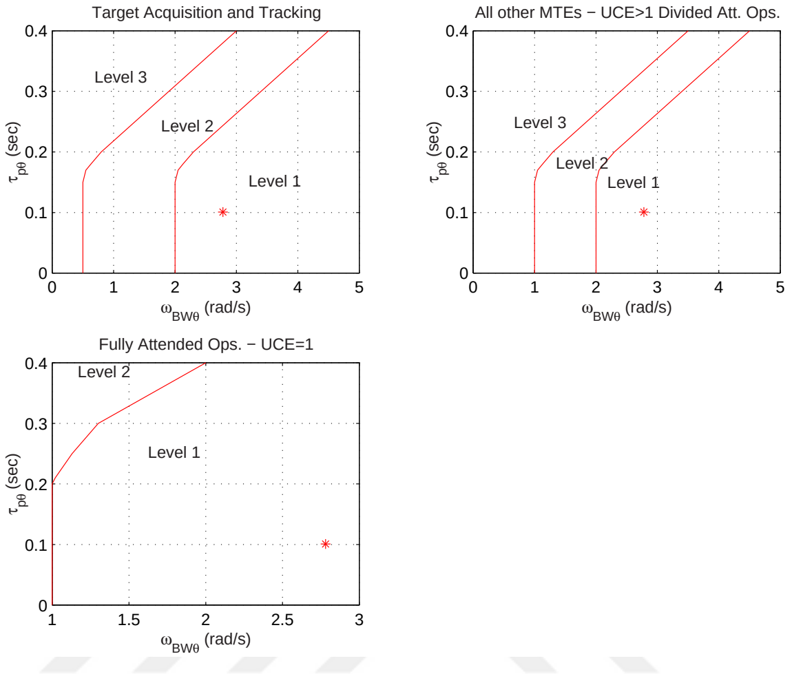
Figure 6.61: Small amplitude pitch attitude changes -hover and low speed for 2nsqDW
