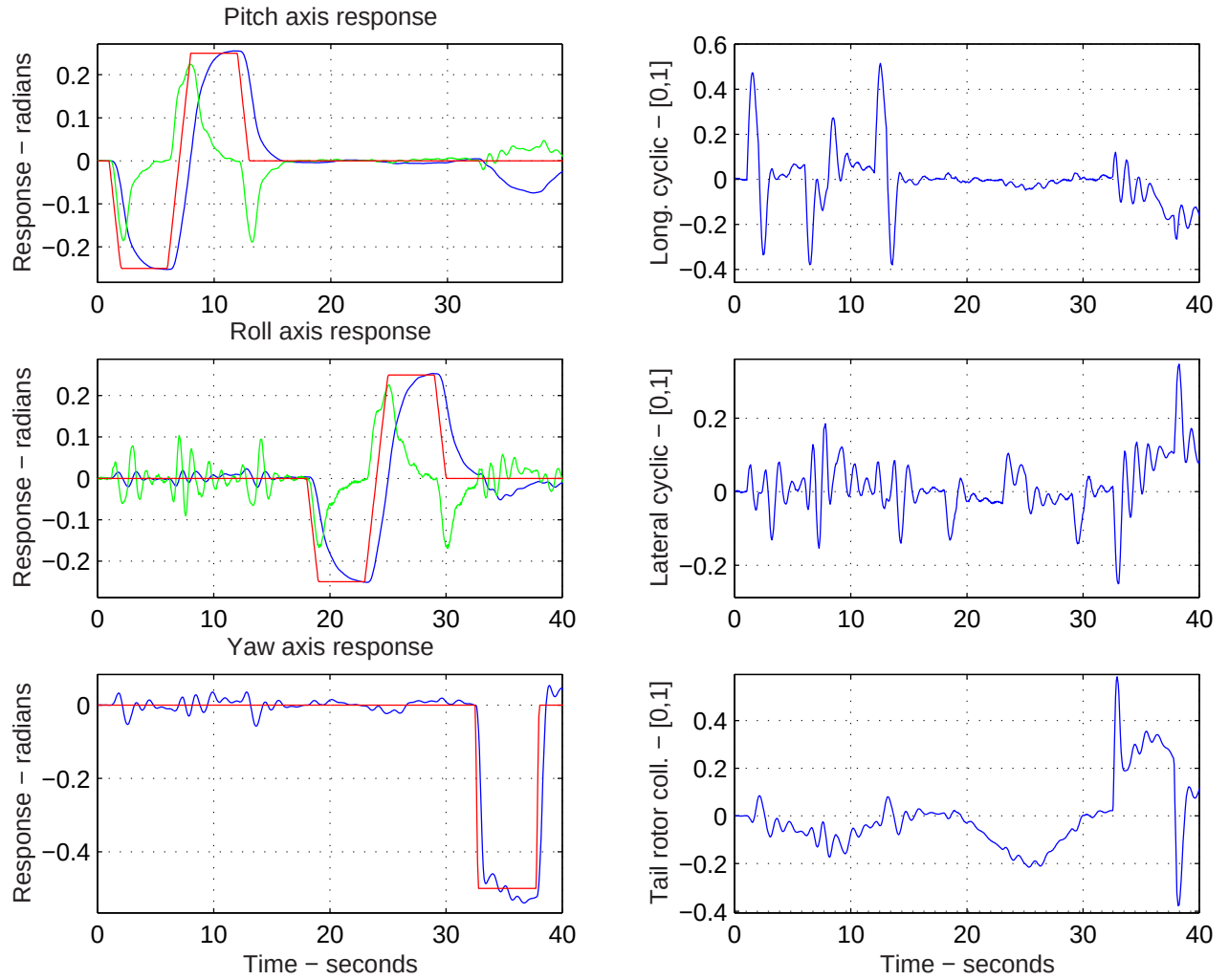
Figure 6.50: Left column- Nonlinear model: demand , rate , attitude responses; Right column: actuator activities for 1nsqNDW
