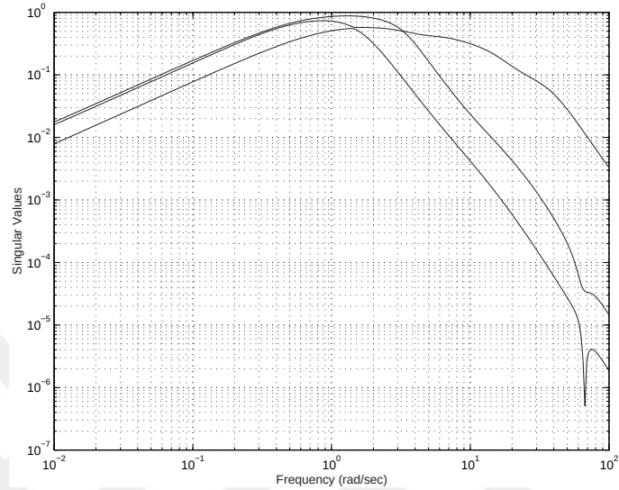
Figure 5.7: Singular values \mathbf{S}_o \mathbf{G}
