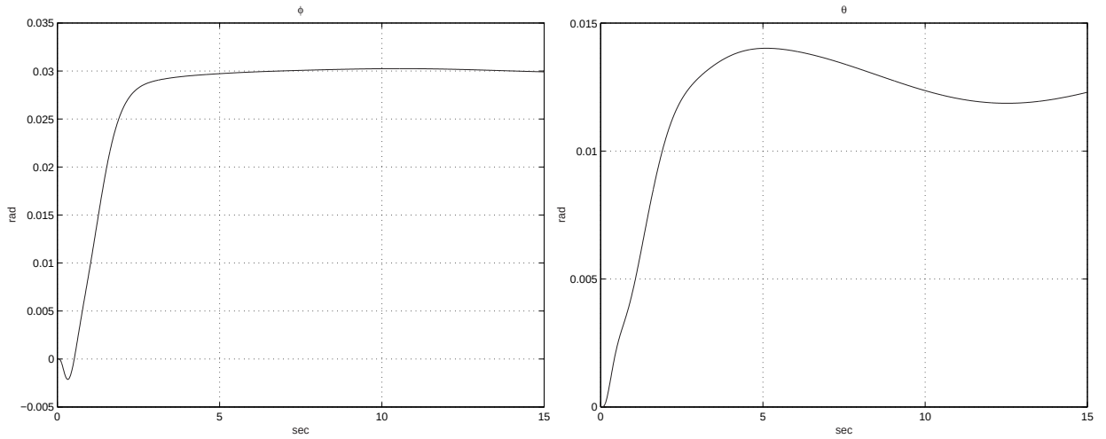
Figure 6.49: to pedal demand of 0.2 rad/sec a) \phi b) \theta
