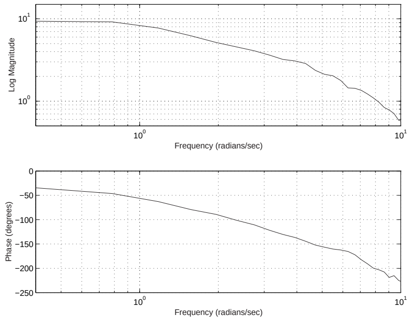
Figure 6.35: Roll axis frequency estimate
