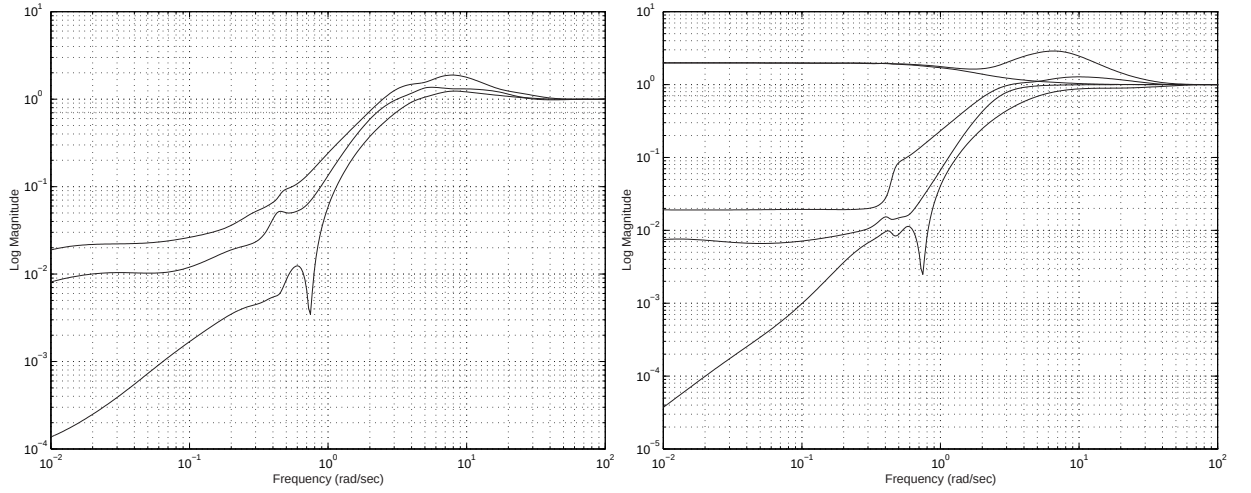
Figure 5.30: a) Input sensitivity S_i b) Output sensitivity S_o
