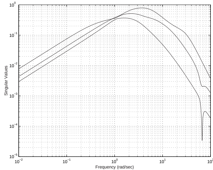
Figure 5.40: Singular values S_o G
