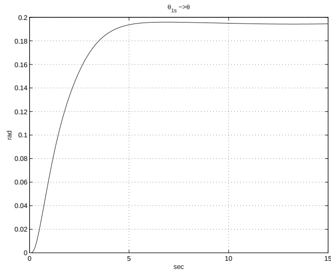
Figure 6.46: Linear response to longitudinal cyclic demand of 0.2 rad
