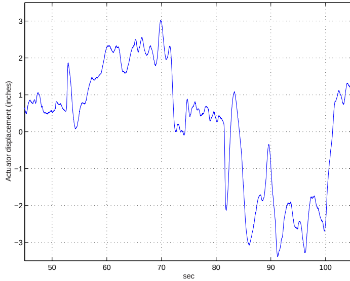
Figure 6.17: Pitch axis actuator (FDE) activity
