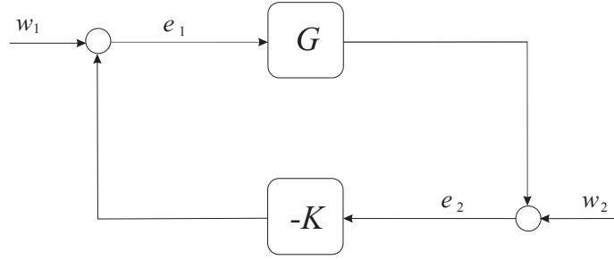
Figure 3.2: Internal stability analysis diagram
