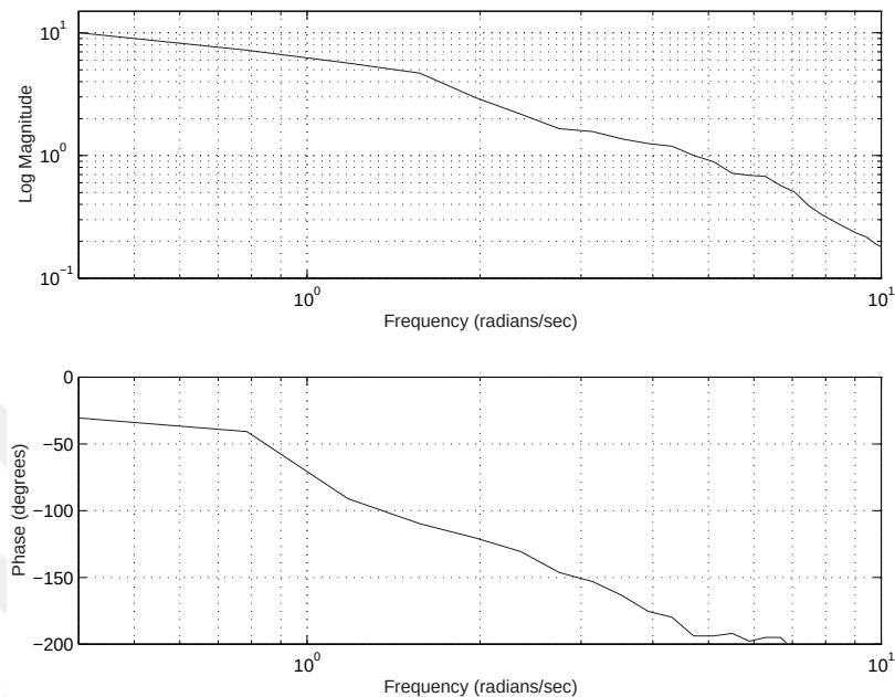
Figure 6.36: Pitch axis frequency estimate
