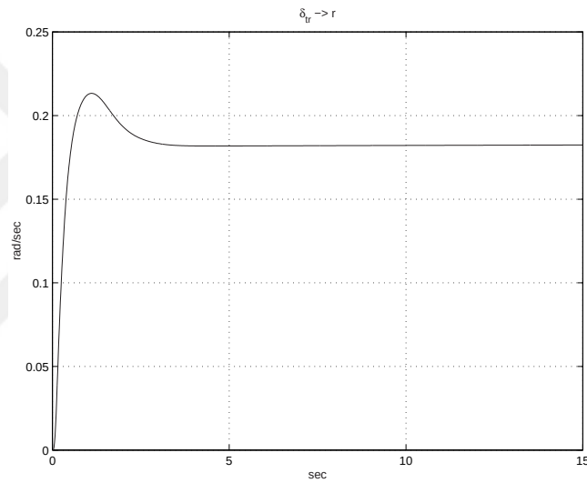
Figure 6.26: Linear response to pedal demand of 0.2 rad/sec
