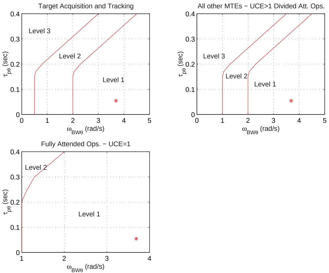
Figure 6.51: Small amplitude pitch attitude changes -hover and low speed- for 1nsqNDW
