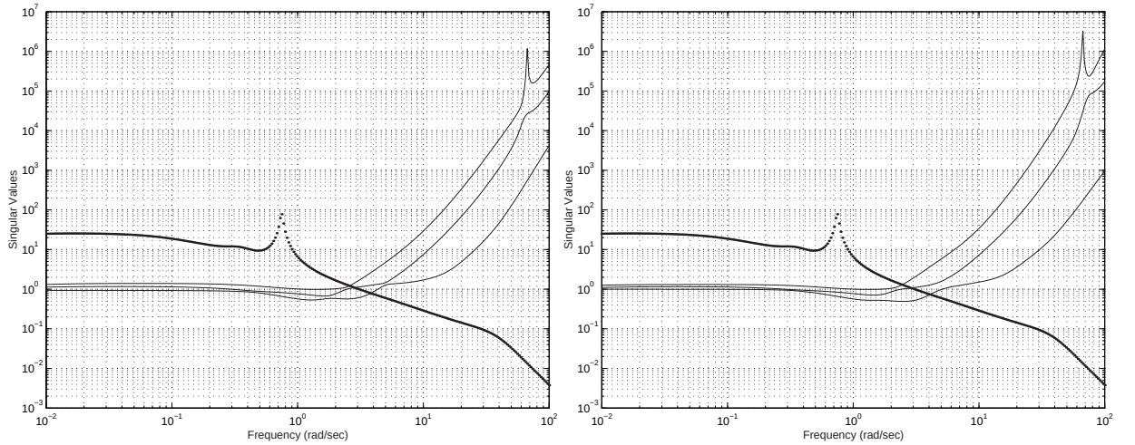
Figure 5.9: a) Inverse input co-sensitivity T_i b) Inverse output co-sensitivity T_o singular values vs. \bar{\sigma}(\mathbf{G})
