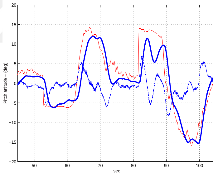
Figure 6.16: Pitch axis in-flight response: demand , solid ( \theta ), dash dot ( q ) for 1sqDW
