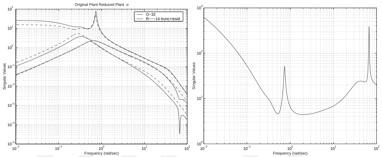
Figure 5.2: Loop shapes of a) solid- actual (32 state), dashed- reduced order plant's singular values (14 state); b) condition number
