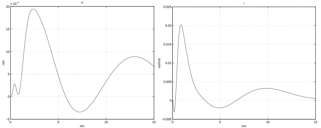
Figure 6.45: Coupling to lateral cyclic demand of 0.2 rad a) \theta b) r
