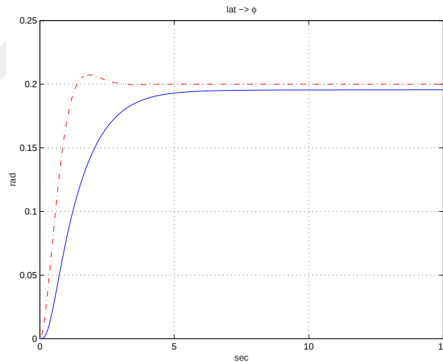
Figure 6.54: Linear responses to lateral cyclic demand of 0.2 rad: system response , ideal model
