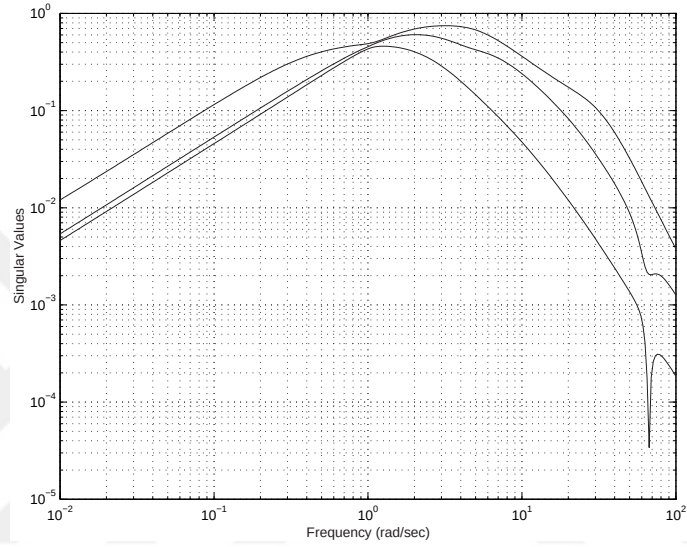
Figure 5.16: Singular values \mathbf{S}_o\mathbf{G}
