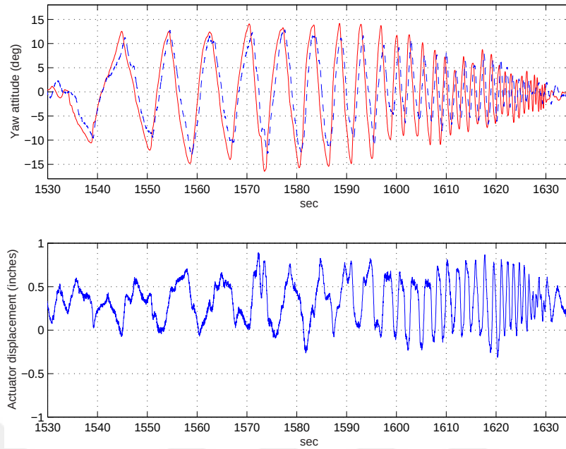
Figure 6.34: Yaw axis frequency sweep: red-(demand), dash dot-(response), solid blue-(actuator displacement) for 1sqDW
