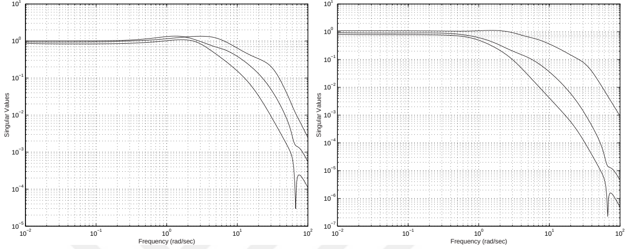
Figure 5.17: a) Input co-sensitivity T_i b) Output co-sensitivity T_o singular values
