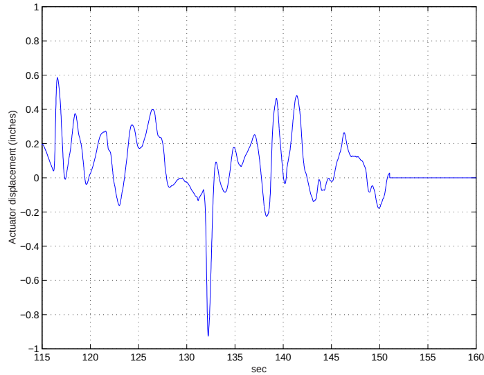
Figure 6.21: Yaw axis actuator (FDR) activity
