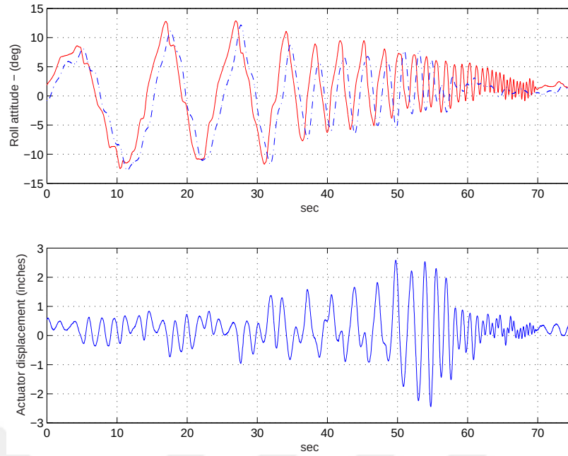
Figure 6.10: Roll axis frequency sweep: red -(demand), dash dot -(response), blue -(actuator displacement) for 1sqDW
