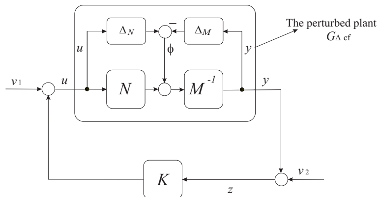
Figure 3.7: Coprime factor uncertainty
