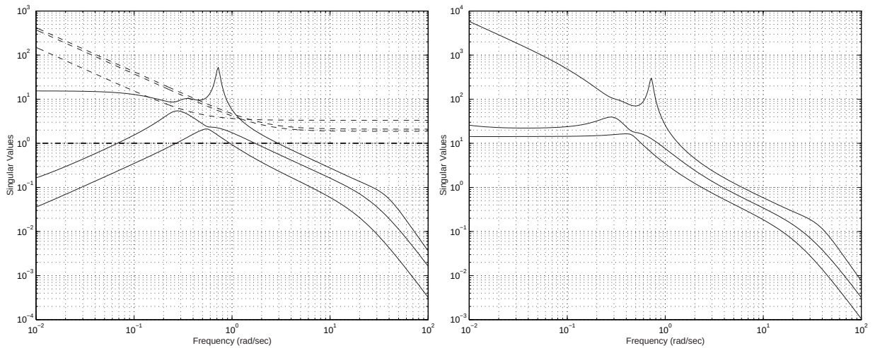
Figure 5.36: a) Nominal plant ( continuous ) and loop-shaping weights ( dashed ) b) Shaped plant
