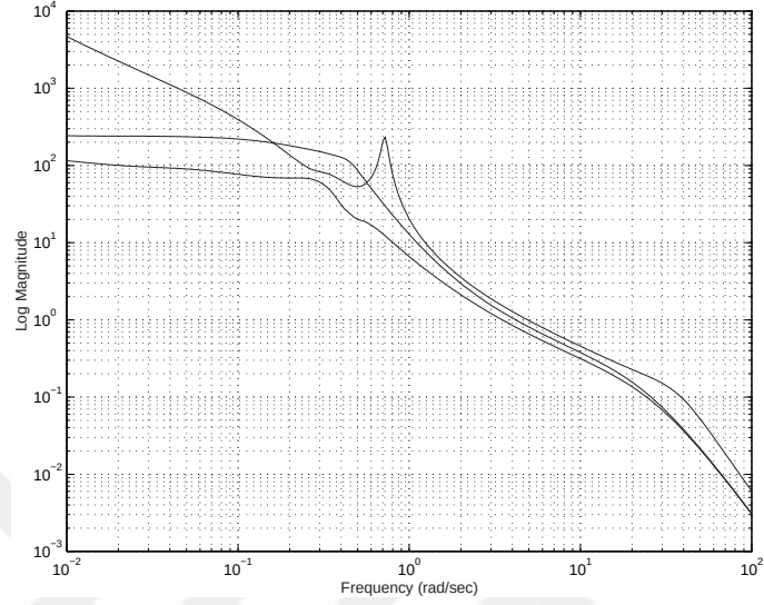
Figure 5.26: Shaped plant: with diagonal and non-diagonal loop-shaping pre-filters
