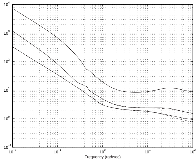
Figure 5.28: Implemented controller \mathbf{K}_{imp} : original ( continuous ) vs. reduced ( dashed ) order plant input where the non-diagonal weight was applied. Additionally, when considered together with the other control laws' \mathbf{L}_i and \mathbf{L}_o vs. \mathbf{G}_s characteristics it brings to evidence that unless dynamic (diagonal or non-diagonal) weighting is applied at the plant output the significant mismatch observed between desired and actual loop-shapes cannot be eliminated.
