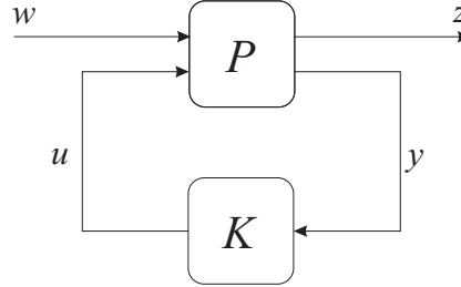
Figure 3.9: Synthesis Framework-LLFT
