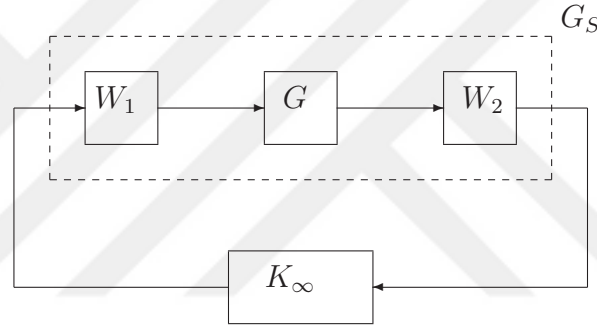
Figure 4.7: Shaped Plant \mathbf{G}_s in the Loop-shaping approach
