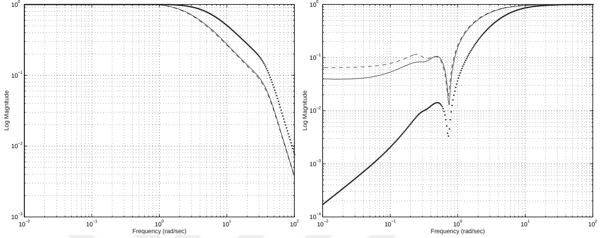
Figure 5.20: a) \bar{\sigma}(\mathbf{N}_s) b) \bar{\sigma}(\mathbf{M}_s) of shaped (dotted), nominal (continuous), reduced (dashed) plant
