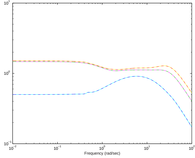
Figure 5.27: Loop shaping controller \mathbf{K}_\infty
