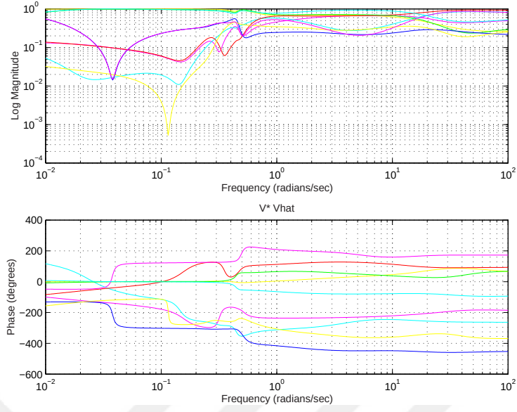
Figure 5.22: Frequency response of (V \cdot \hat{V}_{red})
