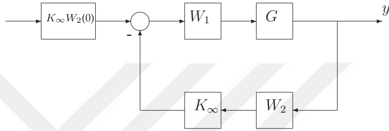
Figure 4.11: Unity Feedback for Loop Shaping
