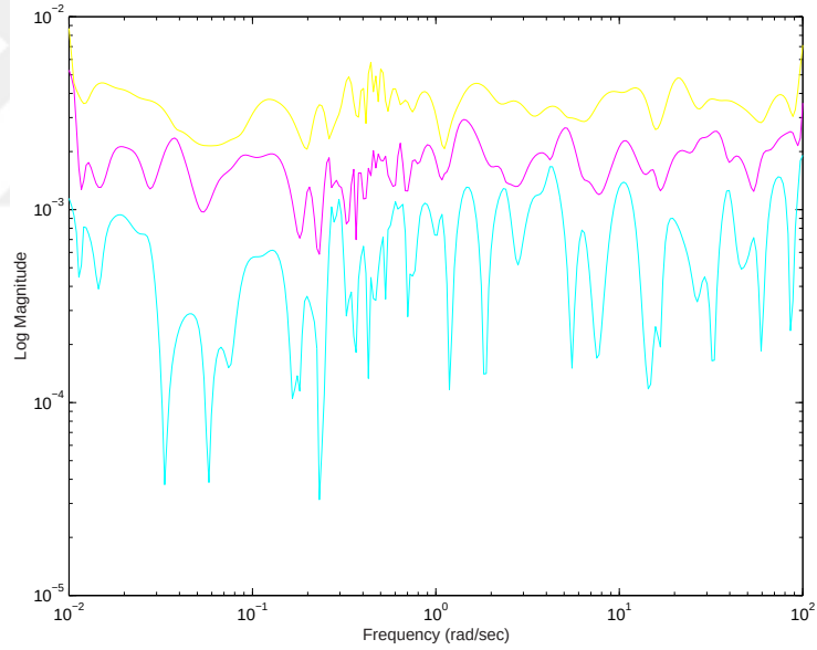
Figure 5.23: \bar{\sigma}(V - \hat{V}_{red})
