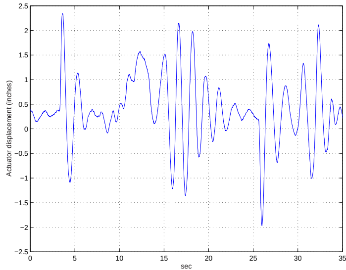
Figure 6.19: Roll axis actuator (FDA) activity
