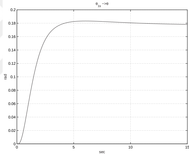
Figure 6.24: Linear response to longitudinal cyclic step demand of 0.2 rad
