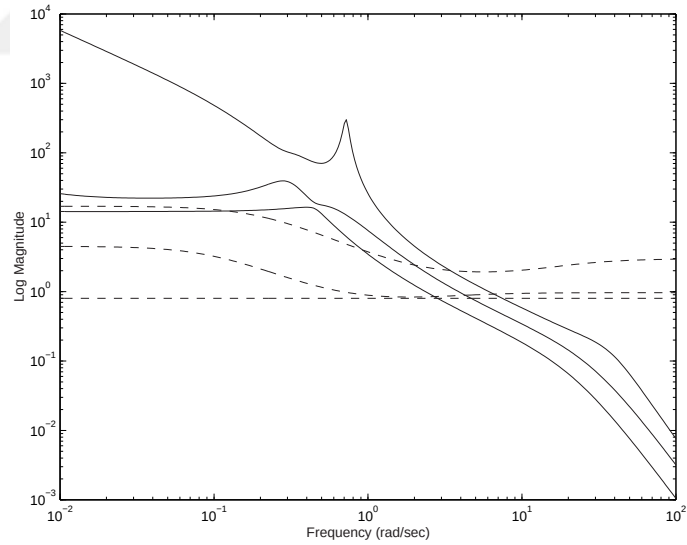
Figure 5.25: Diagonally weighted plant vs tentative non-diagonal weights
