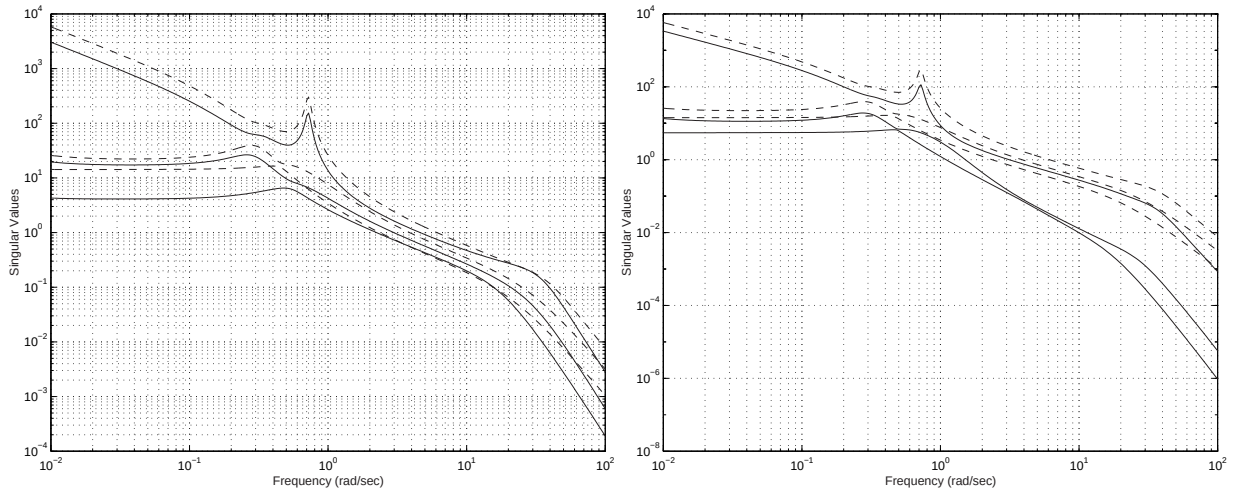
Figure 5.38: Shaped ( dashed ) vs. actual ( solid ) loop- shapes at: a) the plant input \mathbf{L}_i b) the plant output \mathbf{L}_o for 2nsqDW
