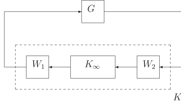
Figure 4.8: Final Controller
