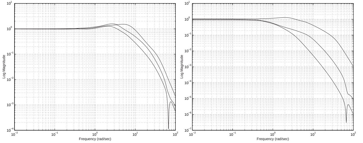
Figure 5.32: a) Input co-sensitivity T_i b) Output co-sensitivity T_o
