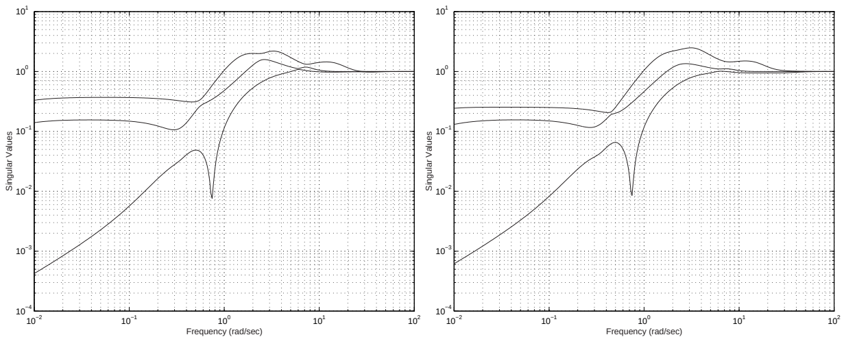
Figure 5.6: a) Input sensitivity S_i b) Output sensitivity S_o singular values
