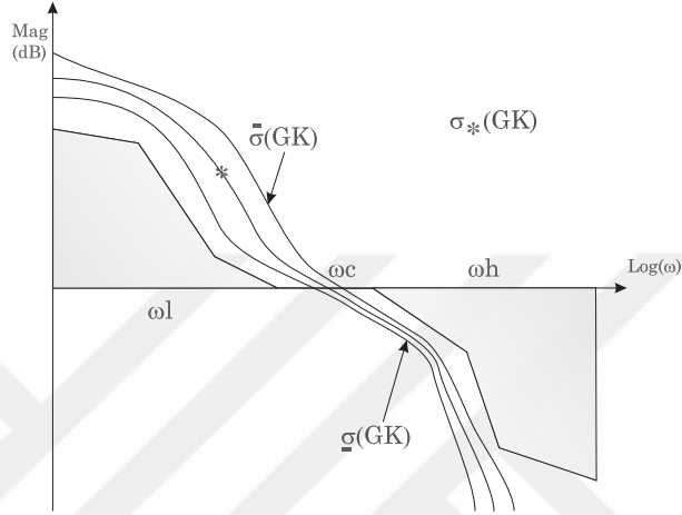
Figure 4.1: Desired Open Loop Singular Values
