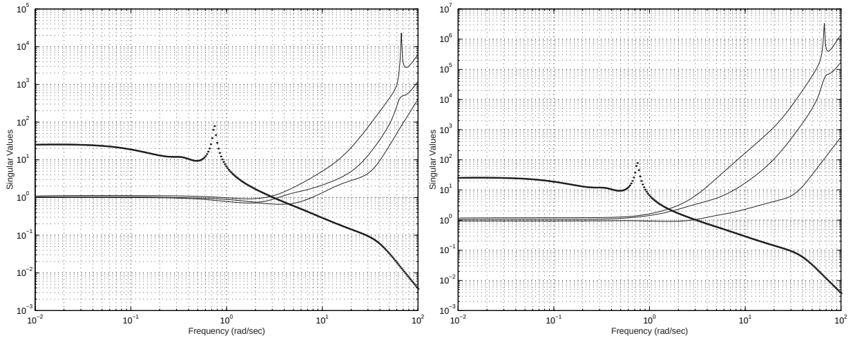
Figure 5.42: a) Inverse input co-sensitivity T_i vs. \bar{\sigma}(\mathbf{G}) b) Inverse output co-sensitivity T_o singular values vs. \bar{\sigma}(\mathbf{G})
