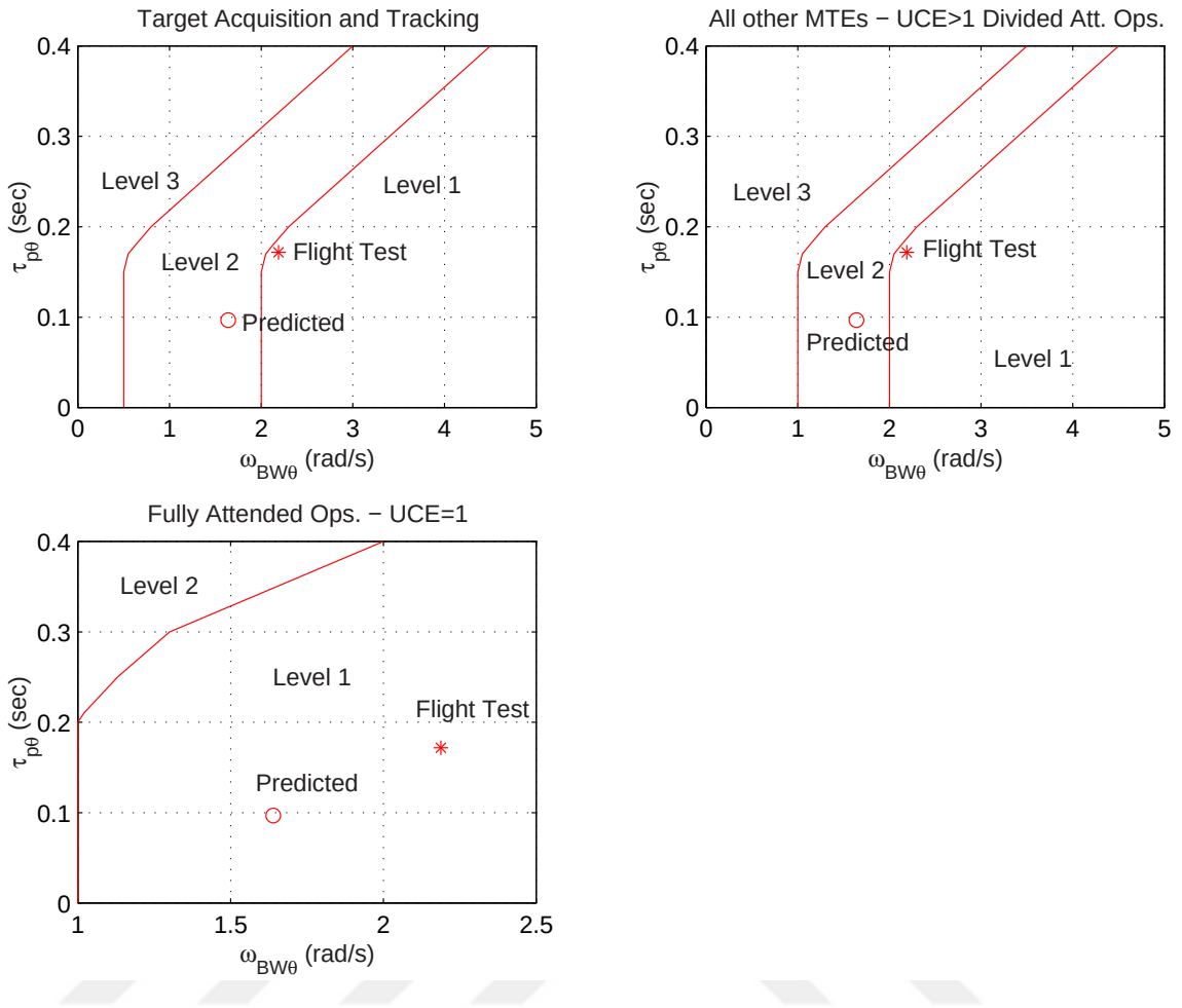
Figure 6.8: Small amplitude pitch attitude changes -hover and low speed-1sqDW
