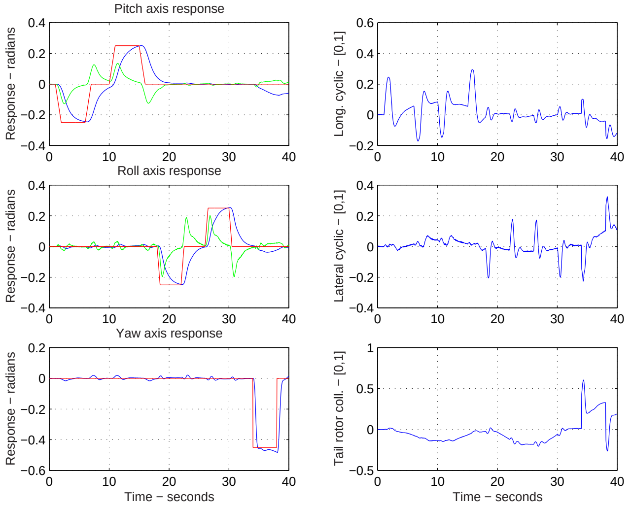
Figure 6.28: Left column- Nonlinear model: demand , rate , attitude responses; Right column: actuator activities for 1nsqDW
