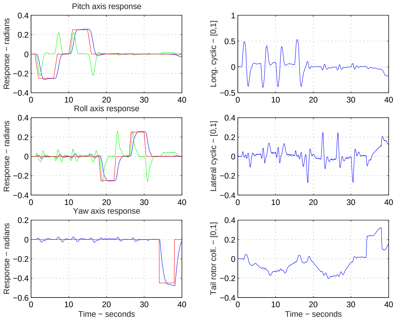
Figure 6.60: Nonlinear attitude responses, rates and actuator activities for 2nsqDW
