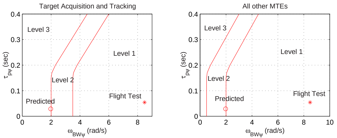
Figure 6.31: Small amplitude heading changes -hover and low speed- for 1nsqDW
