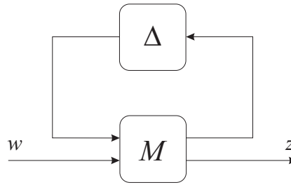
Figure 3.10: Analysis Framework-ULFT
