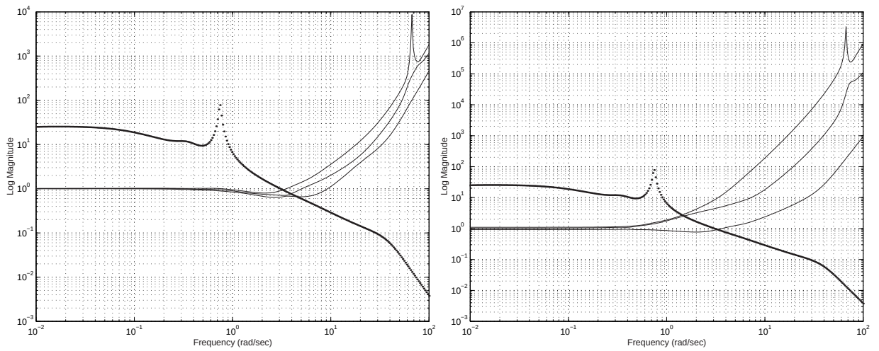
Figure 5.33: a) Inverse input co-sensitivity T_i vs. \bar{\sigma}(G) b) Inverse output co-sensitivity T_o singular values vs. \bar{\sigma}(G)
