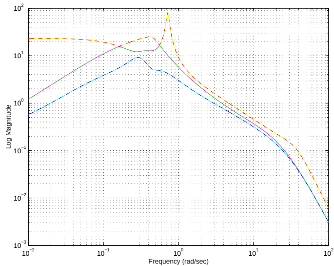
Figure 5.21: Plant augmented with integrators free pre-filter
