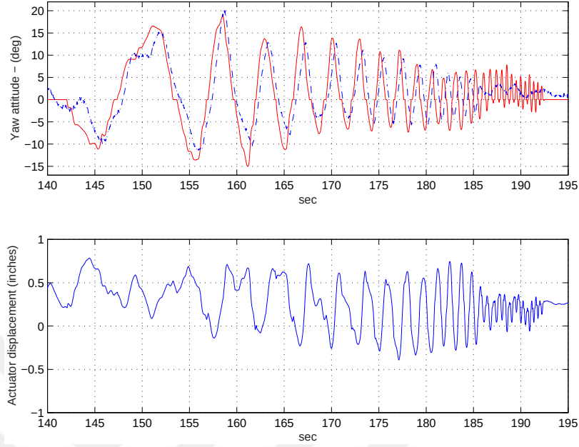
Figure 6.12: Yaw axis frequency sweep: red -(demand), dash dot -(response), blue -(actuator displacement) for 1sqDW
