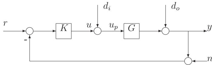
Figure 3.1: General Feedback Configuration
