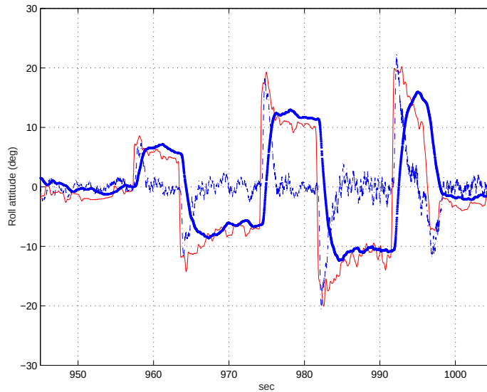
Figure 6.40: Roll axis in-flight response: demand ; solid (\phi) ; dash dot (p) for 1sqDW
