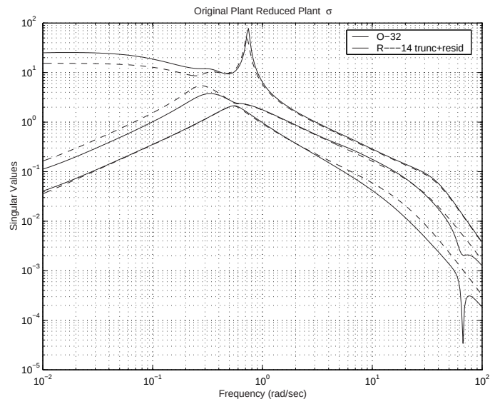
Figure 4.3: Shapes of actual (32 state) and reduced order (14 states) plant’s singular values; (continuous line-actual), (dashed line- reduced)
