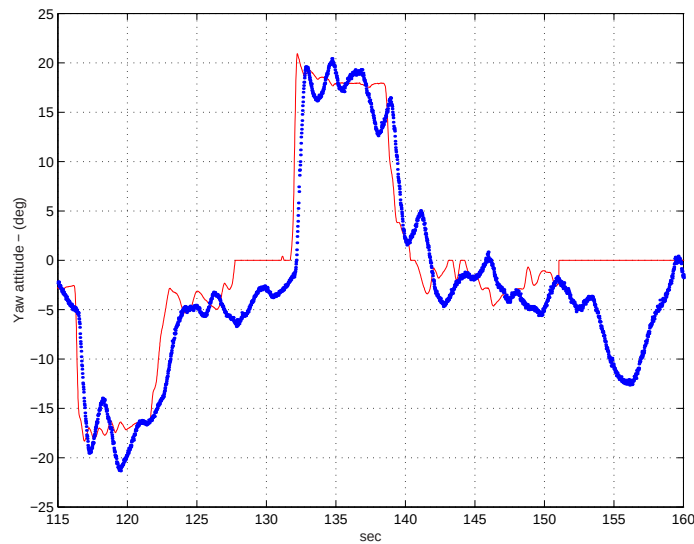
Figure 6.20: Yaw axis in-flight response: demand ; response for 1sqDW
