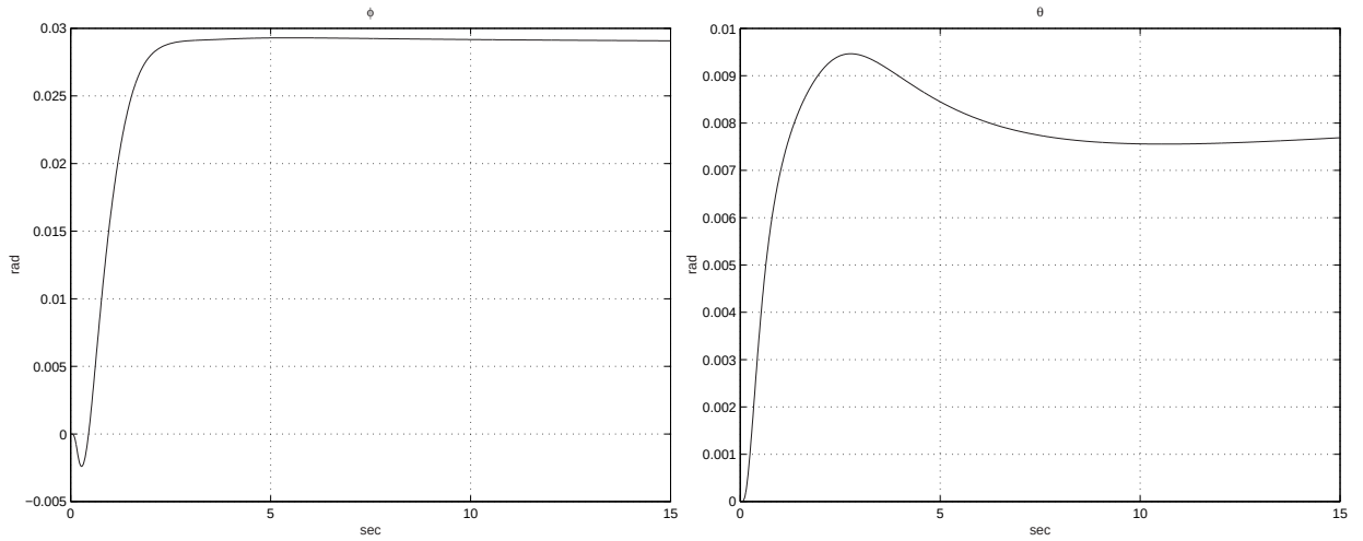
Figure 6.59: Coupling to pedal demand of 0.2 rad/sec a) \phi b) \theta
