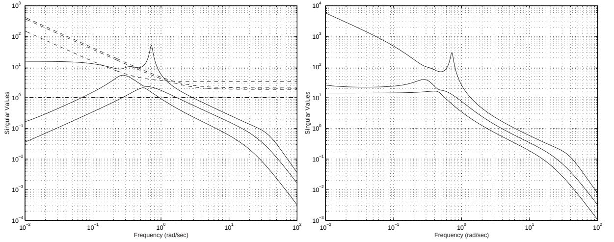
Figure 5.12: a) Nominal plant ( continuous ) and loop-shaping weights ( dashed ) b) Shaped plant
