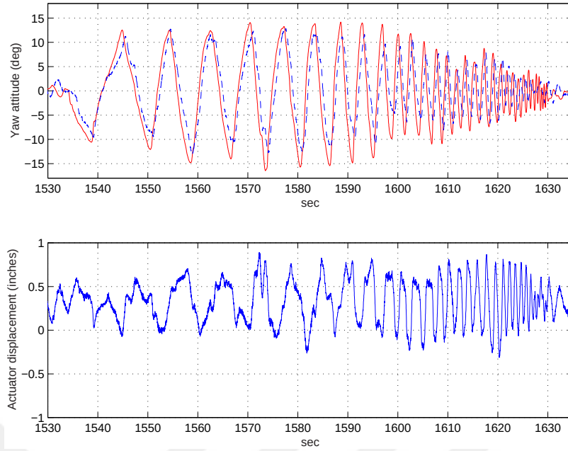
Figure A.1: Yaw axis sweep- top subplot: demand , response ; bottom subplot: actuator displacement
