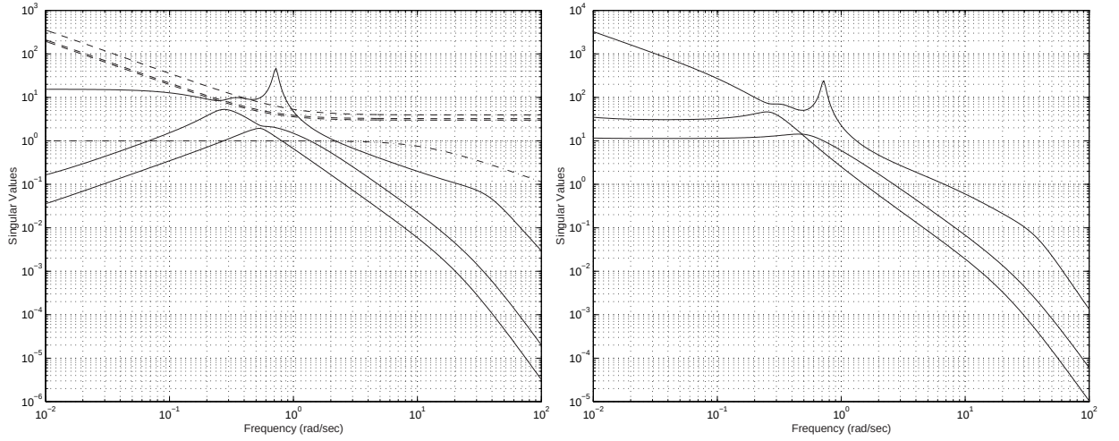
Figure 5.3: a) Nominal plant ( continuous ) and loop-shaping weights ( dashed ) b) Shaped plant
