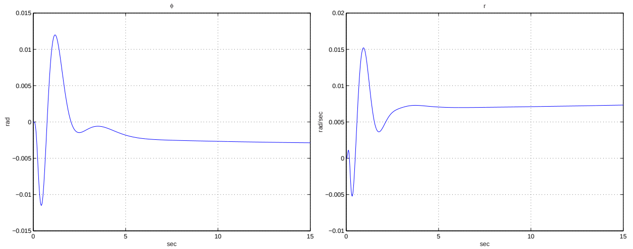
Figure 6.57: Coupling to longitudinal cyclic demand of 0.2 rad a) \phi b) r
