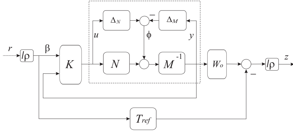
Figure 4.9: Two Degree-of-freedom design architecture
