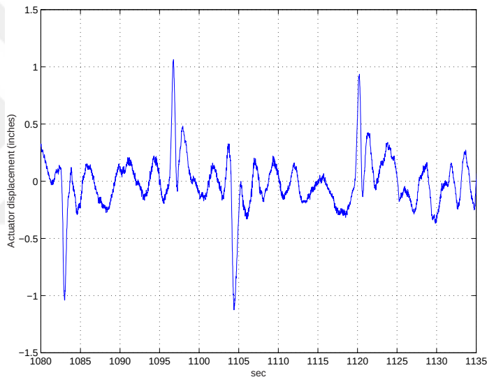
Figure 6.42: Yaw axis in-flight response: demand ; response for 1nsqDW
