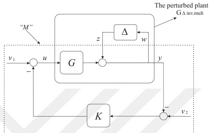
Figure 3.6: Inverse Multiplicative Uncertainty
