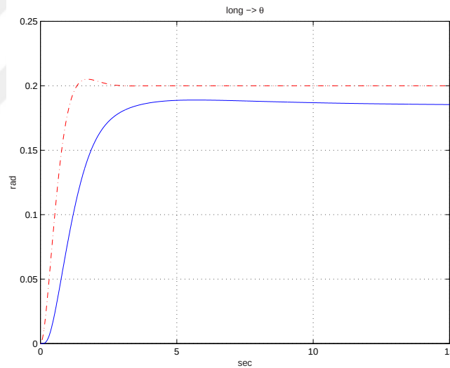
Figure 6.56: Linear response to longitudinal cyclic demand of 0.2 rad: system response , ideal model
