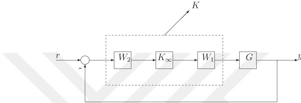
Figure 4.6: Unity Feedback for Loop-shaping
