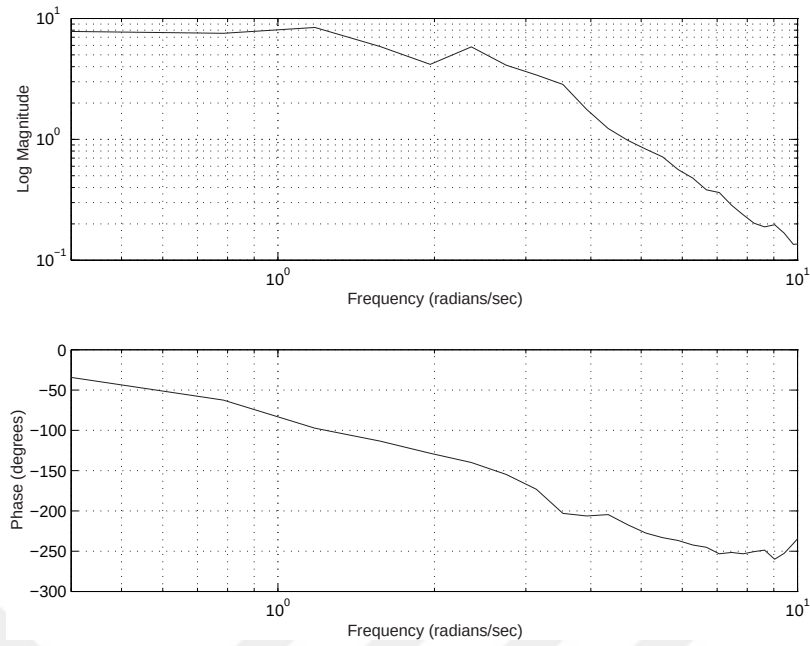
Figure 6.14: Pitch axis frequency estimate for 1sqDW
