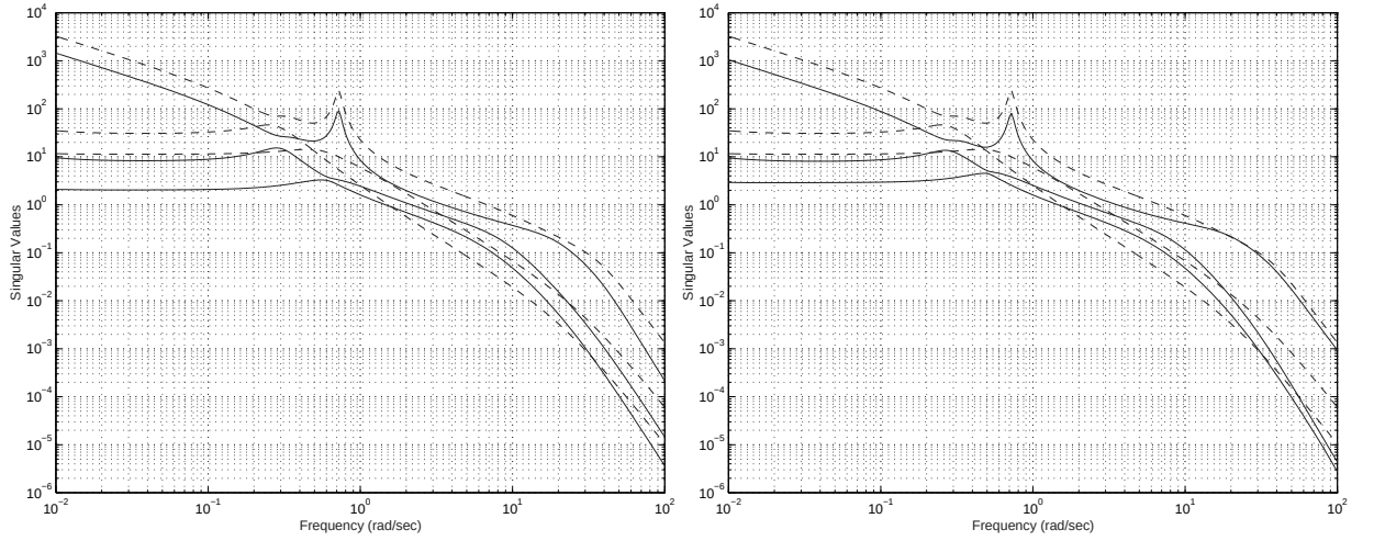
Figure 5.5: Shaped ( dashed ) vs. actual ( solid ) loop shapes: a) at the plant input L_i b) at the plant output L_o
