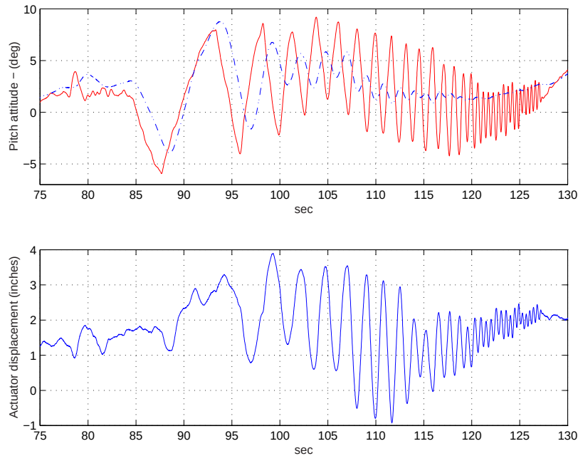
Figure 6.11: Pitch axis frequency sweep: red -(demand), dash dot -(response), blue -(actuator displacement) for 1sqDW
