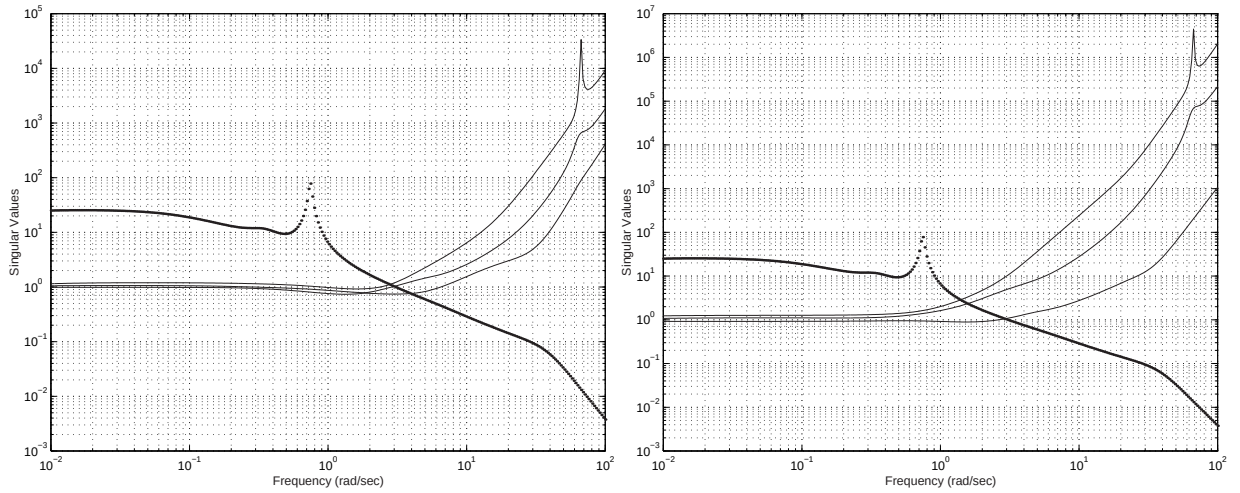
Figure 5.18: a) Inverse input co-sensitivity T_i b) Inverse output co-sensitivity T_o singular values vs. \bar{\sigma}(G)
