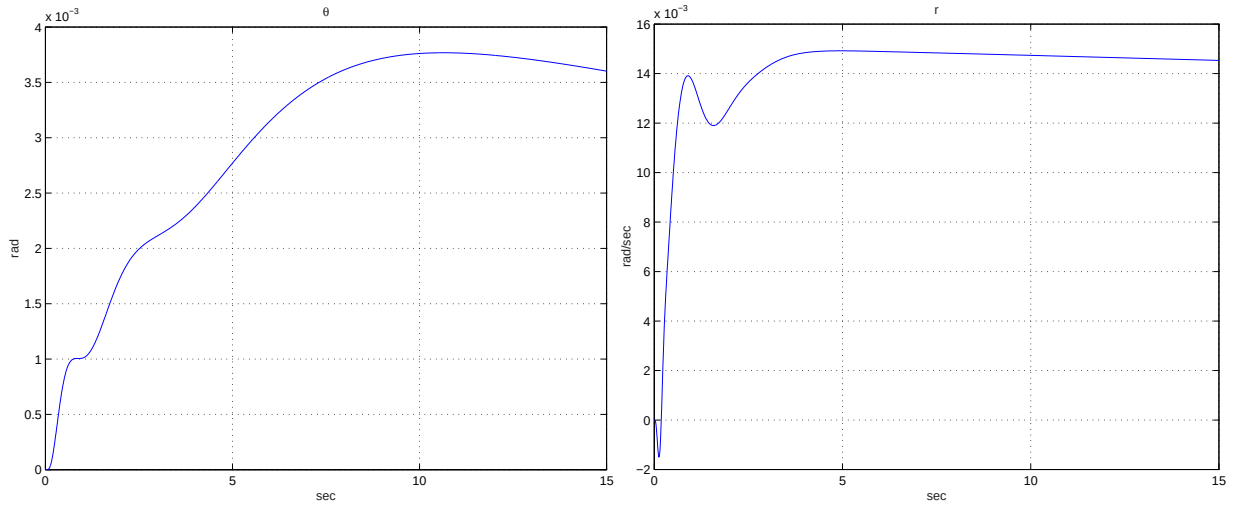
Figure 6.55: Coupling to lateral cyclic demand of 0.2 rad a) \theta b) r
