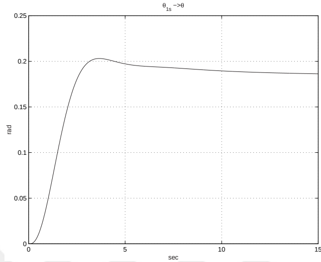
Figure 6.3: Linear response to longitudinal cyclic step demand of 0.2 rad
