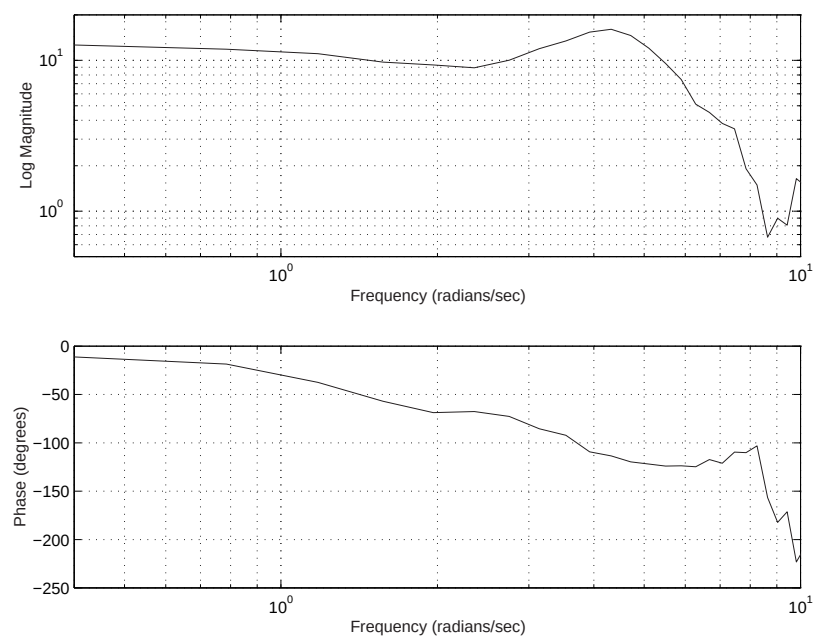
Figure 6.37: Yaw axis frequency estimate
