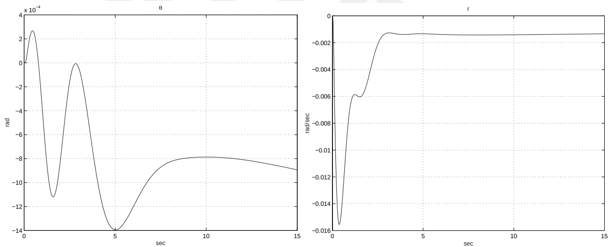
Figure 6.2: Couplings to lateral cyclic step demand of 0.2 rad a) \theta b) r
