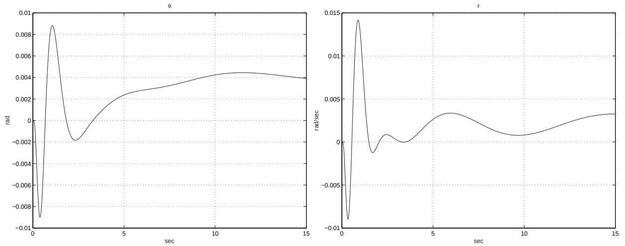
Figure 6.47: Coupling to longitudinal cyclic demand of 0.2 rad a) \theta b) \phi
