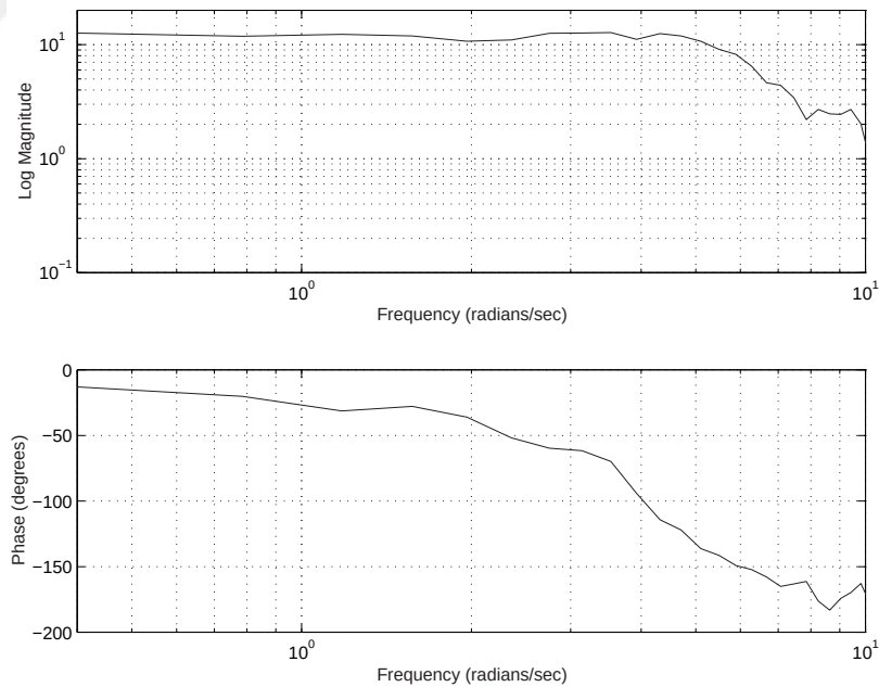
Figure 6.15: Yaw axis frequency estimate for 1sqDW
