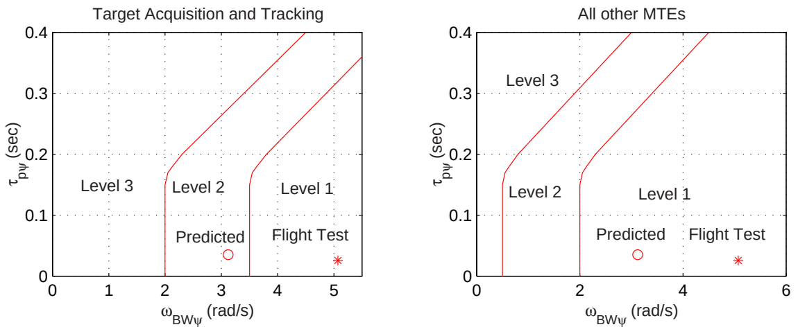
Figure 6.9: Small amplitude heading changes -hover and low speed-1sqDW
