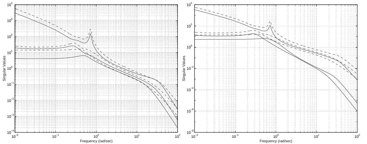
Figure 5.14: Shaped ( dashed ) vs. actual ( solid ) loop shapes: a) at the plant input \mathbf{L}_i b) at the plant output \mathbf{L}_o
