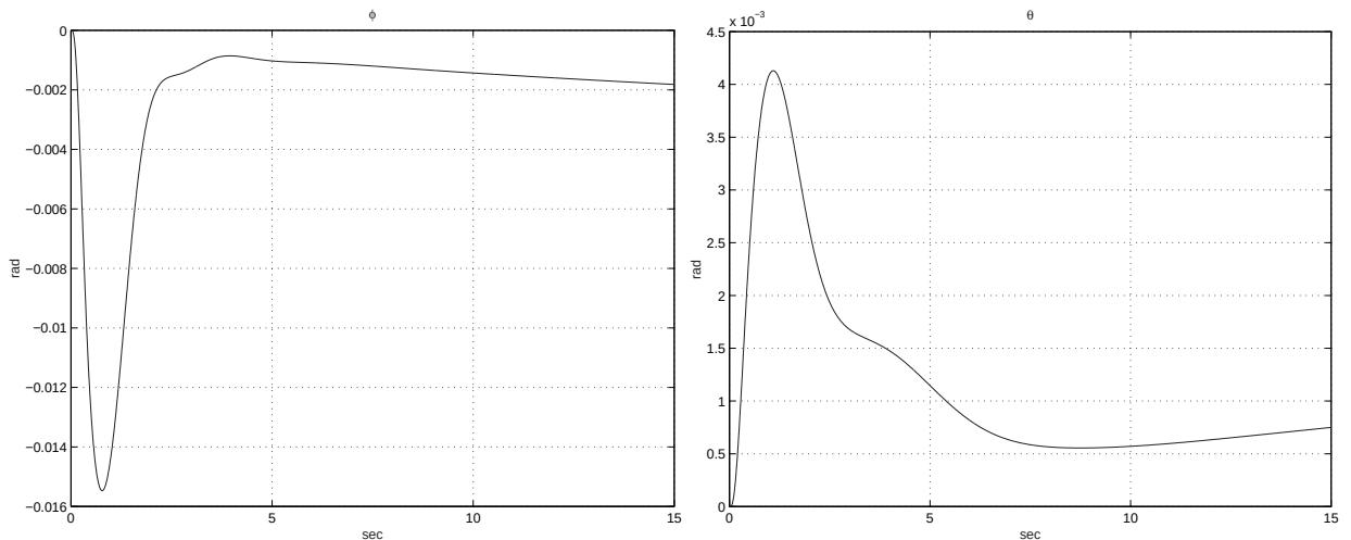
Figure 6.6: Coupling to pedal demand of 0.2 rad/sec a) \phi b) \theta
