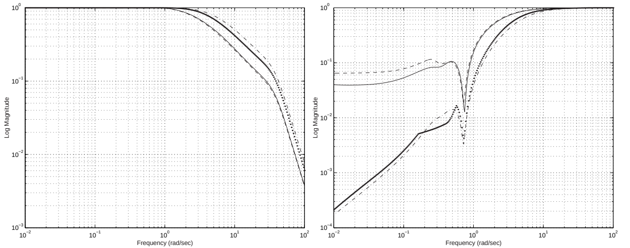
Figure 5.35: a) \bar{\sigma}(\mathbf{N}_s) b) \bar{\sigma}(\mathbf{M}_s) of shaped (dotted), nominal (continuous), reduced (dashed) plant
