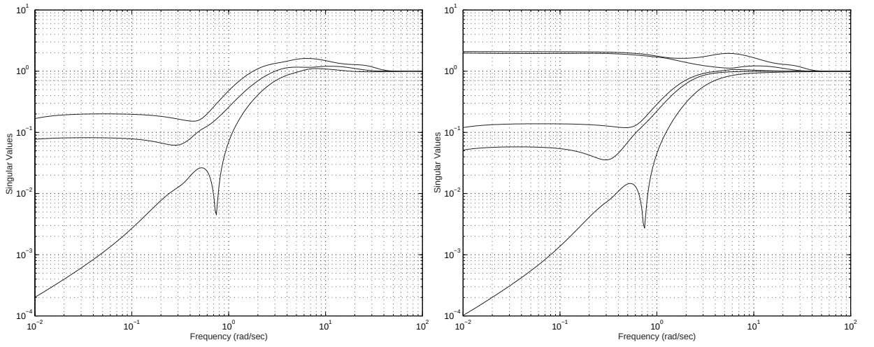
Figure 5.15: a) Input sensitivity \mathbf{S}_i b) Output sensitivity \mathbf{S}_o singular values
