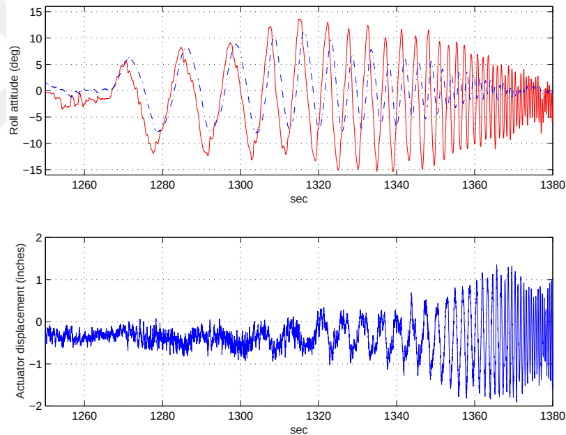
Figure 6.32: Roll axis frequency sweep: red -(demand), dash dot -(response), solid blue -(actuator displacement) for 1nsqDW
