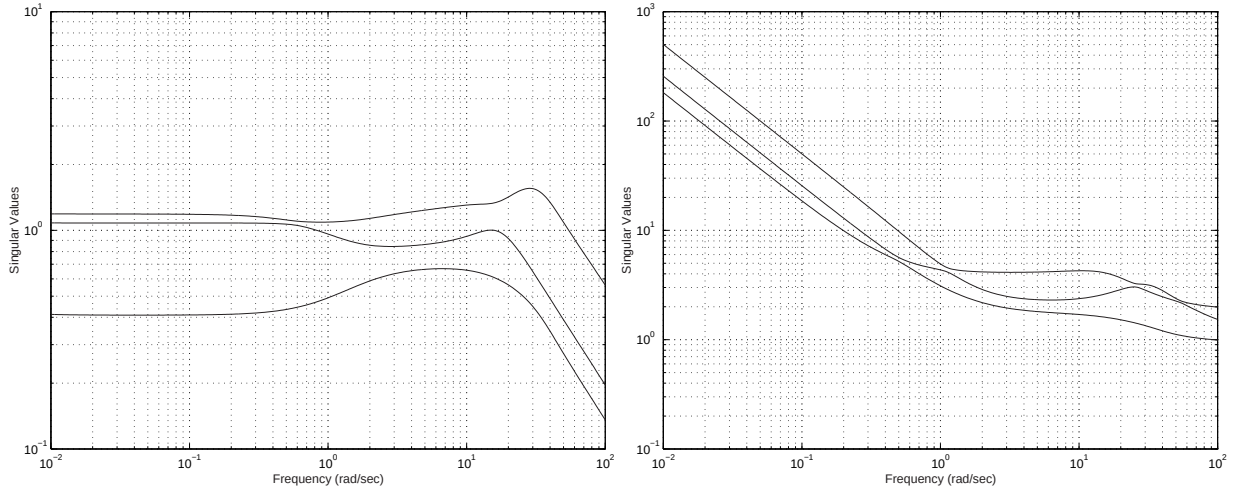
Figure 5.13: Singular values: a) Loop-shaping controller \mathbf{K}_\infty b) Implemented controller \mathbf{K}_{imp}
