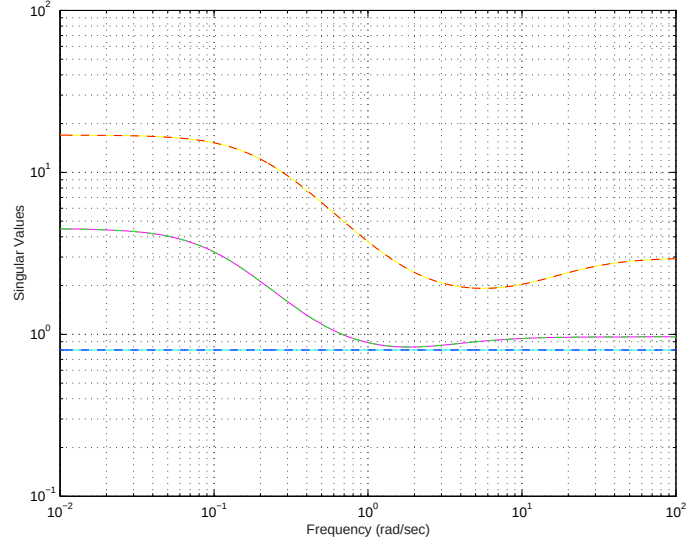
Figure 5.24: Non-diagonal weight and \Gamma
