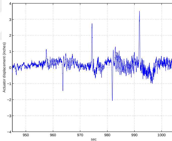
Figure 6.41: Roll axis actuator (FDA) activity
