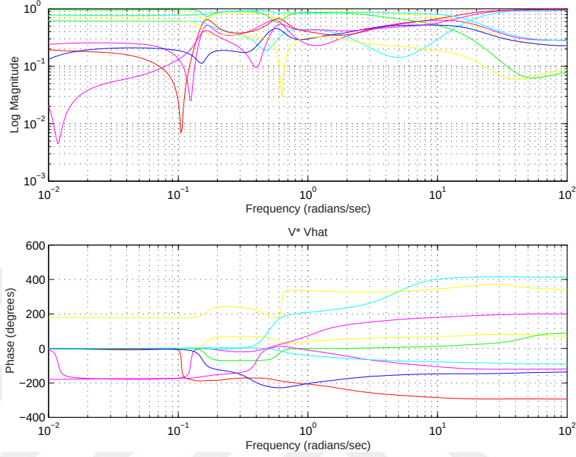
Figure 4.5: Frequency response of alignment product: V^* \cdot \hat{V}
