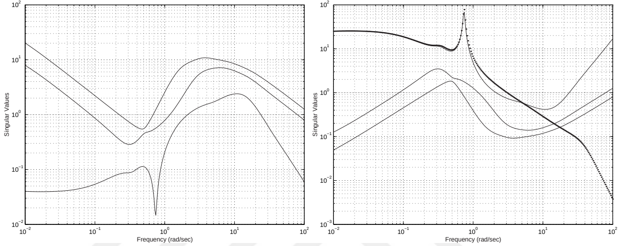
Figure 5.10: a ) Actuator activity due to output disturbance b ) Maximum allowable additive uncertainty vs. \bar{\sigma}(\mathbf{G})
