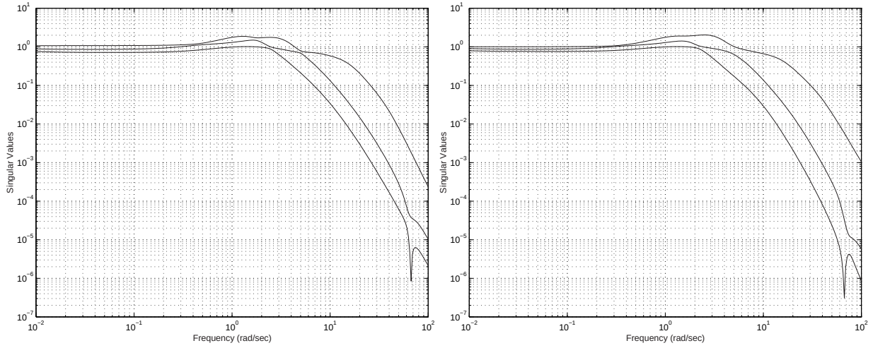
Figure 5.8: a) Input co-sensitivity T_i b) Output co-sensitivity T_o singular values
