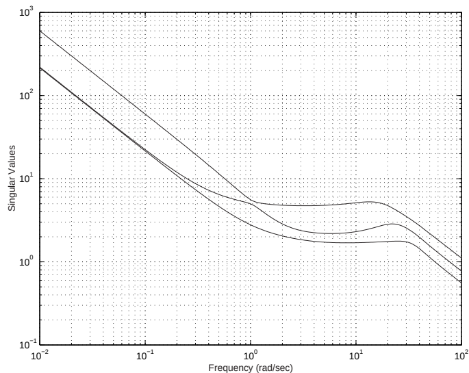
Figure 5.37: Singular values of \mathbf{K}_{imp}
