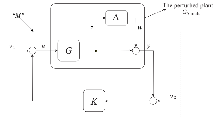
Figure 3.5: Multiplicative Uncertainty
