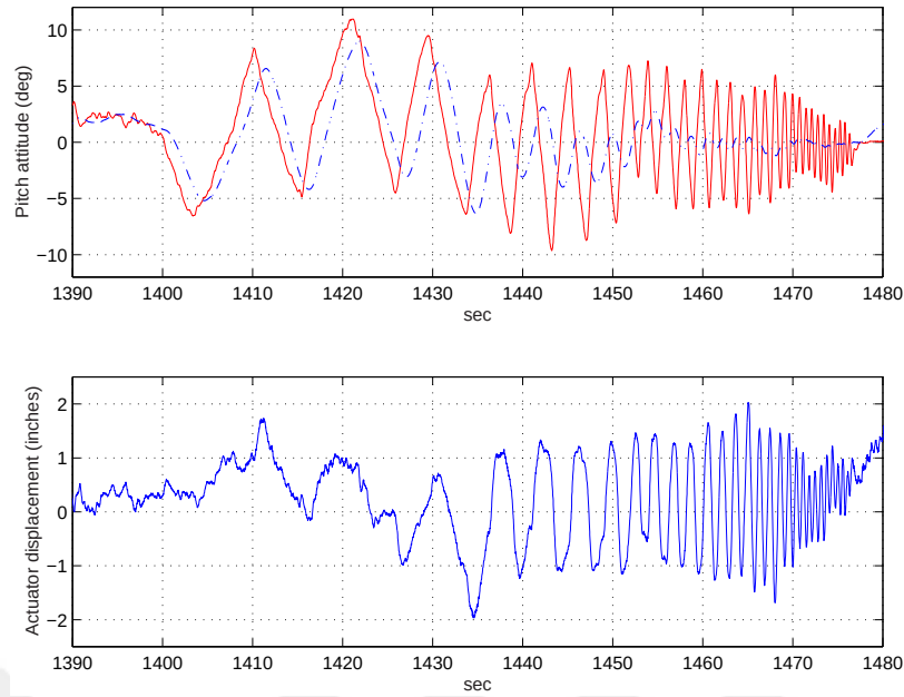
Figure 6.33: Pitch axis frequency sweep: red-(demand), dash dot-(response), solid blue-(actuator displacement) for 1nsqDW
