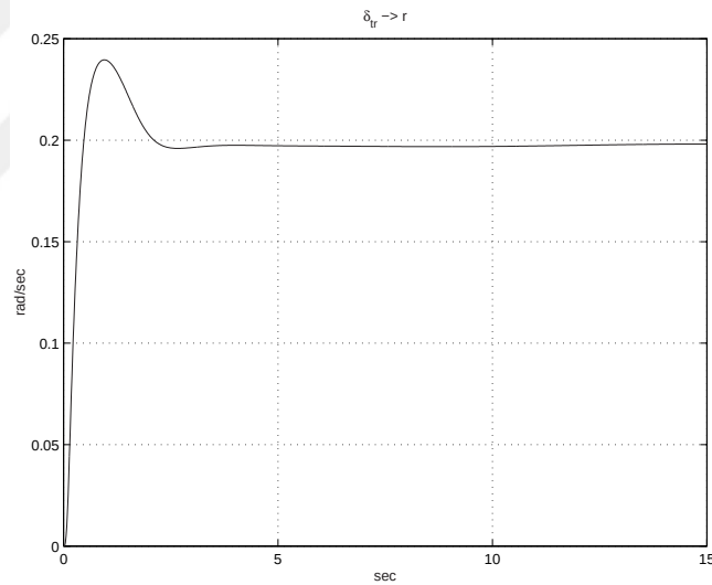
Figure 6.48: Linear response to pedal demand of 0.2 rad/sec
