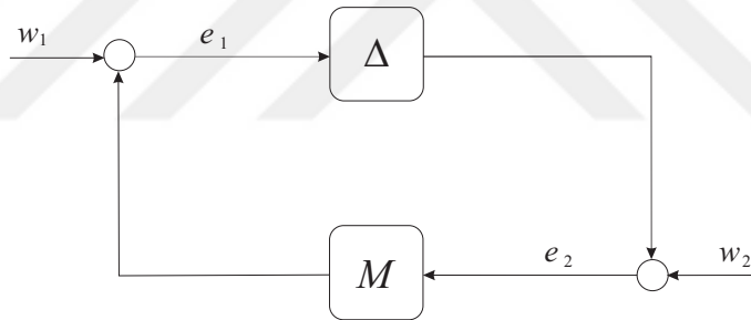
Figure 3.3: Small Gain Interconnection
