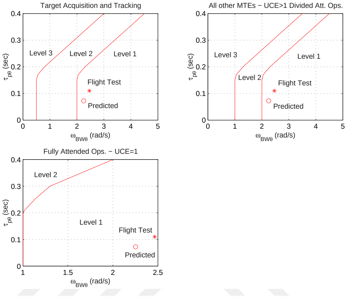
Figure 6.29: Small amplitude pitch attitude changes -hover and low speed- for 1nsqDW
