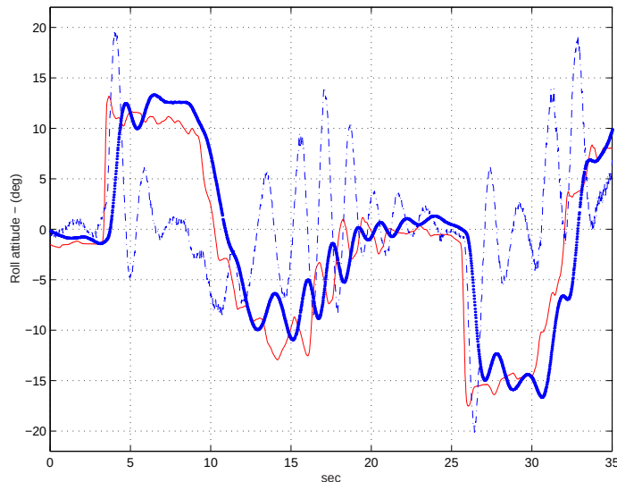
Figure 6.18: Roll axis in-flight response: demand; solid ( \phi ); dash dot ( p ) for 1sqDW
