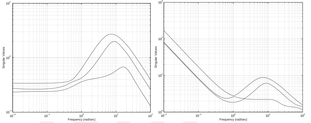
Figure 5.4: Singular values: a) Loop shaping controller \mathbf{K}_\infty b) Implemented controller \mathbf{K}_{imp}
