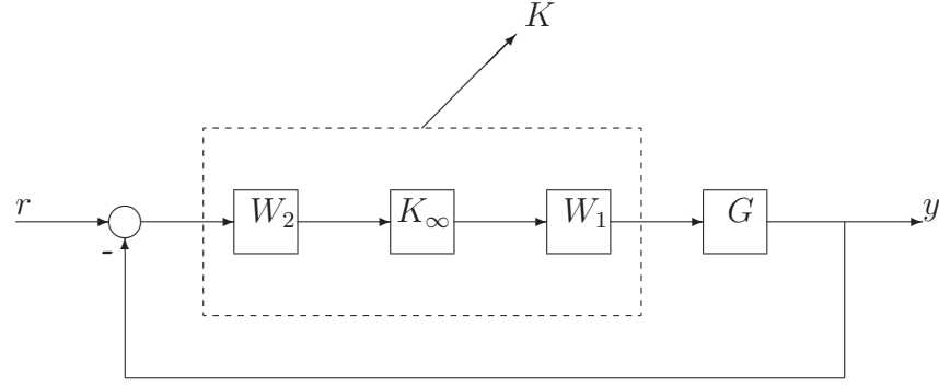
Figure 4.11: Unity Feedback for Loop Shaping
