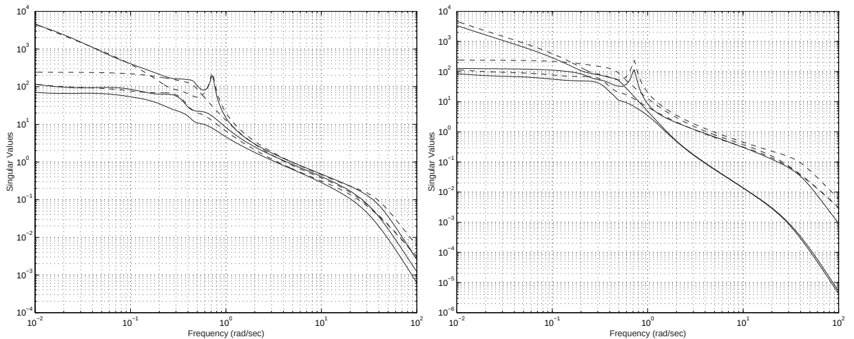
Figure 5.29: Shaped ( dashed ) vs. actual ( solid ) loop shapes: a) at the plant input \mathbf{L}_i b) at the plant output \mathbf{L}_o - 1nsqNDW
