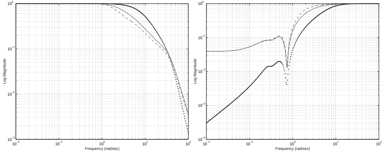
Figure 5.11: a) \bar{\sigma}(\mathbf{N}_s) b) \bar{\sigma}(\mathbf{M}_s) of shaped (dotted), nominal (continuous), reduced (dashed) plant
