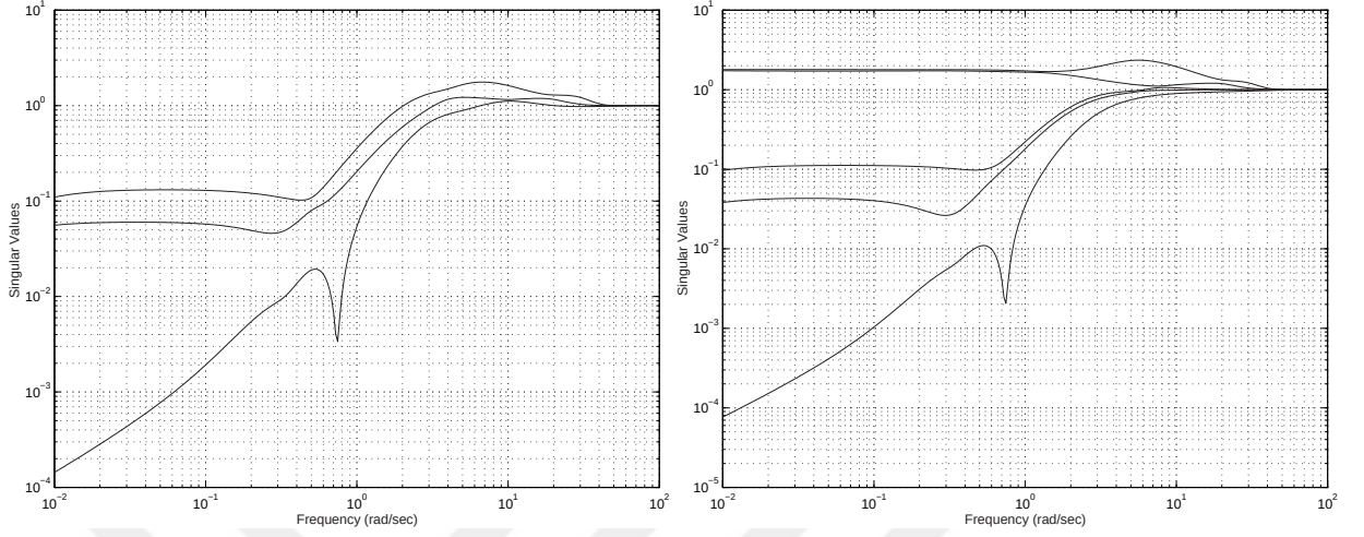
Figure 5.39: a) Input sensitivity S_i b) Output sensitivity S_o singular values
