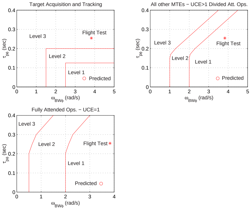
Figure 6.30: Small amplitude roll attitude changes -hover and low speed- for 1nsqDW
