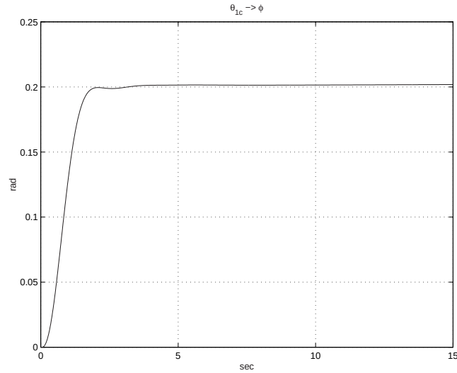
Figure 6.1: Linear response to lateral cyclic step demand of 0.2 rad
