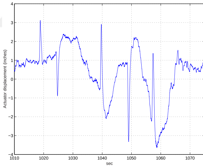
Figure 6.39: Pitch axis actuator (FDE) activity
