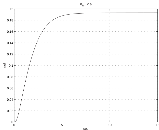
Figure 6.22: Linear response to lateral cyclic step demand of 0.2 rad
