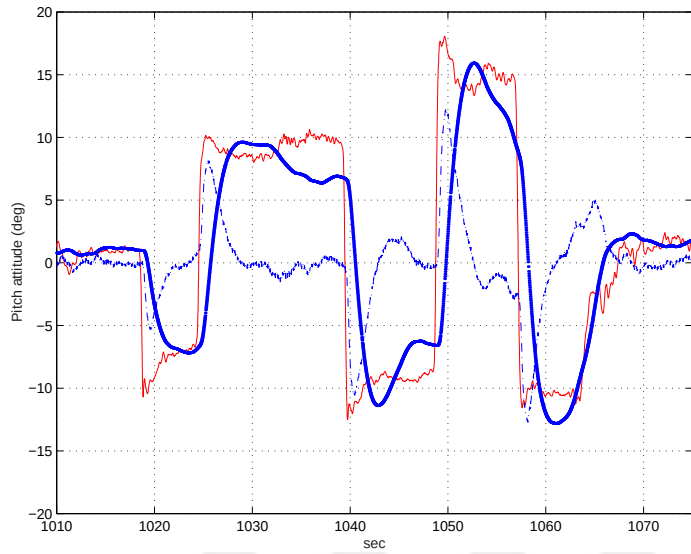
Figure 6.38: Pitch axis in-flight response: demand ; solid ( \theta ); dash dot ( q ) for 1sqDW
