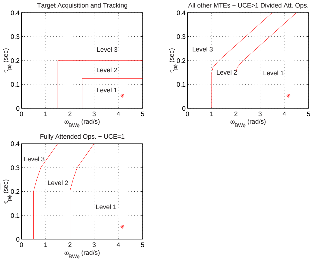
Figure 6.52: Small amplitude roll attitude changes -hover and low speed- for 1nsqNDW
