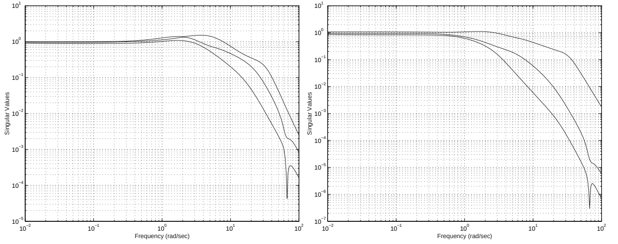
Figure 5.41: a) Input co-sensitivity T_i b) Output co-sensitivity T_o singular values
