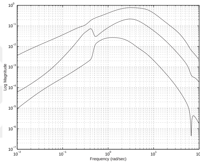
Figure 5.31: Singular values \mathbf{S}_o\mathbf{G}
