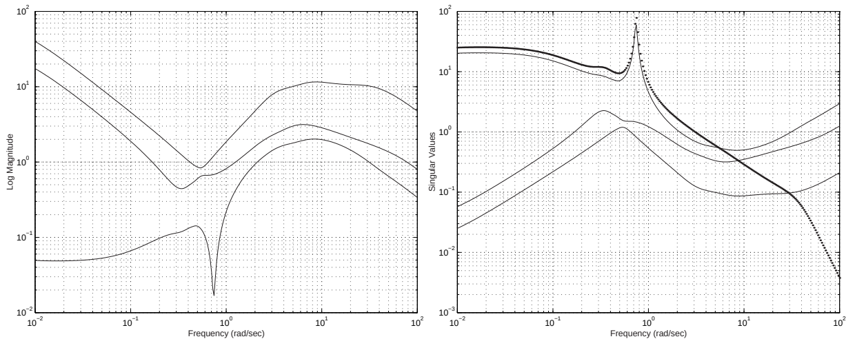
Figure 5.34: a) Actuator activity due output disturbance b) Maximum allowable additive uncertainty vs. \bar{\sigma}(G)
