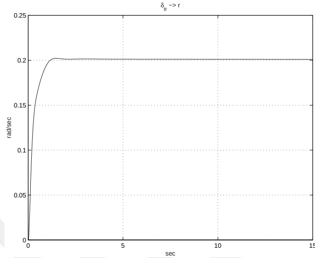
Figure 6.5: Linear response to pedal step demand of 0.2 rad/sec
