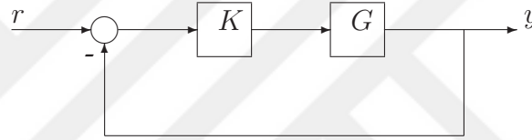
Figure 4.10: Unity Feedback implementation of K
