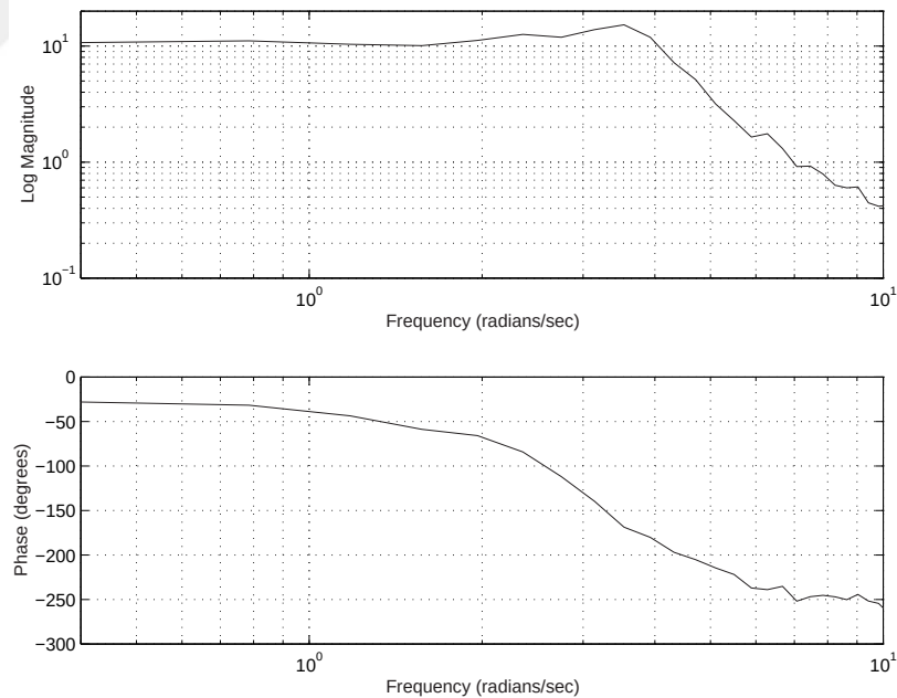
Figure 6.13: Roll axis frequency estimate for 1sqDW
