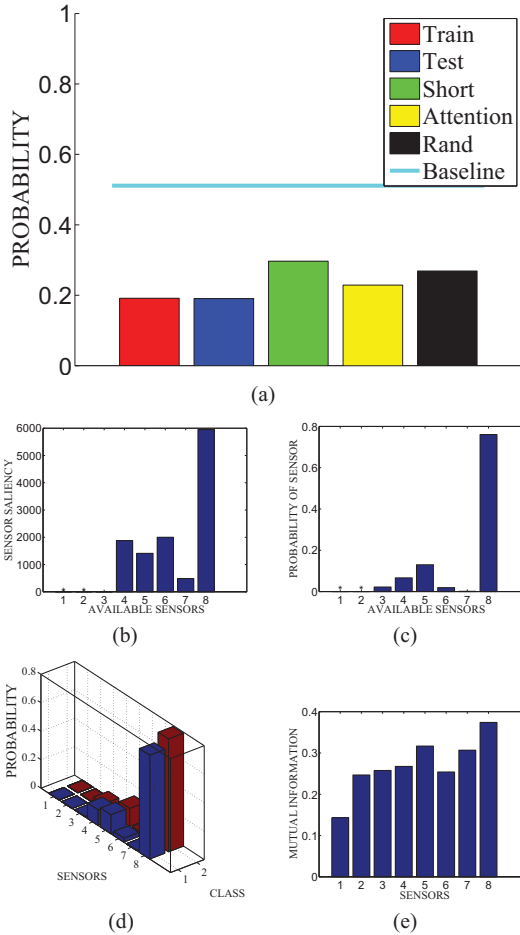
Fig. 3. Abalone data converted to a classification problem (old/young). Eight input features are considered. We simulate incomplete test measurement, in which only features (1,2) are included. The panels show: (a) Error rates in the training set of complete data ( N_{\text{train}} = 2500 ) and the error on the test set ( N_{\text{test}} = 677 ) using complete data, test error rate when using the initial feature set (1,2), test error using (1,2) and the feature chosen by the top down saliency estimate, and finally the test error obtained using (1,2) and a randomly chosen additional feature; (b) Estimated information saliency obtained on the test data, given the incomplete feature vector (1,2); (c) Frequency of selection of the additional features; (d) Frequency of selection of features in test cases within the two classes; (e) The \log_2 mutual information between features and class label.
