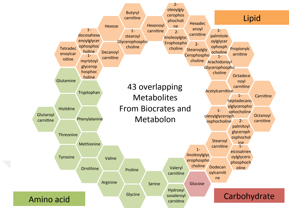
Figure 3-6 Forty-three overlapping metabolites from both platforms separated into 3 pathways (amino acid: green, lipid: orange, carbohydrate: red).
