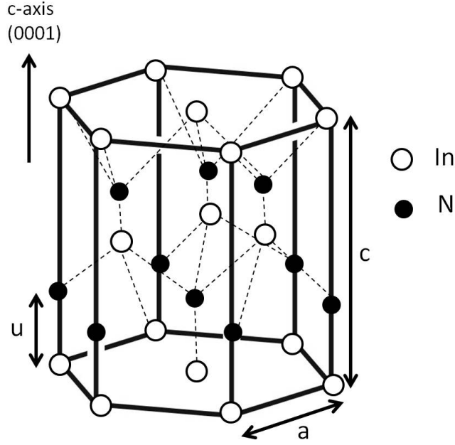
Figure 2.1: Wurtzite structure of InN crystal with its lattice constants 'a' and 'c'. The open spheres are In atoms and the smaller closed spheres indicate N atoms.
