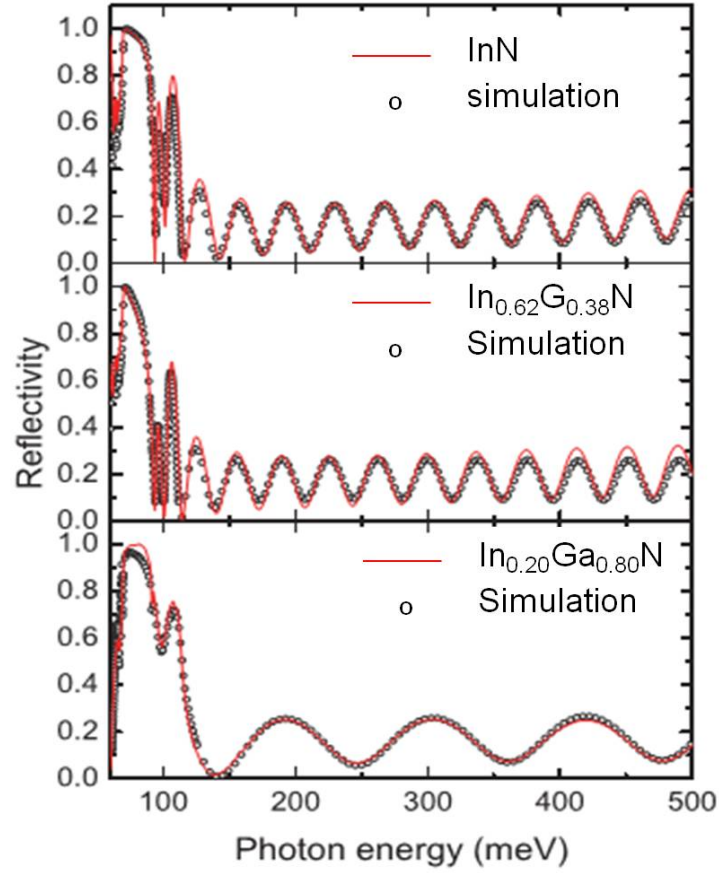
Figure 6.8: The experimental infrared reflectivity spectra for InN, In 0.62 Ga 0.38 N and In 0.20 Ga 0.80 N with the simulated spectra.
