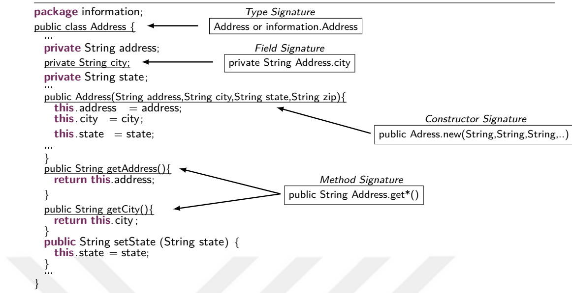
Figure 1.3: Connection between program elements and signatures
