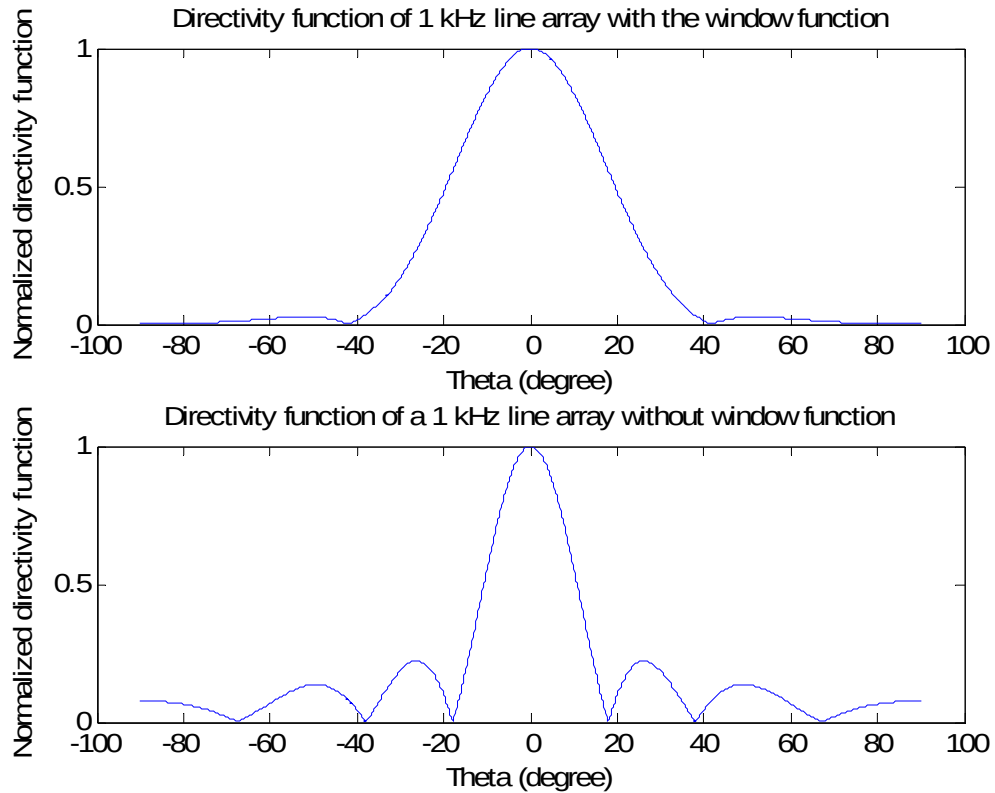
Figure 18. The far field beam pattern of the line array. Top figure is the result of using a Hanning window. This has reduced the side lobes at the expense of wider beam width.
