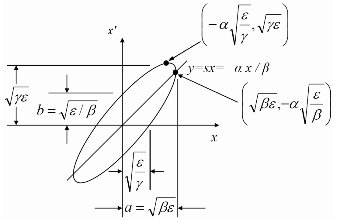
FIG. 4: The phase space ellipse of the beam representing the area that it occupies is plotted [5]. Here \beta , \alpha and \gamma are twiss parameters of the beam. The \epsilon is the emittance of the beam with \epsilon = \text{Area}/\pi .
