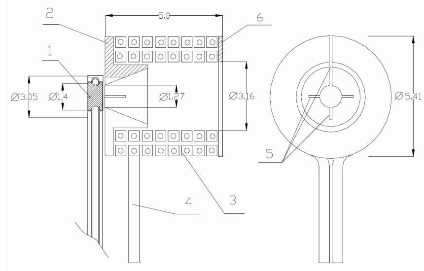
(b) Flux concentrator and other assembly
