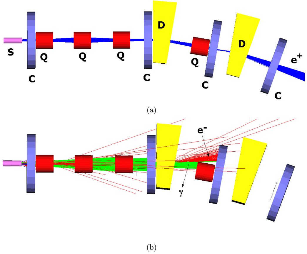
FIG. 66: A snapshot from the G4BEAMLIN simulation showing the forward secondary particles. The long cylinder on the left is the solenoid (S), quadrupoles are designated with letter (Q), dipoles (D) and the collimators (C) are located in between elements. As the dipole field diverts opposite signed particles in opposite directions, collimators are used to stop electrons. Almost all photons will be stopped as well. (a) Only e^+ beam is shown, where the beam passes cleanly through the holes of collimators. (b) e^- and \gamma are tracked, where the secondary e^- are stopped at the first dipole. The cryomodule is secured at a far enough location from the radiation zone. In this figure, the particles are intentionally stopped at the collimators to present a more clear picture. When simulating the power deposition in the elements then they are not killed.
