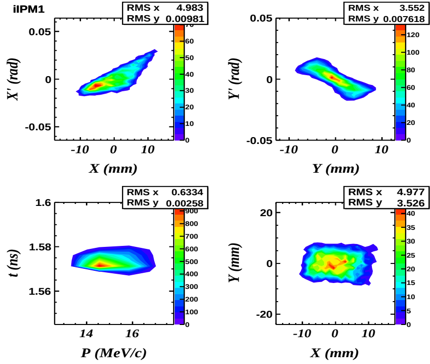
FIG. 59: The e^+ beam after the 1st CFM magnet in the CFM lattice. \varepsilon_x = 25.3 \text{ mm}\cdot\text{mrad} \varepsilon_y = 14.3 \text{ mm}\cdot\text{mrad} .
