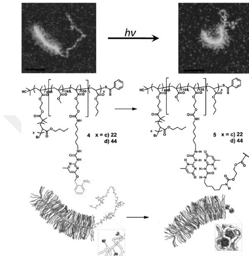
Figure 3.8 Polymer structures 4(c,d) and 5(c,d) including representative AFM height micrographs of 4d (top left) and 5d (top right) (scale bar=50 nm). Schematic representation of the polymer structures on the mica surface (bottom) (From P. J. M. Stals et al., J Am Chem Soc, 2013, 135, 11421–11424, with permission from the American Chemical Society).
