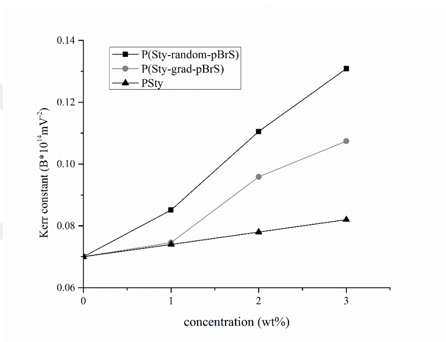
Figure 3.4 Kerr constants of PS (commercial), poly(random-S/p-BrS), and poly(“gradient”-S/p-BrS) by ATRP as measured on (1–3 wt %) 1,4-dioxane (>99% purity) solutions at 293 K.
