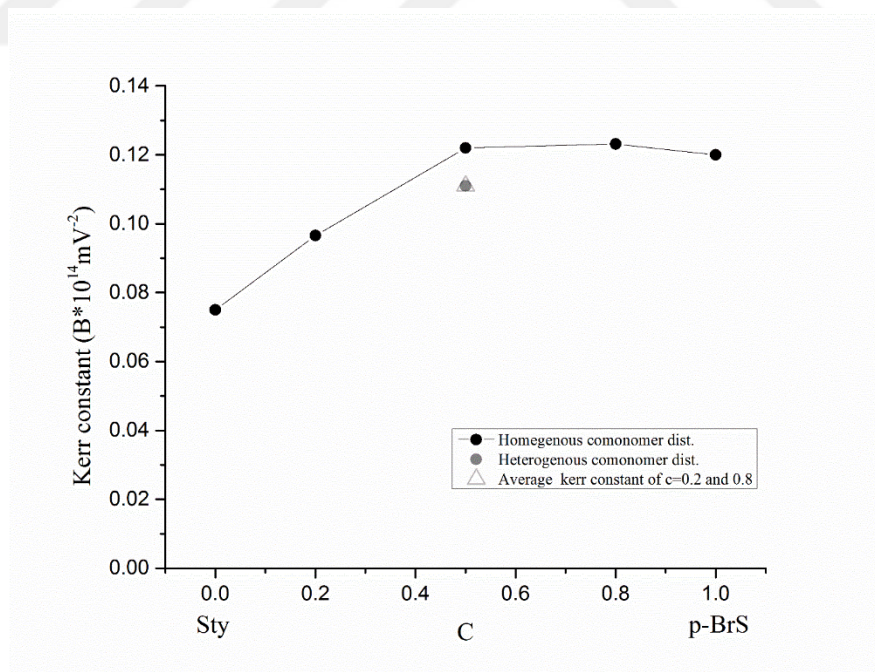
Figure 4.3 Comparison of Kerr constants B ( \times 10^{-14} \text{ Vm}^{-2} )/repeat unit observed for S/p-BrS copolymers in 2 wt% dioxane solutions at room temperature. c is mole fractional content of p-BrS units.
