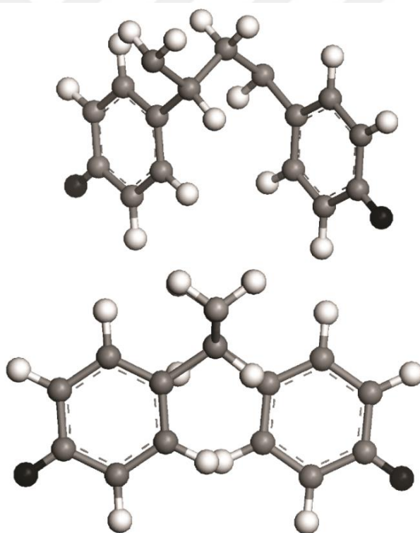
Figure 3.3 Along backbone end-view (bottom) and \sim 45^\circ from full frontal-view (top) of a r-p-BrS-p-BrS diad.
