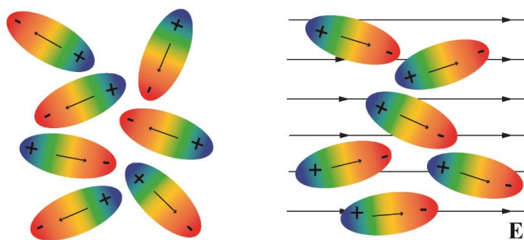
Figure 1.2 Molecular orientation under electric field, E . Over all molecular dipole moment is parallel to the long axis of the ellipsoidal molecular polarizability tensor.
