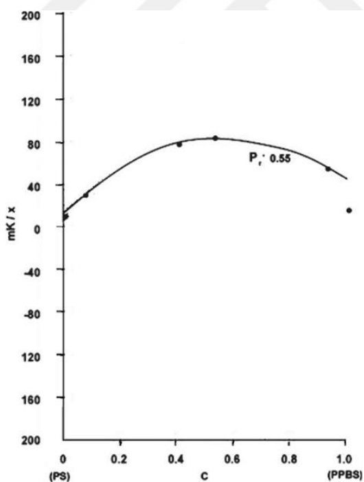
Figure 3.5 Comparison of mKs ( \times 10^{-1} \text{ cm}^7 \text{ SC}^{-2} \text{ mol}^{-1} ) observed and calculated for atactic S/pBr copolymers made by bromination of a-PS.[6] x , c , and Pr are the number of repeat units (200) and the fractional contents of p-BrS units and racemic or r-diads, respectively.
