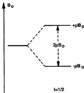
Figure 1.8 Possible energy levels of a nucleus with spin \frac{1}{2} in an applied magnetic field.
