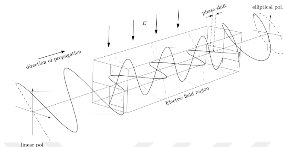
Figure 1. 3 The Kerr effect on linearly polarized light, producing elliptically polarized light. Figure is taken from Ref.11
