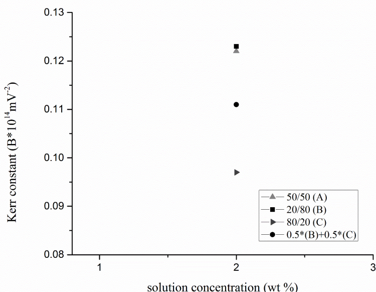
Figure 4.4 Kerr constants (B)/repeat unit measured on 2 wt% dioxane solutions of 50:50, 20:80, 80:20, and a 50:50 mixture of the latter two S/p-BrS copolymers.
