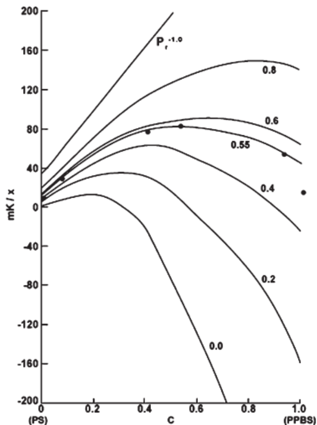
Figure 1.10 Comparison of mKs observed and calculated for S/p-BrS-I copolymers. x , P_r , and C are the number of repeat units (200), fraction of r-diads, and fractional content of p-BrS units. 49
