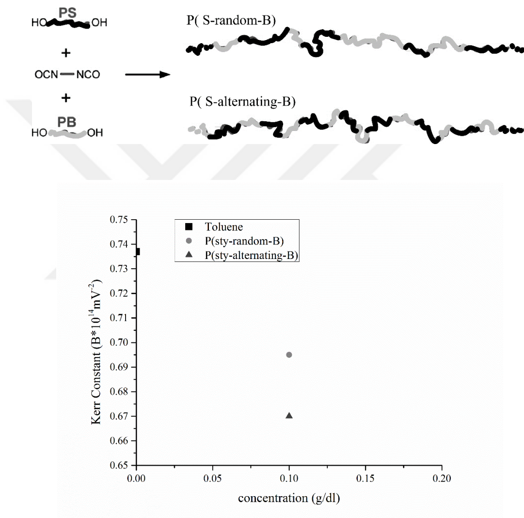
Figure 3.6 Structures and Kerr constants of 0.1 g/dL toluene solutions of styrene/butadiene multiblock copolymers with random and regularly alternating blocks 9 .
