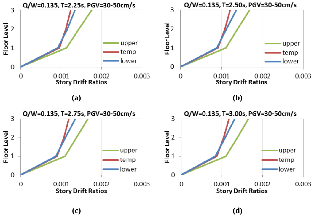
Figure 6.46 Average peak story drift ratios of 3 story steel structures with same Q/W=0.135 , PGV=30-50\text{cm/s} and different T : a) T=2.25\text{s} , b) T=2.50\text{s} , c) T=2.75\text{s} , d) T=3.00\text{s}
