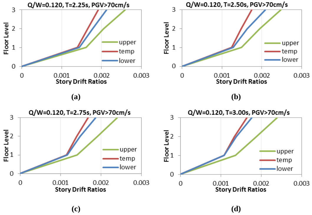
Figure 6.45 Average peak story drift ratios of 3 story steel structures with same Q/W=0.120 , PGV>70\text{cm/s} and different T : a) T=2.25\text{s} , b) T=2.50\text{s} , c) T=2.75\text{s} , d) T=3.00\text{s}
