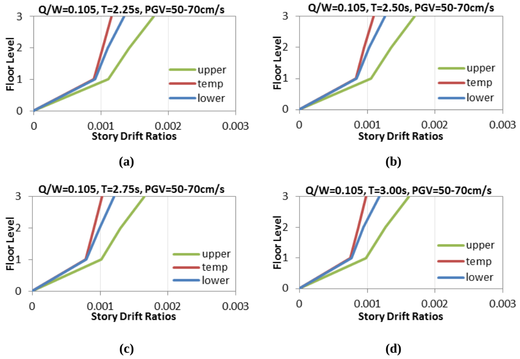
Figure 6.41 Average peak story drift ratios of 3 story steel structures with same Q/W=0.105 , PGV=50-70cm/s and different T : a) T=2.25s , b) T=2.50s , c) T=2.75s , d) T=3.00s
