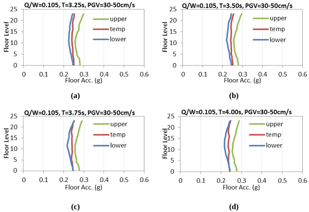
Figure 6.4 Average peak floor accelerations of 23 story reinforced concrete structures with same Q/W=0.105 , PGV=30-50\text{cm/s} and different T : a) T=3.25\text{s} , b) T=3.50\text{s} , c) T=3.75\text{s} , d) T=4.00\text{s}
