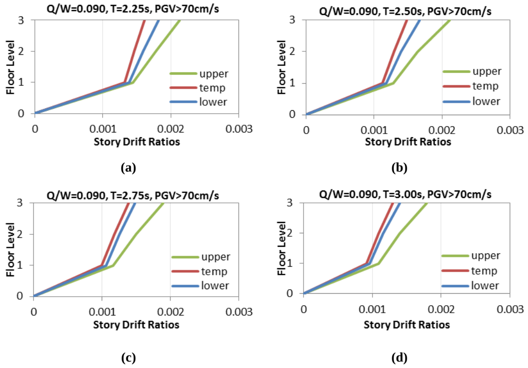
Figure 6.39 Average peak story drift ratios of 3 story steel structures with same Q/W=0.090 , PGV>70\text{cm/s} and different T : a) T=2.25\text{s} , b) T=2.50\text{s} , c) T=2.75\text{s} , d) T=3.00\text{s}
