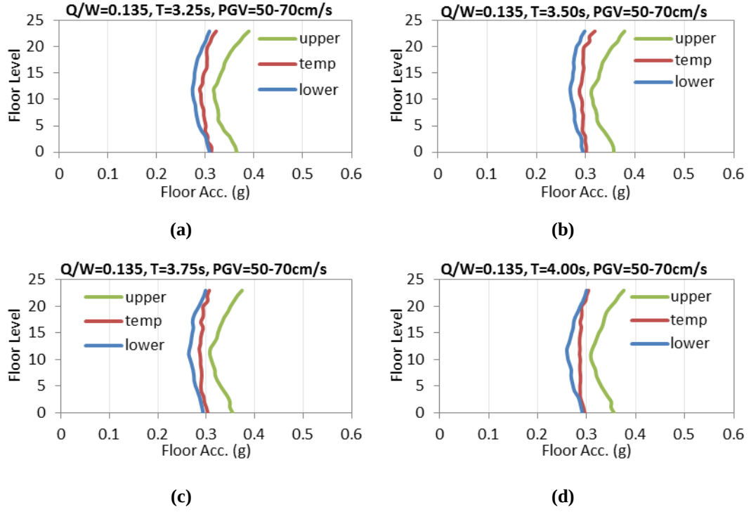
Figure 6.11 Average peak floor accelerations of 23 story reinforced concrete structures with same Q/W=0.135 , PGV=50-70\text{cm/s} and different T: a) T=3.25\text{s} , b) T=3.50\text{s} , c) T=3.75\text{s} , d) T=4.00\text{s}
