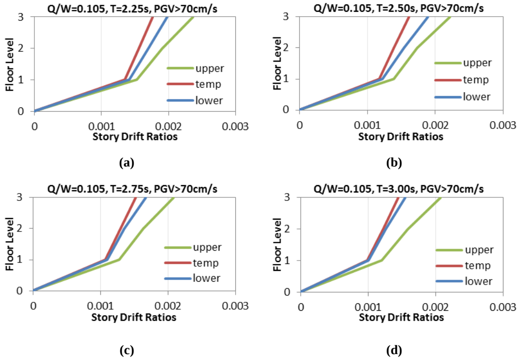
Figure 6.42 Average peak story drift ratios of 3 story steel structures with same Q/W=0.105 , PGV>70cm/s and different T : a) T=2.25s , b) T=2.50s , c) T=2.75s , d) T=3.00s
