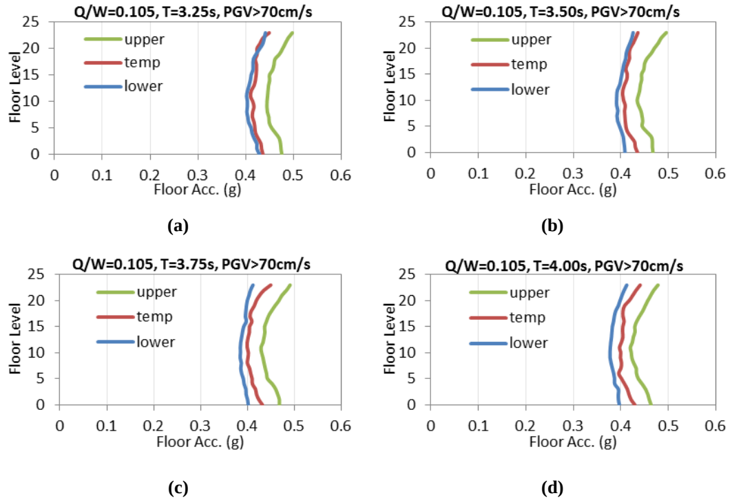
Figure 6.6 Average peak floor accelerations of 23 story reinforced concrete structures with same Q/W=0.105 , PGV>70\text{cm/s} and different T : a) T=3.25\text{s} , b) T=3.50\text{s} , c) T=3.75\text{s} , d) T=4.00\text{s}
