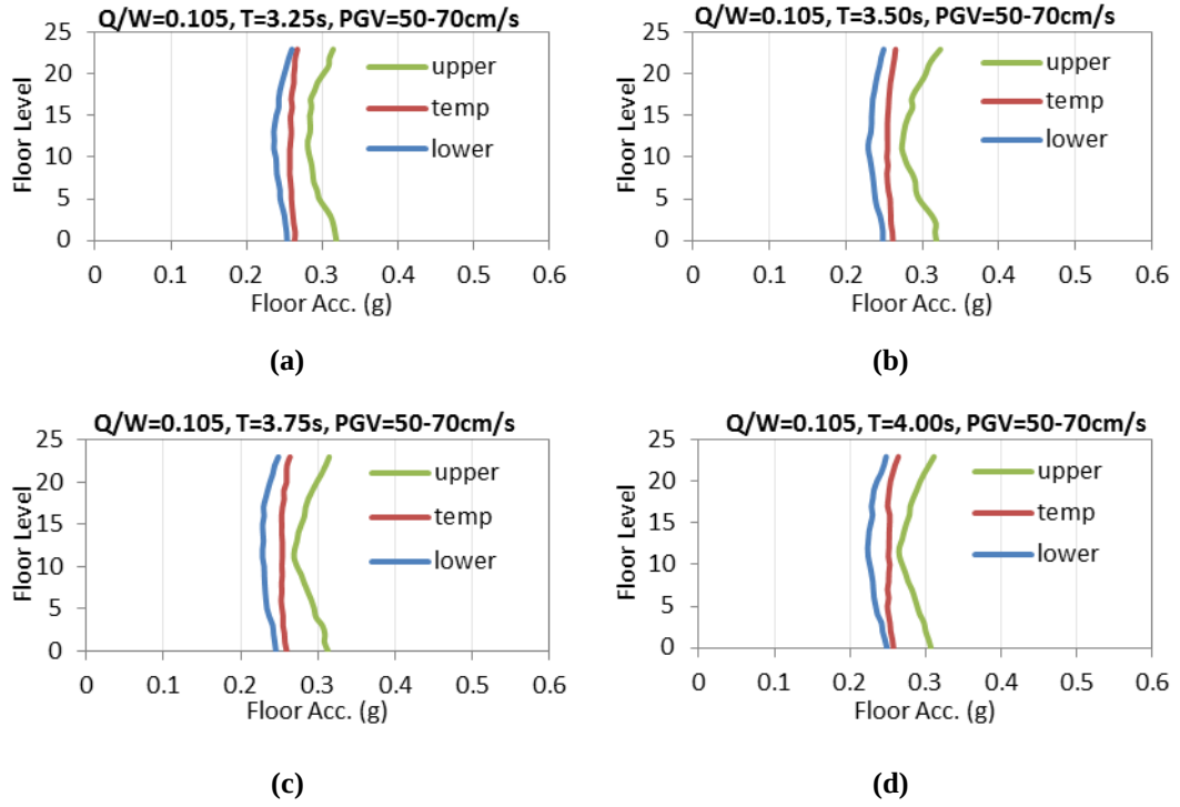
Figure 6.5 Average peak floor accelerations of 23 story reinforced concrete structures with same Q/W=0.105 , PGV=50-70\text{cm/s} and different T : a) T=3.25\text{s} , b) T=3.50\text{s} , c) T=3.75\text{s} , d) T=4.00\text{s}
