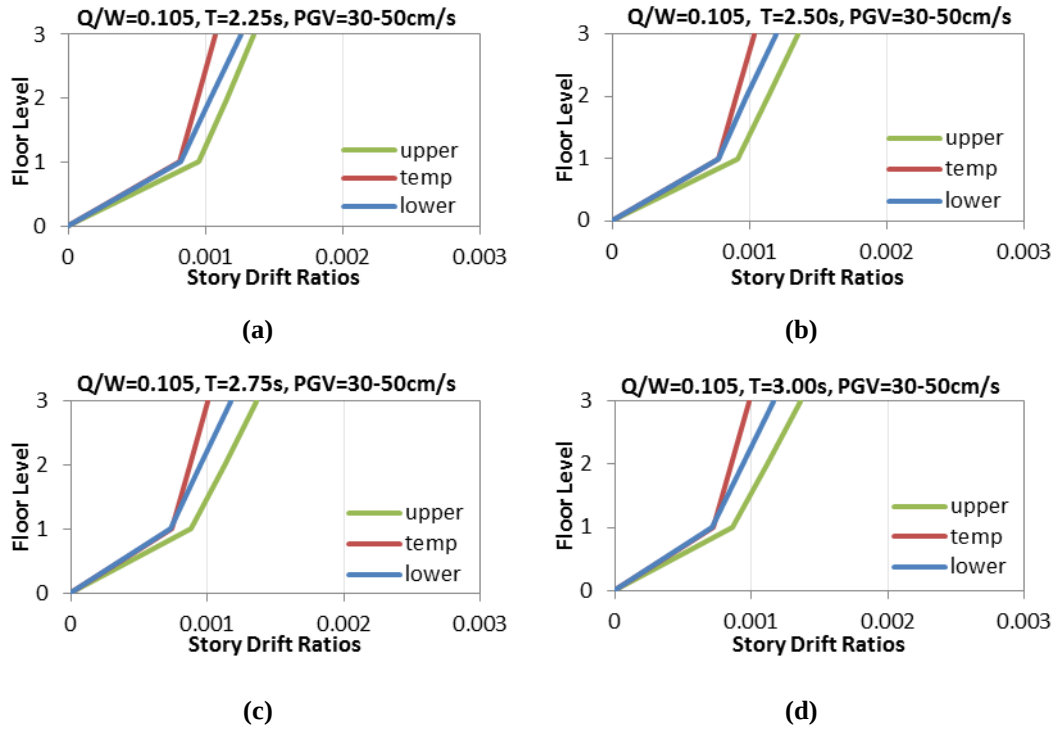
Figure 6.40 Average peak story drift ratios of 3 story steel structures with same Q/W=0.105 , PGV=30-50\text{cm/s} and different T : a) T=2.25\text{s} , b) T=2.50\text{s} , c) T=2.75\text{s} , d) T=3.00\text{s}
