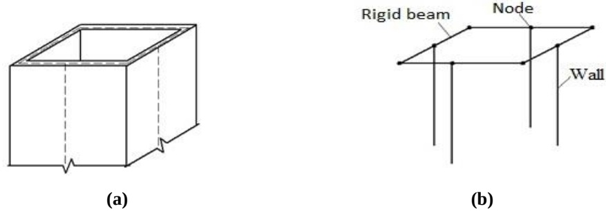
Figure 4.3. Shear wall model a) 3-D view, b) mathematical model
