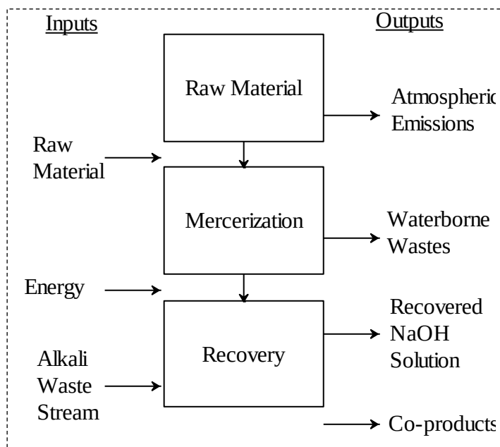
Figure 11. System under consideration for evaporative recovery
