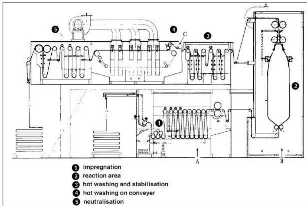
Figure 4. Example of mercerizing equipment for knitted fabric [2]
