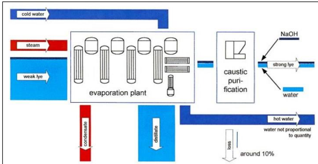
Figure 5. Scheme of evaporation plant for caustic recovery [2]
