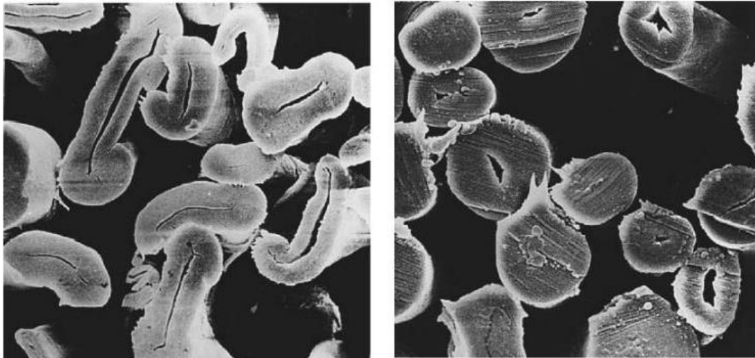
Figure 3. Electronic microscope image of cotton fibers before (on the left) and after (on the right) mercerization [10]
