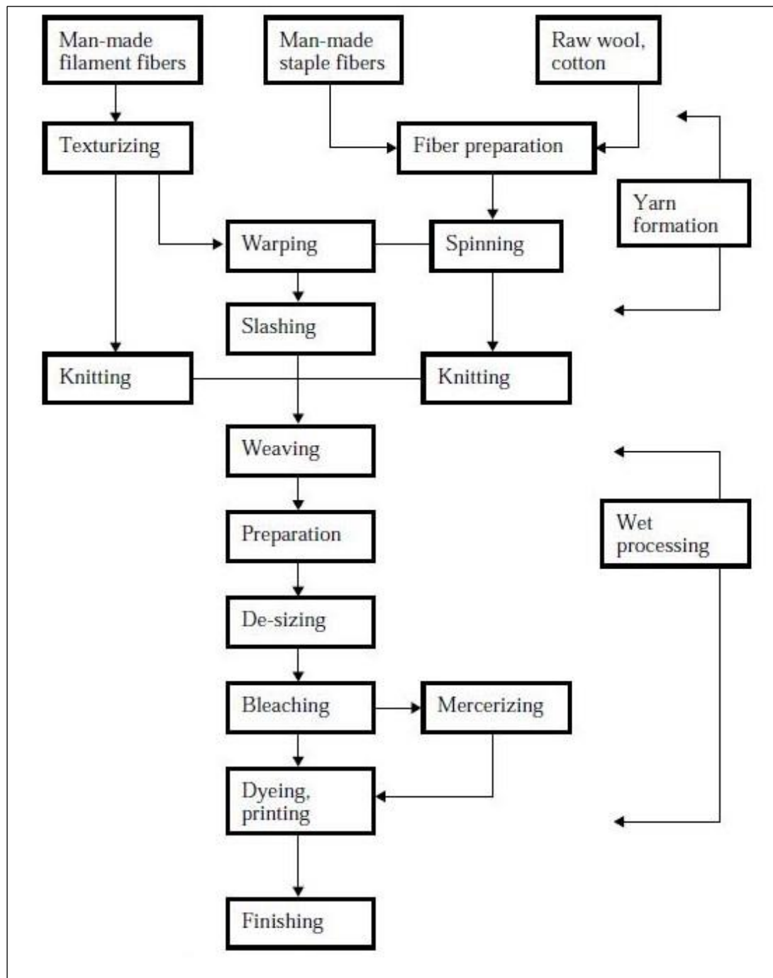
Figure 1. Processes for cotton processing textile mill [3]
