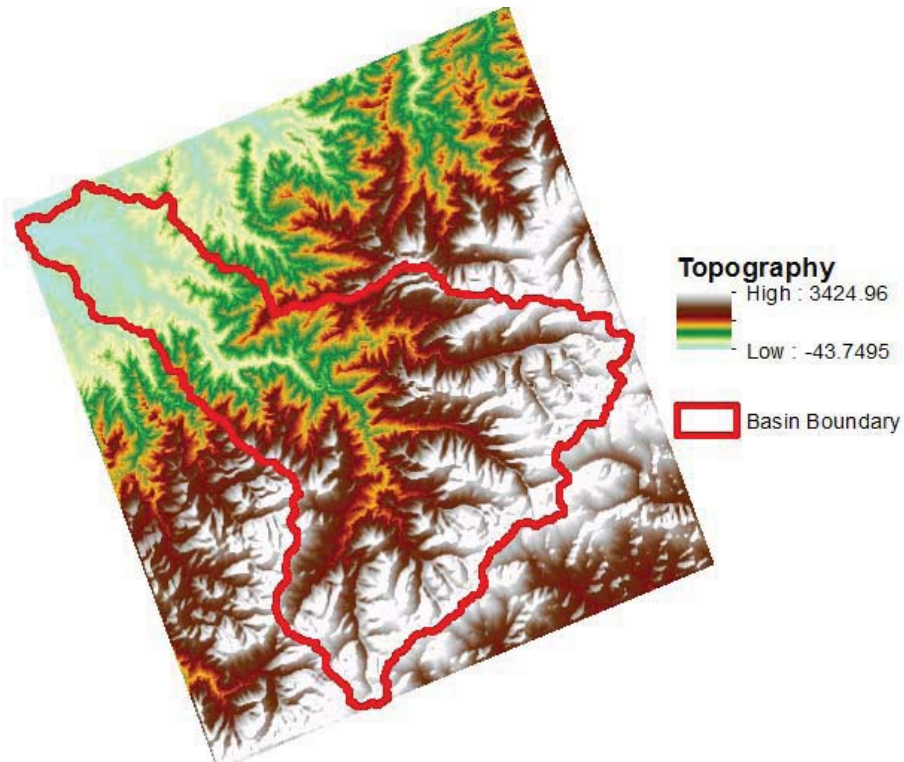
Figure 3.2 Basin topography
