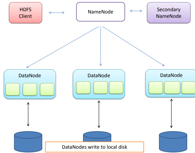
Figure 1: Hadoop distributed files system architecture.
