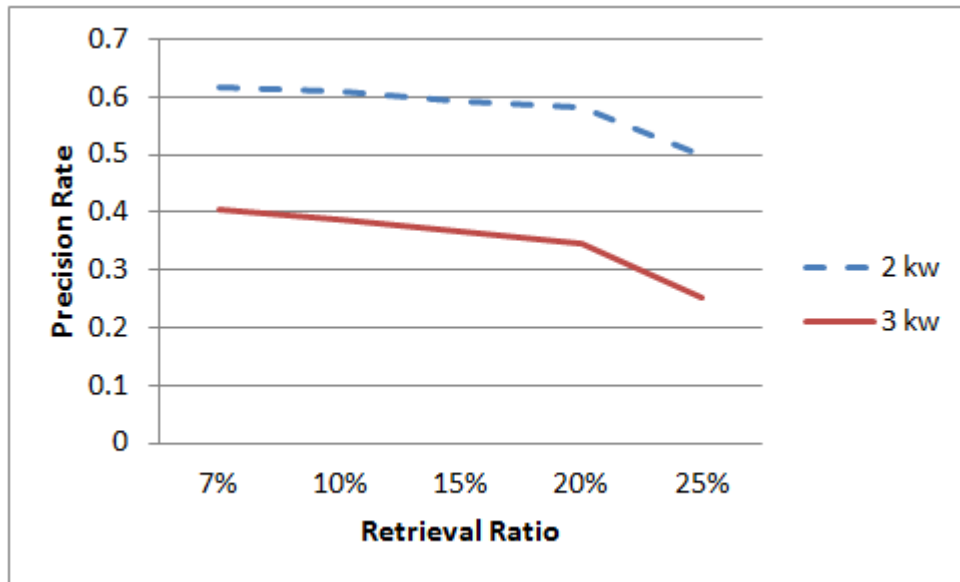
Figure 10: Average Precision Rate, \lambda = 100
