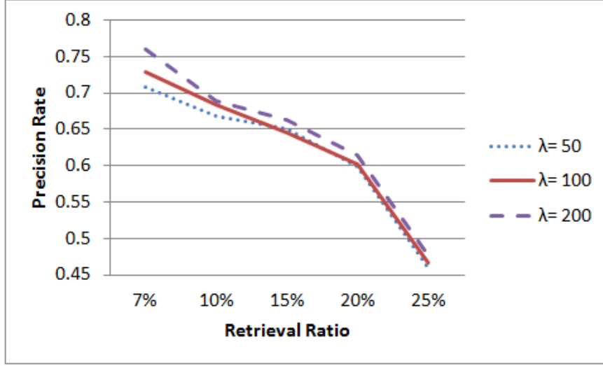
Figure 14: Average Precision Rate for different \lambda
