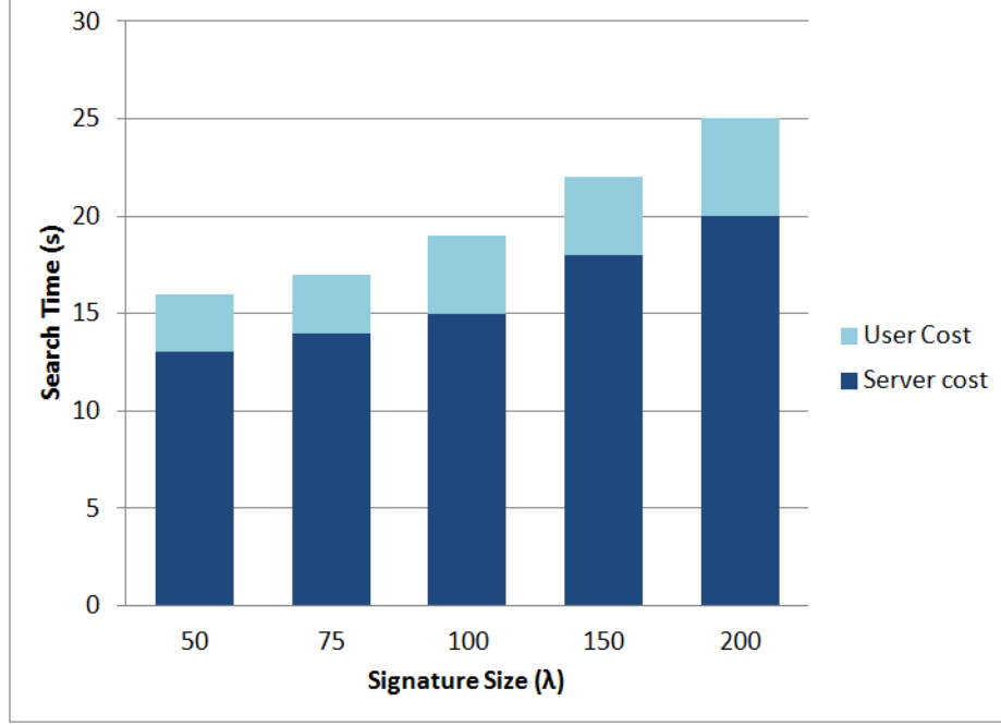
Figure 9: Search Time
