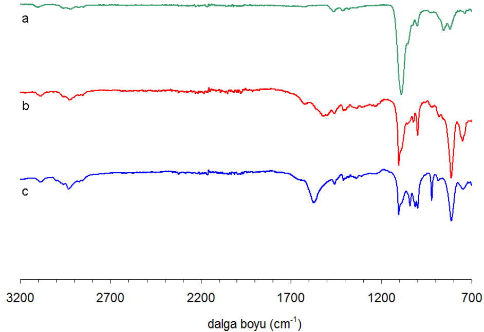
Şekil 8.12. (a) \text{PVF}^+\text{ClO}_4^- , (b) \text{PoPD}/\text{PVF}^+\text{ClO}_4^- ve (c) \text{Gox}/\text{PoPD}/\text{PVF}^+\text{ClO}_4^- 'nin FT-IR spektrumları
