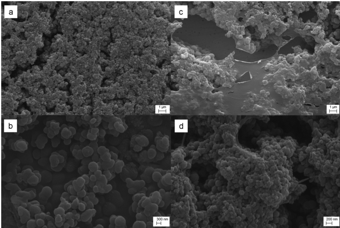
Şekil 8.13. (a) \text{PVF}^+\text{ClO}_4^-/\text{Pt} (b) \text{PtNPs}/\text{PVF}^+\text{ClO}_4^-/\text{Pt} (c) \text{PoPD}/\text{PVF}^+\text{ClO}_4^-/\text{Pt} (d) \text{Gox-PoPD}/\text{PtNPs}/\text{PVF}^+\text{ClO}_4^-/\text{Pt} yüzeylerine ait SEM görüntüleri
