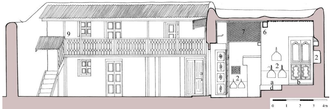
Resim 4.44: Kadija Ahmed evinin kesit-cephesi (Revault, Santelli, 2004, s:137)
