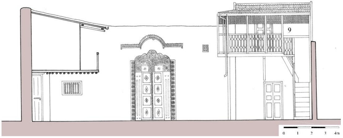
Resim 4.45: Kadija Ahmed evinin kesit-cephesi (Revault, Santelli, 2004, s:137)
