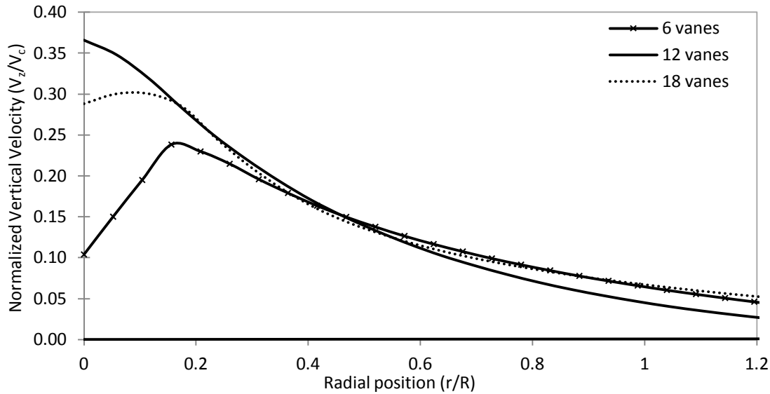
Figure 5.7 Variations of normalized axial velocity in radial direction with respect to the number of vanes at an elevation of respective peak axial volumetric flow rate
