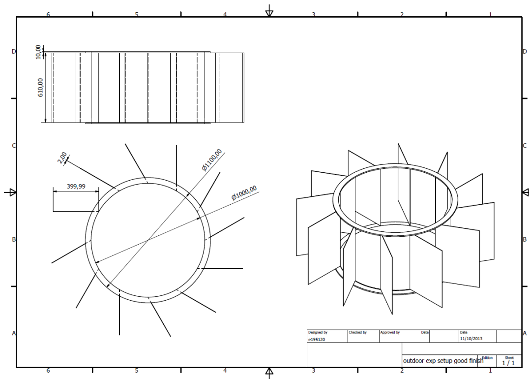
Figure 0.4 Technical drawing of the outdoor experimental setup
