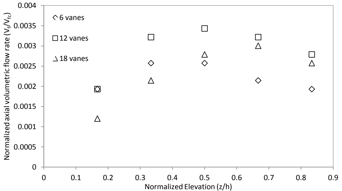
Figure 5.6 Vertical variations of normalized axial volumetric flow rate for different number of vanes
