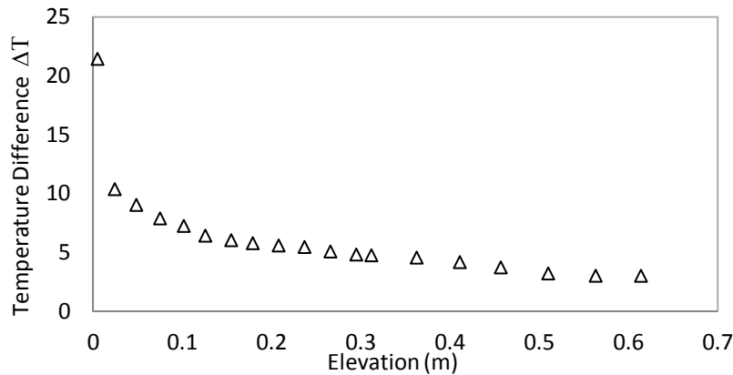
Figure 2.3 Measured temperature profile along the Vortex centerline for the field Vortex
