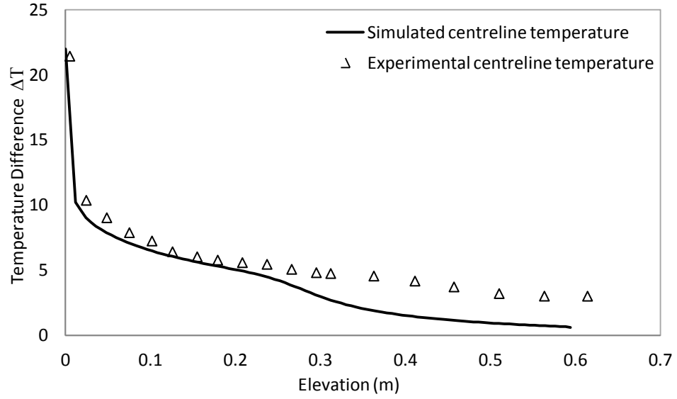
Figure 4.4 Comparison of experimental and simulated centerline temperature profile
