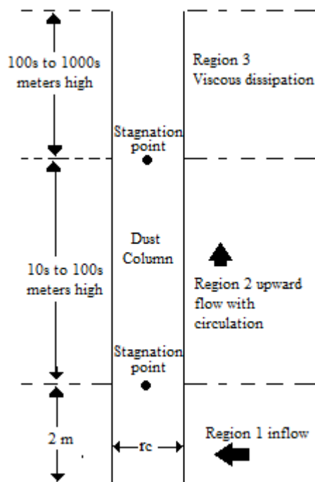
Figure 1.1 Regions within a dust devil
