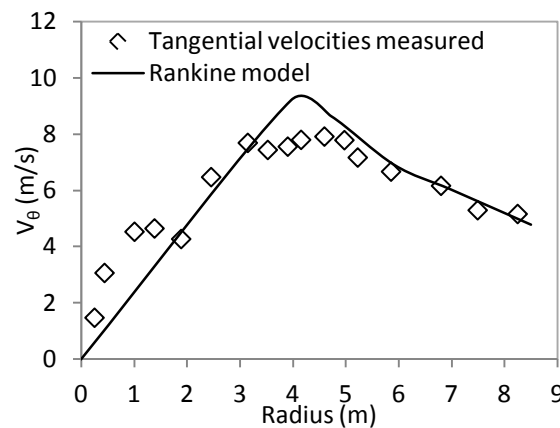
Figure 2.1 Tangential velocity profile measured by Sinclair, with Rankine vortex model
