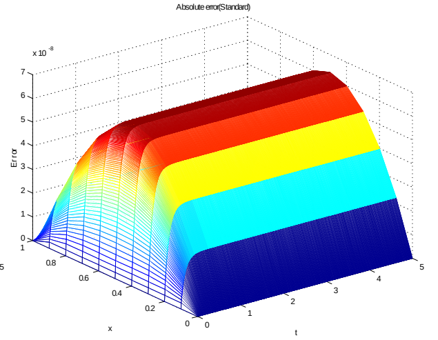
Figure 4.4 Absolute error for SFD scheme (4.2.3)
