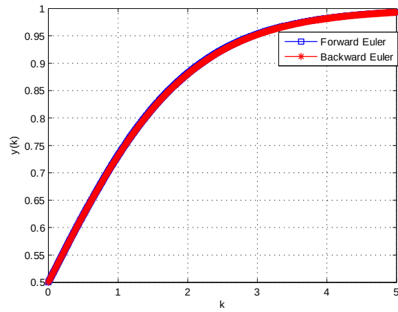
Figure 3.4. SFD schemes (3.2.8) for h = 0.01
