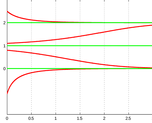
Figure 3.21 Typical trajectories for (3.8.37)
