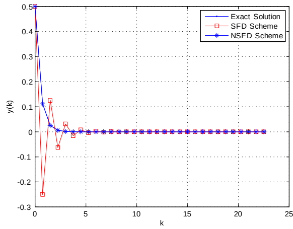
Figure 3.16. Comparison of methods for (3.5.1) h=0.75
