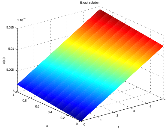
Figure 4.1 Plot of exact solution (4.2.2)
