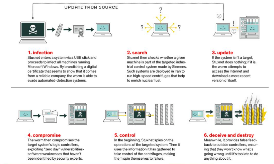
Figure 8. How Stuxnet Worked 339
