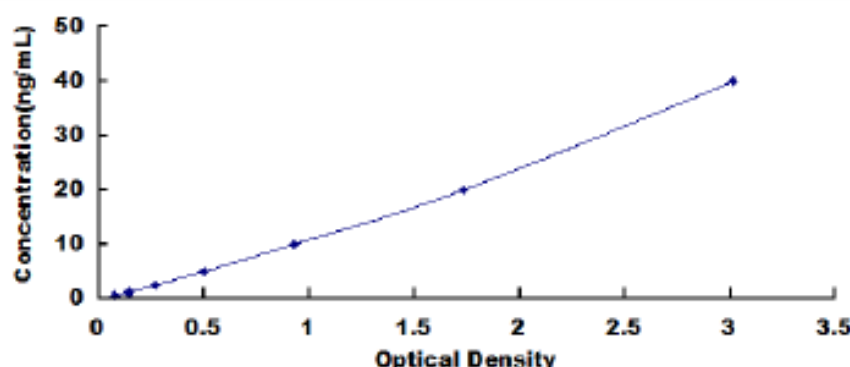
Typical Standard Curve for Uromodulin, Human ELISA.
