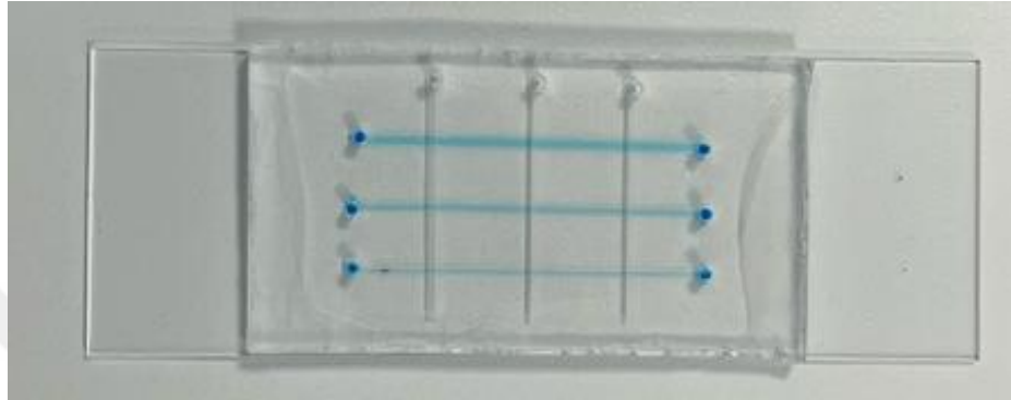
Figure 3.4. View of the chip with pneumatic valve designs. Control and fluidic channels, designed with widths of 200, 400, and 800 \mu\text{m} respectively, are filled with water and a blue-colored solution.
