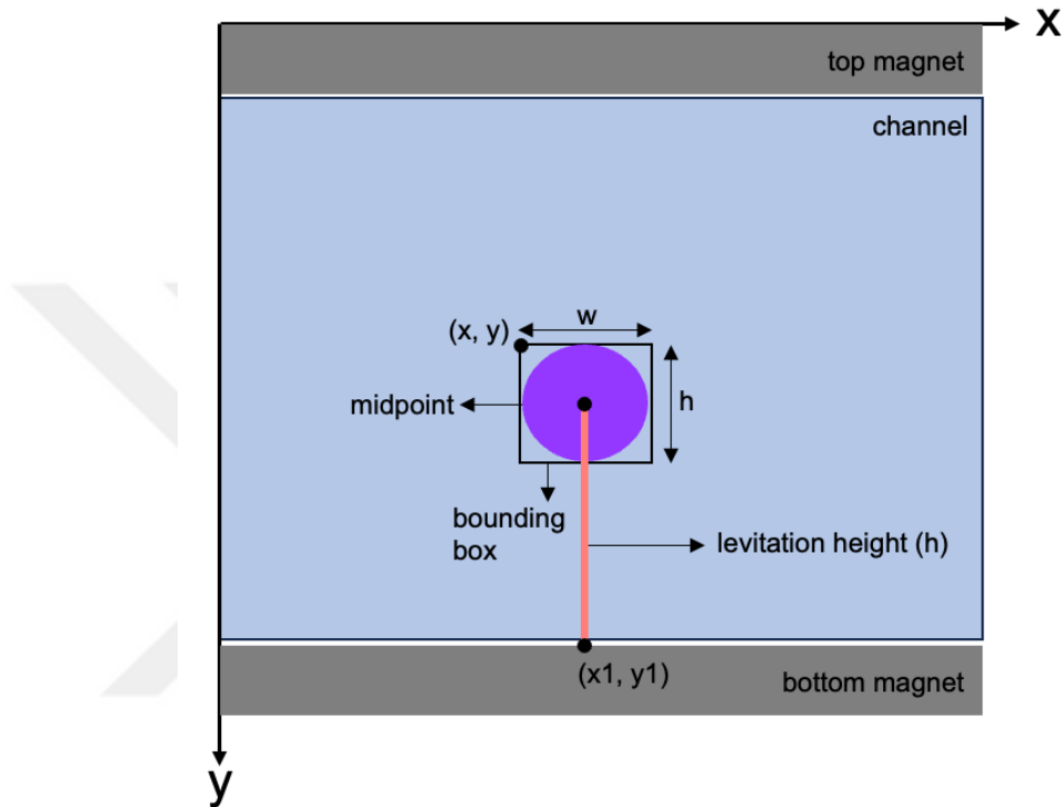
Figure 2.12. YOLO was used to determine the bounding box of the detected bead. The levitation height (i.e., the distance between the bottom magnet and the bounding box midpoint) and radius (i.e., half of h ) of the bead were determined using the bounding box's width ( w ), height ( h ), and upper left corner (x, y) coordinates.
