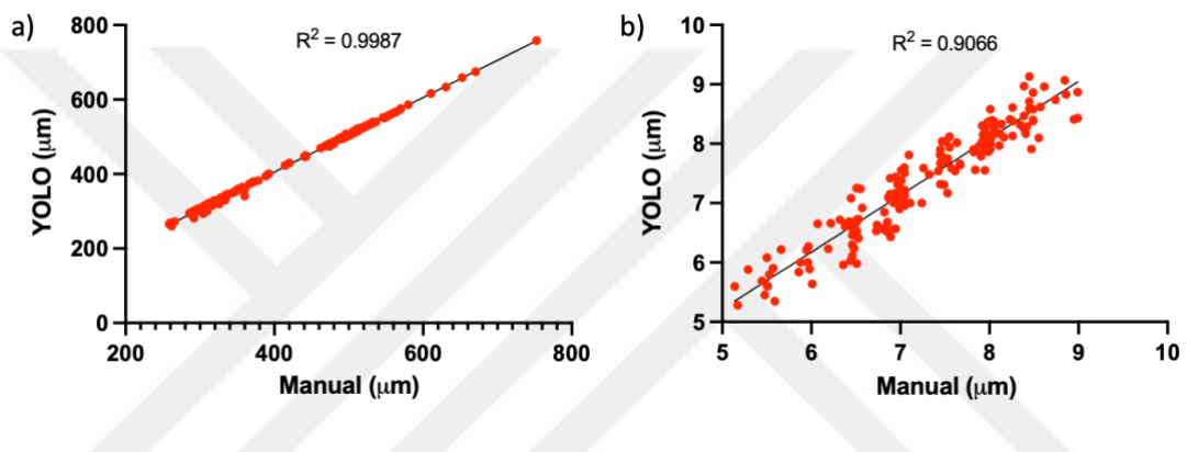
Figure 2.22. Comparison of bead data analysis performed manually and automatically using YOLO. The comparison graphs of (a) the levitation heights and (b) the radius of beads. The figures displayed the coefficient of determination ( R^2 ) values obtained from the linear regression model.
