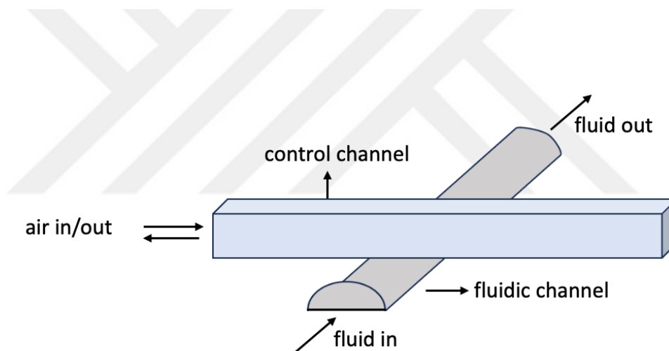
Figure 3.2. Illustration of valve formation with fluidic and control channels.
