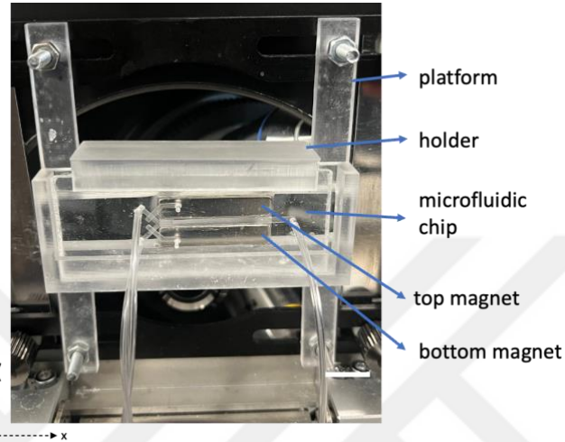
Figure 2.9. A photograph of the platform on an inverted microscope.
