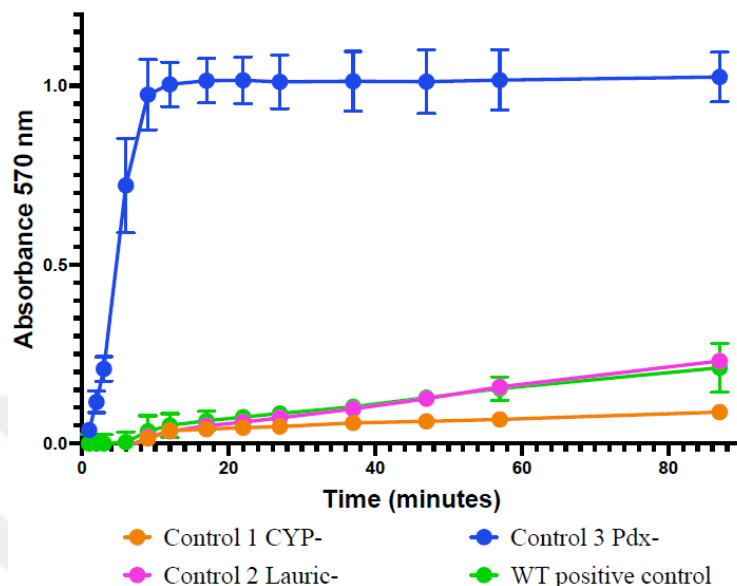
Figure 3.24. \text{H}_2\text{O}_2 formation in a reaction with Control 1 – in the absence of CYP119 (orange), Control 2 – in the absence of lauric acid (pink), Control 3 – in the absence of Pdx (blue), over time, 570 nm was followed for resorufin production, WT positive control (green).
