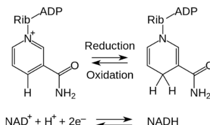
Figure 1.14. NADH oxidation/reduction.
