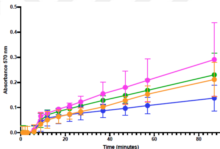
Figure 3.23. \text{H}_2\text{O}_2 formation in a reaction with WT CYP119 (orange), N34E (pink), N34E-D77R (blue), D77R (green) mutations over time, 570 nm was followed for resorufin production.
