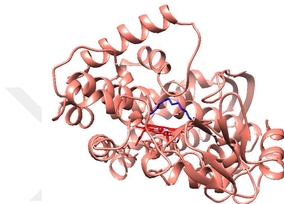
Figure 1.13. CYP119 PDBID: 1IO7. Hydroxylation reaction starts with substrate binding. Lauric acid (in blue) binds CYP119 (in pink) in the region of active site from the distal side of the structure of heme (in red). The image was created with UCSF Chimera.
