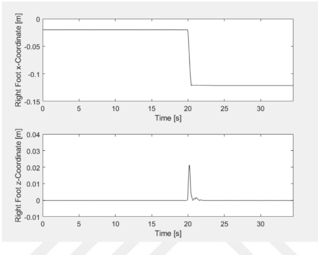
Figure 5.8 Position plot of the right foot, which performs backwards stepping, with respect to z-axis (to visualize the amount of lifting) and x-axis (to visualize the size of the step) of world coordinate frame
