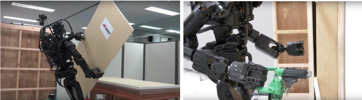
Figure 2.7 HRP-5P Performing Assembly Task without Human Assistance (Kaneko, 2019).
