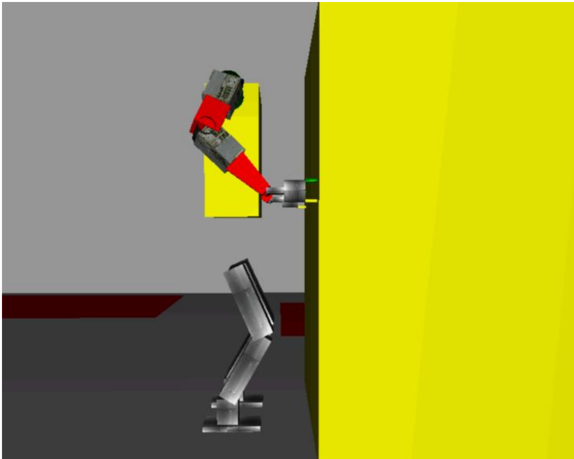
Figure 5.4 Robot arms achieved the first contact to the wall in phase 2
