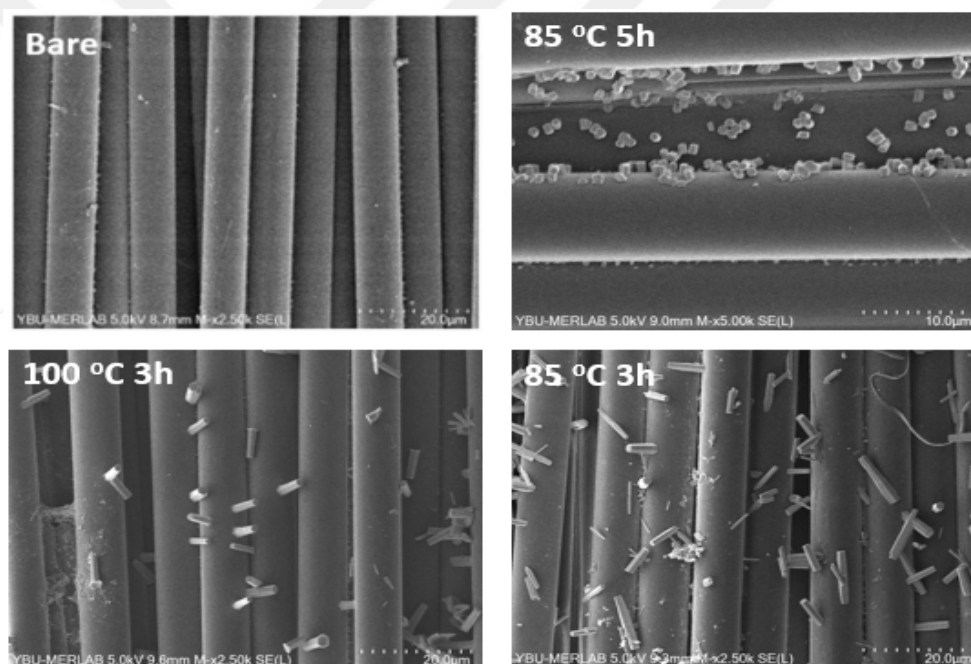
Figure 3.6 SEM images of the ZnO-coated Kevlar™ fabrics without seed layer.
